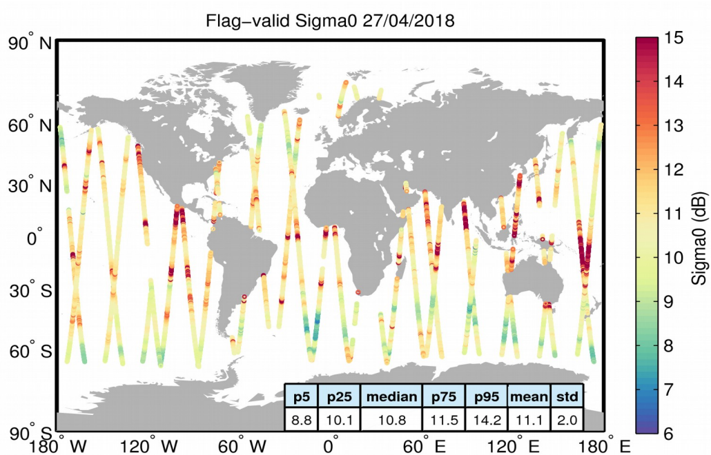
Figure 23. Geographical distribution of flag-valid sigma0 data over oceans and lakes for 27/04/2018. The statistical values shown in the table refer to the sigma0 in dB and are calculated over all measurements shown in the figure.
