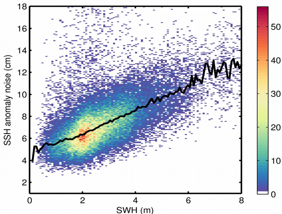
Figure 9. 2D histogram showing flag-valid SSH anomaly noise as a function of SWH for 27/04/2018. The black line denotes the median SSH anomaly noise as a function of SWH.
