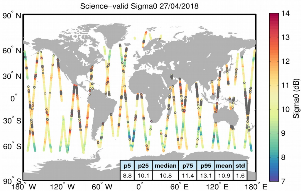
Figure 27. Geographical distribution of science-valid sigma0 data over oceans and lakes for 27/04/2018. The statistical values shown in the table refer to the sigma0 in dB and are calculated over all measurements shown in the figure. Gray circles denote records that have been rejected based on the editing criteria described in Table 4.
