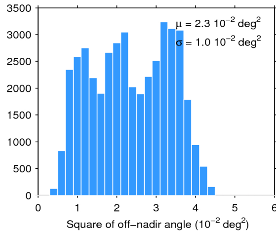
Figure 39. Histogram of flag-valid mispointing over oceans and lakes for 27/04/2018. The mean ( \mu ) and standard deviation ( \sigma ) are also shown. Note that values larger than 6 \cdot 10^{-2} \text{ deg}^2 are excluded from the histogram for the sake of readability but not from the computation of \mu and \sigma .
