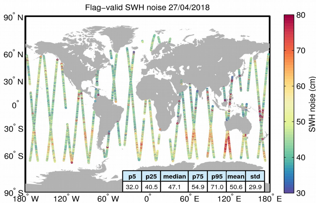
Figure 18. Geographical distribution of flag-valid 20-Hz SWH measurement noise over oceans and lakes for 27/04/2018. The statistical values shown in the figure refer to the SWH noise and are calculated over all measurements shown in the figure.
