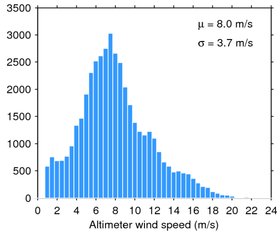
Figure 33. Histogram of flag-valid wind over oceans and lakes for 27/04/2018. The mean ( \mu ) and standard deviation ( \sigma ) are also shown. Note that values larger than 24 m/s are excluded from the histogram for the sake of readability but not from the computation of \mu and \sigma .
