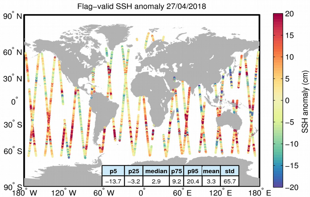
Figure 5. Geographical distribution of flag-valid 1-Hz SSH anomaly data over oceans and lakes for 27/04/2018. The statistical values shown in the table refer to the SSH anomaly in cm and are calculated over all measurements shown in the figure.
