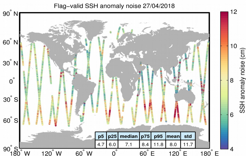
Figure 8. Geographical distribution of flag-valid 20-Hz SSH anomaly measurement noise over oceans and lakes for 27/04/2018. The statistical values shown in the table refer to the SSH anomaly noise and are calculated over all measurements shown in the figure.
