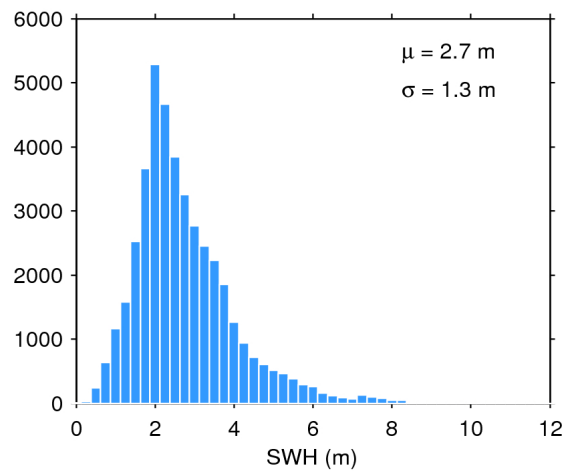
Figure 17. Histogram of flag-valid SWH over oceans and lakes for 27/04/2018. The mean ( \mu ) and standard deviation ( \sigma ) are also shown. Note that values larger than 12 m are excluded from the histogram for the sake of readability but not from the computation of \mu and \sigma .
