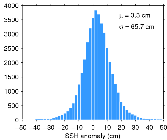
Figure 7. Histogram of flag-valid SSH anomaly over oceans and lakes for 27/04/2018. The mean ( \mu ) and standard deviation ( \sigma ) are also shown. Note that values outside [-50 50] cm are excluded from the histogram for the sake of readability but not from the computation of \mu and \sigma .
