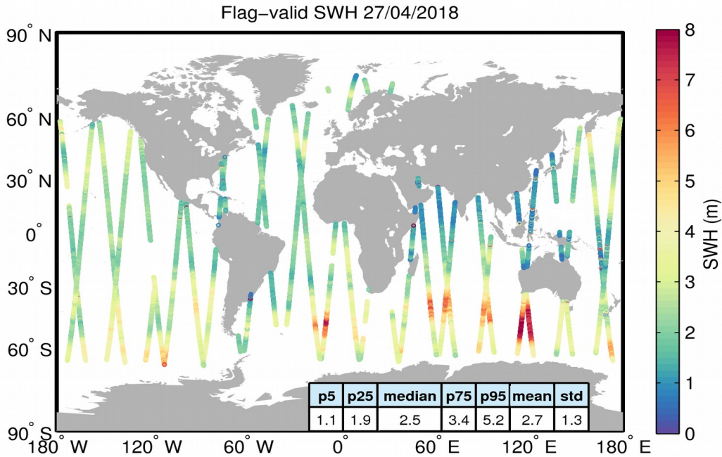
Figure 15. Geographical distribution of flag-valid SWH data over oceans and lakes for 27/04/2018. The statistical values shown in the table refer to the SWH in m and are calculated over all measurements shown in the figure.
