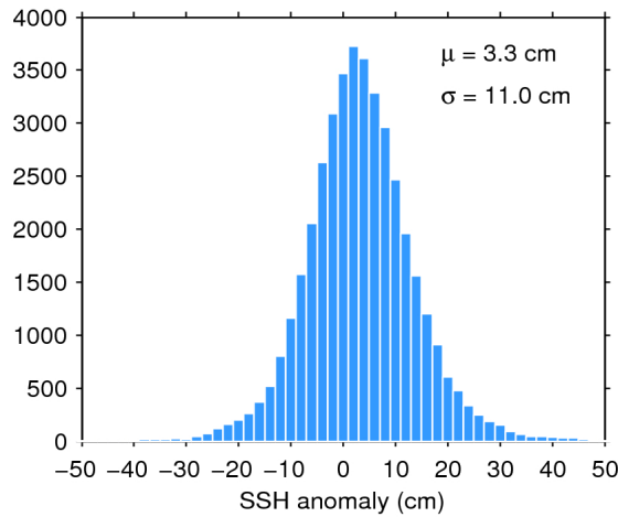
Figure 11. Histogram of science-valid SSH anomaly over oceans and lakes for 27/04/2018. The mean ( \mu ) and standard deviation ( \sigma ) are also shown. Note that values outside [-50 50] cm are excluded from the histogram for the sake of readability but not from the computation of \mu and \sigma .
