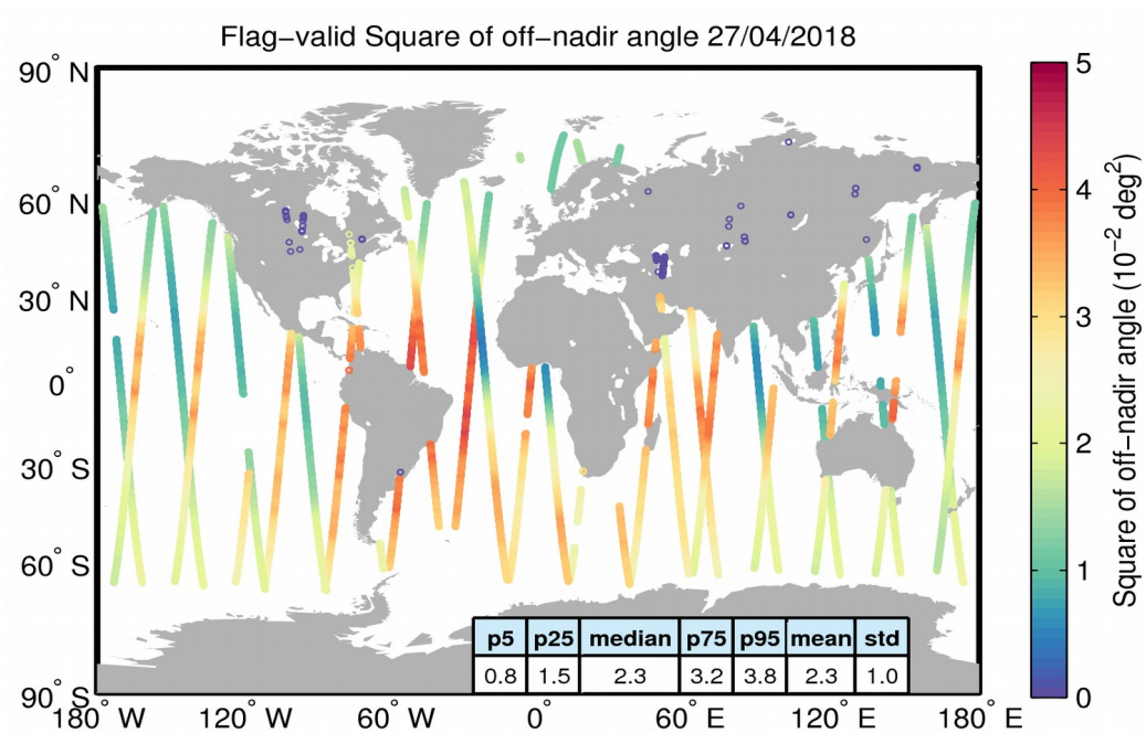
Figure 37. Geographical distribution of flag-valid mispointing data over oceans and lakes for 27/04/2018. The statistical values shown in the table refer to the mispointing in 10^{-2} deg 2 and are calculated over all measurements shown in the figure.
