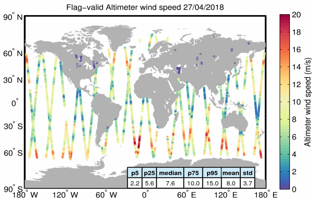
Figure 31. Geographical distribution of flag-valid wind data over oceans and lakes for 27/04/2018. The statistical values shown in the table refer to the wind in m/s and are calculated over all measurements shown in the figure.
