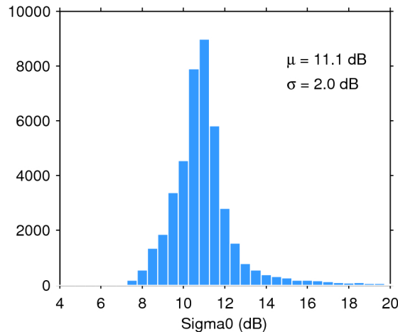
Figure 25. Histogram of flag-valid sigma0 over oceans and lakes for 27/04/2018. The mean ( \mu ) and standard deviation ( \sigma ) are also shown. Note that values outside [4 20] dB are excluded from the histogram for the sake of readability but not from the computation of \mu and \sigma .
