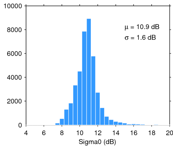
Figure 28. Histogram of science-valid sigma0 over oceans and lakes for 27/04/2018. The mean ( \mu ) and standard deviation ( \sigma ) are also shown. Note that values outside [4 20] dB are excluded from the histogram for the sake of readability but not from the computation of \mu and \sigma .
