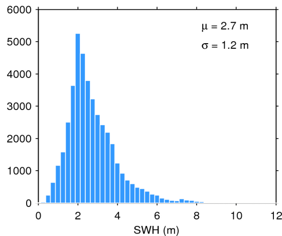
Figure 20. Histogram of science-valid SWH over oceans and lakes for 27/04/2018. The mean ( \mu ) and standard deviation ( \sigma ) are also shown. Note that values larger than 12 m are excluded from the histogram for the sake of readability but not from the computation of \mu and \sigma .
