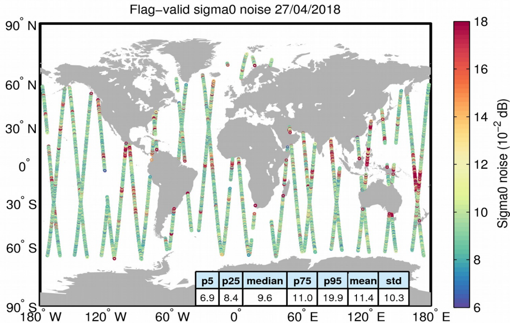
Figure 26. Geographical distribution of flag-valid 20-Hz sigma0 measurement noise over oceans and lakes for 27/04/2018. The statistical values shown in the table refer to the sigma0 noise and are calculated over all measurements shown in the figure.
