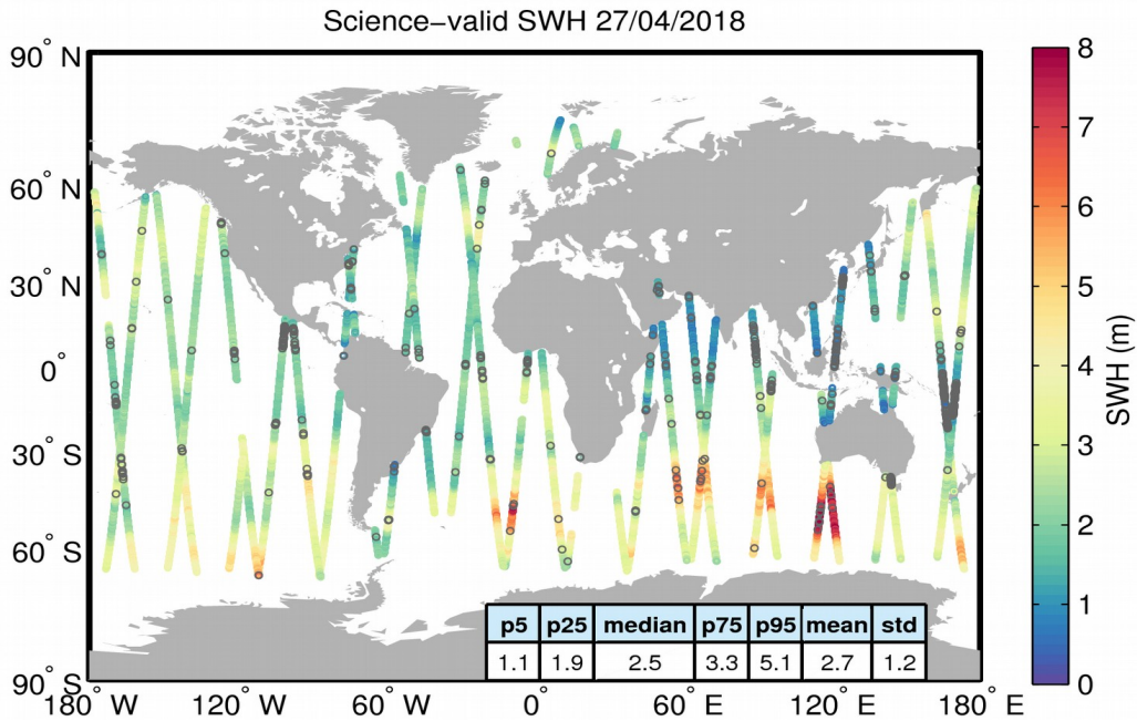
Figure 19. Geographical distribution of science-valid SWH data over oceans and lakes for 27/04/2018. The statistical values shown in the table refer to the SWH in m and are calculated over all measurements shown in the figure. Gray circles denote records that have been rejected based on the editing criteria described in Table 3.
