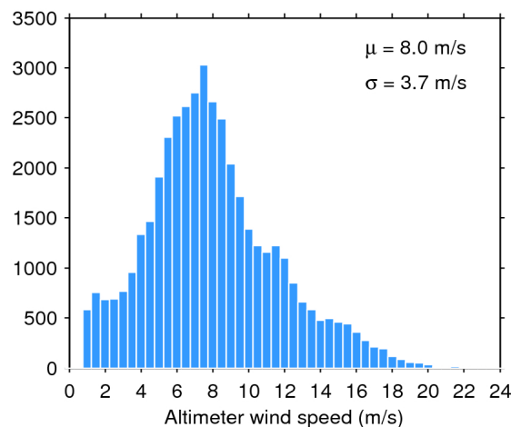
Figure 35. Histogram of science-valid wind over oceans and lakes for 27/04/2018. The mean ( \mu ) and standard deviation ( \sigma ) are also shown. Note that values larger than 24 m/s are excluded from the histogram for the sake of readability but not from the computation of \mu and \sigma .
