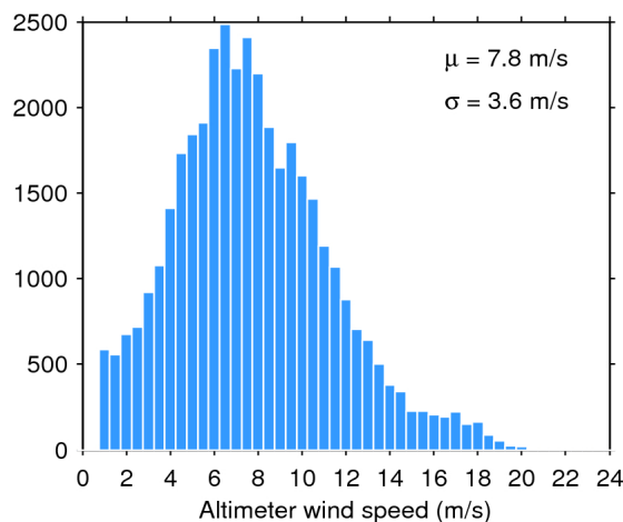
Figure 35. Histogram of science-valid wind over oceans and lakes for 26/04/2018. The mean ( \mu ) and standard deviation ( \sigma ) are also shown. Note that values larger than 24 m/s are excluded from the histogram for the sake of readability but not from the computation of \mu and \sigma .
