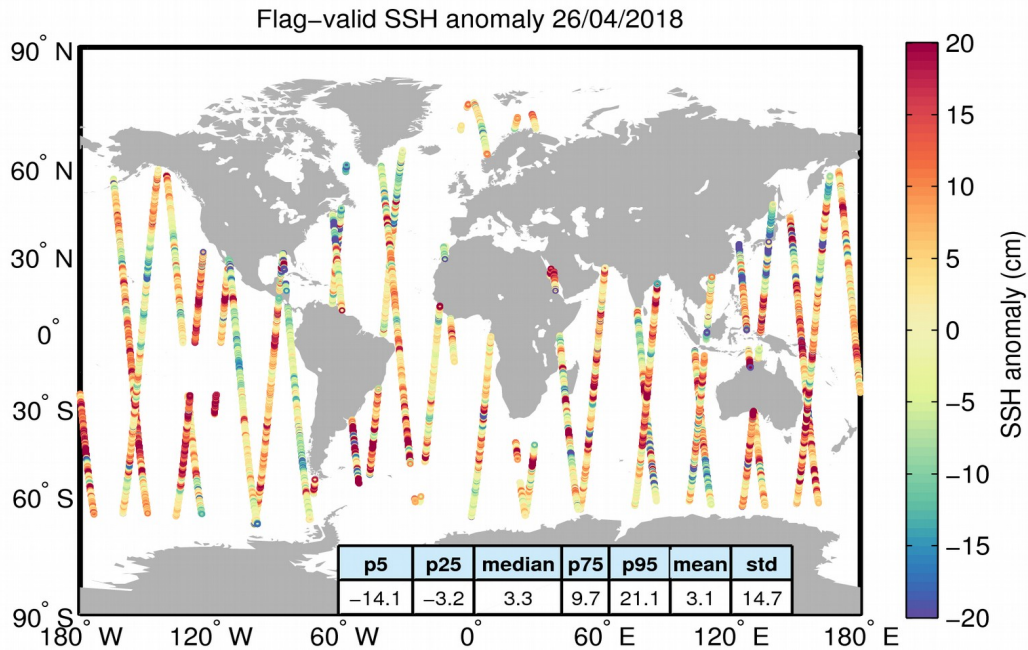
Figure 5. Geographical distribution of flag-valid 1-Hz SSH anomaly data over oceans and lakes for 26/04/2018. The statistical values shown in the table refer to the SSH anomaly in cm and are calculated over all measurements shown in the figure.
