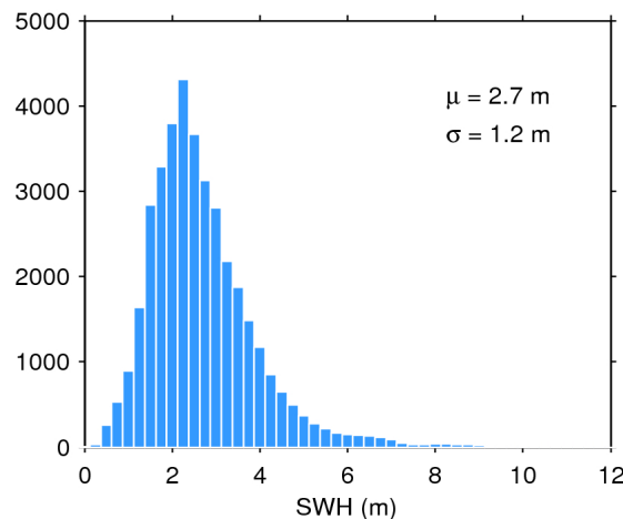
Figure 20. Histogram of science-valid SWH over oceans and lakes for 26/04/2018. The mean ( \mu ) and standard deviation ( \sigma ) are also shown. Note that values larger than 12 m are excluded from the histogram for the sake of readability but not from the computation of \mu and \sigma .
