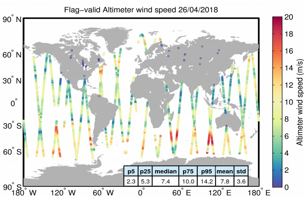
Figure 31. Geographical distribution of flag-valid wind data over oceans and lakes for 26/04/2018. The statistical values shown in the table refer to the wind in m/s and are calculated over all measurements shown in the figure.
