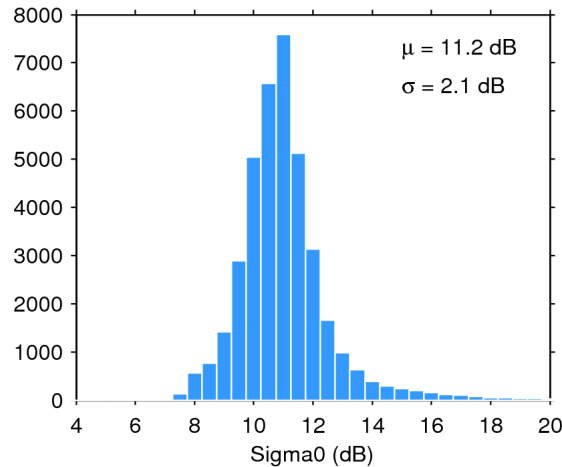
Figure 25. Histogram of flag-valid sigma0 over oceans and lakes for 26/04/2018. The mean ( \mu ) and standard deviation ( \sigma ) are also shown. Note that values outside [4 20] dB are excluded from the histogram for the sake of readability but not from the computation of \mu and \sigma .
