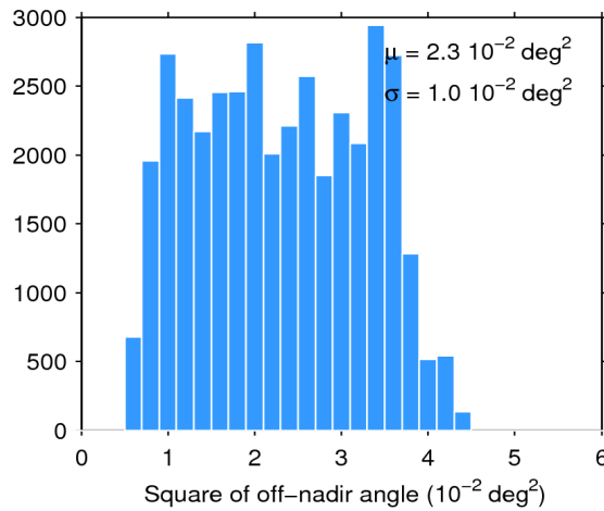
Figure 39. Histogram of flag-valid mispointing over oceans and lakes for 26/04/2018. The mean ( \mu ) and standard deviation ( \sigma ) are also shown. Note that values larger than 6 \cdot 10^{-2} \text{ deg}^2 are excluded from the histogram for the sake of readability but not from the computation of \mu and \sigma .
