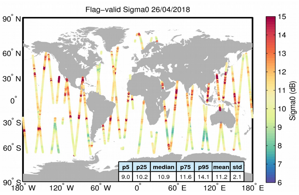
Figure 23. Geographical distribution of flag-valid sigma0 data over oceans and lakes for 26/04/2018. The statistical values shown in the table refer to the sigma0 in dB and are calculated over all measurements shown in the figure.
