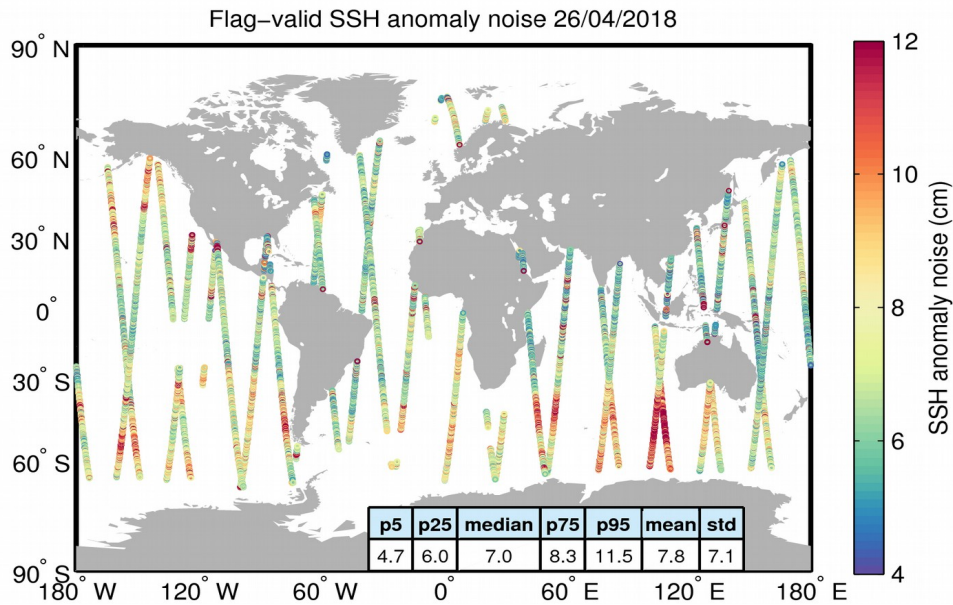
Figure 8. Geographical distribution of flag-valid 20-Hz SSH anomaly measurement noise over oceans and lakes for 26/04/2018. The statistical values shown in the table refer to the SSH anomaly noise and are calculated over all measurements shown in the figure.
