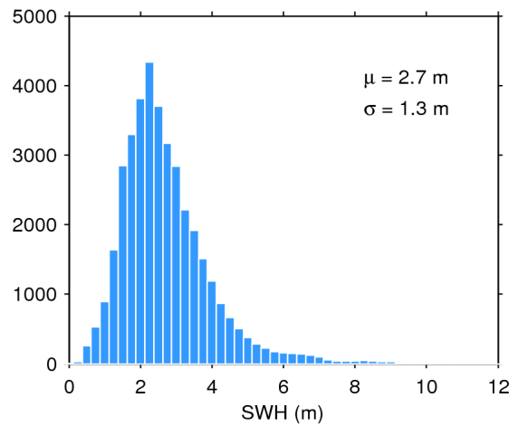
Figure 17. Histogram of flag-valid SWH over oceans and lakes for 26/04/2018. The mean ( \mu ) and standard deviation ( \sigma ) are also shown. Note that values larger than 12 m are excluded from the histogram for the sake of readability but not from the computation of \mu and \sigma .
