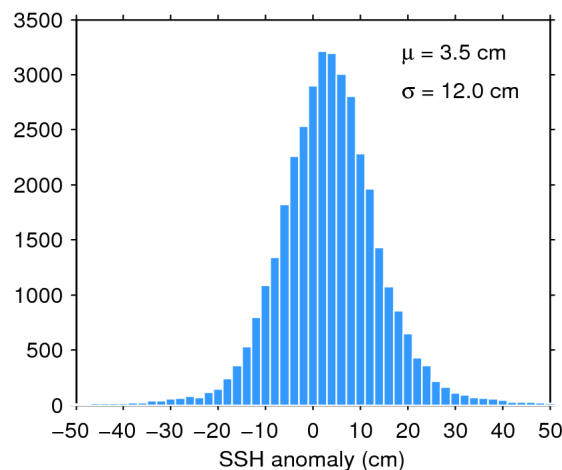
Figure 11. Histogram of science-valid SSH anomaly over oceans and lakes for 26/04/2018. The mean ( \mu ) and standard deviation ( \sigma ) are also shown. Note that values outside [-50 50] cm are excluded from the histogram for the sake of readability but not from the computation of \mu and \sigma .
