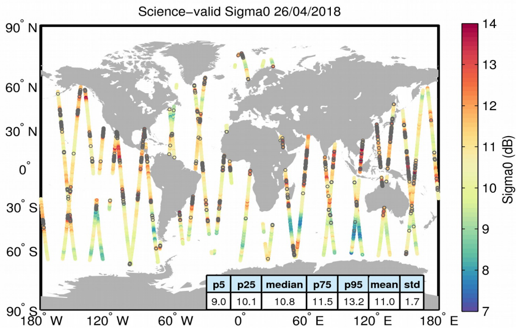
Figure 27. Geographical distribution of science-valid sigma0 data over oceans and lakes for 26/04/2018. The statistical values shown in the table refer to the sigma0 in dB and are calculated over all measurements shown in the figure. Gray circles denote records that have been rejected based on the editing criteria described in Table 4.
