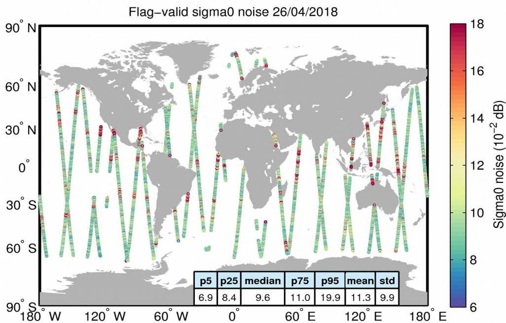
Figure 26. Geographical distribution of flag-valid 20-Hz sigma0 measurement noise over oceans and lakes for 26/04/2018. The statistical values shown in the table refer to the sigma0 noise and are calculated over all measurements shown in the figure.
