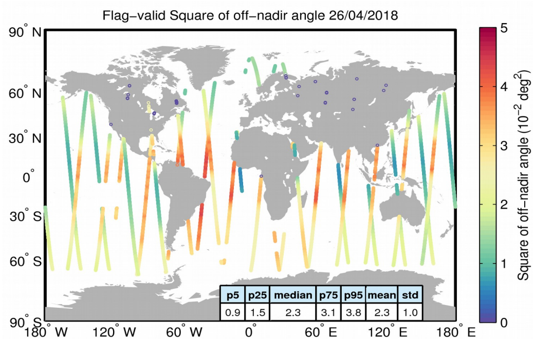
Figure 37. Geographical distribution of flag-valid mispointing data over oceans and lakes for 26/04/2018. The statistical values shown in the table refer to the mispointing in 10^{-2} deg 2 and are calculated over all measurements shown in the figure.
