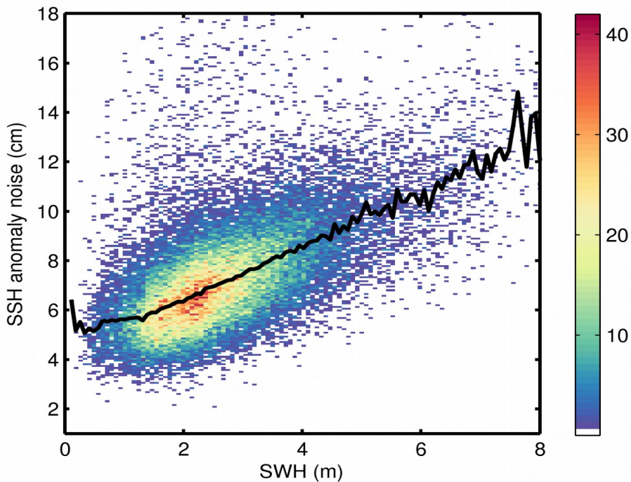
Figure 9. 2D histogram showing flag-valid SSH anomaly noise as a function of SWH for 26/04/2018. The black line denotes the median SSH anomaly noise as a function of SWH.
