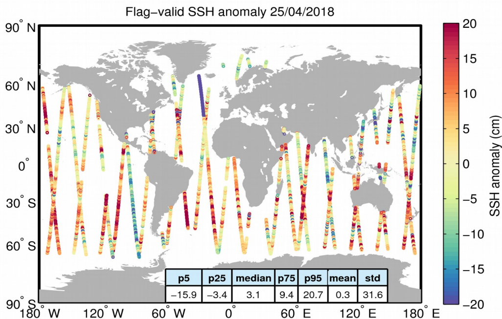
Figure 5. Geographical distribution of flag-valid 1-Hz SSH anomaly data over oceans and lakes for 25/04/2018. The statistical values shown in the table refer to the SSH anomaly in cm and are calculated over all measurements shown in the figure.
