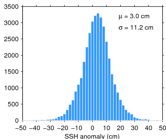
Figure 11. Histogram of science-valid SSH anomaly over oceans and lakes for 25/04/2018. The mean ( \mu ) and standard deviation ( \sigma ) are also shown. Note that values outside [-50 50] cm are excluded from the histogram for the sake of readability but not from the computation of \mu and \sigma .
