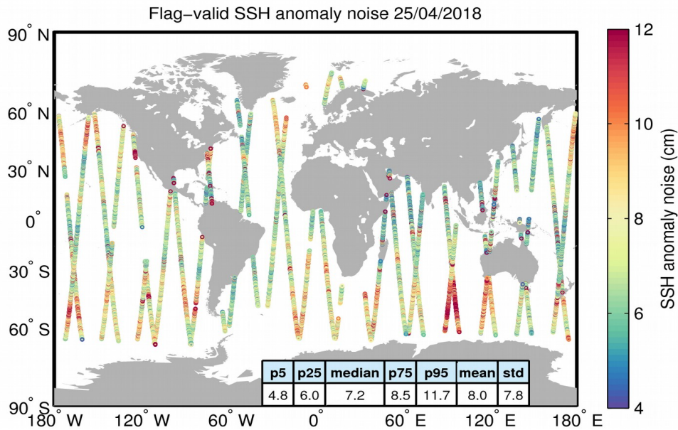
Figure 8. Geographical distribution of flag-valid 20-Hz SSH anomaly measurement noise over oceans and lakes for 25/04/2018. The statistical values shown in the table refer to the SSH anomaly noise and are calculated over all measurements shown in the figure.
