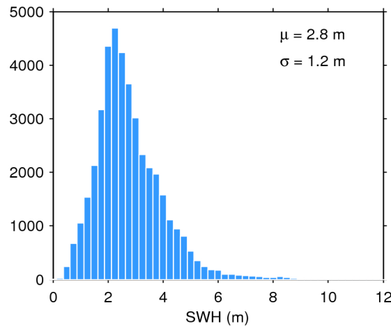
Figure 20. Histogram of science-valid SWH over oceans and lakes for 25/04/2018. The mean ( \mu ) and standard deviation ( \sigma ) are also shown. Note that values larger than 12 m are excluded from the histogram for the sake of readability but not from the computation of \mu and \sigma .
