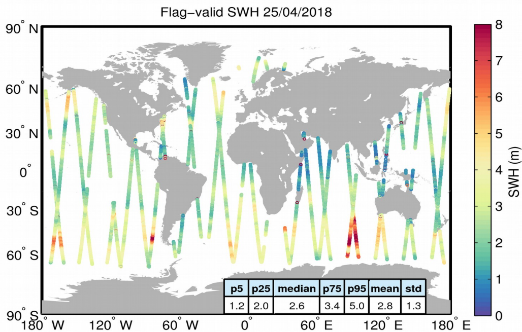
Figure 15. Geographical distribution of flag-valid SWH data over oceans and lakes for 25/04/2018. The statistical values shown in the table refer to the SWH in m and are calculated over all measurements shown in the figure.
