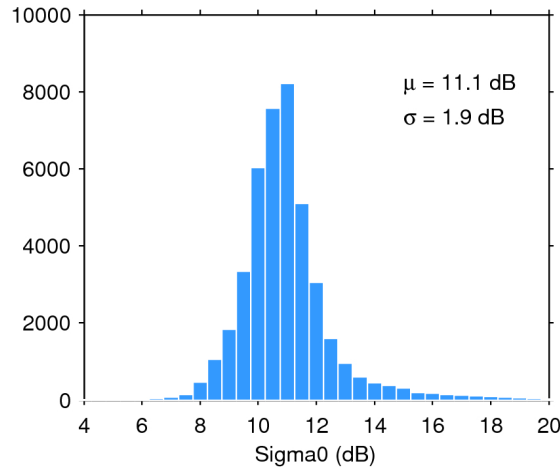
Figure 25. Histogram of flag-valid sigma0 over oceans and lakes for 25/04/2018. The mean ( \mu ) and standard deviation ( \sigma ) are also shown. Note that values outside [4 20] dB are excluded from the histogram for the sake of readability but not from the computation of \mu and \sigma .
