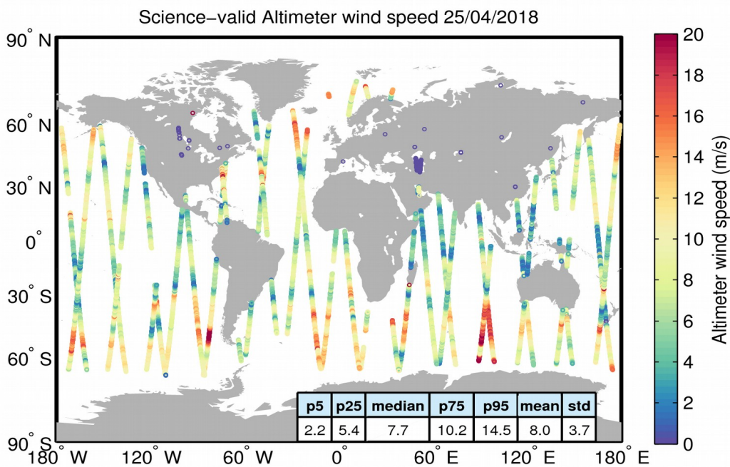
Figure 34. Geographical distribution of science-valid wind data over oceans and lakes for 25/04/2018. The statistical values shown in the table refer to the wind in m/s and are calculated over all measurements shown in the figure. Gray circles denote records that have been rejected based on the editing criteria described in Table 5.
