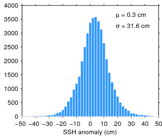
Figure 7. Histogram of flag-valid SSH anomaly over oceans and lakes for 25/04/2018. The mean ( \mu ) and standard deviation ( \sigma ) are also shown. Note that values outside [-50 50] cm are excluded from the histogram for the sake of readability but not from the computation of \mu and \sigma .
