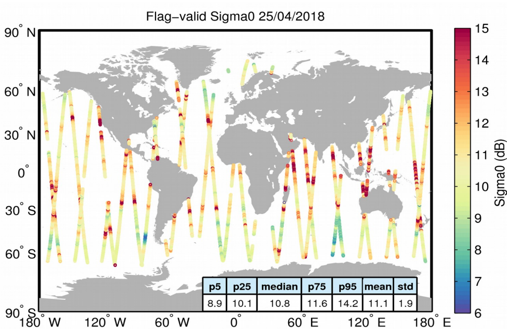
Figure 23. Geographical distribution of flag-valid sigma0 data over oceans and lakes for 25/04/2018. The statistical values shown in the table refer to the sigma0 in dB and are calculated over all measurements shown in the figure.
