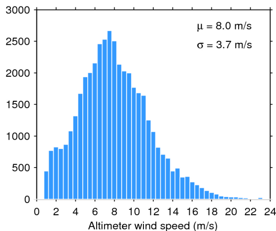
Figure 35. Histogram of science-valid wind over oceans and lakes for 25/04/2018. The mean ( \mu ) and standard deviation ( \sigma ) are also shown. Note that values larger than 24 m/s are excluded from the histogram for the sake of readability but not from the computation of \mu and \sigma .
