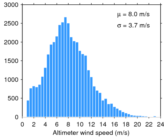
Figure 33. Histogram of flag-valid wind over oceans and lakes for 25/04/2018. The mean ( \mu ) and standard deviation ( \sigma ) are also shown. Note that values larger than 24 m/s are excluded from the histogram for the sake of readability but not from the computation of \mu and \sigma .
