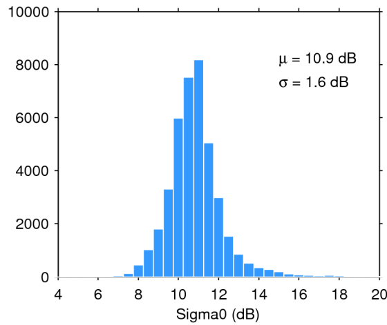
Figure 28. Histogram of science-valid sigma0 over oceans and lakes for 25/04/2018. The mean ( \mu ) and standard deviation ( \sigma ) are also shown. Note that values outside [4 20] dB are excluded from the histogram for the sake of readability but not from the computation of \mu and \sigma .
