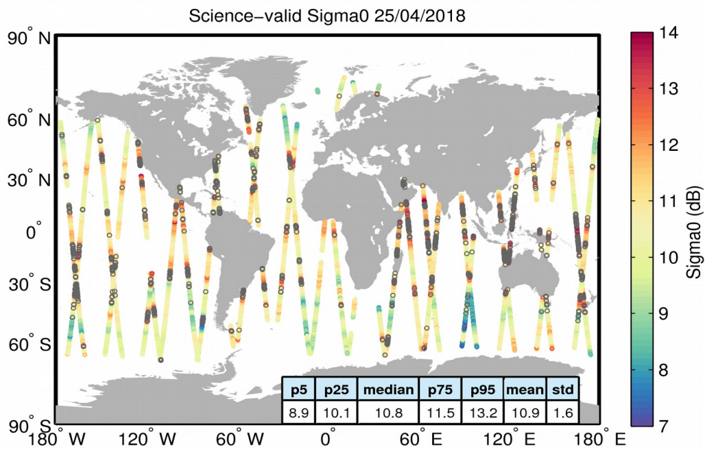
Figure 27. Geographical distribution of science-valid sigma0 data over oceans and lakes for 25/04/2018. The statistical values shown in the table refer to the sigma0 in dB and are calculated over all measurements shown in the figure. Gray circles denote records that have been rejected based on the editing criteria described in Table 4.
