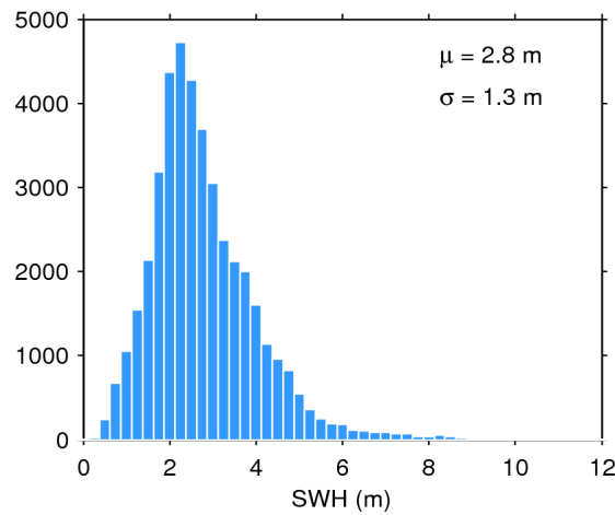
Figure 17. Histogram of flag-valid SWH over oceans and lakes for 25/04/2018. The mean ( \mu ) and standard deviation ( \sigma ) are also shown. Note that values larger than 12 m are excluded from the histogram for the sake of readability but not from the computation of \mu and \sigma .
