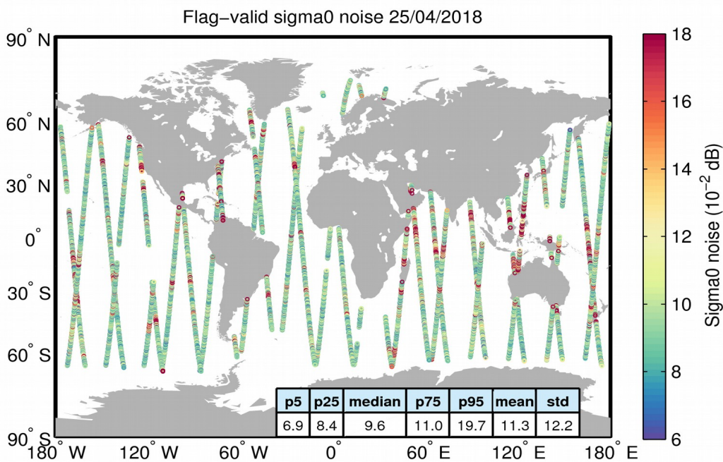
Figure 26. Geographical distribution of flag-valid 20-Hz sigma0 measurement noise over oceans and lakes for 25/04/2018. The statistical values shown in the table refer to the sigma0 noise and are calculated over all measurements shown in the figure.
