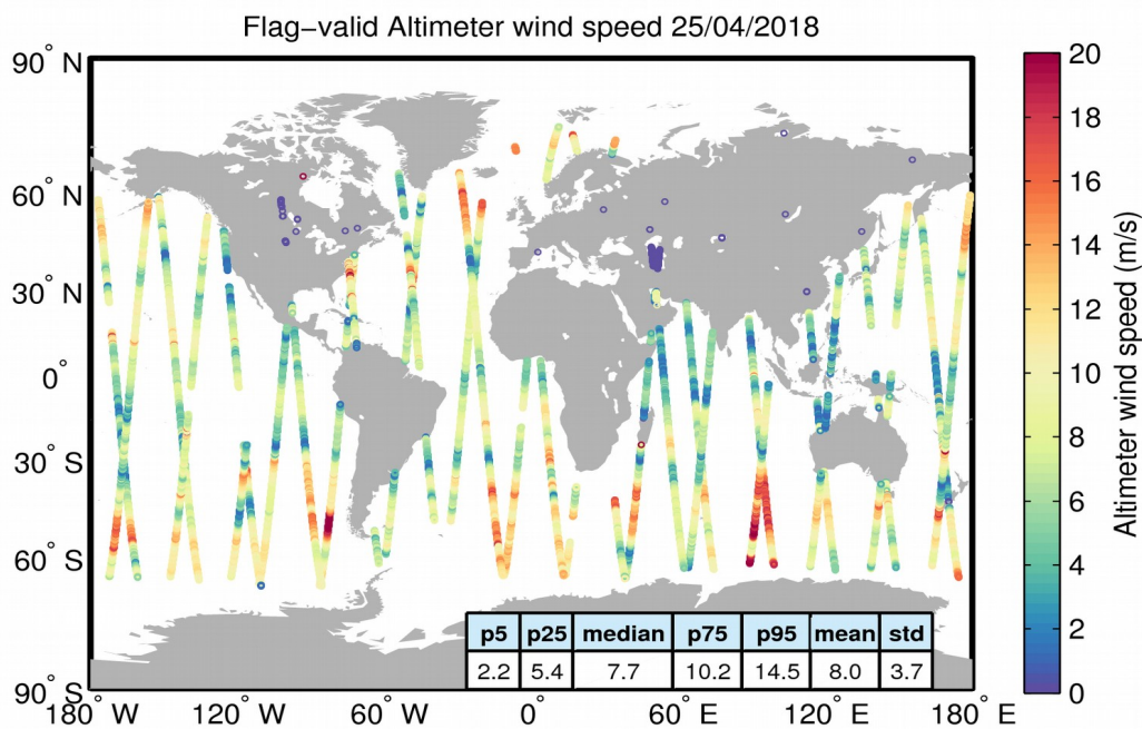
Figure 31. Geographical distribution of flag-valid wind data over oceans and lakes for 25/04/2018. The statistical values shown in the table refer to the wind in m/s and are calculated over all measurements shown in the figure.
