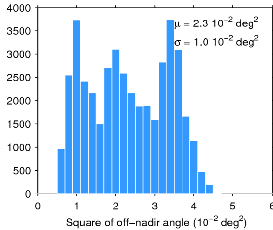
Figure 39. Histogram of flag-valid mispointing over oceans and lakes for 25/04/2018. The mean ( \mu ) and standard deviation ( \sigma ) are also shown. Note that values larger than 6 \cdot 10^{-2} \text{ deg}^2 are excluded from the histogram for the sake of readability but not from the computation of \mu and \sigma .
