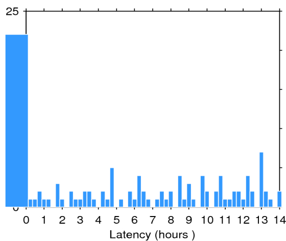
Figure 2. Histogram of the data latency for 24/04/2018. The y-axis denotes the number of files that are made available with a delay of x-hours with respect to the mean time of the records stored in the file.
