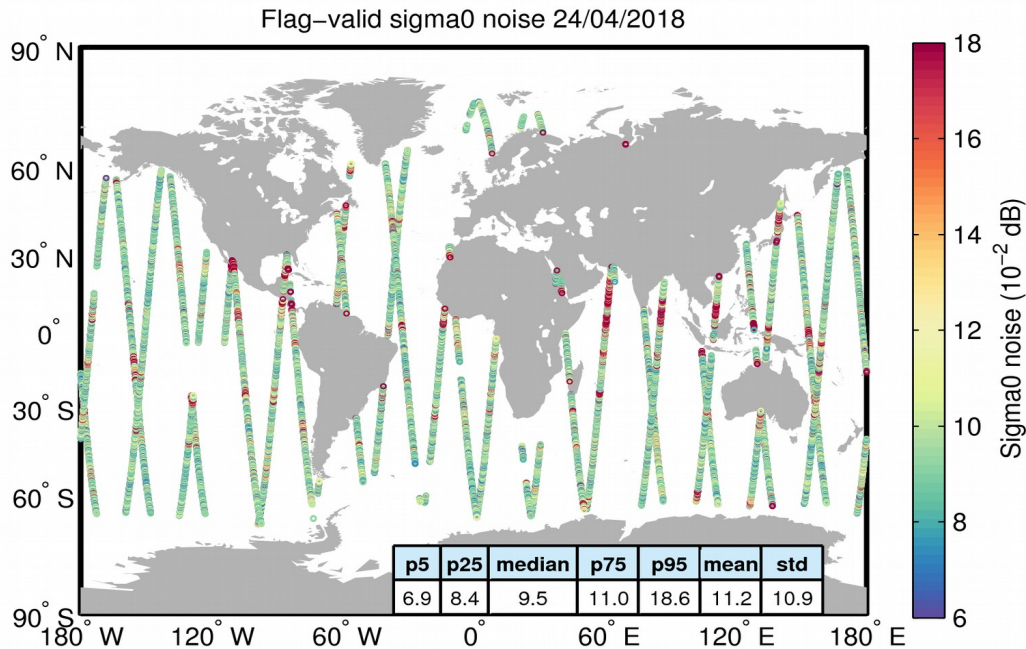
Figure 26. Geographical distribution of flag-valid 20-Hz sigma0 measurement noise over oceans and lakes for 24/04/2018. The statistical values shown in the table refer to the sigma0 noise and are calculated over all measurements shown in the figure.
