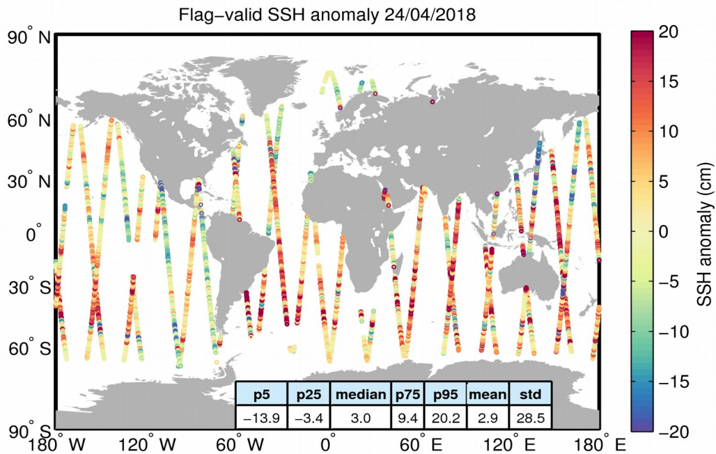
Figure 5. Geographical distribution of flag-valid 1-Hz SSH anomaly data over oceans and lakes for 24/04/2018. The statistical values shown in the table refer to the SSH anomaly in cm and are calculated over all measurements shown in the figure.
