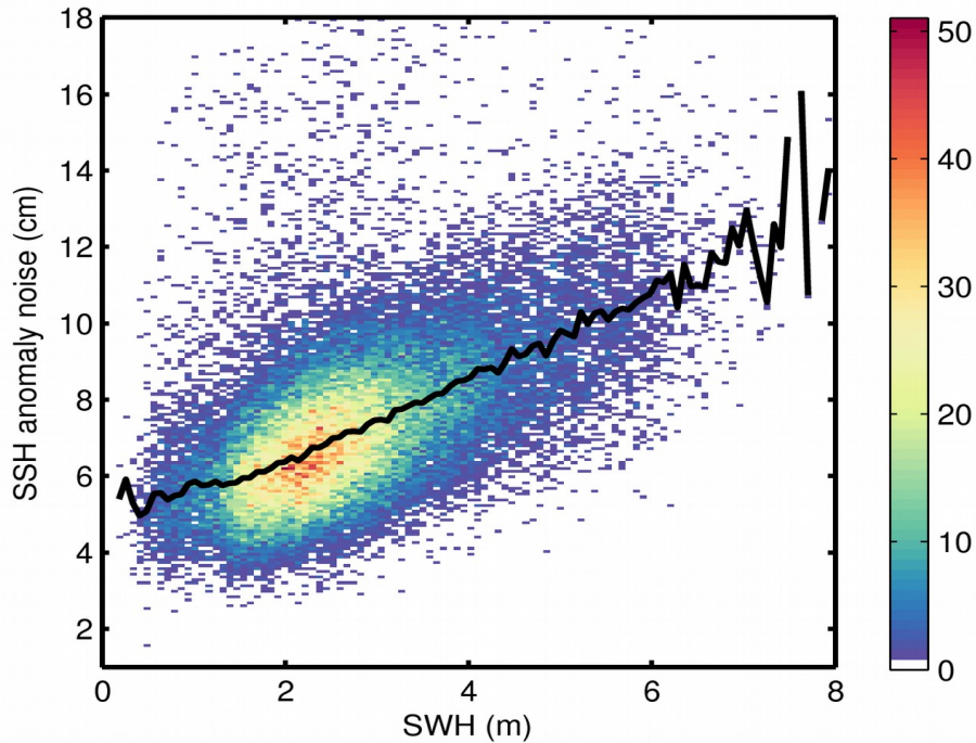
Figure 9. 2D histogram showing flag-valid SSH anomaly noise as a function of SWH for 24/04/2018. The black line denotes the median SSH anomaly noise as a function of SWH.
