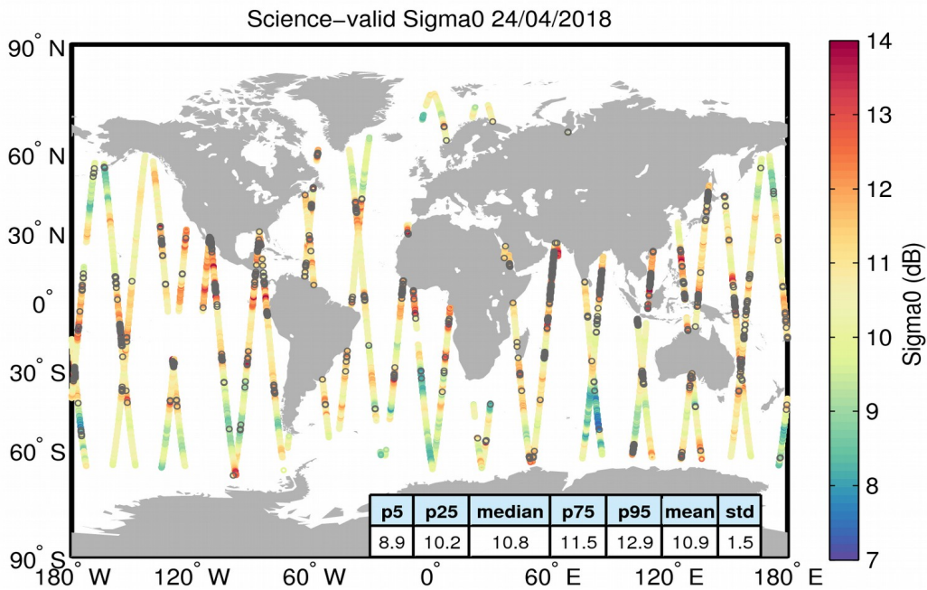
Figure 27. Geographical distribution of science-valid sigma0 data over oceans and lakes for 24/04/2018. The statistical values shown in the table refer to the sigma0 in dB and are calculated over all measurements shown in the figure. Gray circles denote records that have been rejected based on the editing criteria described in Table 4.
