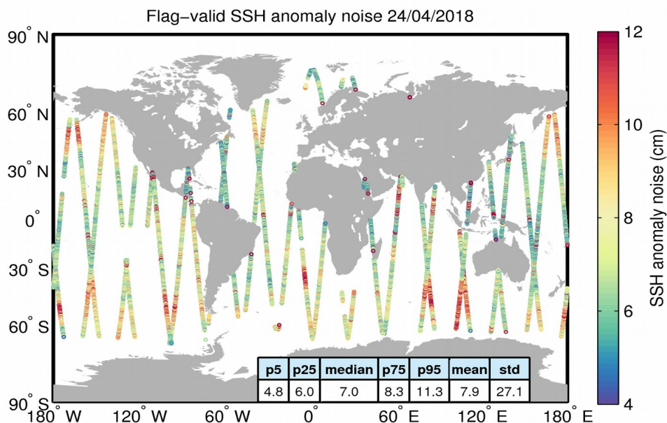
Figure 8. Geographical distribution of flag-valid 20-Hz SSH anomaly measurement noise over oceans and lakes for 24/04/2018. The statistical values shown in the table refer to the SSH anomaly noise and are calculated over all measurements shown in the figure.
