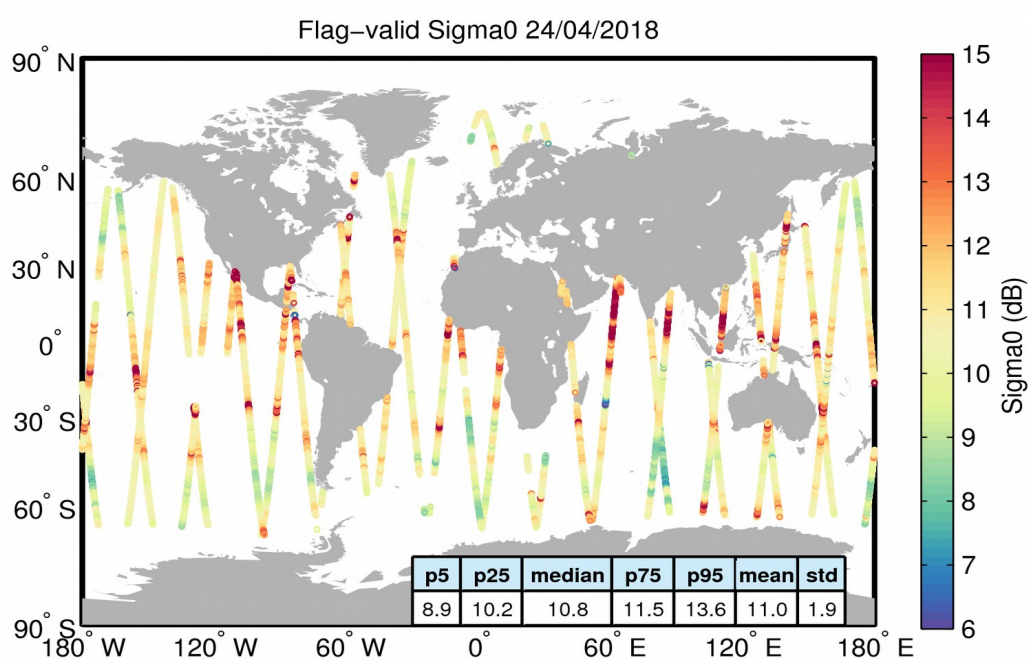
Figure 23. Geographical distribution of flag-valid sigma0 data over oceans and lakes for 24/04/2018. The statistical values shown in the table refer to the sigma0 in dB and are calculated over all measurements shown in the figure.
