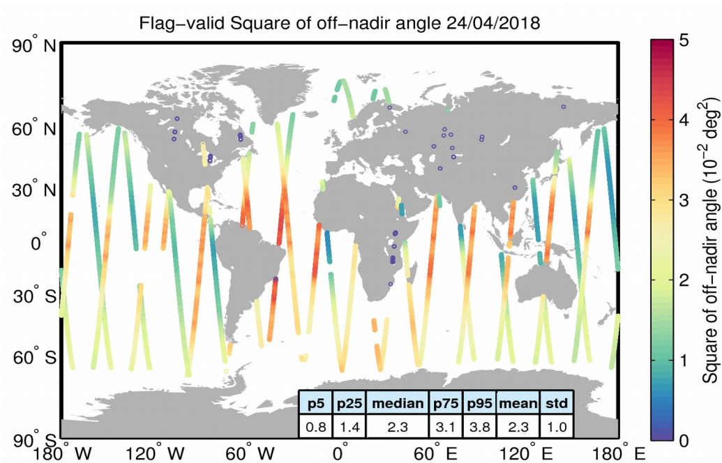
Figure 37. Geographical distribution of flag-valid mispointing data over oceans and lakes for 24/04/2018. The statistical values shown in the table refer to the mispointing in 10^{-2} deg 2 and are calculated over all measurements shown in the figure.
