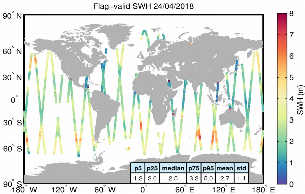
Figure 15. Geographical distribution of flag-valid SWH data over oceans and lakes for 24/04/2018. The statistical values shown in the table refer to the SWH in m and are calculated over all measurements shown in the figure.
