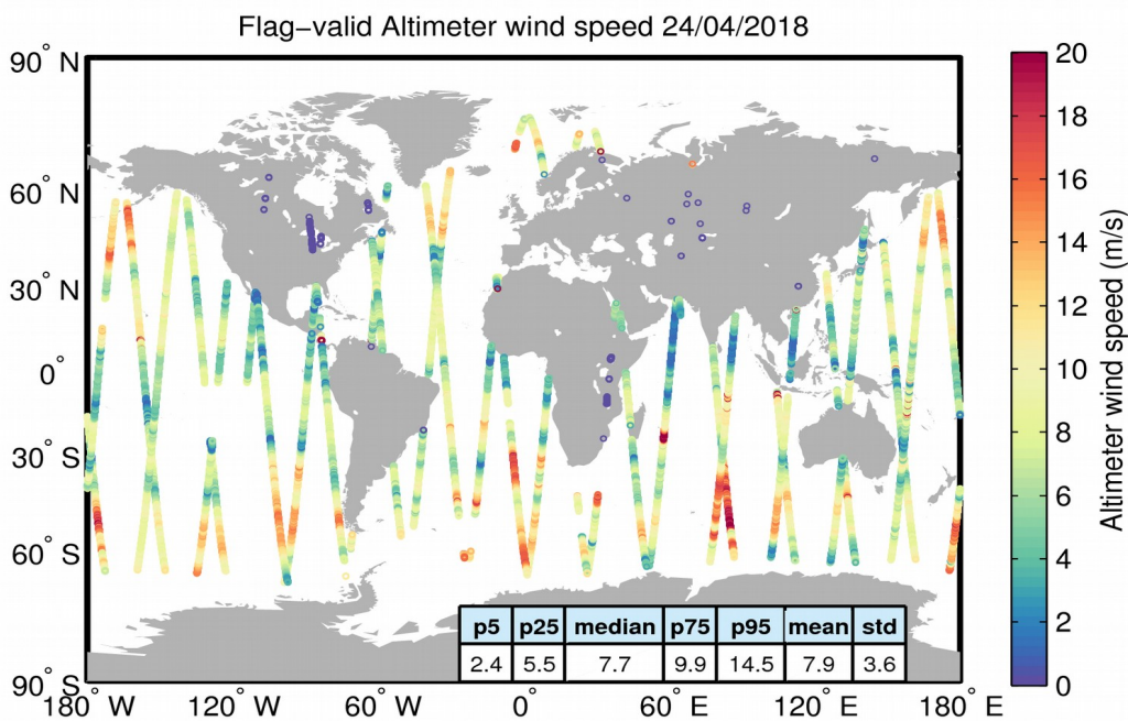
Figure 31. Geographical distribution of flag-valid wind data over oceans and lakes for 24/04/2018. The statistical values shown in the table refer to the wind in m/s and are calculated over all measurements shown in the figure.
