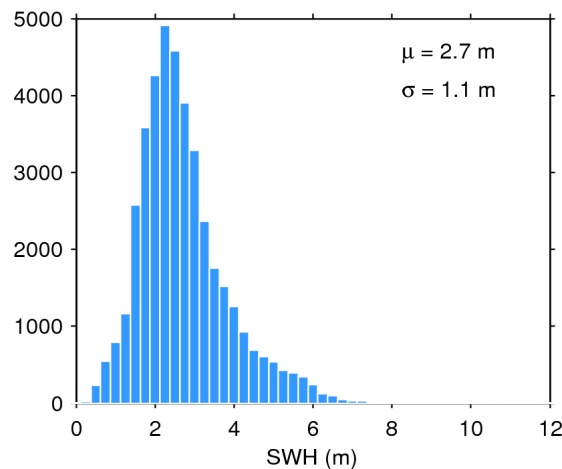
Figure 17. Histogram of flag-valid SWH over oceans and lakes for 24/04/2018. The mean ( \mu ) and standard deviation ( \sigma ) are also shown. Note that values larger than 12 m are excluded from the histogram for the sake of readability but not from the computation of \mu and \sigma .
