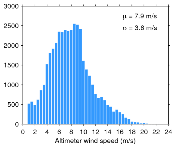
Figure 35. Histogram of science-valid wind over oceans and lakes for 24/04/2018. The mean ( \mu ) and standard deviation ( \sigma ) are also shown. Note that values larger than 24 m/s are excluded from the histogram for the sake of readability but not from the computation of \mu and \sigma .
