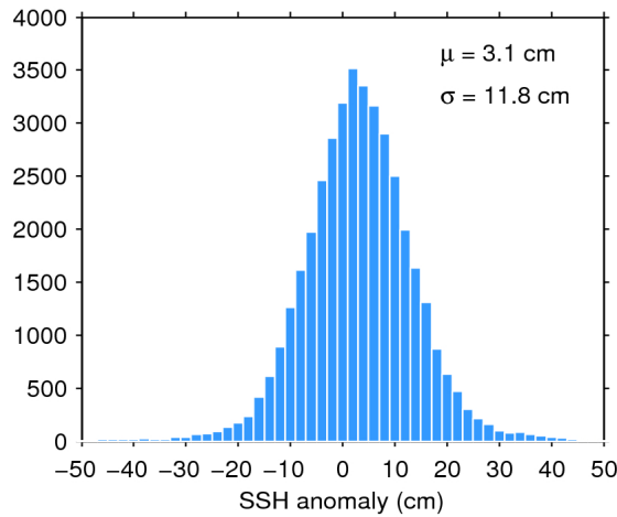
Figure 11. Histogram of science-valid SSH anomaly over oceans and lakes for 24/04/2018. The mean ( \mu ) and standard deviation ( \sigma ) are also shown. Note that values outside [-50 50] cm are excluded from the histogram for the sake of readability but not from the computation of \mu and \sigma .
