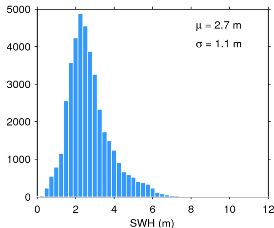
Figure 20. Histogram of science-valid SWH over oceans and lakes for 24/04/2018. The mean ( \mu ) and standard deviation ( \sigma ) are also shown. Note that values larger than 12 m are excluded from the histogram for the sake of readability but not from the computation of \mu and \sigma .
