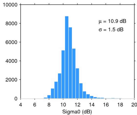
Figure 28. Histogram of science-valid sigma0 over oceans and lakes for 24/04/2018. The mean ( \mu ) and standard deviation ( \sigma ) are also shown. Note that values outside [4 20] dB are excluded from the histogram for the sake of readability but not from the computation of \mu and \sigma .
