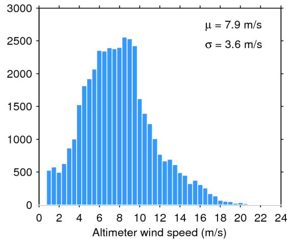
Figure 33. Histogram of flag-valid wind over oceans and lakes for 24/04/2018. The mean ( \mu ) and standard deviation ( \sigma ) are also shown. Note that values larger than 24 m/s are excluded from the histogram for the sake of readability but not from the computation of \mu and \sigma .
