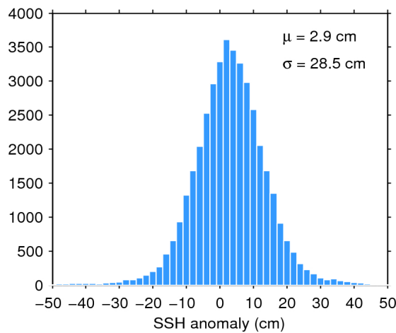
Figure 7. Histogram of flag-valid SSH anomaly over oceans and lakes for 24/04/2018. The mean ( \mu ) and standard deviation ( \sigma ) are also shown. Note that values outside [-50 50] cm are excluded from the histogram for the sake of readability but not from the computation of \mu and \sigma .
