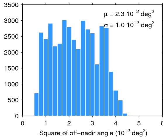
Figure 39. Histogram of flag-valid mispointing over oceans and lakes for 24/04/2018. The mean ( \mu ) and standard deviation ( \sigma ) are also shown. Note that values larger than 6 \cdot 10^{-2} \text{ deg}^2 are excluded from the histogram for the sake of readability but not from the computation of \mu and \sigma .
