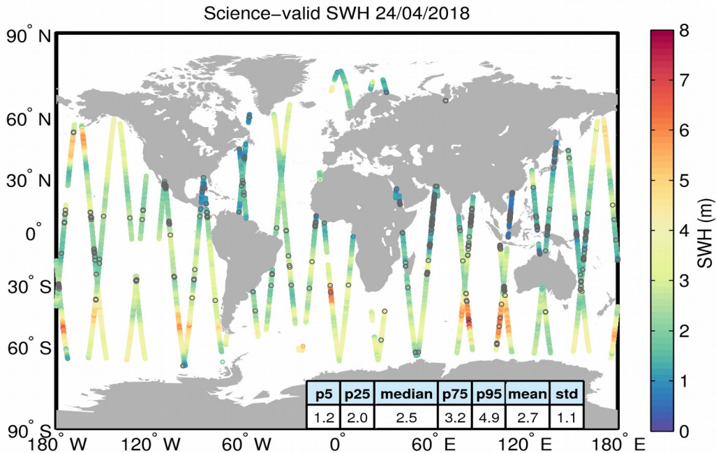
Figure 19. Geographical distribution of science-valid SWH data over oceans and lakes for 24/04/2018. The statistical values shown in the table refer to the SWH in m and are calculated over all measurements shown in the figure. Gray circles denote records that have been rejected based on the editing criteria described in Table 3.
