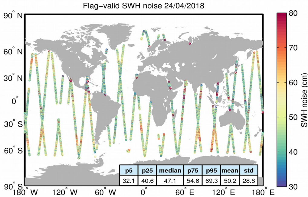
Figure 18. Geographical distribution of flag-valid 20-Hz SWH measurement noise over oceans and lakes for 24/04/2018. The statistical values shown in the figure refer to the SWH noise and are calculated over all measurements shown in the figure.
