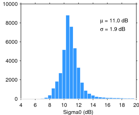
Figure 25. Histogram of flag-valid sigma0 over oceans and lakes for 24/04/2018. The mean ( \mu ) and standard deviation ( \sigma ) are also shown. Note that values outside [4 20] dB are excluded from the histogram for the sake of readability but not from the computation of \mu and \sigma .
