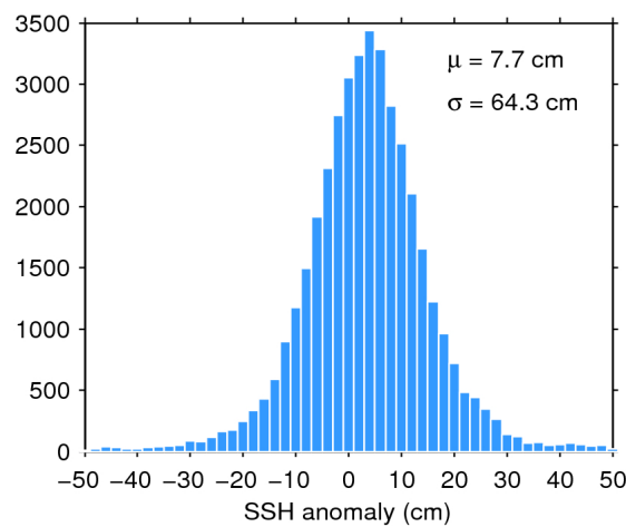
Figure 7. Histogram of flag-valid SSH anomaly over oceans and lakes for 23/04/2018. The mean ( \mu ) and standard deviation ( \sigma ) are also shown. Note that values outside [-50 50] cm are excluded from the histogram for the sake of readability but not from the computation of \mu and \sigma .
