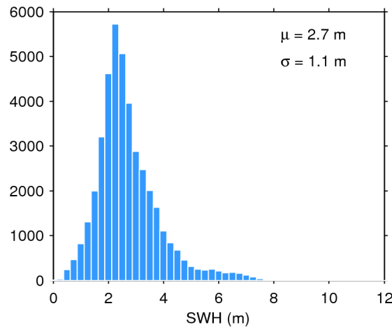
Figure 20. Histogram of science-valid SWH over oceans and lakes for 23/04/2018. The mean ( \mu ) and standard deviation ( \sigma ) are also shown. Note that values larger than 12 m are excluded from the histogram for the sake of readability but not from the computation of \mu and \sigma .
