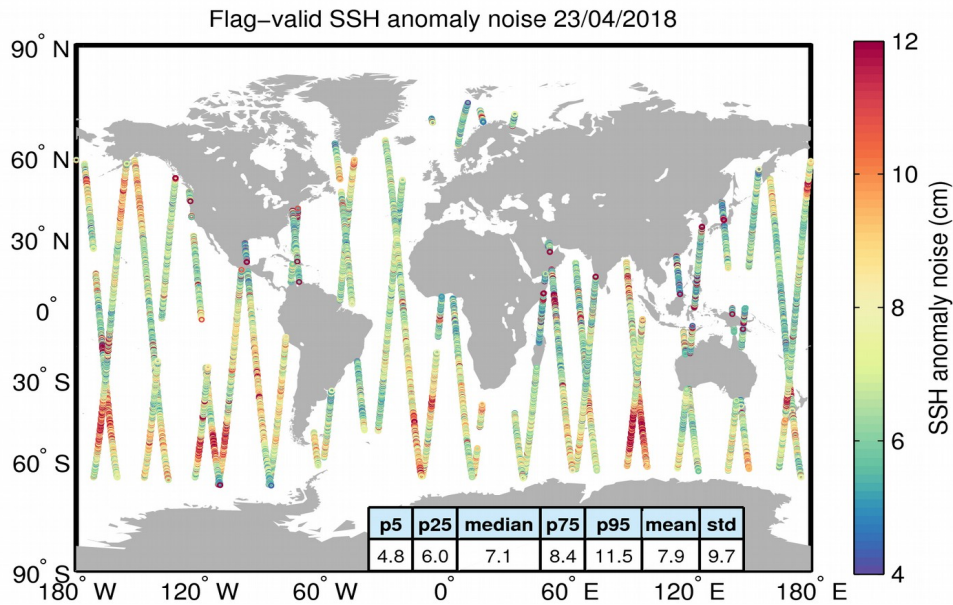
Figure 8. Geographical distribution of flag-valid 20-Hz SSH anomaly measurement noise over oceans and lakes for 23/04/2018. The statistical values shown in the table refer to the SSH anomaly noise and are calculated over all measurements shown in the figure.
