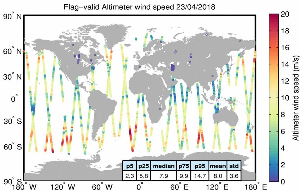
Figure 31. Geographical distribution of flag-valid wind data over oceans and lakes for 23/04/2018. The statistical values shown in the table refer to the wind in m/s and are calculated over all measurements shown in the figure.
