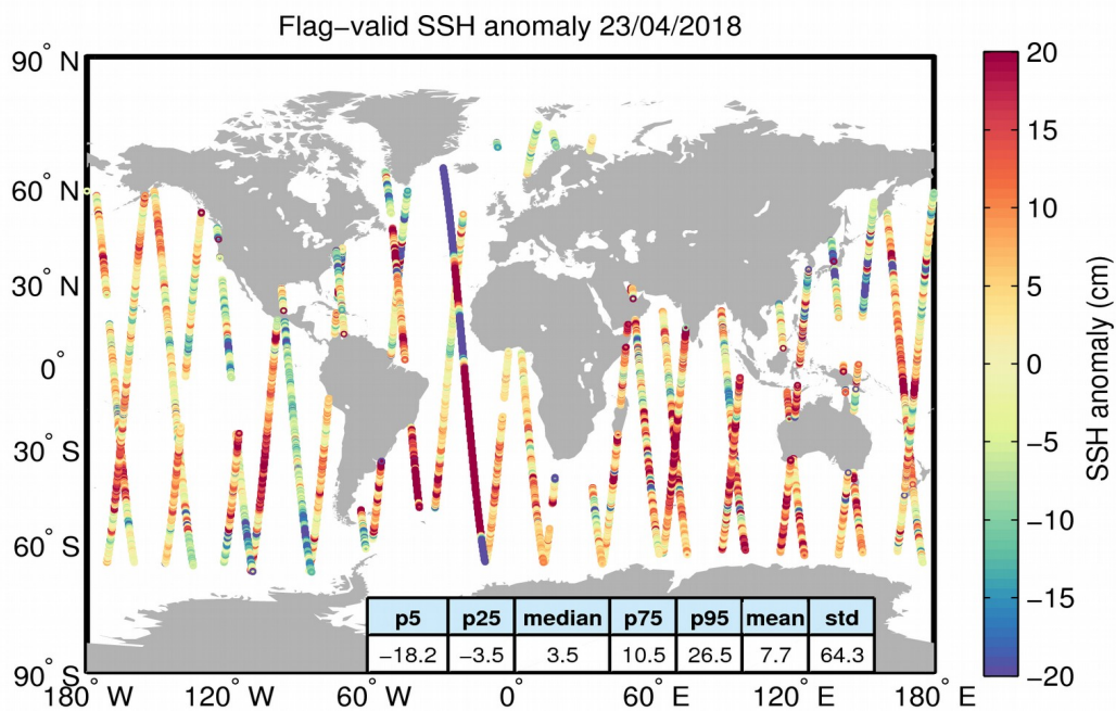
Figure 5. Geographical distribution of flag-valid 1-Hz SSH anomaly data over oceans and lakes for 23/04/2018. The statistical values shown in the table refer to the SSH anomaly in cm and are calculated over all measurements shown in the figure.
