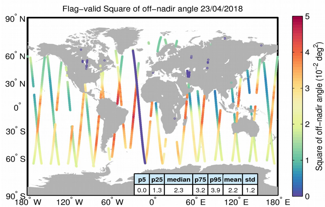
Figure 37. Geographical distribution of flag-valid mispointing data over oceans and lakes for 23/04/2018. The statistical values shown in the table refer to the mispointing in 10^{-2} \text{ deg}^2 and are calculated over all measurements shown in the figure.
