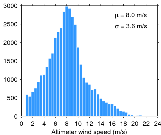
Figure 35. Histogram of science-valid wind over oceans and lakes for 23/04/2018. The mean ( \mu ) and standard deviation ( \sigma ) are also shown. Note that values larger than 24 m/s are excluded from the histogram for the sake of readability but not from the computation of \mu and \sigma .
