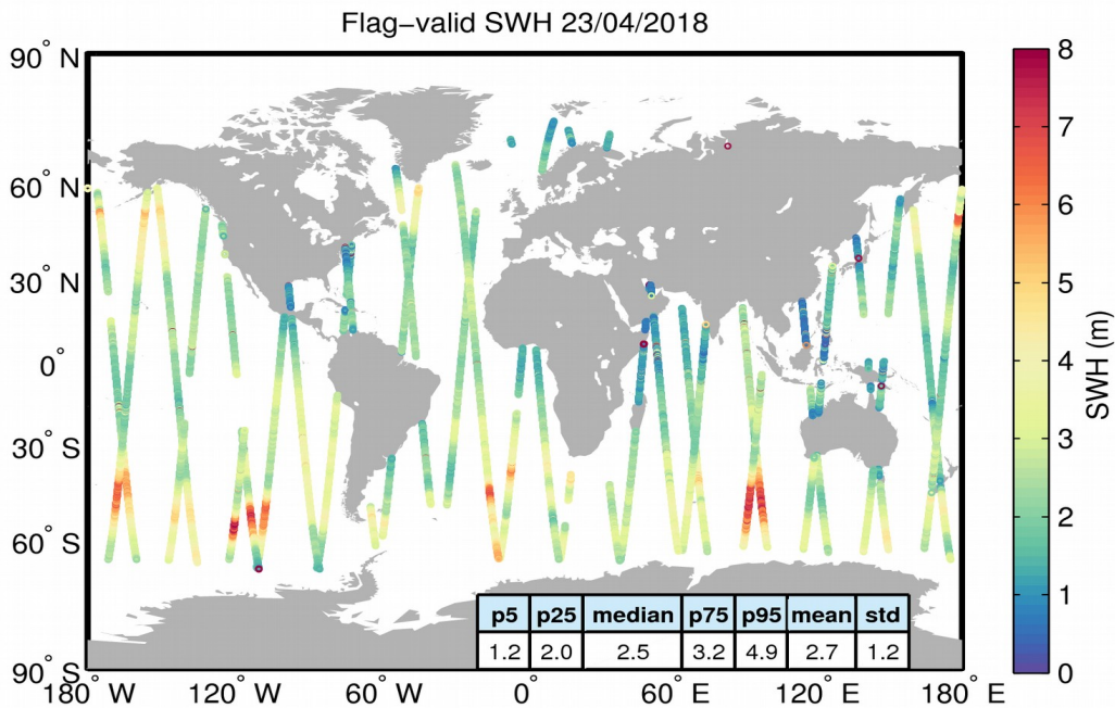
Figure 15. Geographical distribution of flag-valid SWH data over oceans and lakes for 23/04/2018. The statistical values shown in the table refer to the SWH in m and are calculated over all measurements shown in the figure.
