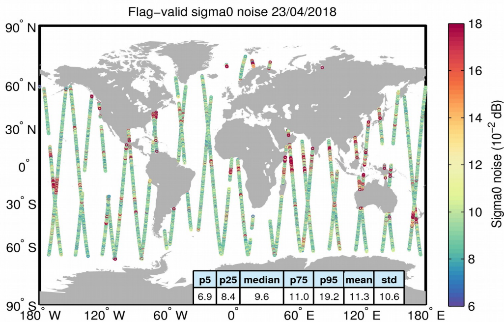
Figure 26. Geographical distribution of flag-valid 20-Hz sigma0 measurement noise over oceans and lakes for 23/04/2018. The statistical values shown in the table refer to the sigma0 noise and are calculated over all measurements shown in the figure.
