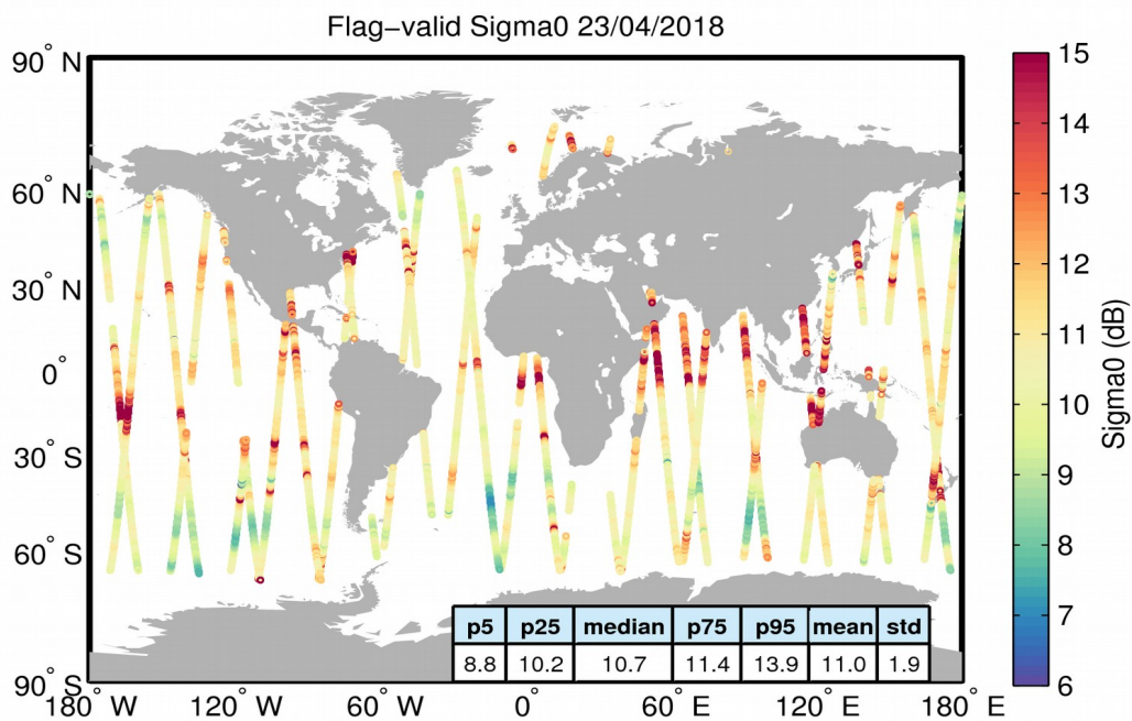
Figure 23. Geographical distribution of flag-valid sigma0 data over oceans and lakes for 23/04/2018. The statistical values shown in the table refer to the sigma0 in dB and are calculated over all measurements shown in the figure.
