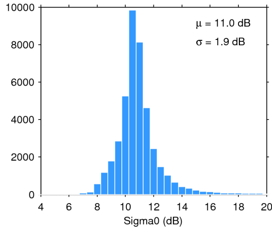
Figure 25. Histogram of flag-valid sigma0 over oceans and lakes for 23/04/2018. The mean ( \mu ) and standard deviation ( \sigma ) are also shown. Note that values outside [4 20] dB are excluded from the histogram for the sake of readability but not from the computation of \mu and \sigma .
