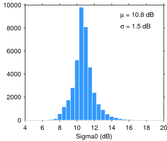
Figure 28. Histogram of science-valid sigma0 over oceans and lakes for 23/04/2018. The mean ( \mu ) and standard deviation ( \sigma ) are also shown. Note that values outside [4 20] dB are excluded from the histogram for the sake of readability but not from the computation of \mu and \sigma .
