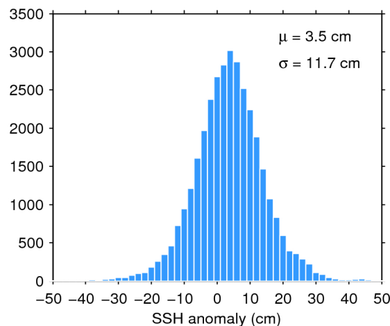
Figure 11. Histogram of science-valid SSH anomaly over oceans and lakes for 23/04/2018. The mean ( \mu ) and standard deviation ( \sigma ) are also shown. Note that values outside [-50 50] cm are excluded from the histogram for the sake of readability but not from the computation of \mu and \sigma .
