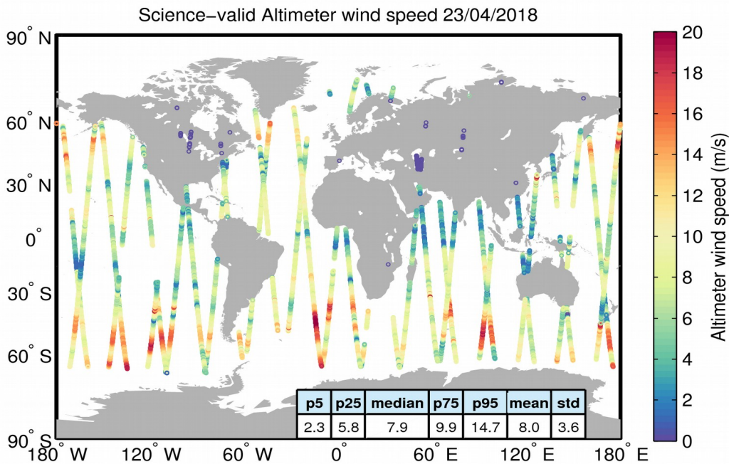
Figure 34. Geographical distribution of science-valid wind data over oceans and lakes for 23/04/2018. The statistical values shown in the table refer to the wind in m/s and are calculated over all measurements shown in the figure. Gray circles denote records that have been rejected based on the editing criteria described in Table 5.
