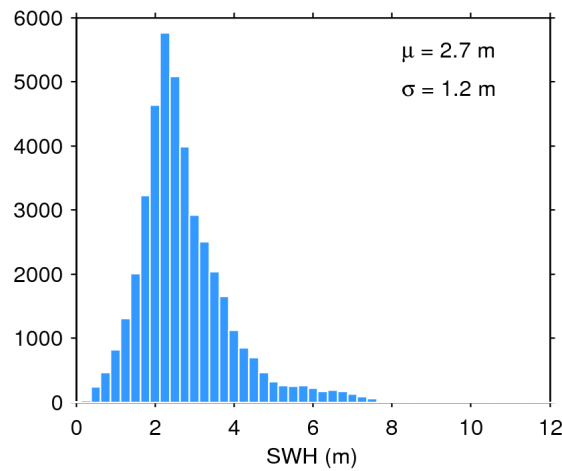
Figure 17. Histogram of flag-valid SWH over oceans and lakes for 23/04/2018. The mean ( \mu ) and standard deviation ( \sigma ) are also shown. Note that values larger than 12 m are excluded from the histogram for the sake of readability but not from the computation of \mu and \sigma .
