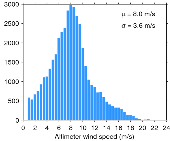
Figure 33. Histogram of flag-valid wind over oceans and lakes for 23/04/2018. The mean ( \mu ) and standard deviation ( \sigma ) are also shown. Note that values larger than 24 m/s are excluded from the histogram for the sake of readability but not from the computation of \mu and \sigma .
