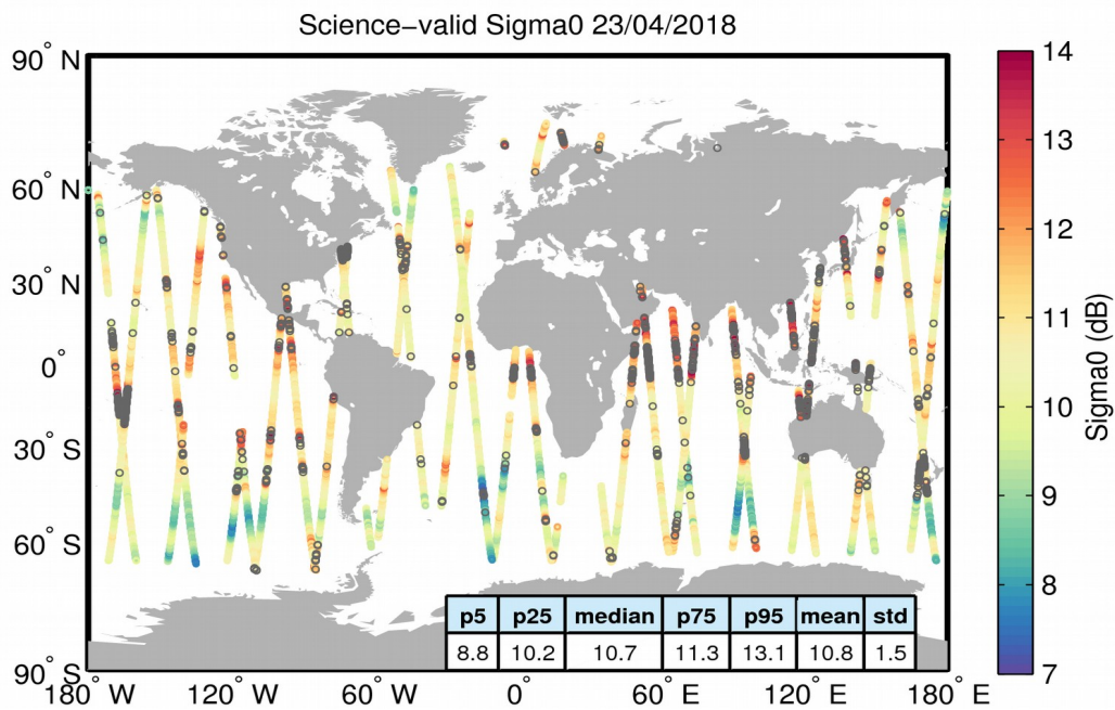
Figure 27. Geographical distribution of science-valid sigma0 data over oceans and lakes for 23/04/2018. The statistical values shown in the table refer to the sigma0 in dB and are calculated over all measurements shown in the figure. Gray circles denote records that have been rejected based on the editing criteria described in Table 4.
