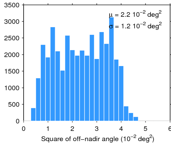
Figure 39. Histogram of flag-valid mispointing over oceans and lakes for 23/04/2018. The mean ( \mu ) and standard deviation ( \sigma ) are also shown. Note that values larger than 6 \cdot 10^{-2} \text{ deg}^2 are excluded from the histogram for the sake of readability but not from the computation of \mu and \sigma .
