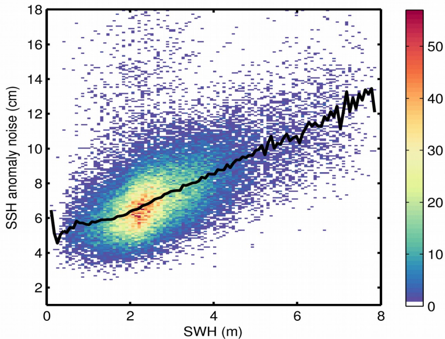
Figure 9. 2D histogram showing flag-valid SSH anomaly noise as a function of SWH for 23/04/2018. The black line denotes the median SSH anomaly noise as a function of SWH.
