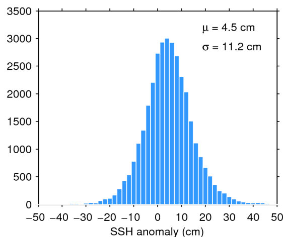
Figure 11. Histogram of science-valid SSH anomaly over oceans and lakes for 21/04/2018. The mean ( \mu ) and standard deviation ( \sigma ) are also shown. Note that values outside [-50 50] cm are excluded from the histogram for the sake of readability but not from the computation of \mu and \sigma .
