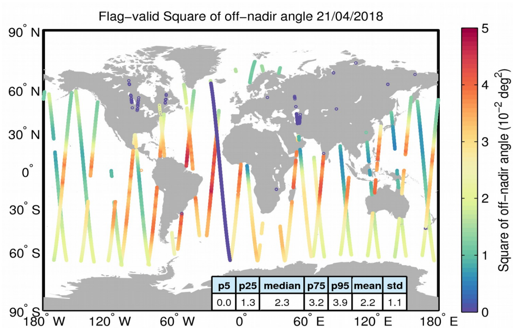
Figure 37. Geographical distribution of flag-valid mispointing data over oceans and lakes for 21/04/2018. The statistical values shown in the table refer to the mispointing in 10^{-2} deg 2 and are calculated over all measurements shown in the figure.
