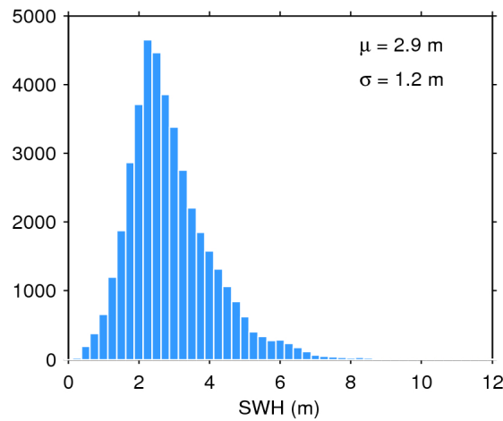
Figure 17. Histogram of flag-valid SWH over oceans and lakes for 21/04/2018. The mean ( \mu ) and standard deviation ( \sigma ) are also shown. Note that values larger than 12 m are excluded from the histogram for the sake of readability but not from the computation of \mu and \sigma .
