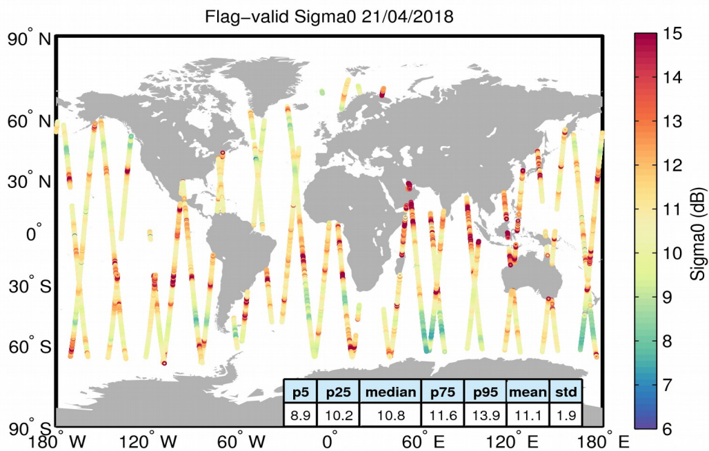
Figure 23. Geographical distribution of flag-valid sigma0 data over oceans and lakes for 21/04/2018. The statistical values shown in the table refer to the sigma0 in dB and are calculated over all measurements shown in the figure.
