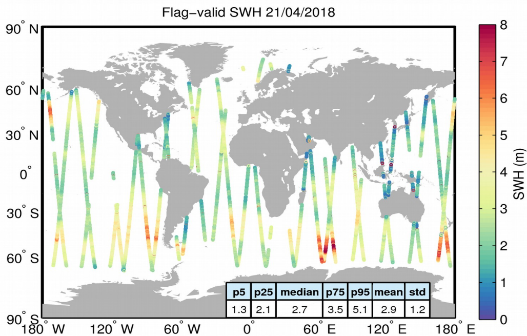
Figure 15. Geographical distribution of flag-valid SWH data over oceans and lakes for 21/04/2018. The statistical values shown in the table refer to the SWH in m and are calculated over all measurements shown in the figure.
