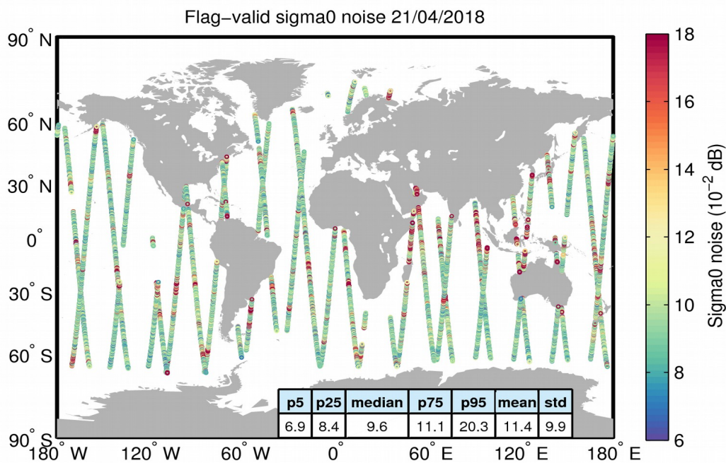
Figure 26. Geographical distribution of flag-valid 20-Hz sigma0 measurement noise over oceans and lakes for 21/04/2018. The statistical values shown in the table refer to the sigma0 noise and are calculated over all measurements shown in the figure.
