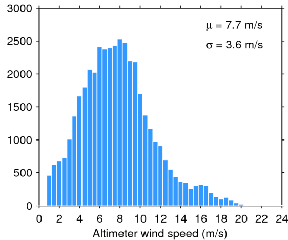
Figure 33. Histogram of flag-valid wind over oceans and lakes for 21/04/2018. The mean ( \mu ) and standard deviation ( \sigma ) are also shown. Note that values larger than 24 m/s are excluded from the histogram for the sake of readability but not from the computation of \mu and \sigma .
