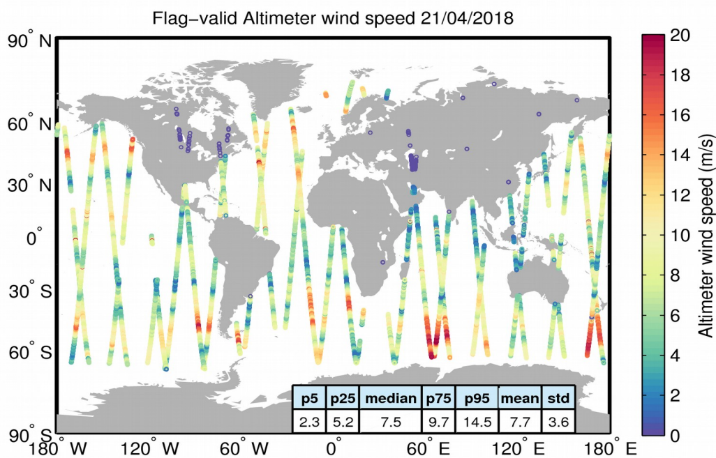
Figure 31. Geographical distribution of flag-valid wind data over oceans and lakes for 21/04/2018. The statistical values shown in the table refer to the wind in m/s and are calculated over all measurements shown in the figure.
