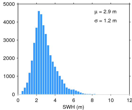
Figure 20. Histogram of science-valid SWH over oceans and lakes for 21/04/2018. The mean ( \mu ) and standard deviation ( \sigma ) are also shown. Note that values larger than 12 m are excluded from the histogram for the sake of readability but not from the computation of \mu and \sigma .
