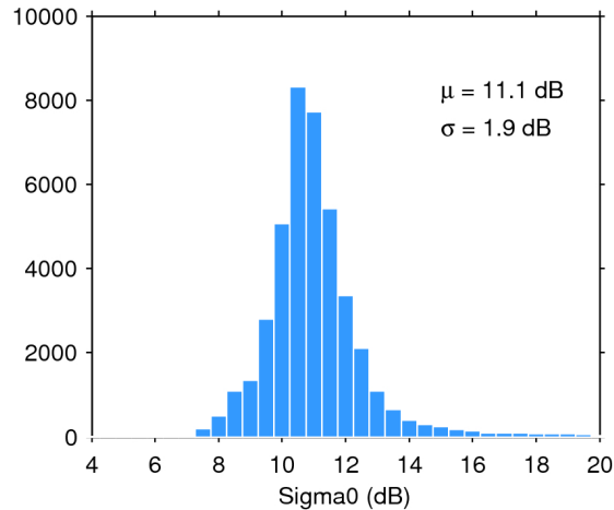
Figure 25. Histogram of flag-valid sigma0 over oceans and lakes for 21/04/2018. The mean ( \mu ) and standard deviation ( \sigma ) are also shown. Note that values outside [4 20] dB are excluded from the histogram for the sake of readability but not from the computation of \mu and \sigma .
