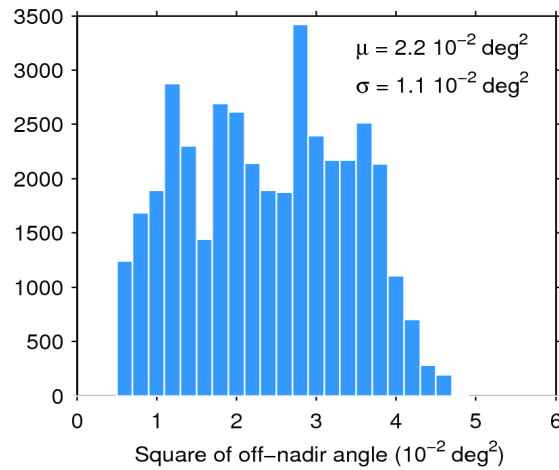
Figure 39. Histogram of flag-valid mispointing over oceans and lakes for 21/04/2018. The mean ( \mu ) and standard deviation ( \sigma ) are also shown. Note that values larger than 6 \cdot 10^{-2} \text{ deg}^2 are excluded from the histogram for the sake of readability but not from the computation of \mu and \sigma .
