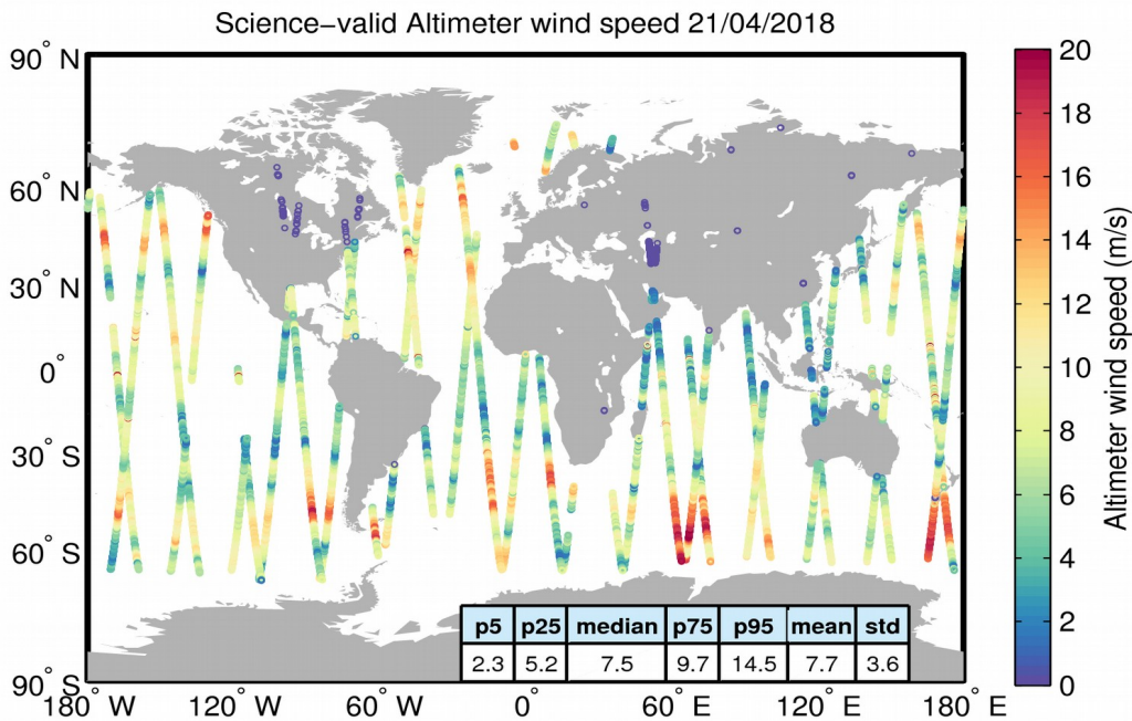
Figure 34. Geographical distribution of science-valid wind data over oceans and lakes for 21/04/2018. The statistical values shown in the table refer to the wind in m/s and are calculated over all measurements shown in the figure. Gray circles denote records that have been rejected based on the editing criteria described in Table 5.
