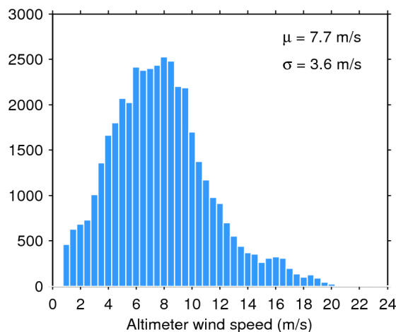
Figure 35. Histogram of science-valid wind over oceans and lakes for 21/04/2018. The mean ( \mu ) and standard deviation ( \sigma ) are also shown. Note that values larger than 24 m/s are excluded from the histogram for the sake of readability but not from the computation of \mu and \sigma .
