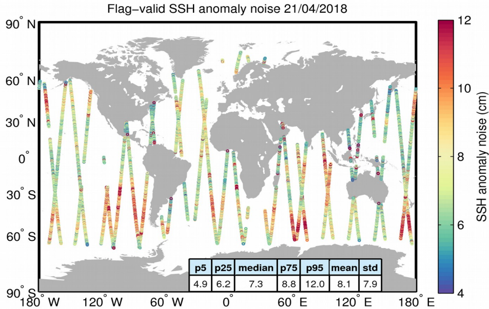
Figure 8. Geographical distribution of flag-valid 20-Hz SSH anomaly measurement noise over oceans and lakes for 21/04/2018. The statistical values shown in the table refer to the SSH anomaly noise and are calculated over all measurements shown in the figure.
