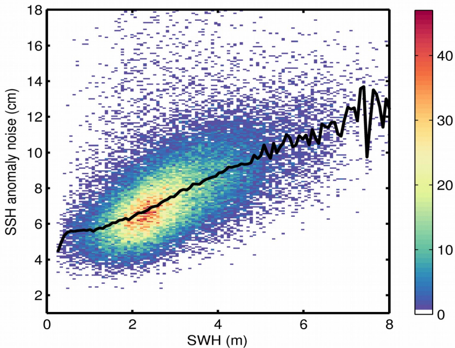
Figure 9. 2D histogram showing flag-valid SSH anomaly noise as a function of SWH for 21/04/2018. The black line denotes the median SSH anomaly noise as a function of SWH.
