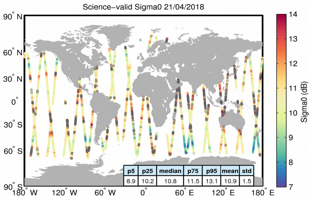
Figure 27. Geographical distribution of science-valid sigma0 data over oceans and lakes for 21/04/2018. The statistical values shown in the table refer to the sigma0 in dB and are calculated over all measurements shown in the figure. Gray circles denote records that have been rejected based on the editing criteria described in Table 4.
