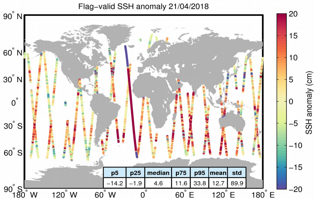
Figure 5. Geographical distribution of flag-valid 1-Hz SSH anomaly data over oceans and lakes for 21/04/2018. The statistical values shown in the table refer to the SSH anomaly in cm and are calculated over all measurements shown in the figure.
