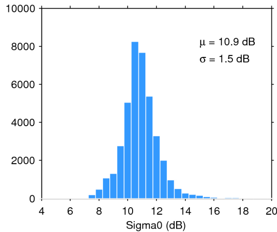
Figure 28. Histogram of science-valid sigma0 over oceans and lakes for 21/04/2018. The mean ( \mu ) and standard deviation ( \sigma ) are also shown. Note that values outside [4 20] dB are excluded from the histogram for the sake of readability but not from the computation of \mu and \sigma .
