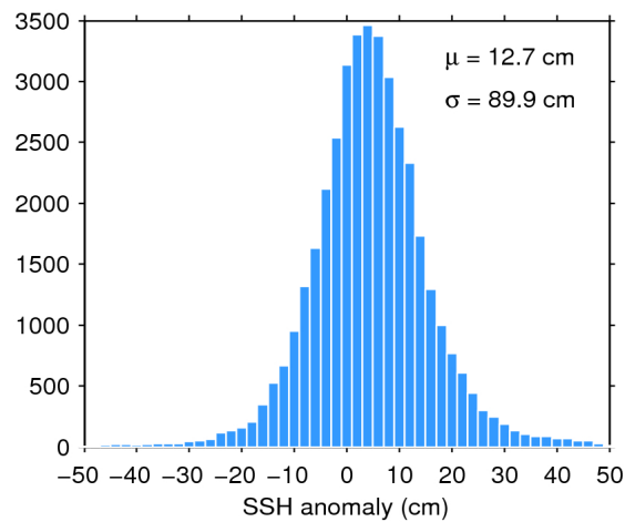
Figure 7. Histogram of flag-valid SSH anomaly over oceans and lakes for 21/04/2018. The mean ( \mu ) and standard deviation ( \sigma ) are also shown. Note that values outside [-50 50] cm are excluded from the histogram for the sake of readability but not from the computation of \mu and \sigma .
