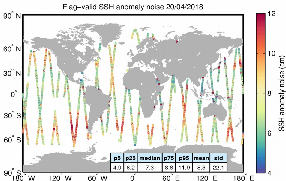
Figure 8. Geographical distribution of flag-valid 20-Hz SSH anomaly measurement noise over oceans and lakes for 20/04/2018. The statistical values shown in the table refer to the SSH anomaly noise and are calculated over all measurements shown in the figure.
