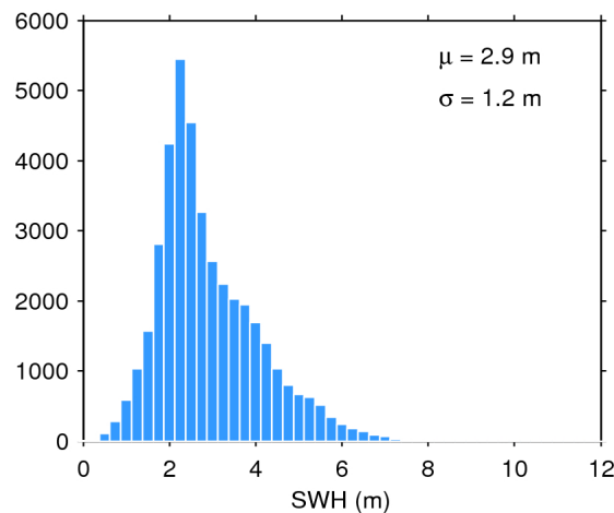
Figure 20. Histogram of science-valid SWH over oceans and lakes for 20/04/2018. The mean ( \mu ) and standard deviation ( \sigma ) are also shown. Note that values larger than 12 m are excluded from the histogram for the sake of readability but not from the computation of \mu and \sigma .
