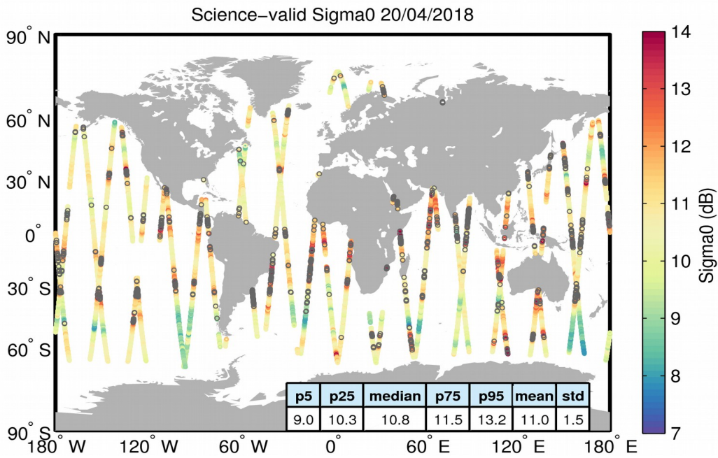
Figure 27. Geographical distribution of science-valid sigma0 data over oceans and lakes for 20/04/2018. The statistical values shown in the table refer to the sigma0 in dB and are calculated over all measurements shown in the figure. Gray circles denote records that have been rejected based on the editing criteria described in Table 4.
