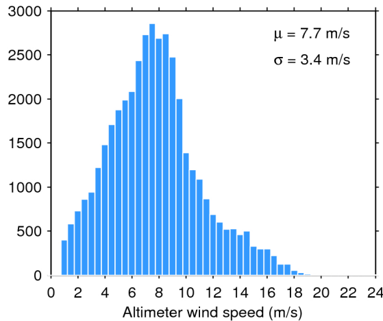
Figure 33. Histogram of flag-valid wind over oceans and lakes for 20/04/2018. The mean ( \mu ) and standard deviation ( \sigma ) are also shown. Note that values larger than 24 m/s are excluded from the histogram for the sake of readability but not from the computation of \mu and \sigma .
