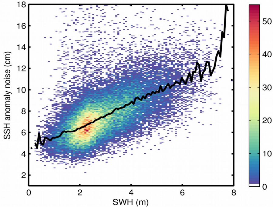
Figure 9. 2D histogram showing flag-valid SSH anomaly noise as a function of SWH for 20/04/2018. The black line denotes the median SSH anomaly noise as a function of SWH.
