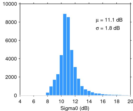
Figure 25. Histogram of flag-valid sigma0 over oceans and lakes for 20/04/2018. The mean ( \mu ) and standard deviation ( \sigma ) are also shown. Note that values outside [4 20] dB are excluded from the histogram for the sake of readability but not from the computation of \mu and \sigma .
