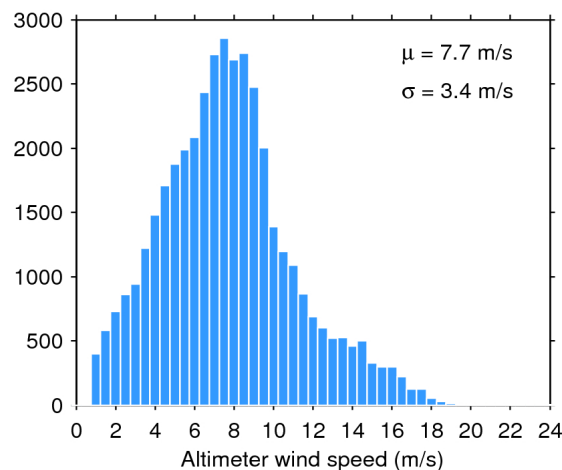
Figure 35. Histogram of science-valid wind over oceans and lakes for 20/04/2018. The mean ( \mu ) and standard deviation ( \sigma ) are also shown. Note that values larger than 24 m/s are excluded from the histogram for the sake of readability but not from the computation of \mu and \sigma .
