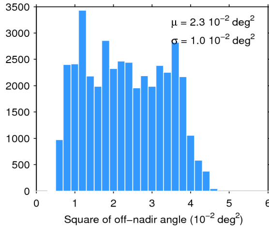
Figure 39. Histogram of flag-valid mispointing over oceans and lakes for 20/04/2018. The mean ( \mu ) and standard deviation ( \sigma ) are also shown. Note that values larger than 6 \cdot 10^{-2} \text{ deg}^2 are excluded from the histogram for the sake of readability but not from the computation of \mu and \sigma .
