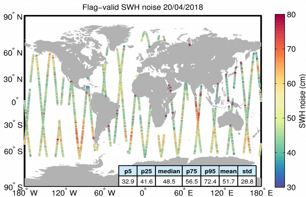
Figure 18. Geographical distribution of flag-valid 20-Hz SWH measurement noise over oceans and lakes for 20/04/2018. The statistical values shown in the table refer to the SWH noise and are calculated over all measurements shown in the figure.
