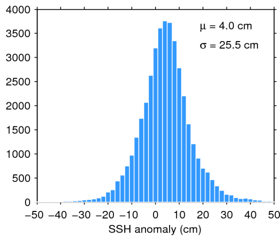
Figure 7. Histogram of flag-valid SSH anomaly over oceans and lakes for 20/04/2018. The mean ( \mu ) and standard deviation ( \sigma ) are also shown. Note that values outside [-50\ 50] cm are excluded from the histogram for the sake of readability but not from the computation of \mu and \sigma .
