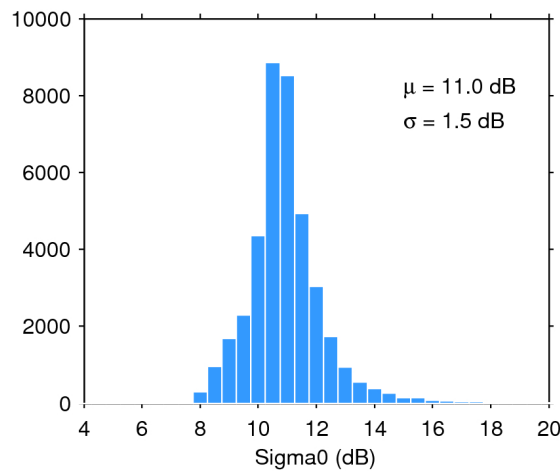
Figure 28. Histogram of science-valid sigma0 over oceans and lakes for 20/04/2018. The mean ( \mu ) and standard deviation ( \sigma ) are also shown. Note that values outside [4 20] dB are excluded from the histogram for the sake of readability but not from the computation of \mu and \sigma .
