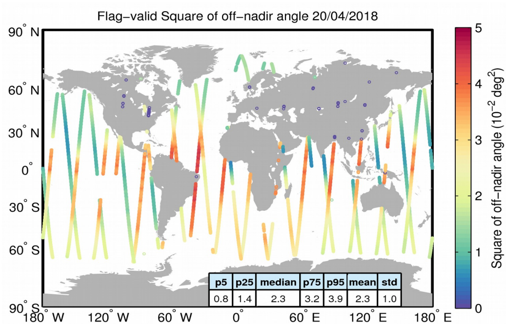
Figure 37. Geographical distribution of flag-valid mispointing data over oceans and lakes for 20/04/2018. The statistical values shown in the table refer to the mispointing in 10^{-2} deg 2 and are calculated over all measurements shown in the figure.
