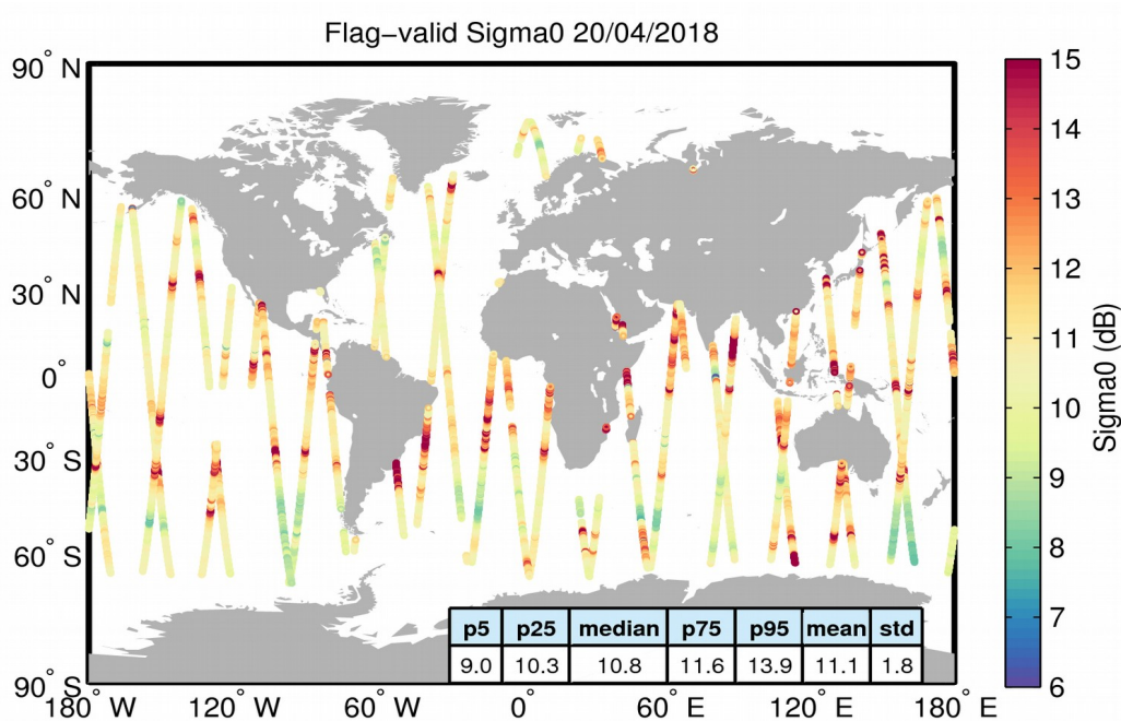
Figure 23. Geographical distribution of flag-valid sigma0 data over oceans and lakes for 20/04/2018. The statistical values shown in the table refer to the sigma0 in dB and are calculated over all measurements shown in the figure.
