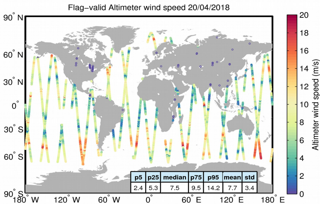
Figure 31. Geographical distribution of flag-valid wind data over oceans and lakes for 20/04/2018. The statistical values shown in the table refer to the wind in m/s and are calculated over all measurements shown in the figure.
