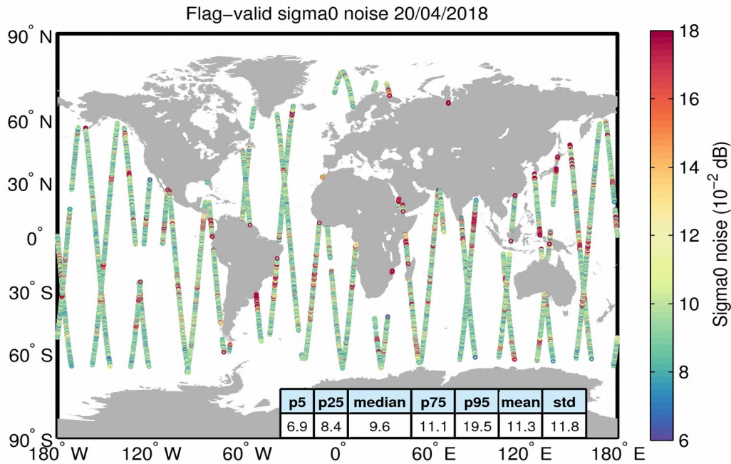
Figure 26. Geographical distribution of flag-valid 20-Hz sigma0 measurement noise over oceans and lakes for 20/04/2018. The statistical values shown in the table refer to the sigma0 noise and are calculated over all measurements shown in the figure.
