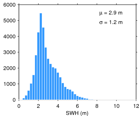
Figure 17. Histogram of flag-valid SWH over oceans and lakes for 20/04/2018. The mean ( \mu ) and standard deviation ( \sigma ) are also shown. Note that values larger than 12 m are excluded from the histogram for the sake of readability but not from the computation of \mu and \sigma .
