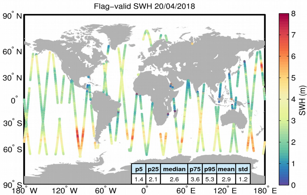
Figure 15. Geographical distribution of flag-valid SWH data over oceans and lakes for 20/04/2018. The statistical values shown in the table refer to the SWH in m and are calculated over all measurements shown in the figure.
