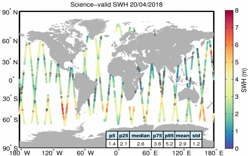
Figure 19. Geographical distribution of science-valid SWH data over oceans and lakes for 20/04/2018. The statistical values shown in the table refer to the SWH in m and are calculated over all measurements shown in the figure. Gray circles denote records that have been rejected based on the editing criteria described in Table 3.
