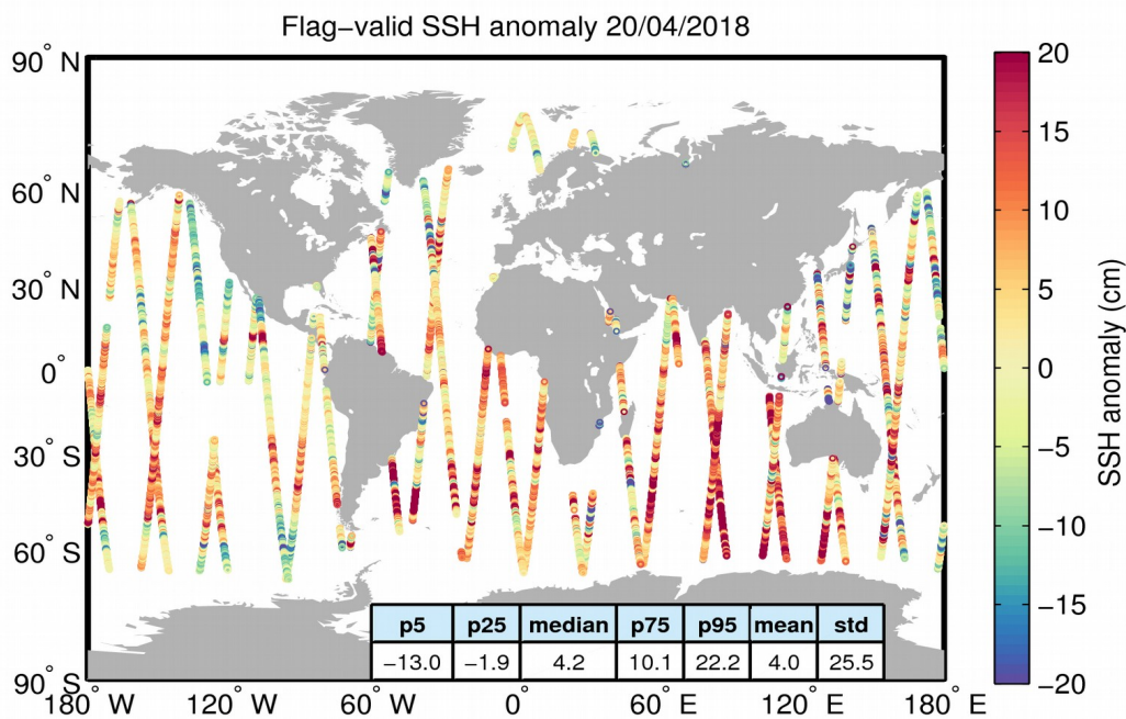
Figure 5. Geographical distribution of flag-valid 1-Hz SSH anomaly data over oceans and lakes for 20/04/2018. The statistical values shown in the table refer to the SSH anomaly in cm and are calculated over all measurements shown in the figure.
