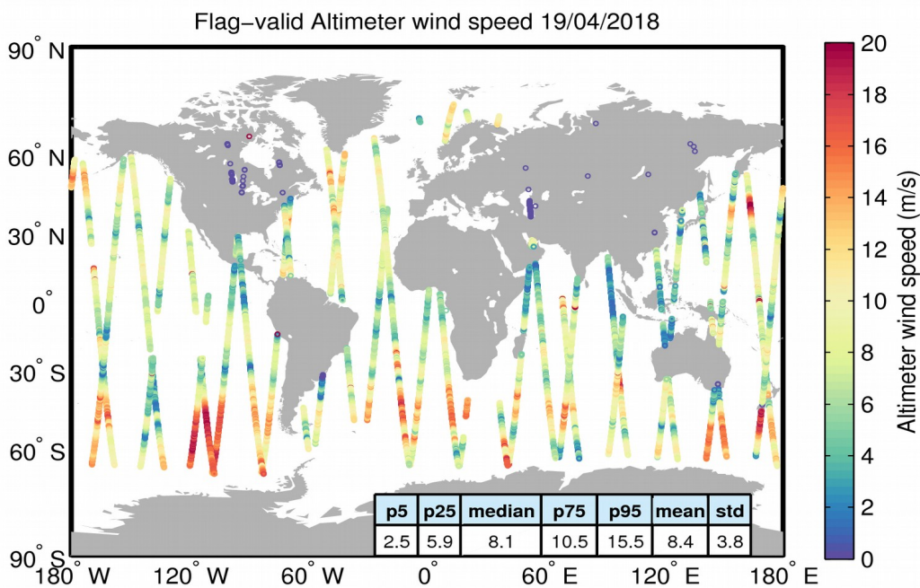
Figure 31. Geographical distribution of flag-valid wind data over oceans and lakes for 19/04/2018. The statistical values shown in the table refer to the wind in m/s and are calculated over all measurements shown in the figure.
