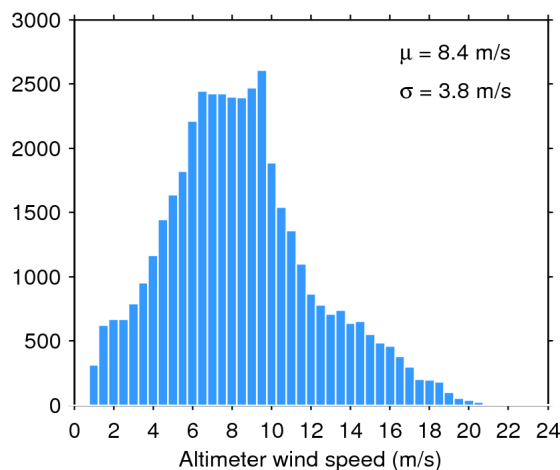
Figure 35. Histogram of science-valid wind over oceans and lakes for 19/04/2018. The mean ( \mu ) and standard deviation ( \sigma ) are also shown. Note that values larger than 24 m/s are excluded from the histogram for the sake of readability but not from the computation of \mu and \sigma .
