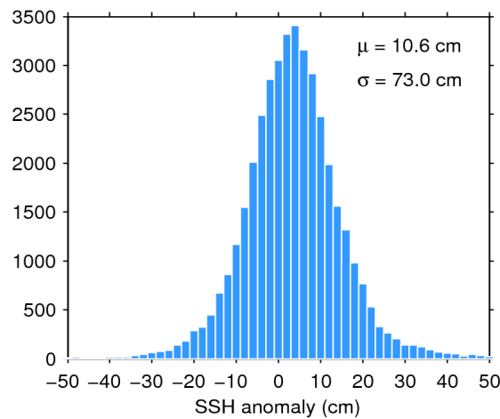
Figure 7. Histogram of flag-valid SSH anomaly over oceans and lakes for 19/04/2018. The mean ( \mu ) and standard deviation ( \sigma ) are also shown. Note that values outside [-50 50] cm are excluded from the histogram for the sake of readability but not from the computation of \mu and \sigma .
