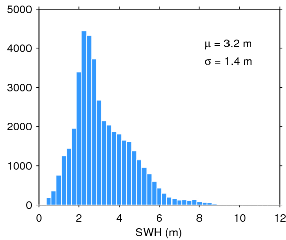
Figure 17. Histogram of flag-valid SWH over oceans and lakes for 19/04/2018. The mean ( \mu ) and standard deviation ( \sigma ) are also shown. Note that values larger than 12 m are excluded from the histogram for the sake of readability but not from the computation of \mu and \sigma .
