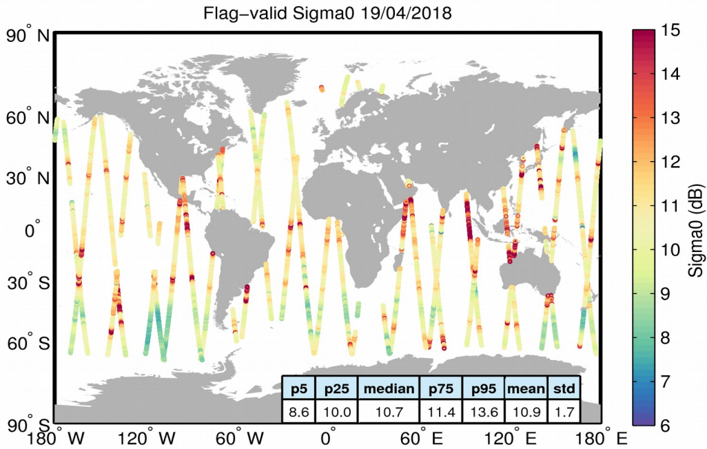
Figure 23. Geographical distribution of flag-valid sigma0 data over oceans and lakes for 19/04/2018. The statistical values shown in the table refer to the sigma0 in dB and are calculated over all measurements shown in the figure.
