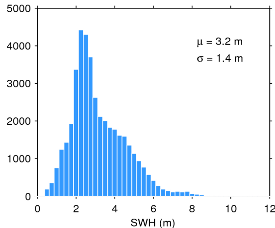
Figure 20. Histogram of science-valid SWH over oceans and lakes for 19/04/2018. The mean ( \mu ) and standard deviation ( \sigma ) are also shown. Note that values larger than 12 m are excluded from the histogram for the sake of readability but not from the computation of \mu and \sigma .
