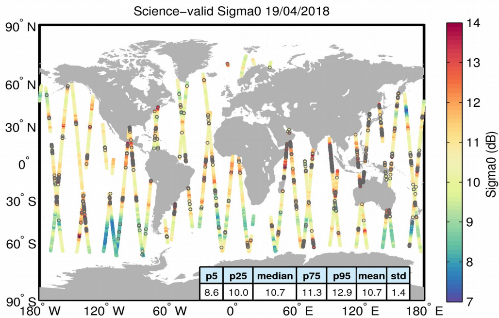
Figure 27. Geographical distribution of science-valid sigma0 data over oceans and lakes for 19/04/2018. The statistical values shown in the table refer to the sigma0 in dB and are calculated over all measurements shown in the figure. Gray circles denote records that have been rejected based on the editing criteria described in Table 4.
