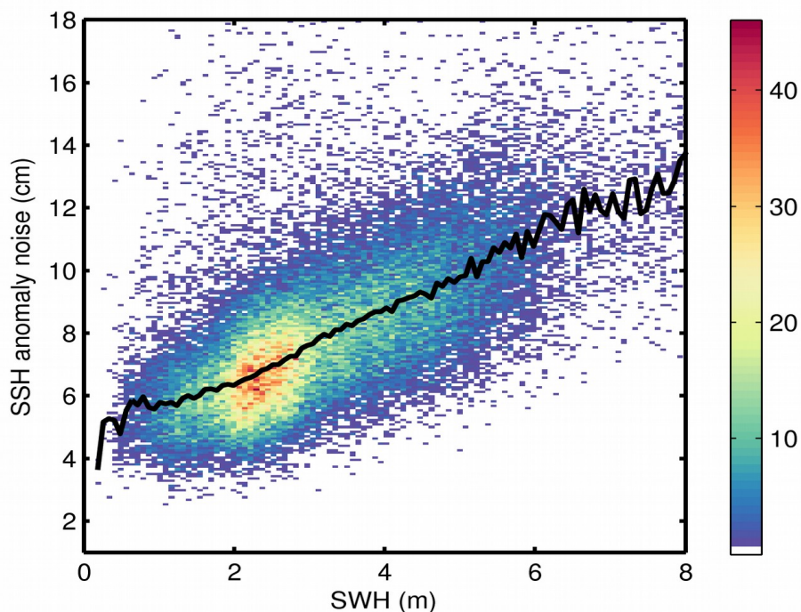
Figure 9. 2D histogram showing flag-valid SSH anomaly noise as a function of SWH for 19/04/2018. The black line denotes the median SSH anomaly noise as a function of SWH.
