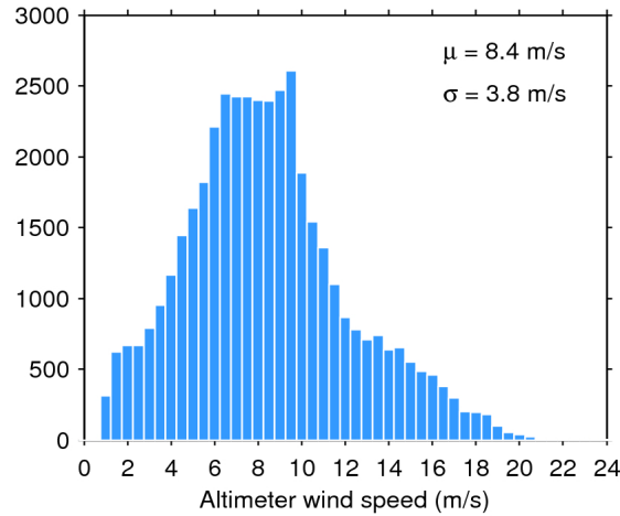
Figure 33. Histogram of flag-valid wind over oceans and lakes for 19/04/2018. The mean ( \mu ) and standard deviation ( \sigma ) are also shown. Note that values larger than 24 m/s are excluded from the histogram for the sake of readability but not from the computation of \mu and \sigma .
