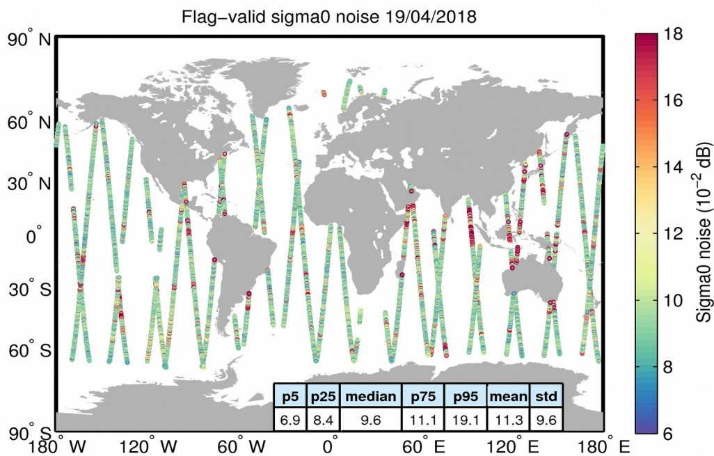
Figure 26. Geographical distribution of flag-valid 20-Hz sigma0 measurement noise over oceans and lakes for 19/04/2018. The statistical values shown in the table refer to the sigma0 noise and are calculated over all measurements shown in the figure.
