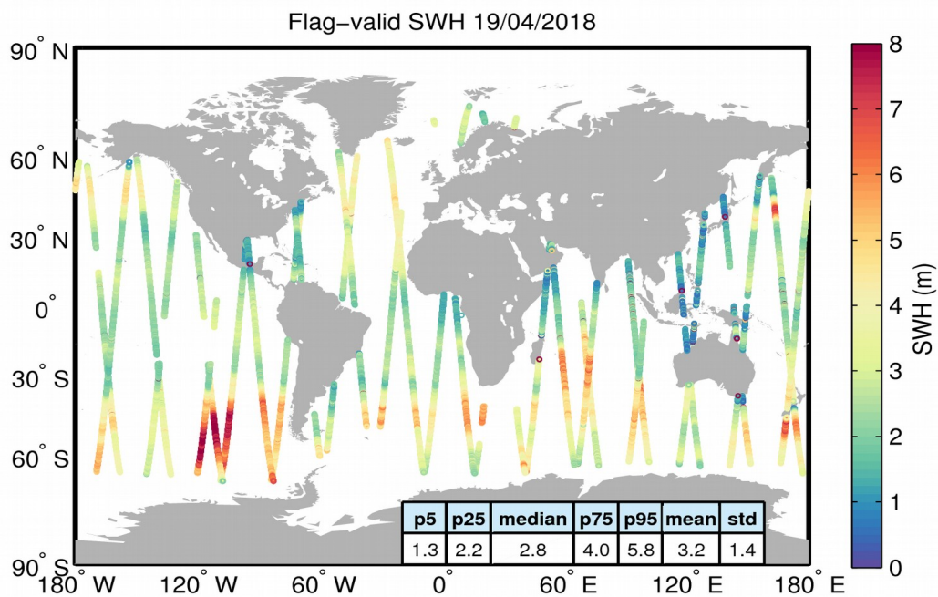
Figure 15. Geographical distribution of flag-valid SWH data over oceans and lakes for 19/04/2018. The statistical values shown in the table refer to the SWH in m and are calculated over all measurements shown in the figure.
