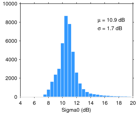
Figure 25. Histogram of flag-valid sigma0 over oceans and lakes for 19/04/2018. The mean ( \mu ) and standard deviation ( \sigma ) are also shown. Note that values outside [4 20] dB are excluded from the histogram for the sake of readability but not from the computation of \mu and \sigma .
