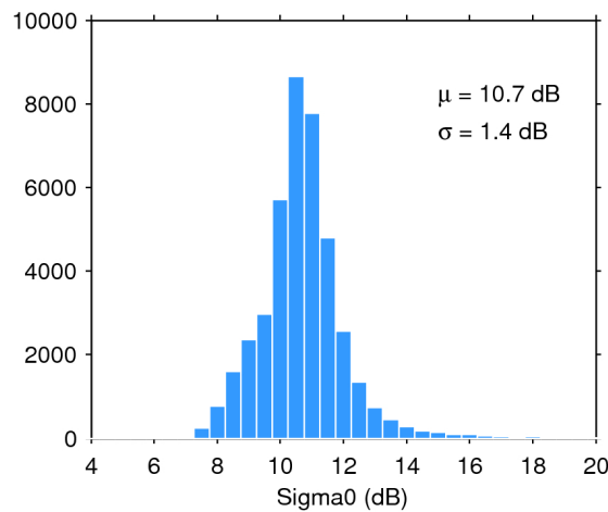
Figure 28. Histogram of science-valid sigma0 over oceans and lakes for 19/04/2018. The mean ( \mu ) and standard deviation ( \sigma ) are also shown. Note that values outside [4 20] dB are excluded from the histogram for the sake of readability but not from the computation of \mu and \sigma .
