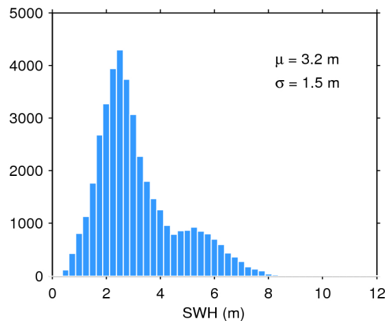
Figure 17. Histogram of flag-valid SWH over oceans and lakes for 18/04/2018. The mean ( \mu ) and standard deviation ( \sigma ) are also shown. Note that values larger than 12 m are excluded from the histogram for the sake of readability but not from the computation of \mu and \sigma .
