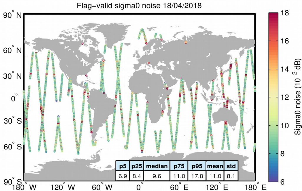
Figure 26. Geographical distribution of flag-valid 20-Hz sigma0 measurement noise over oceans and lakes for 18/04/2018. The statistical values shown in the table refer to the sigma0 noise and are calculated over all measurements shown in the figure.
