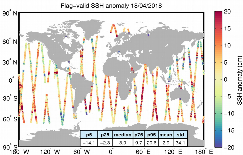
Figure 5. Geographical distribution of flag-valid 1-Hz SSH anomaly data over oceans and lakes for 18/04/2018. The statistical values shown in the table refer to the SSH anomaly in cm and are calculated over all measurements shown in the figure.
