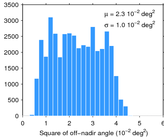
Figure 39. Histogram of flag-valid mispointing over oceans and lakes for 18/04/2018. The mean ( \mu ) and standard deviation ( \sigma ) are also shown. Note that values larger than 6 \cdot 10^{-2} \text{ deg}^2 are excluded from the histogram for the sake of readability but not from the computation of \mu and \sigma .
