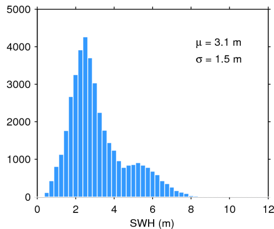
Figure 20. Histogram of science-valid SWH over oceans and lakes for 18/04/2018. The mean ( \mu ) and standard deviation ( \sigma ) are also shown. Note that values larger than 12 m are excluded from the histogram for the sake of readability but not from the computation of \mu and \sigma .
