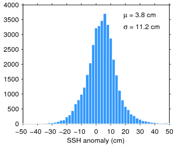
Figure 11. Histogram of science-valid SSH anomaly over oceans and lakes for 18/04/2018. The mean ( \mu ) and standard deviation ( \sigma ) are also shown. Note that values outside [-50 50] cm are excluded from the histogram for the sake of readability but not from the computation of \mu and \sigma .
