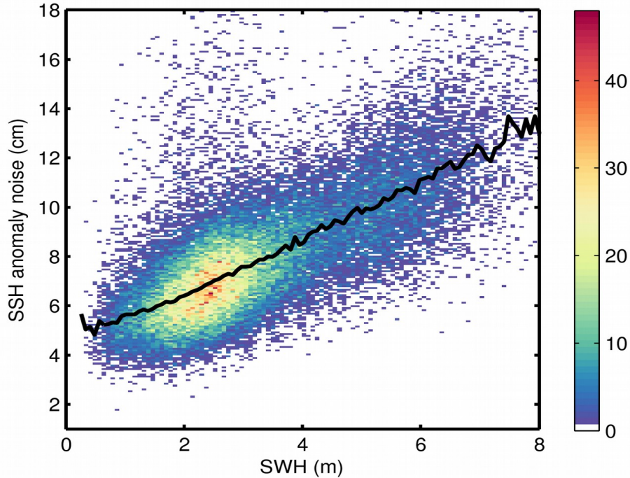
Figure 9. 2D histogram showing flag-valid SSH anomaly noise as a function of SWH for 18/04/2018. The black line denotes the median SSH anomaly noise as a function of SWH.
