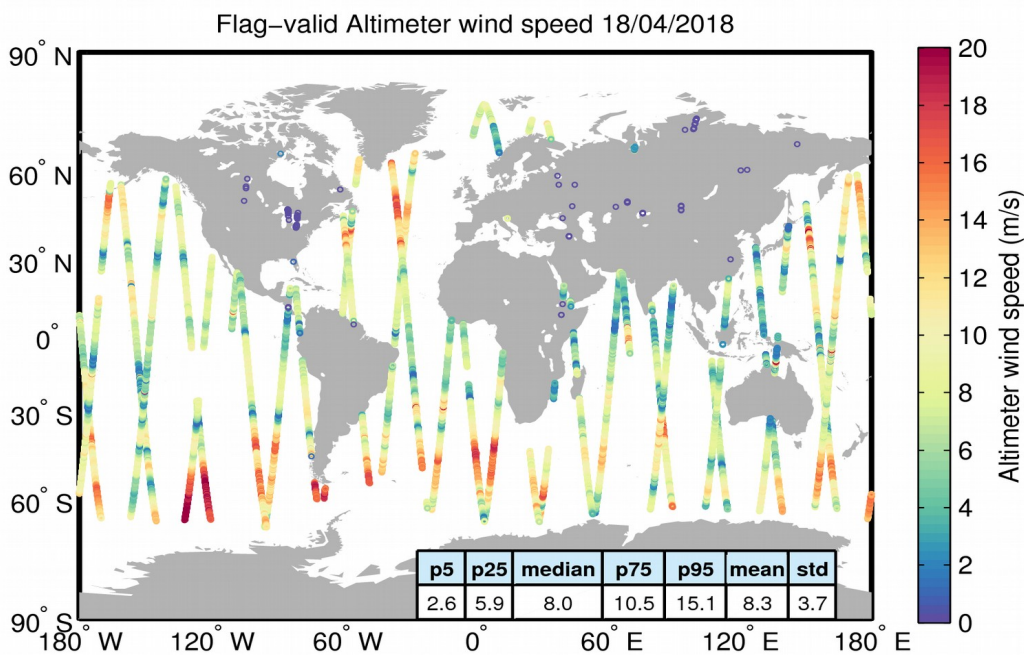
Figure 31. Geographical distribution of flag-valid wind data over oceans and lakes for 18/04/2018. The statistical values shown in the table refer to the wind in m/s and are calculated over all measurements shown in the figure.
