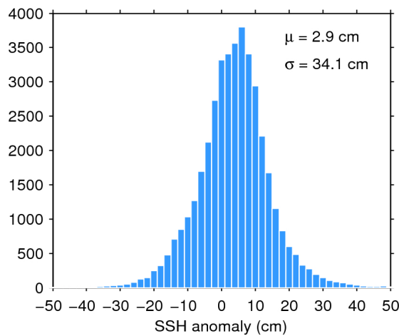
Figure 7. Histogram of flag-valid SSH anomaly over oceans and lakes for 18/04/2018. The mean ( \mu ) and standard deviation ( \sigma ) are also shown. Note that values outside [-50\ 50] cm are excluded from the histogram for the sake of readability but not from the computation of \mu and \sigma .
