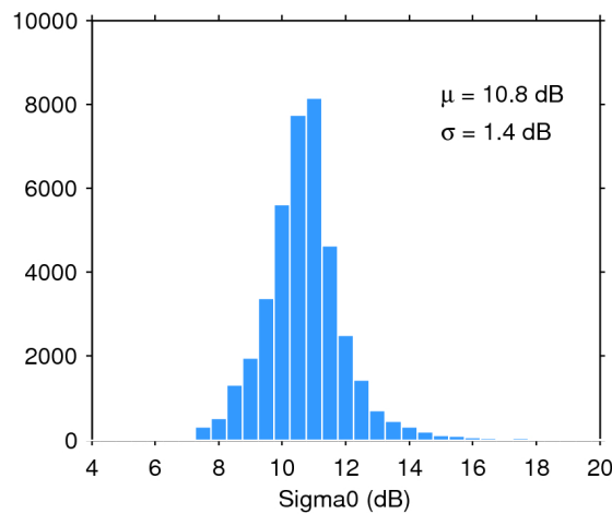
Figure 28. Histogram of science-valid sigma0 over oceans and lakes for 18/04/2018. The mean ( \mu ) and standard deviation ( \sigma ) are also shown. Note that values outside [4 20] dB are excluded from the histogram for the sake of readability but not from the computation of \mu and \sigma .
