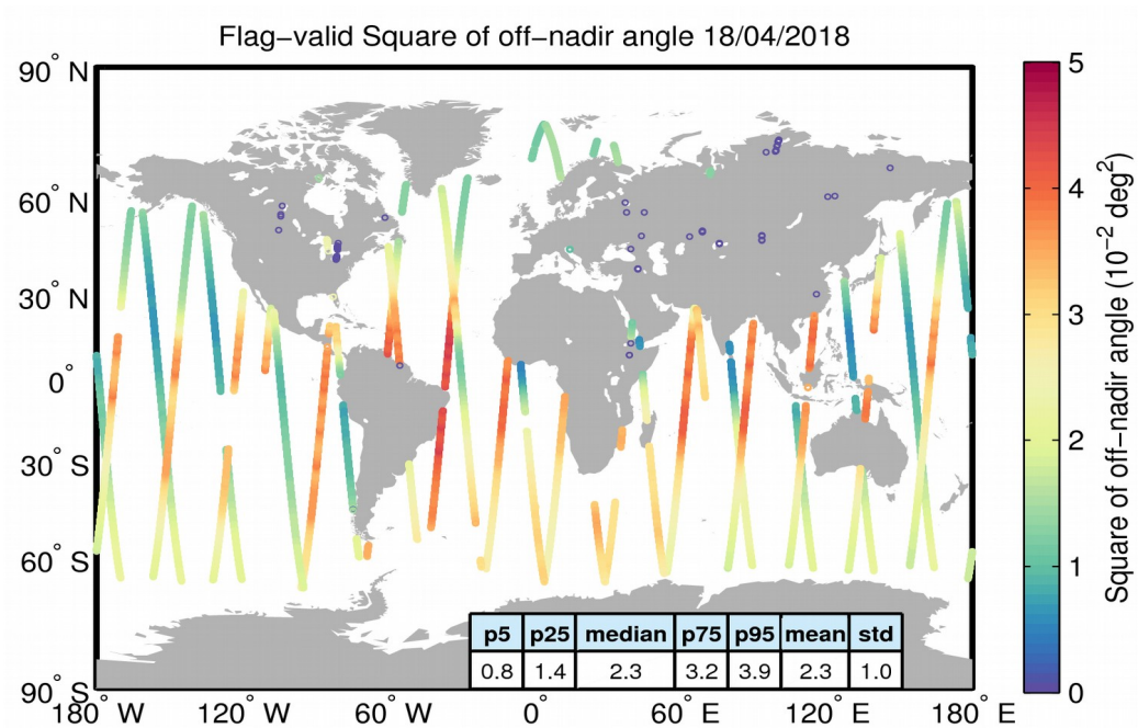
Figure 37. Geographical distribution of flag-valid mispointing data over oceans and lakes for 18/04/2018. The statistical values shown in the table refer to the mispointing in 10^{-2} deg 2 and are calculated over all measurements shown in the figure.
