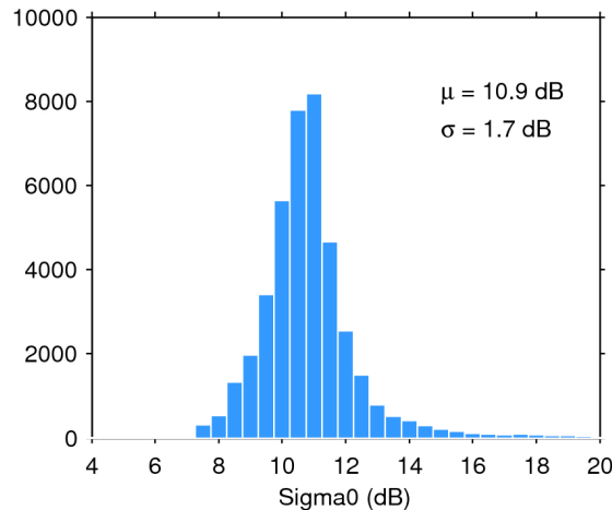
Figure 25. Histogram of flag-valid sigma0 over oceans and lakes for 18/04/2018. The mean ( \mu ) and standard deviation ( \sigma ) are also shown. Note that values outside [4 20] dB are excluded from the histogram for the sake of readability but not from the computation of \mu and \sigma .
