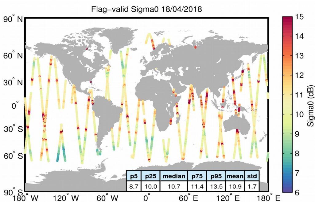
Figure 23. Geographical distribution of flag-valid sigma0 data over oceans and lakes for 18/04/2018. The statistical values shown in the table refer to the sigma0 in dB and are calculated over all measurements shown in the figure.
