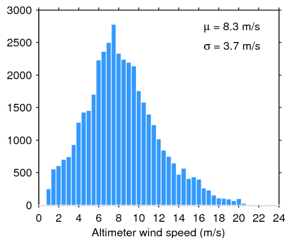
Figure 35. Histogram of science-valid wind over oceans and lakes for 18/04/2018. The mean ( \mu ) and standard deviation ( \sigma ) are also shown. Note that values larger than 24 m/s are excluded from the histogram for the sake of readability but not from the computation of \mu and \sigma .
