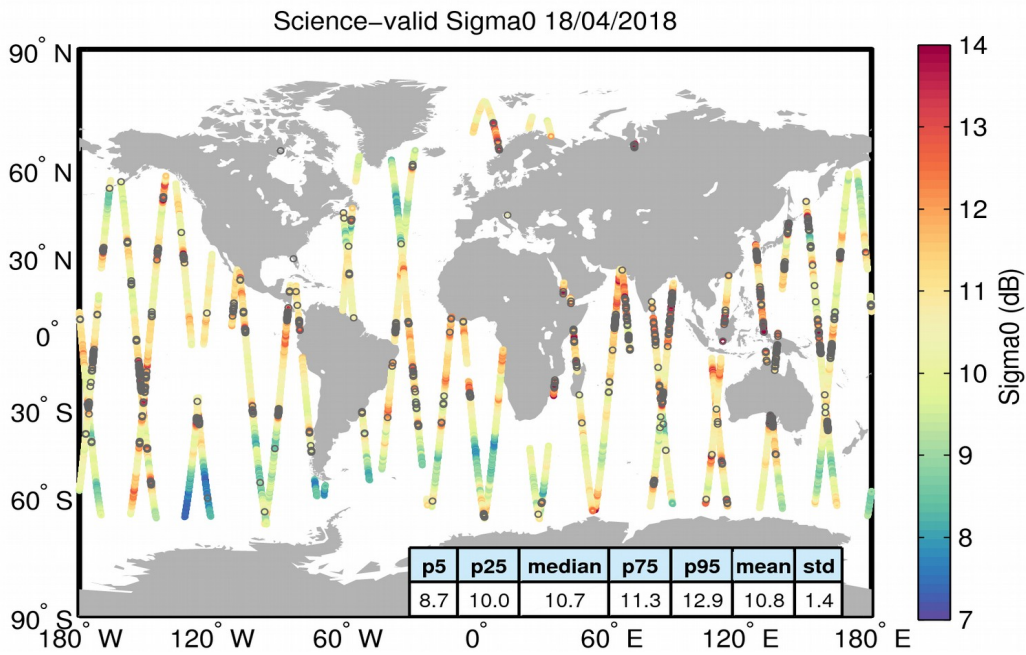
Figure 27. Geographical distribution of science-valid sigma0 data over oceans and lakes for 18/04/2018. The statistical values shown in the table refer to the sigma0 in dB and are calculated over all measurements shown in the figure. Gray circles denote records that have been rejected based on the editing criteria described in Table 4.
