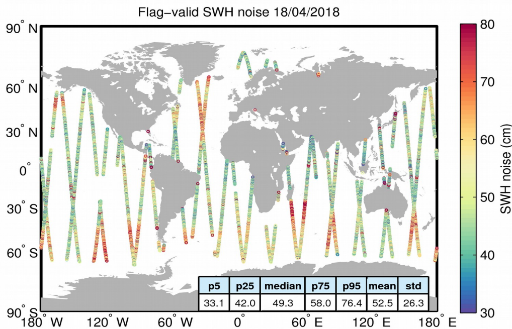
Figure 18. Geographical distribution of flag-valid 20-Hz SWH measurement noise over oceans and lakes for 18/04/2018. The statistical values shown in the table refer to the SWH noise and are calculated over all measurements shown in the figure.
