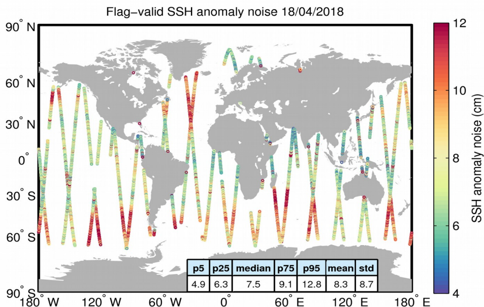
Figure 8. Geographical distribution of flag-valid 20-Hz SSH anomaly measurement noise over oceans and lakes for 18/04/2018. The statistical values shown in the table refer to the SSH anomaly noise and are calculated over all measurements shown in the figure.
