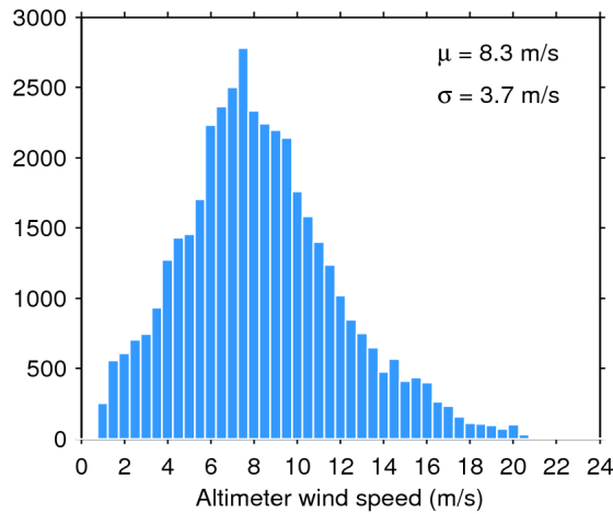
Figure 33. Histogram of flag-valid wind over oceans and lakes for 18/04/2018. The mean ( \mu ) and standard deviation ( \sigma ) are also shown. Note that values larger than 24 m/s are excluded from the histogram for the sake of readability but not from the computation of \mu and \sigma .
