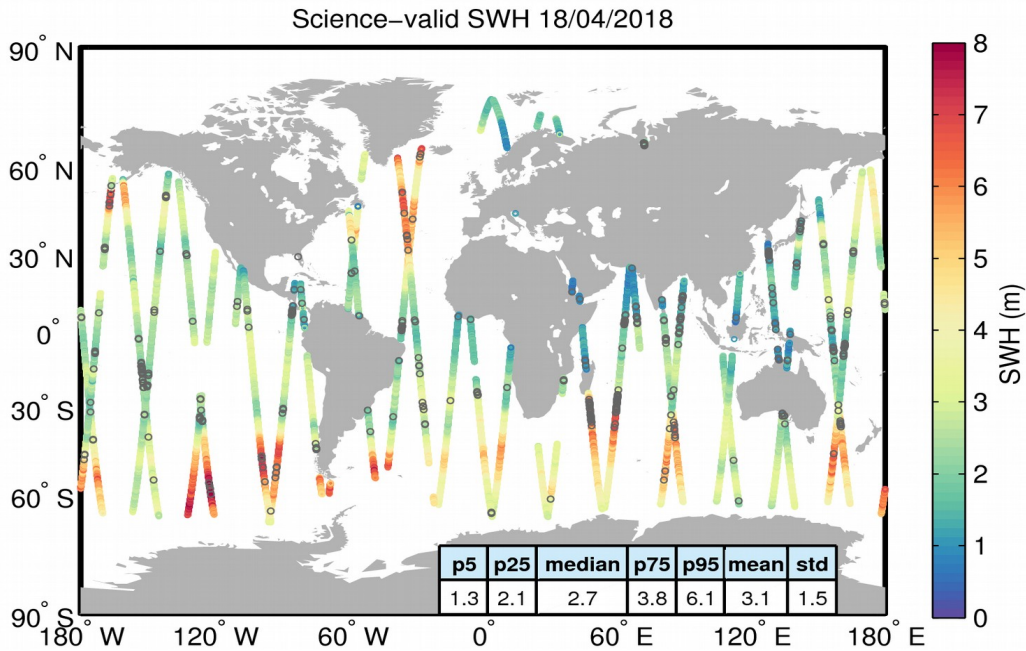
Figure 19. Geographical distribution of science-valid SWH data over oceans and lakes for 18/04/2018. The statistical values shown in the table refer to the SWH in m and are calculated over all measurements shown in the figure. Gray circles denote records that have been rejected based on the editing criteria described in Table 3.
