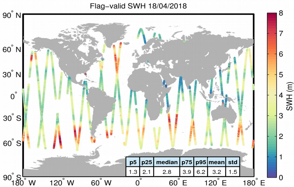
Figure 15. Geographical distribution of flag-valid SWH data over oceans and lakes for 18/04/2018. The statistical values shown in the table refer to the SWH in m and are calculated over all measurements shown in the figure.
