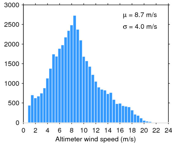
Figure 33. Histogram of flag-valid wind over oceans and lakes for 17/04/2018. The mean ( \mu ) and standard deviation ( \sigma ) are also shown. Note that values larger than 24 m/s are excluded from the histogram for the sake of readability but not from the computation of \mu and \sigma .
