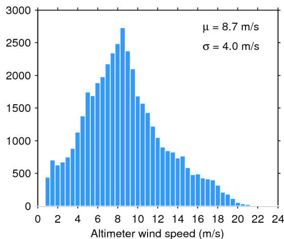
Figure 35. Histogram of science-valid wind over oceans and lakes for 17/04/2018. The mean ( \mu ) and standard deviation ( \sigma ) are also shown. Note that values larger than 24 m/s are excluded from the histogram for the sake of readability but not from the computation of \mu and \sigma .
