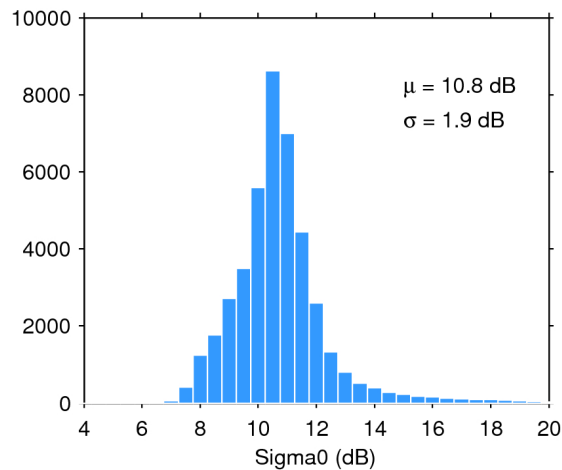
Figure 25. Histogram of flag-valid sigma0 over oceans and lakes for 17/04/2018. The mean ( \mu ) and standard deviation ( \sigma ) are also shown. Note that values outside [4 20] dB are excluded from the histogram for the sake of readability but not from the computation of \mu and \sigma .
