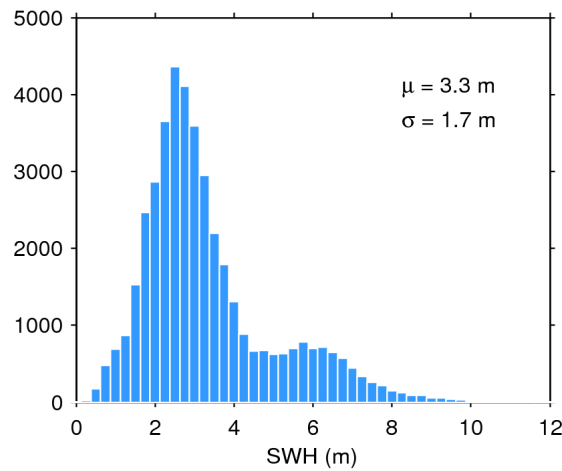
Figure 17. Histogram of flag-valid SWH over oceans and lakes for 17/04/2018. The mean ( \mu ) and standard deviation ( \sigma ) are also shown. Note that values larger than 12 m are excluded from the histogram for the sake of readability but not from the computation of \mu and \sigma .
