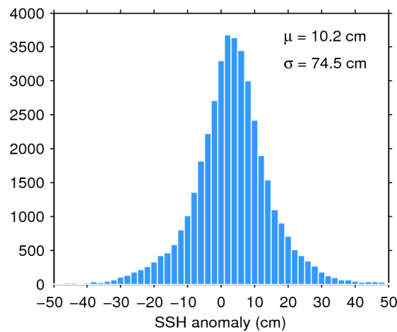
Figure 7. Histogram of flag-valid SSH anomaly over oceans and lakes for 17/04/2018. The mean ( \mu ) and standard deviation ( \sigma ) are also shown. Note that values outside [-50\ 50] cm are excluded from the histogram for the sake of readability but not from the computation of \mu and \sigma .
