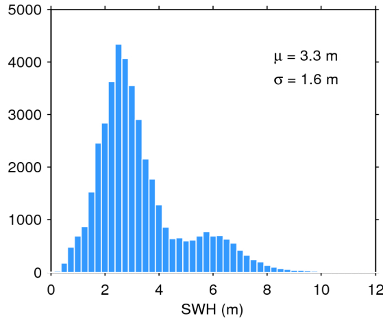
Figure 20. Histogram of science-valid SWH over oceans and lakes for 17/04/2018. The mean ( \mu ) and standard deviation ( \sigma ) are also shown. Note that values larger than 12 m are excluded from the histogram for the sake of readability but not from the computation of \mu and \sigma .
