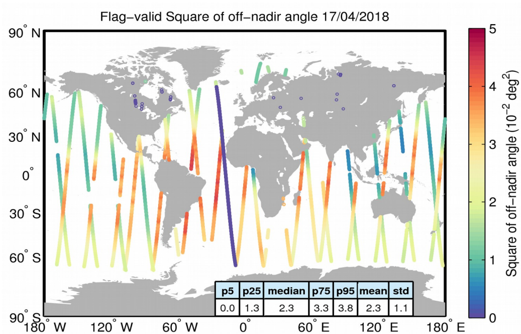
Figure 37. Geographical distribution of flag-valid mispointing data over oceans and lakes for 17/04/2018. The statistical values shown in the table refer to the mispointing in 10^{-2} \text{ deg}^2 and are calculated over all measurements shown in the figure.
