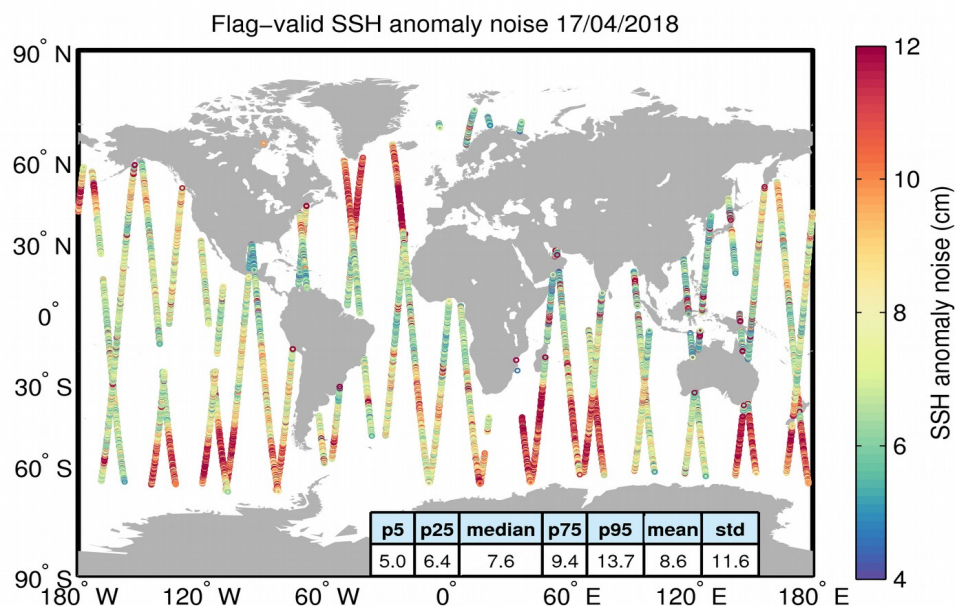
Figure 8. Geographical distribution of flag-valid 20-Hz SSH anomaly measurement noise over oceans and lakes for 17/04/2018. The statistical values shown in the table refer to the SSH anomaly noise and are calculated over all measurements shown in the figure.
