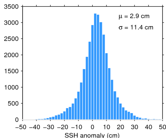
Figure 11. Histogram of science-valid SSH anomaly over oceans and lakes for 17/04/2018. The mean ( \mu ) and standard deviation ( \sigma ) are also shown. Note that values outside [-50 50] cm are excluded from the histogram for the sake of readability but not from the computation of \mu and \sigma .
