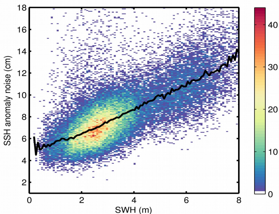
Figure 9. 2D histogram showing flag-valid SSH anomaly noise as a function of SWH for 17/04/2018. The black line denotes the median SSH anomaly noise as a function of SWH.
