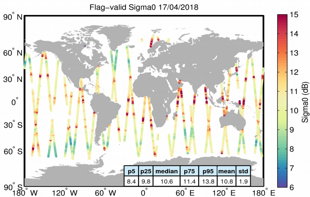
Figure 23. Geographical distribution of flag-valid sigma0 data over oceans and lakes for 17/04/2018. The statistical values shown in the table refer to the sigma0 in dB and are calculated over all measurements shown in the figure.
