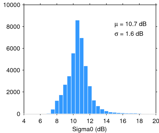
Figure 28. Histogram of science-valid sigma0 over oceans and lakes for 17/04/2018. The mean ( \mu ) and standard deviation ( \sigma ) are also shown. Note that values outside [4 20] dB are excluded from the histogram for the sake of readability but not from the computation of \mu and \sigma .
