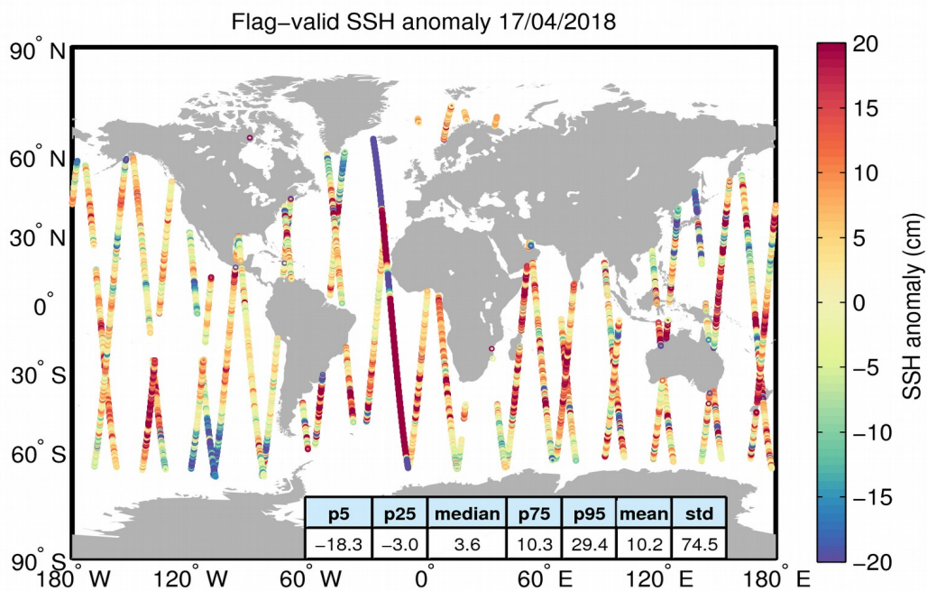
Figure 5. Geographical distribution of flag-valid 1-Hz SSH anomaly data over oceans and lakes for 17/04/2018. The statistical values shown in the table refer to the SSH anomaly in cm and are calculated over all measurements shown in the figure.
