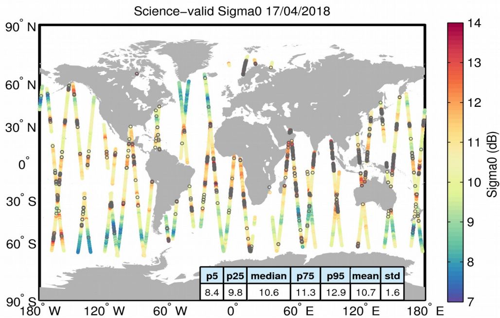
Figure 27. Geographical distribution of science-valid sigma0 data over oceans and lakes for 17/04/2018. The statistical values shown in the table refer to the sigma0 in dB and are calculated over all measurements shown in the figure. Gray circles denote records that have been rejected based on the editing criteria described in Table 4.
