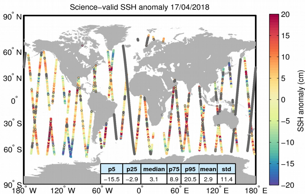
Figure 10. Geographical distribution of science-valid SSH anomaly data over oceans and lakes for 17/04/2018. The statistical values shown in the table refer to the SSH anomaly in cm and are calculated over all measurements shown in the figure. Gray circles denote records that have been rejected based on the editing criteria described in Table 2.
