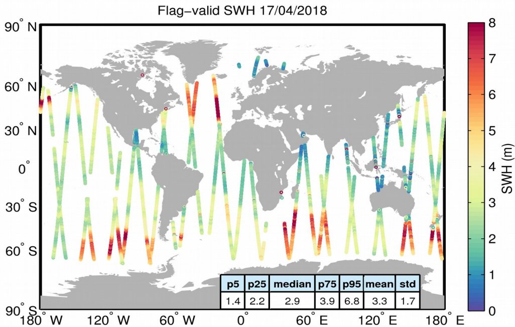
Figure 15. Geographical distribution of flag-valid SWH data over oceans and lakes for 17/04/2018. The statistical values shown in the table refer to the SWH in m and are calculated over all measurements shown in the figure.
