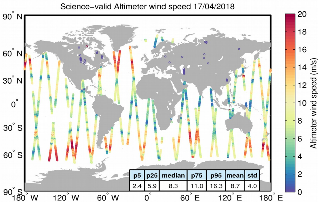
Figure 34. Geographical distribution of science-valid wind data over oceans and lakes for 17/04/2018. The statistical values shown in the table refer to the wind in m/s and are calculated over all measurements shown in the figure. Gray circles denote records that have been rejected based on the editing criteria described in Table 5.
