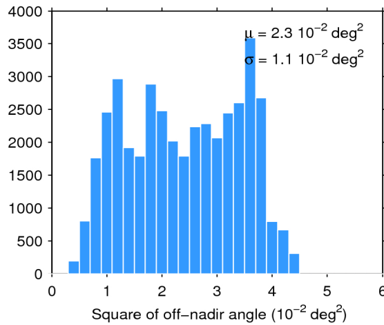
Figure 39. Histogram of flag-valid mispointing over oceans and lakes for 17/04/2018. The mean ( \mu ) and standard deviation ( \sigma ) are also shown. Note that values larger than 6 \cdot 10^{-2} \text{ deg}^2 are excluded from the histogram for the sake of readability but not from the computation of \mu and \sigma .
