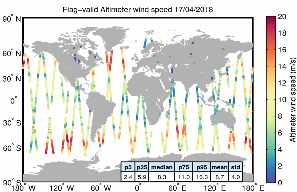
Figure 31. Geographical distribution of flag-valid wind data over oceans and lakes for 17/04/2018. The statistical values shown in the table refer to the wind in m/s and are calculated over all measurements shown in the figure.
