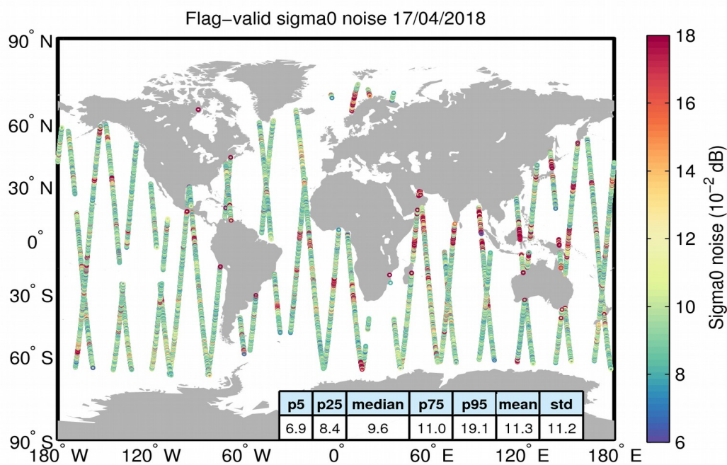
Figure 26. Geographical distribution of flag-valid 20-Hz sigma0 measurement noise over oceans and lakes for 17/04/2018. The statistical values shown in the table refer to the sigma0 noise and are calculated over all measurements shown in the figure.
