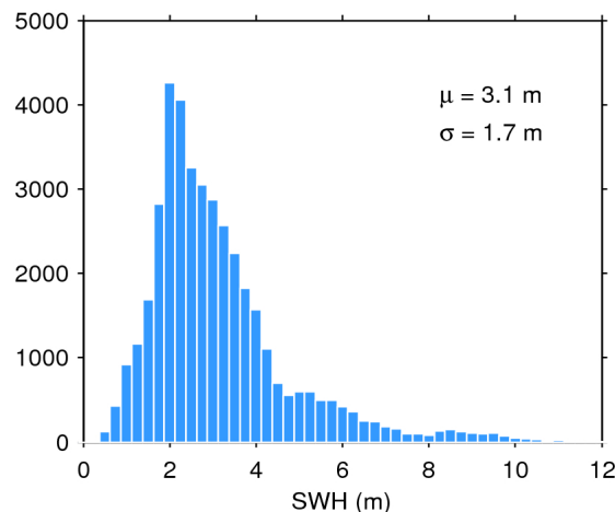
Figure 20. Histogram of science-valid SWH over oceans and lakes for 16/04/2018. The mean ( \mu ) and standard deviation ( \sigma ) are also shown. Note that values larger than 12 m are excluded from the histogram for the sake of readability but not from the computation of \mu and \sigma .
