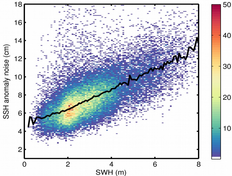
Figure 9. 2D histogram showing flag-valid SSH anomaly noise as a function of SWH for 16/04/2018. The black line denotes the median SSH anomaly noise as a function of SWH.
