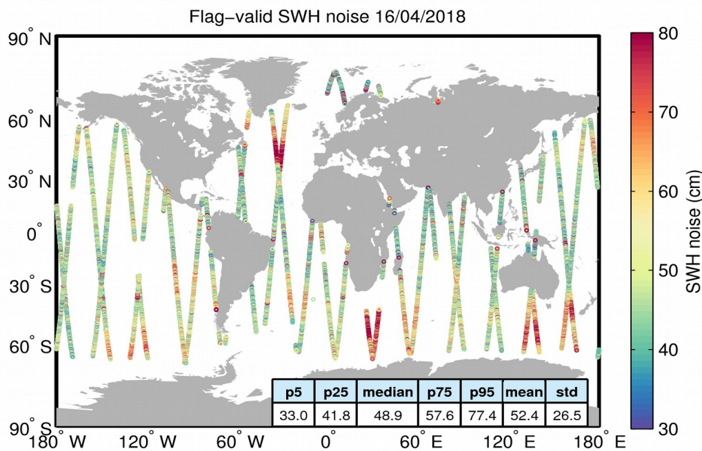
Figure 18. Geographical distribution of flag-valid 20-Hz SWH measurement noise over oceans and lakes for 16/04/2018. The statistical values shown in the table refer to the SWH noise and are calculated over all measurements shown in the figure.
