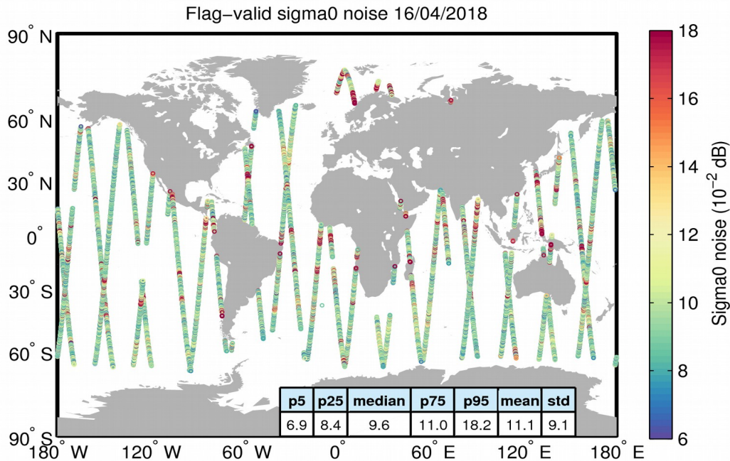
Figure 26. Geographical distribution of flag-valid 20-Hz sigma0 measurement noise over oceans and lakes for 16/04/2018. The statistical values shown in the table refer to the sigma0 noise and are calculated over all measurements shown in the figure.
