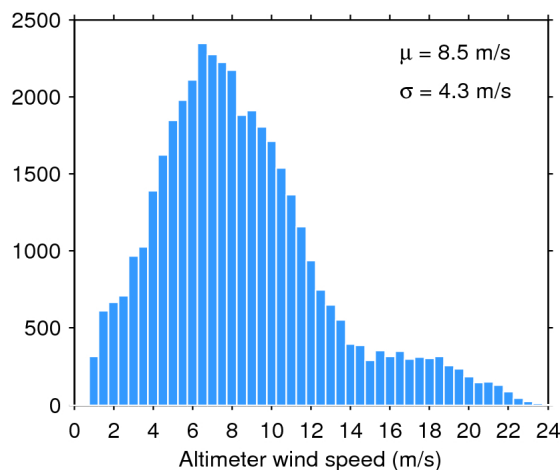
Figure 35. Histogram of science-valid wind over oceans and lakes for 16/04/2018. The mean ( \mu ) and standard deviation ( \sigma ) are also shown. Note that values larger than 24 m/s are excluded from the histogram for the sake of readability but not from the computation of \mu and \sigma .
