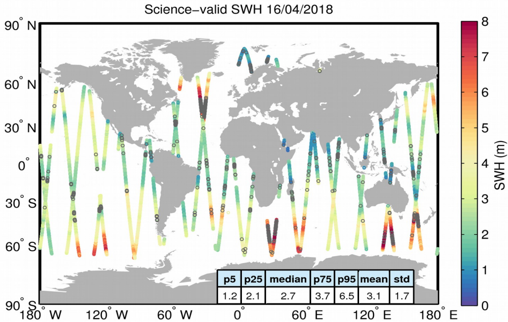
Figure 19. Geographical distribution of science-valid SWH data over oceans and lakes for 16/04/2018. The statistical values shown in the table refer to the SWH in m and are calculated over all measurements shown in the figure. Gray circles denote records that have been rejected based on the editing criteria described in Table 3.
