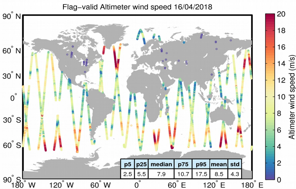
Figure 31. Geographical distribution of flag-valid wind data over oceans and lakes for 16/04/2018. The statistical values shown in the table refer to the wind in m/s and are calculated over all measurements shown in the figure.
