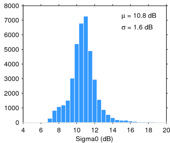
Figure 28. Histogram of science-valid sigma0 over oceans and lakes for 16/04/2018. The mean ( \mu ) and standard deviation ( \sigma ) are also shown. Note that values outside [4 20] dB are excluded from the histogram for the sake of readability but not from the computation of \mu and \sigma .
