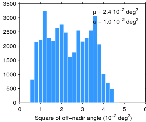
Figure 39. Histogram of flag-valid mispointing over oceans and lakes for 16/04/2018. The mean ( \mu ) and standard deviation ( \sigma ) are also shown. Note that values larger than 6 \cdot 10^{-2} \text{ deg}^2 are excluded from the histogram for the sake of readability but not from the computation of \mu and \sigma .
