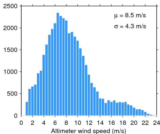
Figure 33. Histogram of flag-valid wind over oceans and lakes for 16/04/2018. The mean ( \mu ) and standard deviation ( \sigma ) are also shown. Note that values larger than 24 m/s are excluded from the histogram for the sake of readability but not from the computation of \mu and \sigma .
