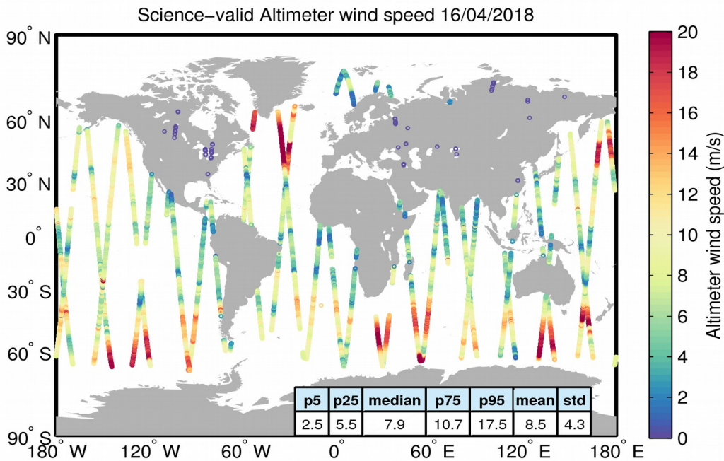
Figure 34. Geographical distribution of science-valid wind data over oceans and lakes for 16/04/2018. The statistical values shown in the table refer to the wind in m/s and are calculated over all measurements shown in the figure. Gray circles denote records that have been rejected based on the editing criteria described in Table 5.
