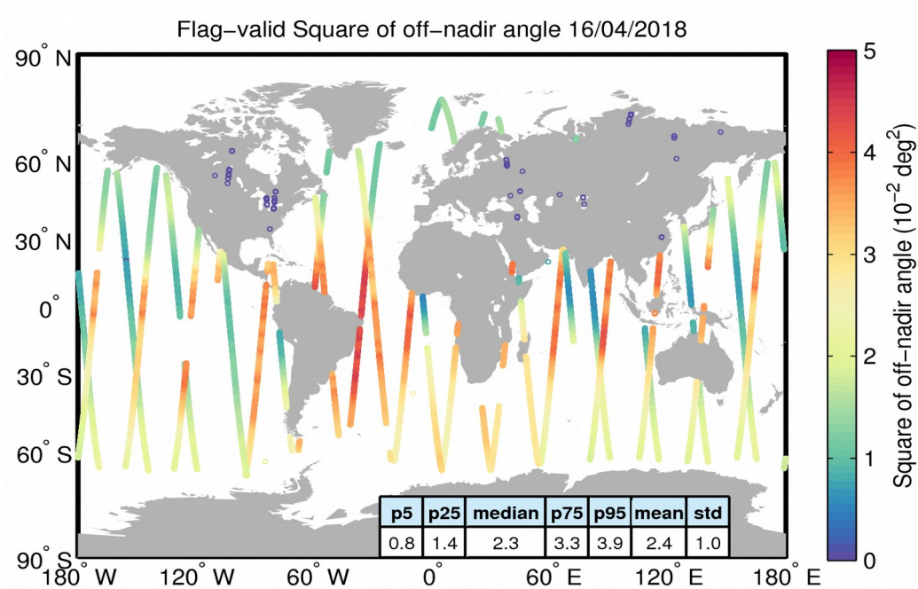
Figure 37. Geographical distribution of flag-valid mispointing data over oceans and lakes for 16/04/2018. The statistical values shown in the table refer to the mispointing in 10^{-2} deg 2 and are calculated over all measurements shown in the figure.
