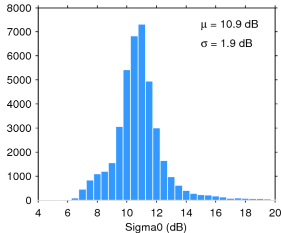
Figure 25. Histogram of flag-valid sigma0 over oceans and lakes for 16/04/2018. The mean ( \mu ) and standard deviation ( \sigma ) are also shown. Note that values outside [4 20] dB are excluded from the histogram for the sake of readability but not from the computation of \mu and \sigma .
