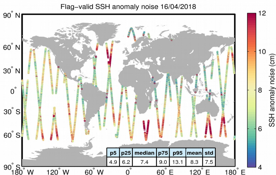
Figure 8. Geographical distribution of flag-valid 20-Hz SSH anomaly measurement noise over oceans and lakes for 16/04/2018. The statistical values shown in the table refer to the SSH anomaly noise and are calculated over all measurements shown in the figure.
