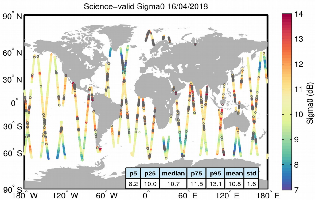
Figure 27. Geographical distribution of science-valid sigma0 data over oceans and lakes for 16/04/2018. The statistical values shown in the table refer to the sigma0 in dB and are calculated over all measurements shown in the figure. Gray circles denote records that have been rejected based on the editing criteria described in Table 4.
