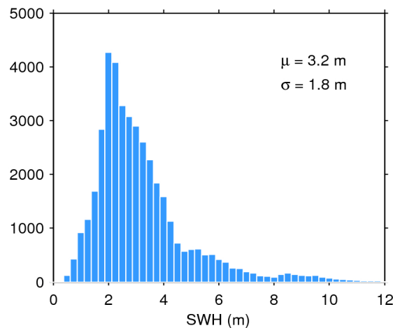
Figure 17. Histogram of flag-valid SWH over oceans and lakes for 16/04/2018. The mean ( \mu ) and standard deviation ( \sigma ) are also shown. Note that values larger than 12 m are excluded from the histogram for the sake of readability but not from the computation of \mu and \sigma .
