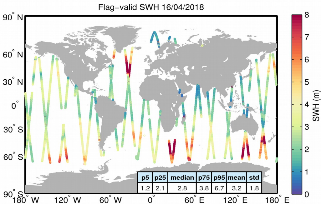
Figure 15. Geographical distribution of flag-valid SWH data over oceans and lakes for 16/04/2018. The statistical values shown in the table refer to the SWH in m and are calculated over all measurements shown in the figure.
