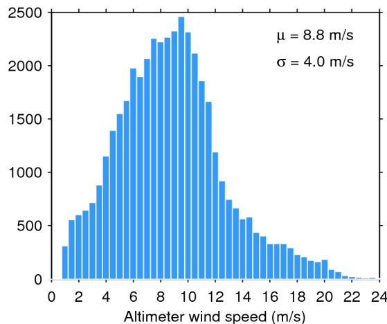
Figure 35. Histogram of science-valid wind over oceans and lakes for 15/04/2018. The mean ( \mu ) and standard deviation ( \sigma ) are also shown. Note that values larger than 24 m/s are excluded from the histogram for the sake of readability but not from the computation of \mu and \sigma .
