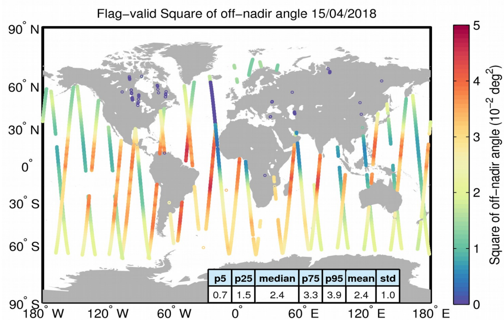
Figure 37. Geographical distribution of flag-valid mispointing data over oceans and lakes for 15/04/2018. The statistical values shown in the table refer to the mispointing in 10^{-2} \text{ deg}^2 and are calculated over all measurements shown in the figure.
