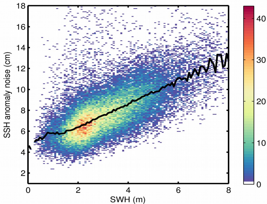
Figure 9. 2D histogram showing flag-valid SSH anomaly noise as a function of SWH for 15/04/2018. The black line denotes the median SSH anomaly noise as a function of SWH.
