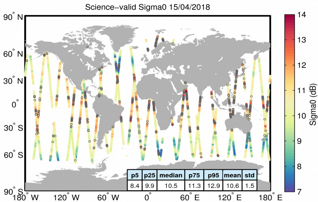
Figure 27. Geographical distribution of science-valid sigma0 data over oceans and lakes for 15/04/2018. The statistical values shown in the table refer to the sigma0 in dB and are calculated over all measurements shown in the figure. Gray circles denote records that have been rejected based on the editing criteria described in Table 4.
