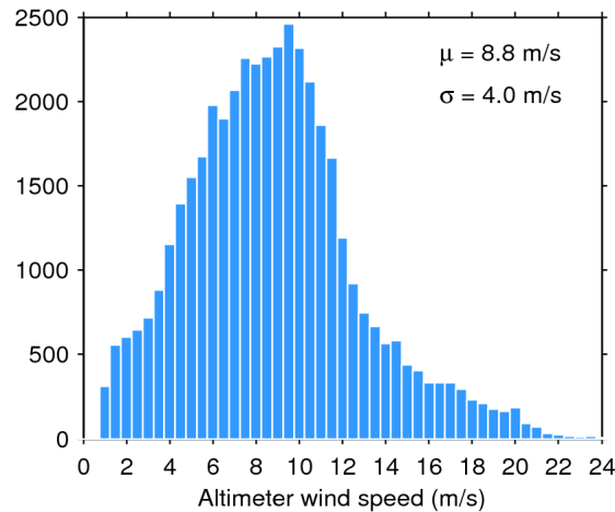
Figure 33. Histogram of flag-valid wind over oceans and lakes for 15/04/2018. The mean ( \mu ) and standard deviation ( \sigma ) are also shown. Note that values larger than 24 m/s are excluded from the histogram for the sake of readability but not from the computation of \mu and \sigma .
