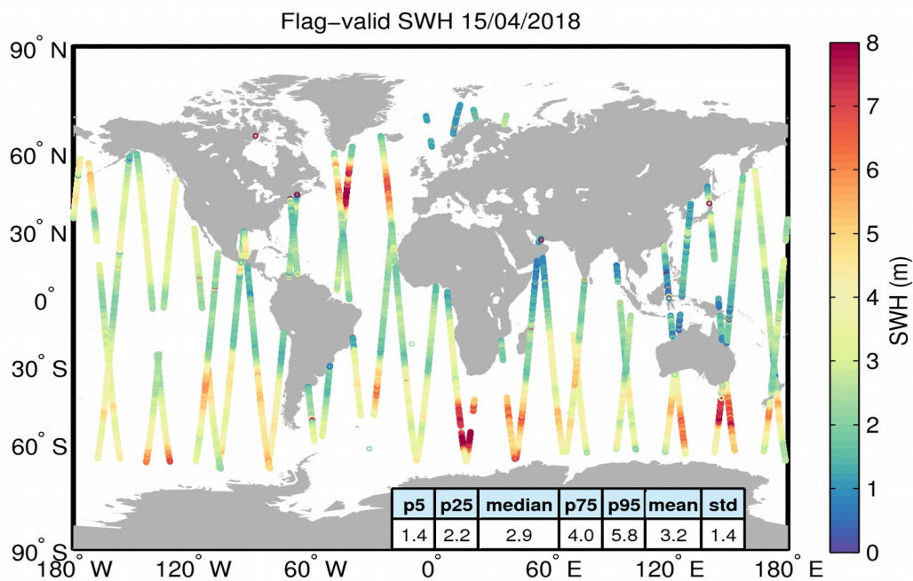
Figure 15. Geographical distribution of flag-valid SWH data over oceans and lakes for 15/04/2018. The statistical values shown in the table refer to the SWH in m and are calculated over all measurements shown in the figure.
