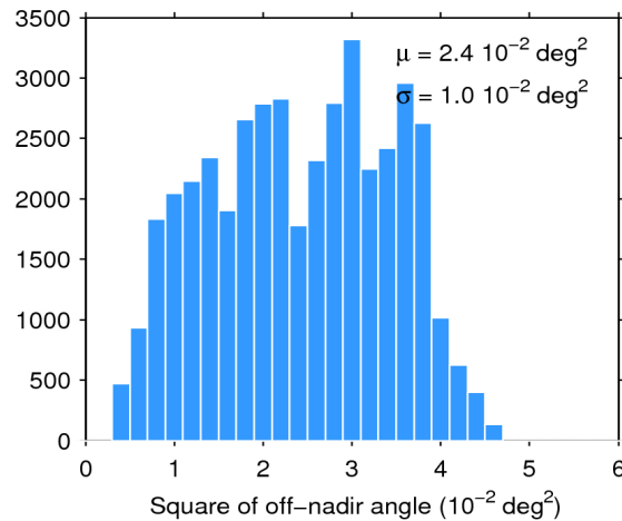
Figure 39. Histogram of flag-valid mispointing over oceans and lakes for 15/04/2018. The mean ( \mu ) and standard deviation ( \sigma ) are also shown. Note that values larger than 6 \cdot 10^{-2} \text{ deg}^2 are excluded from the histogram for the sake of readability but not from the computation of \mu and \sigma .
