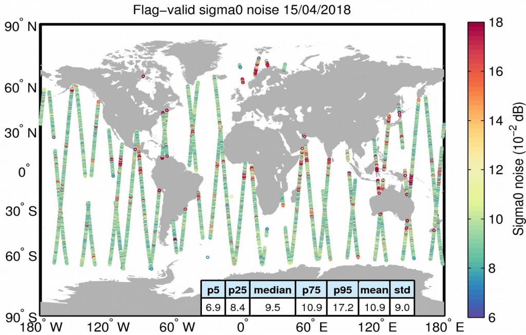
Figure 26. Geographical distribution of flag-valid 20-Hz sigma0 measurement noise over oceans and lakes for 15/04/2018. The statistical values shown in the table refer to the sigma0 noise and are calculated over all measurements shown in the figure.
