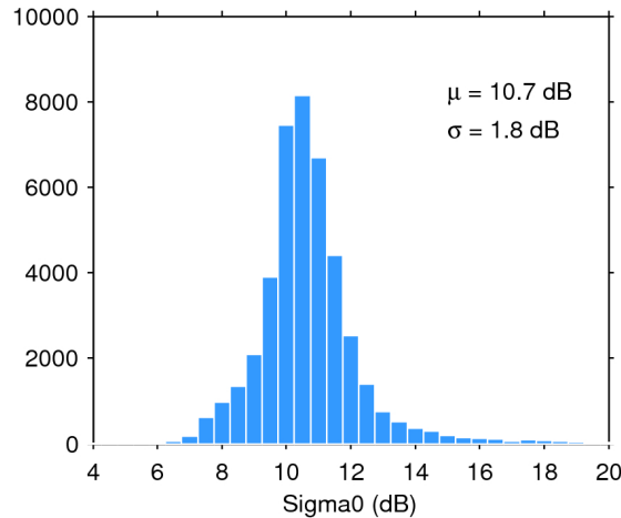
Figure 25. Histogram of flag-valid sigma0 over oceans and lakes for 15/04/2018. The mean ( \mu ) and standard deviation ( \sigma ) are also shown. Note that values outside [4 20] dB are excluded from the histogram for the sake of readability but not from the computation of \mu and \sigma .
