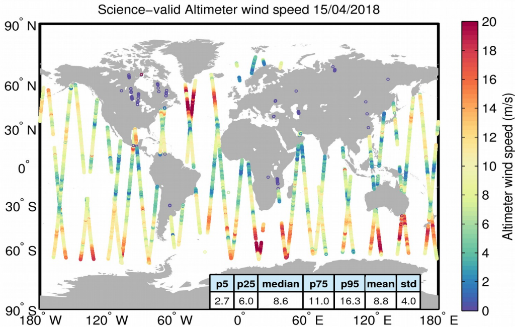
Figure 34. Geographical distribution of science-valid wind data over oceans and lakes for 15/04/2018. The statistical values shown in the table refer to the wind in m/s and are calculated over all measurements shown in the figure. Gray circles denote records that have been rejected based on the editing criteria described in Table 5.
