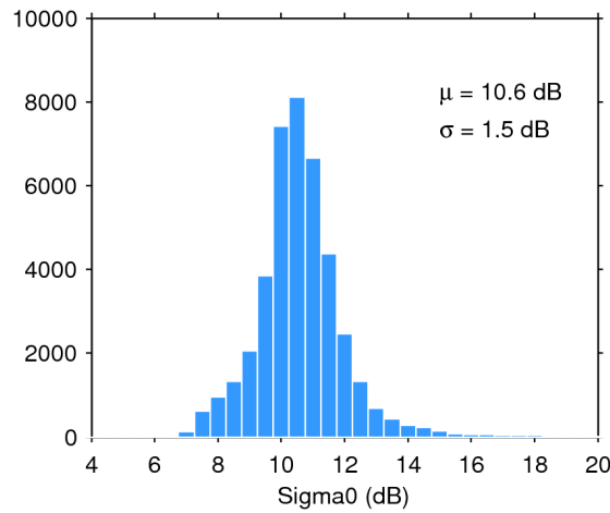
Figure 28. Histogram of science-valid sigma0 over oceans and lakes for 15/04/2018. The mean ( \mu ) and standard deviation ( \sigma ) are also shown. Note that values outside [4 20] dB are excluded from the histogram for the sake of readability but not from the computation of \mu and \sigma .
