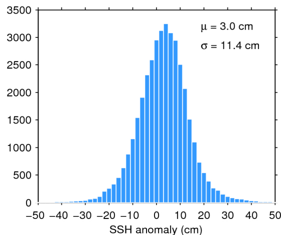
Figure 11. Histogram of science-valid SSH anomaly over oceans and lakes for 15/04/2018. The mean ( \mu ) and standard deviation ( \sigma ) are also shown. Note that values outside [-50 50] cm are excluded from the histogram for the sake of readability but not from the computation of \mu and \sigma .
