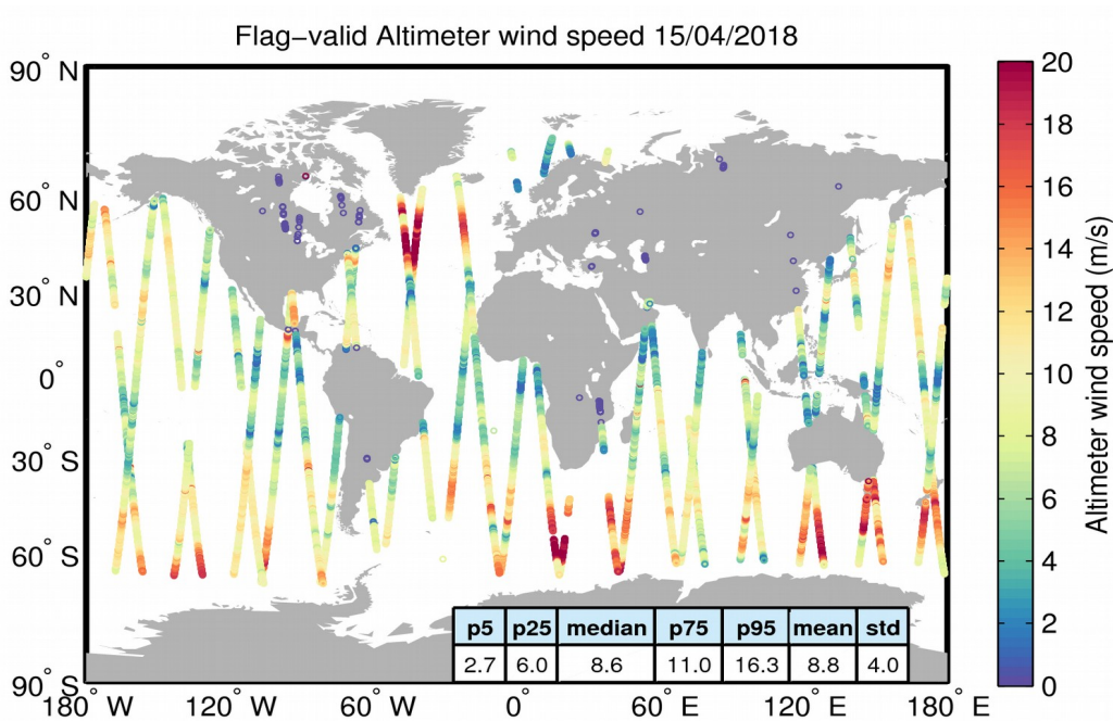
Figure 31. Geographical distribution of flag-valid wind data over oceans and lakes for 15/04/2018. The statistical values shown in the table refer to the wind in m/s and are calculated over all measurements shown in the figure.
