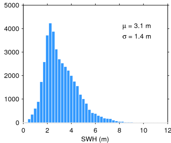
Figure 20. Histogram of science-valid SWH over oceans and lakes for 15/04/2018. The mean ( \mu ) and standard deviation ( \sigma ) are also shown. Note that values larger than 12 m are excluded from the histogram for the sake of readability but not from the computation of \mu and \sigma .
