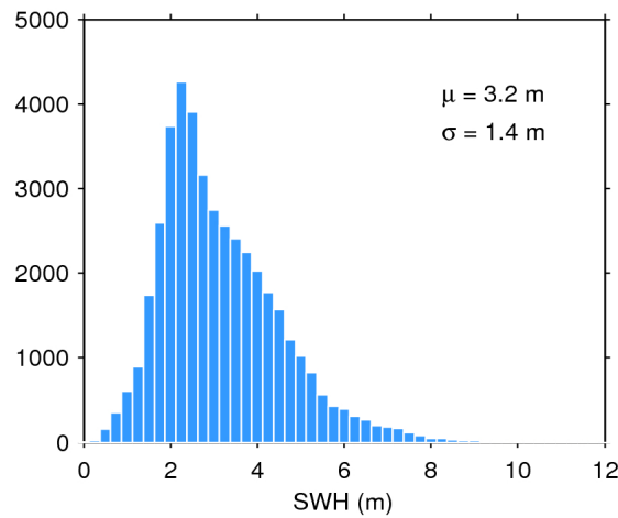
Figure 17. Histogram of flag-valid SWH over oceans and lakes for 15/04/2018. The mean ( \mu ) and standard deviation ( \sigma ) are also shown. Note that values larger than 12 m are excluded from the histogram for the sake of readability but not from the computation of \mu and \sigma .
