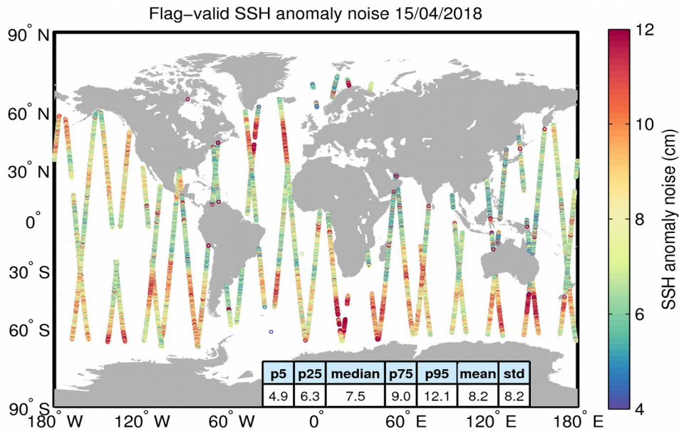
Figure 8. Geographical distribution of flag-valid 20-Hz SSH anomaly measurement noise over oceans and lakes for 15/04/2018. The statistical values shown in the table refer to the SSH anomaly noise and are calculated over all measurements shown in the figure.
