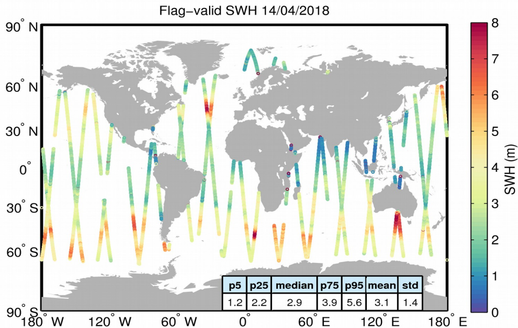
Figure 15. Geographical distribution of flag-valid SWH data over oceans and lakes for 14/04/2018. The statistical values shown in the table refer to the SWH in m and are calculated over all measurements shown in the figure.
