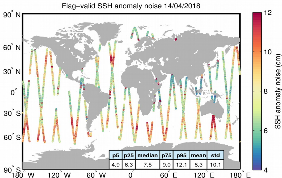
Figure 8. Geographical distribution of flag-valid 20-Hz SSH anomaly measurement noise over oceans and lakes for 14/04/2018. The statistical values shown in the table refer to the SSH anomaly noise and are calculated over all measurements shown in the figure.
