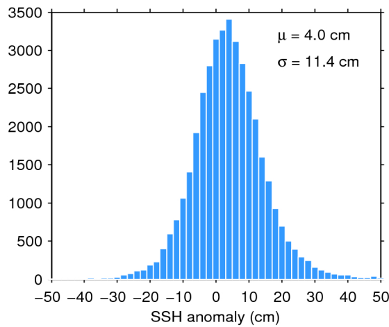
Figure 11. Histogram of science-valid SSH anomaly over oceans and lakes for 14/04/2018. The mean ( \mu ) and standard deviation ( \sigma ) are also shown. Note that values outside [-50 50] cm are excluded from the histogram for the sake of readability but not from the computation of \mu and \sigma .
