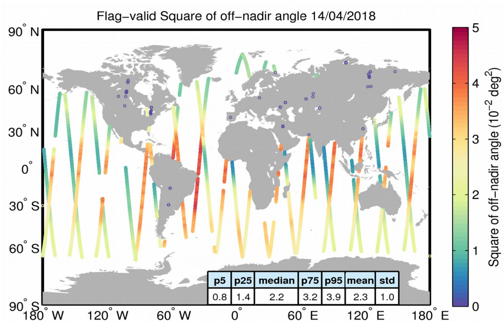
Figure 37. Geographical distribution of flag-valid mispointing data over oceans and lakes for 14/04/2018. The statistical values shown in the table refer to the mispointing in 10^{-2} deg 2 and are calculated over all measurements shown in the figure.
