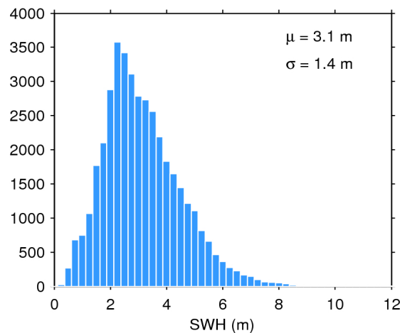
Figure 17. Histogram of flag-valid SWH over oceans and lakes for 14/04/2018. The mean ( \mu ) and standard deviation ( \sigma ) are also shown. Note that values larger than 12 m are excluded from the histogram for the sake of readability but not from the computation of \mu and \sigma .
