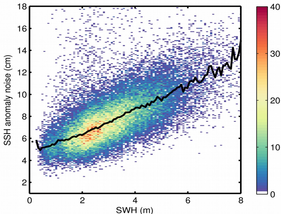
Figure 9. 2D histogram showing flag-valid SSH anomaly noise as a function of SWH for 14/04/2018. The black line denotes the median SSH anomaly noise as a function of SWH.
