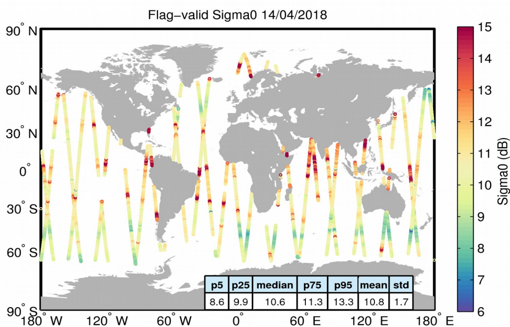
Figure 23. Geographical distribution of flag-valid sigma0 data over oceans and lakes for 14/04/2018. The statistical values shown in the table refer to the sigma0 in dB and are calculated over all measurements shown in the figure.
