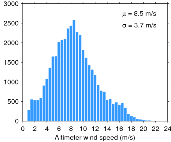
Figure 33. Histogram of flag-valid wind over oceans and lakes for 14/04/2018. The mean ( \mu ) and standard deviation ( \sigma ) are also shown. Note that values larger than 24 m/s are excluded from the histogram for the sake of readability but not from the computation of \mu and \sigma .
