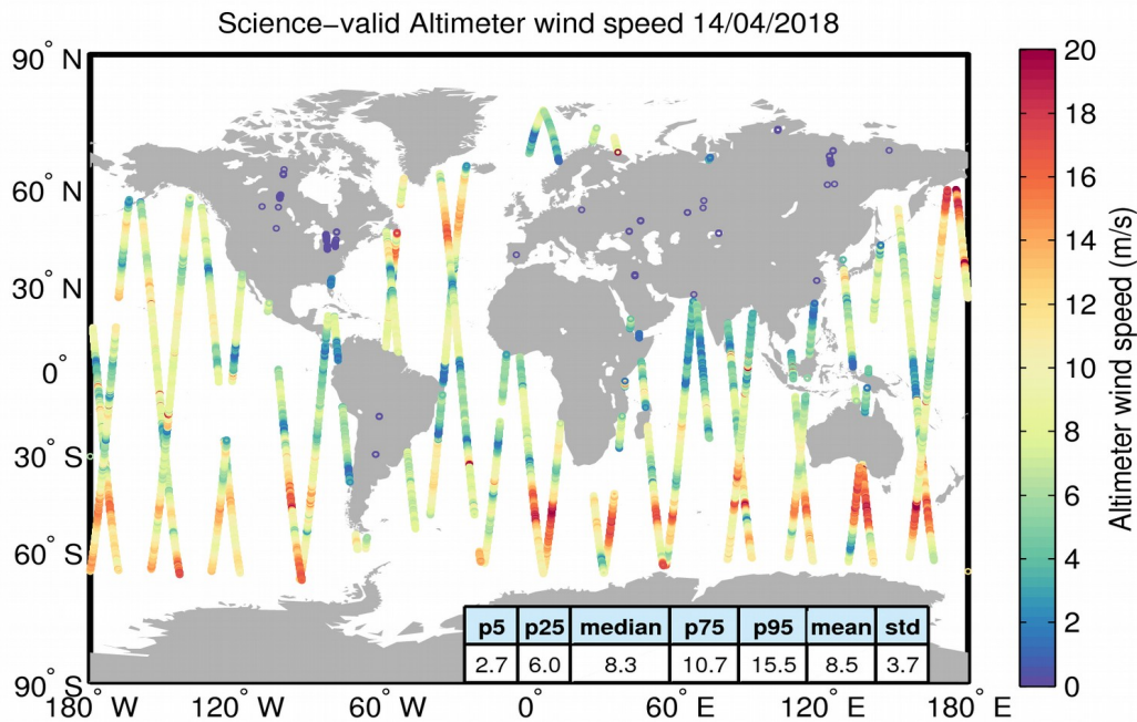
Figure 34. Geographical distribution of science-valid wind data over oceans and lakes for 14/04/2018. The statistical values shown in the table refer to the wind in m/s and are calculated over all measurements shown in the figure. Gray circles denote records that have been rejected based on the editing criteria described in Table 5.
