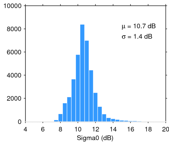
Figure 28. Histogram of science-valid sigma0 over oceans and lakes for 14/04/2018. The mean ( \mu ) and standard deviation ( \sigma ) are also shown. Note that values outside [4 20] dB are excluded from the histogram for the sake of readability but not from the computation of \mu and \sigma .
