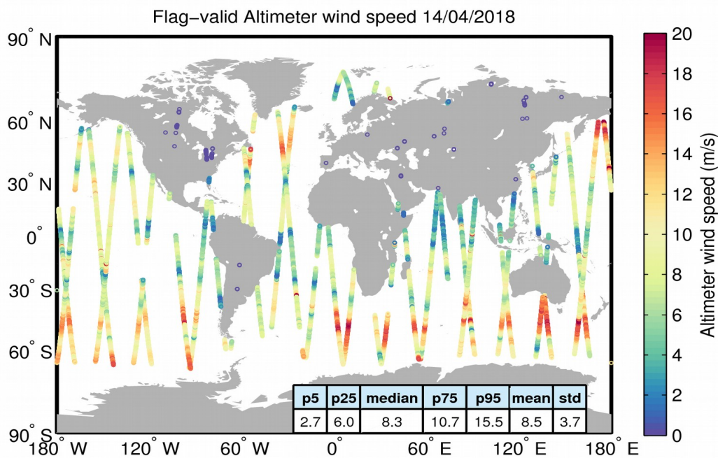
Figure 31. Geographical distribution of flag-valid wind data over oceans and lakes for 14/04/2018. The statistical values shown in the table refer to the wind in m/s and are calculated over all measurements shown in the figure.
