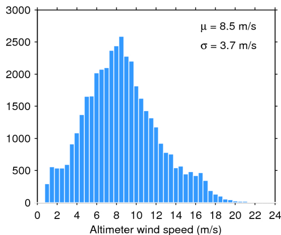
Figure 35. Histogram of science-valid wind over oceans and lakes for 14/04/2018. The mean ( \mu ) and standard deviation ( \sigma ) are also shown. Note that values larger than 24 m/s are excluded from the histogram for the sake of readability but not from the computation of \mu and \sigma .
