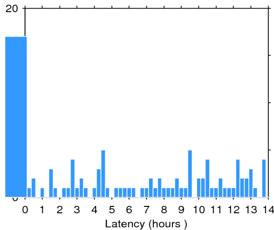
Figure 2. Histogram of the data latency for 14/04/2018. The y-axis denotes the number of files that are made available with a delay of x-hours with respect to the mean time of the records stored in the file.
