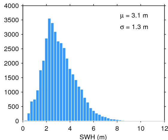
Figure 20. Histogram of science-valid SWH over oceans and lakes for 14/04/2018. The mean ( \mu ) and standard deviation ( \sigma ) are also shown. Note that values larger than 12 m are excluded from the histogram for the sake of readability but not from the computation of \mu and \sigma .
