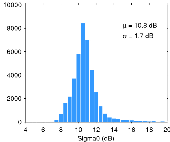
Figure 25. Histogram of flag-valid sigma0 over oceans and lakes for 14/04/2018. The mean ( \mu ) and standard deviation ( \sigma ) are also shown. Note that values outside [4 20] dB are excluded from the histogram for the sake of readability but not from the computation of \mu and \sigma .
