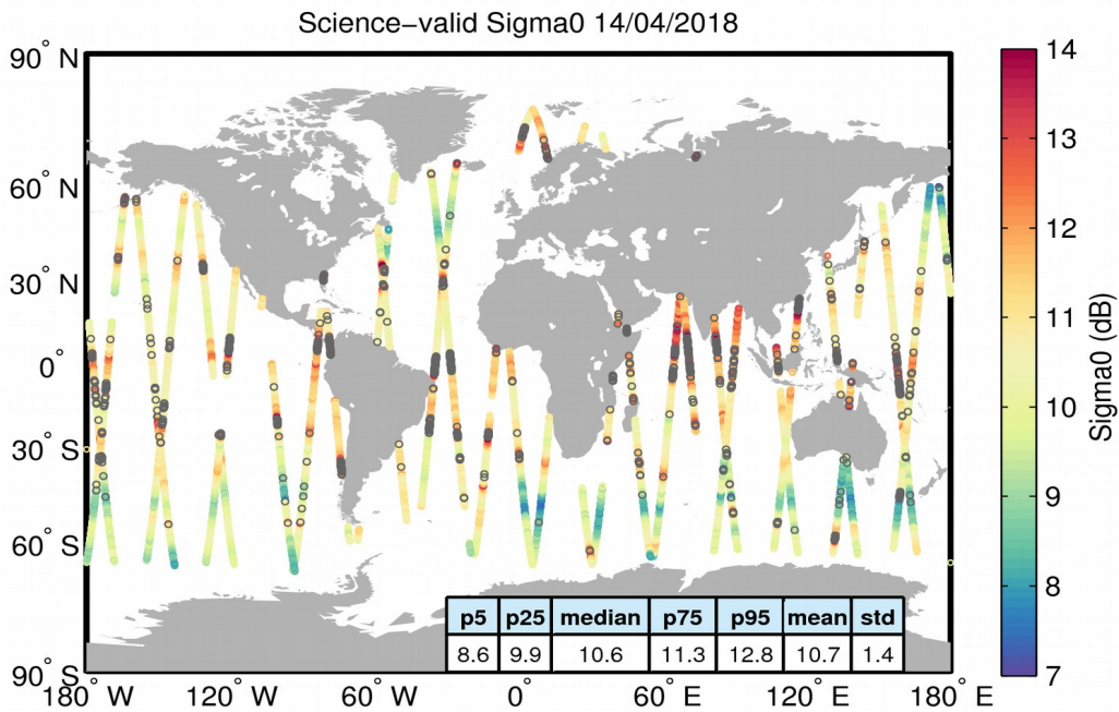
Figure 27. Geographical distribution of science-valid sigma0 data over oceans and lakes for 14/04/2018. The statistical values shown in the table refer to the sigma0 in dB and are calculated over all measurements shown in the figure. Gray circles denote records that have been rejected based on the editing criteria described in Table 4.
