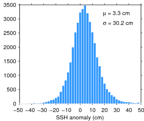
Figure 7. Histogram of flag-valid SSH anomaly over oceans and lakes for 14/04/2018. The mean ( \mu ) and standard deviation ( \sigma ) are also shown. Note that values outside [-50\ 50] cm are excluded from the histogram for the sake of readability but not from the computation of \mu and \sigma .
