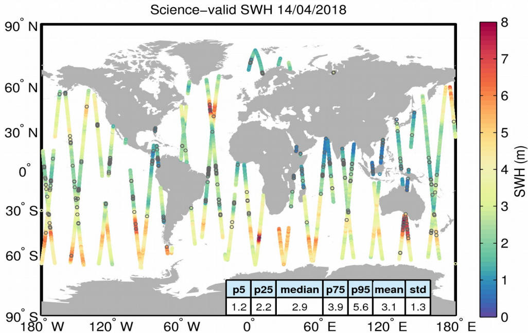
Figure 19. Geographical distribution of science-valid SWH data over oceans and lakes for 14/04/2018. The statistical values shown in the table refer to the SWH in m and are calculated over all measurements shown in the figure. Gray circles denote records that have been rejected based on the editing criteria described in Table 3.
