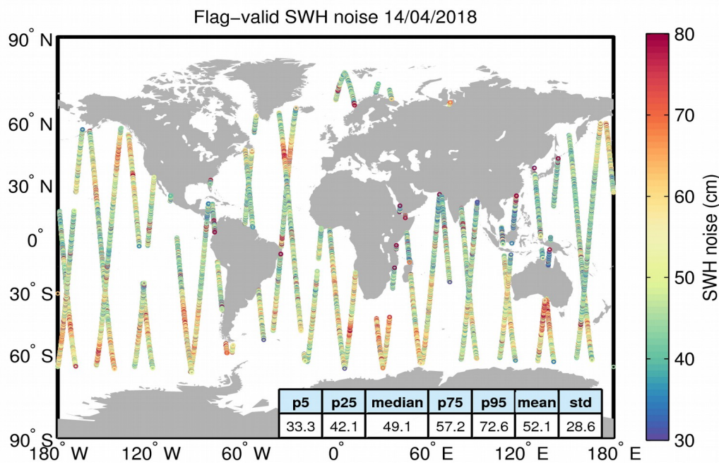
Figure 18. Geographical distribution of flag-valid 20-Hz SWH measurement noise over oceans and lakes for 14/04/2018. The statistical values shown in the table refer to the SWH noise and are calculated over all measurements shown in the figure.
