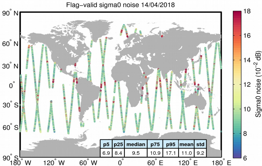
Figure 26. Geographical distribution of flag-valid 20-Hz sigma0 measurement noise over oceans and lakes for 14/04/2018. The statistical values shown in the table refer to the sigma0 noise and are calculated over all measurements shown in the figure.
