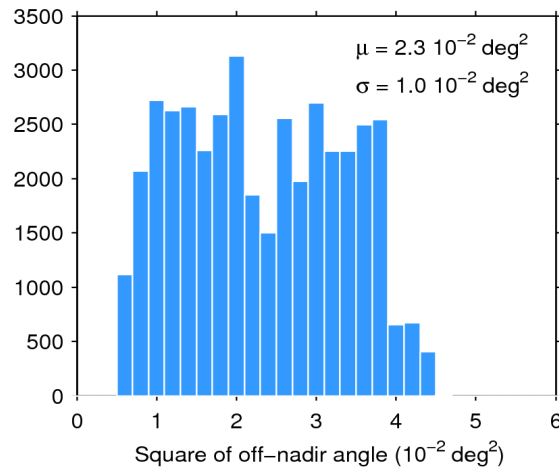
Figure 39. Histogram of flag-valid mispointing over oceans and lakes for 14/04/2018. The mean ( \mu ) and standard deviation ( \sigma ) are also shown. Note that values larger than 6 \cdot 10^{-2} \text{ deg}^2 are excluded from the histogram for the sake of readability but not from the computation of \mu and \sigma .
