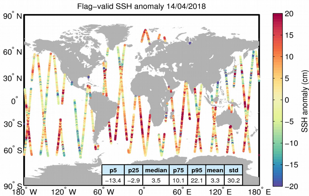
Figure 5. Geographical distribution of flag-valid 1-Hz SSH anomaly data over oceans and lakes for 14/04/2018. The statistical values shown in the table refer to the SSH anomaly in cm and are calculated over all measurements shown in the figure.
