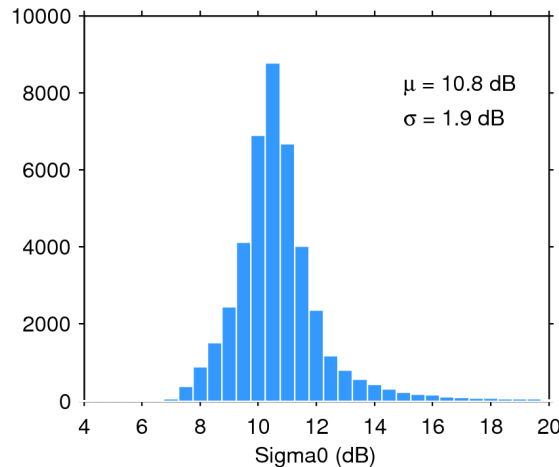
Figure 25. Histogram of flag-valid sigma0 over oceans and lakes for 13/04/2018. The mean ( \mu ) and standard deviation ( \sigma ) are also shown. Note that values outside [4 20] dB are excluded from the histogram for the sake of readability but not from the computation of \mu and \sigma .
