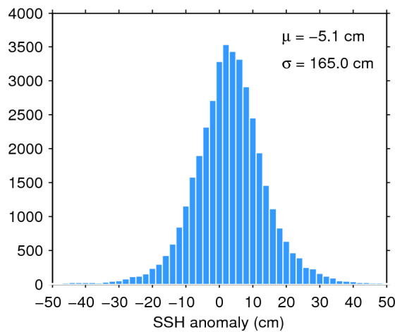
Figure 7. Histogram of flag-valid SSH anomaly over oceans and lakes for 13/04/2018. The mean ( \mu ) and standard deviation ( \sigma ) are also shown. Note that values outside [-50\ 50] cm are excluded from the histogram for the sake of readability but not from the computation of \mu and \sigma .
