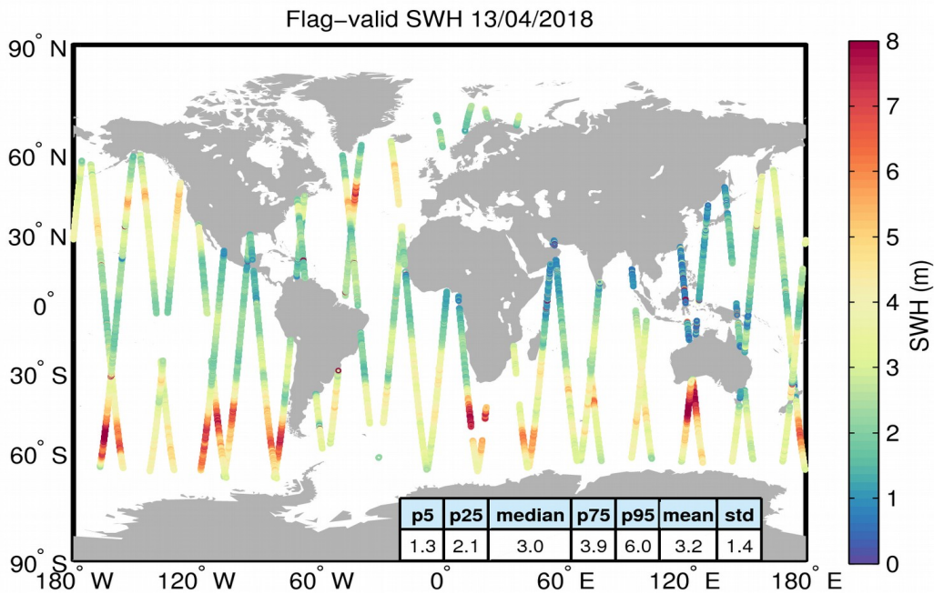
Figure 15. Geographical distribution of flag-valid SWH data over oceans and lakes for 13/04/2018. The statistical values shown in the table refer to the SWH in m and are calculated over all measurements shown in the figure.
