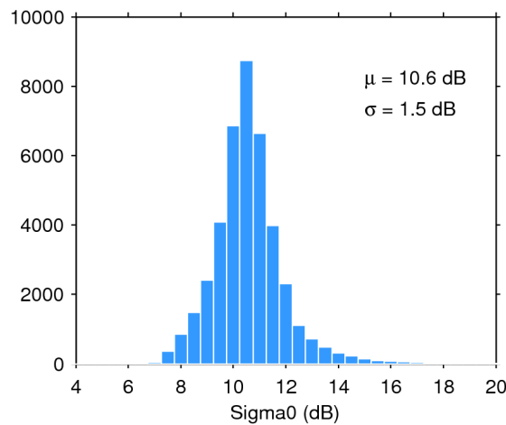
Figure 28. Histogram of science-valid sigma0 over oceans and lakes for 13/04/2018. The mean ( \mu ) and standard deviation ( \sigma ) are also shown. Note that values outside [4 20] dB are excluded from the histogram for the sake of readability but not from the computation of \mu and \sigma .
