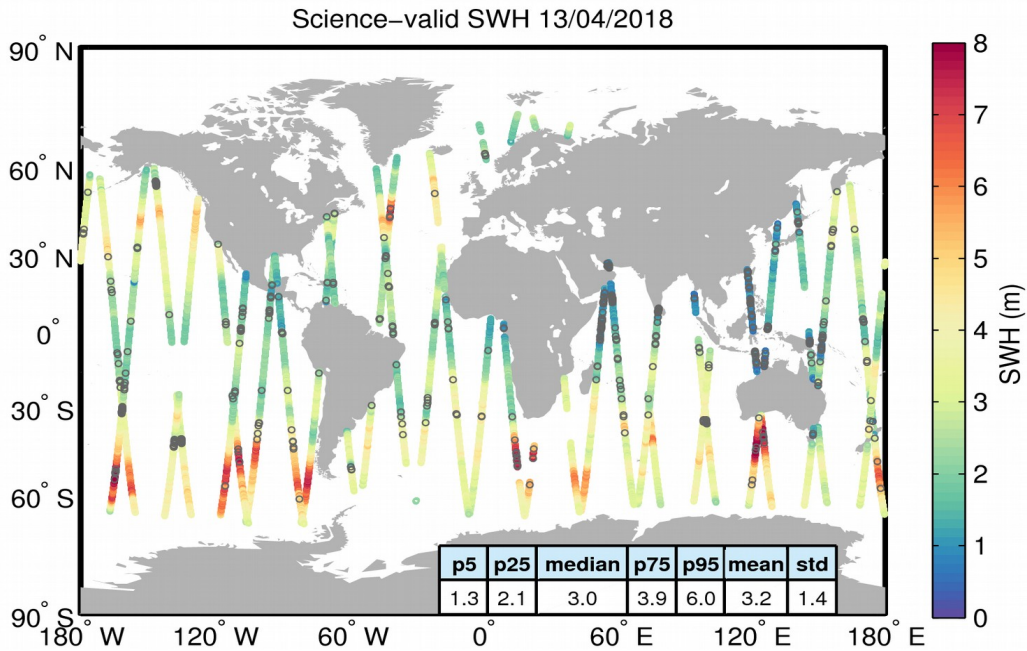
Figure 19. Geographical distribution of science-valid SWH data over oceans and lakes for 13/04/2018. The statistical values shown in the table refer to the SWH in m and are calculated over all measurements shown in the figure. Gray circles denote records that have been rejected based on the editing criteria described in Table 3.
