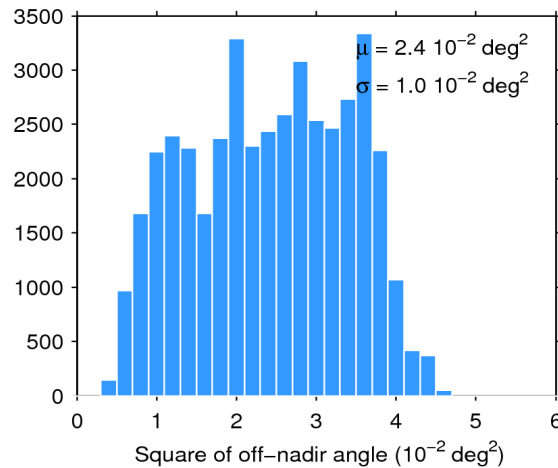
Figure 39. Histogram of flag-valid mispointing over oceans and lakes for 13/04/2018. The mean ( \mu ) and standard deviation ( \sigma ) are also shown. Note that values larger than 6 \cdot 10^{-2} \text{ deg}^2 are excluded from the histogram for the sake of readability but not from the computation of \mu and \sigma .
