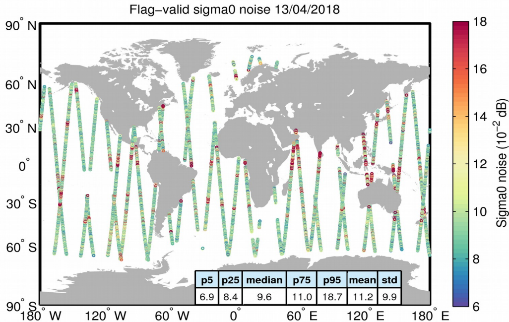
Figure 26. Geographical distribution of flag-valid 20-Hz sigma0 measurement noise over oceans and lakes for 13/04/2018. The statistical values shown in the table refer to the sigma0 noise and are calculated over all measurements shown in the figure.
