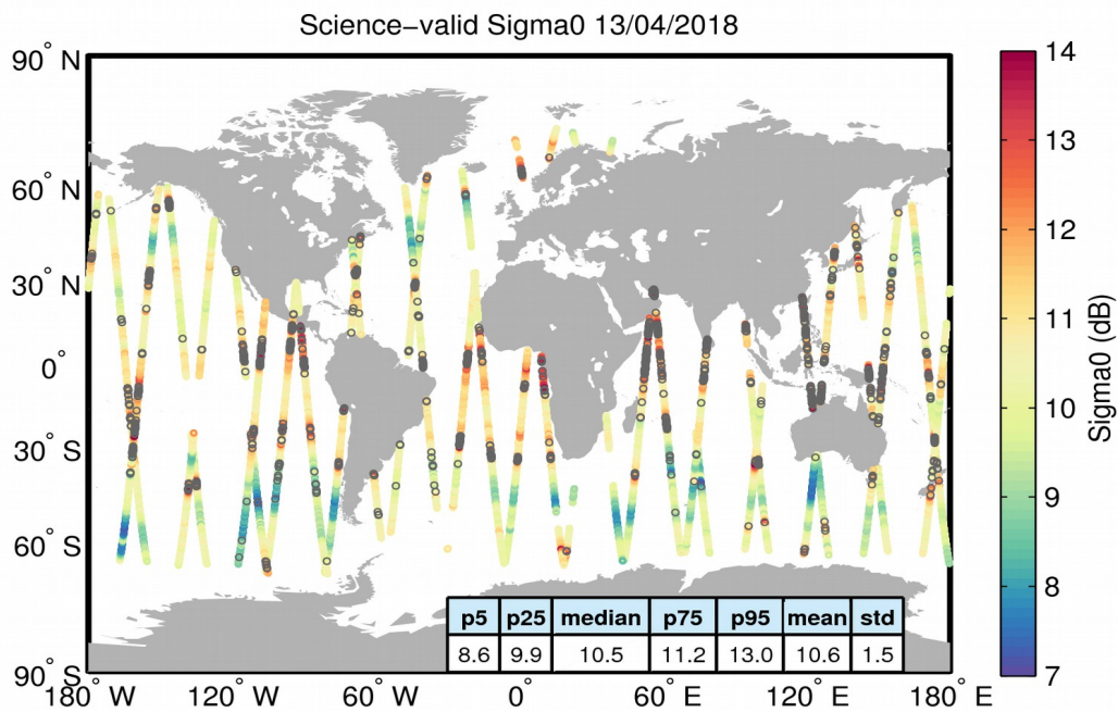
Figure 27. Geographical distribution of science-valid sigma0 data over oceans and lakes for 13/04/2018. The statistical values shown in the table refer to the sigma0 in dB and are calculated over all measurements shown in the figure. Gray circles denote records that have been rejected based on the editing criteria described in Table 4.
