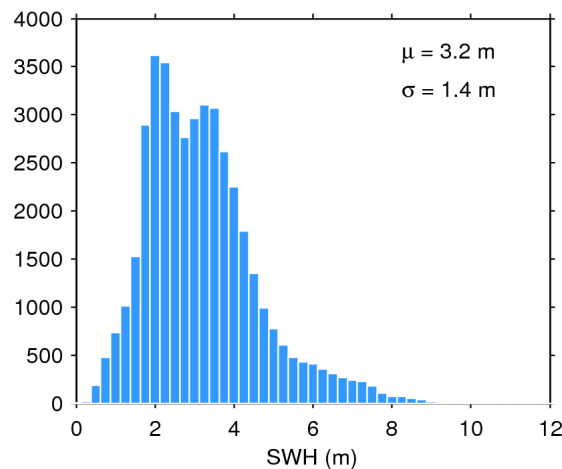
Figure 17. Histogram of flag-valid SWH over oceans and lakes for 13/04/2018. The mean ( \mu ) and standard deviation ( \sigma ) are also shown. Note that values larger than 12 m are excluded from the histogram for the sake of readability but not from the computation of \mu and \sigma .
