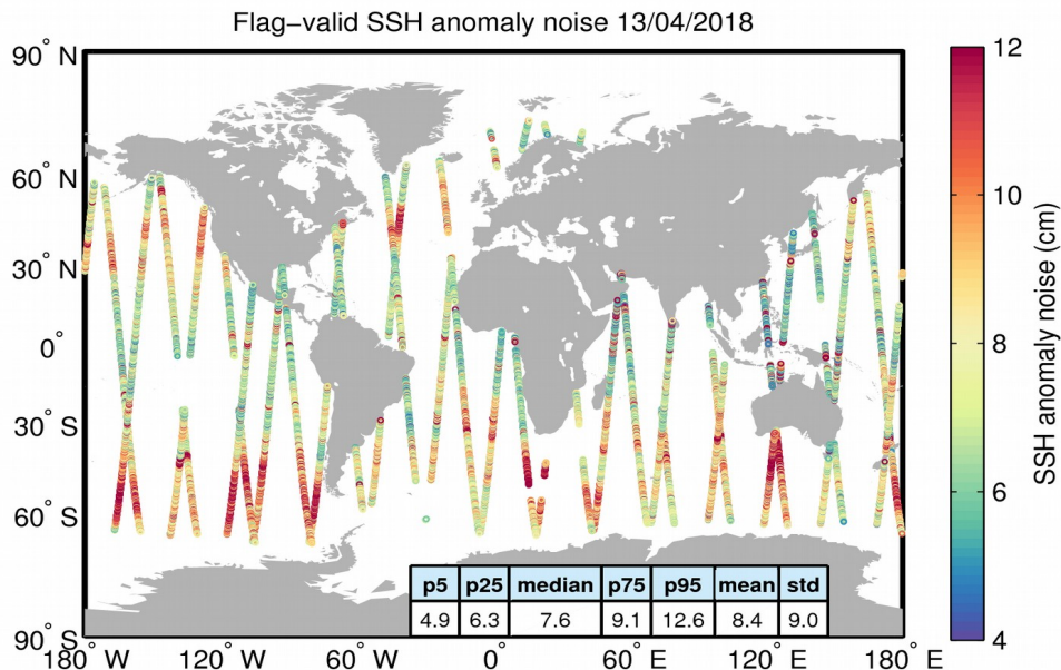
Figure 8. Geographical distribution of flag-valid 20-Hz SSH anomaly measurement noise over oceans and lakes for 13/04/2018. The statistical values shown in the table refer to the SSH anomaly noise and are calculated over all measurements shown in the figure.
