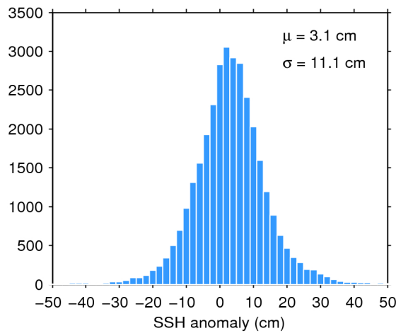
Figure 11. Histogram of science-valid SSH anomaly over oceans and lakes for 13/04/2018. The mean ( \mu ) and standard deviation ( \sigma ) are also shown. Note that values outside [-50 50] cm are excluded from the histogram for the sake of readability but not from the computation of \mu and \sigma .
