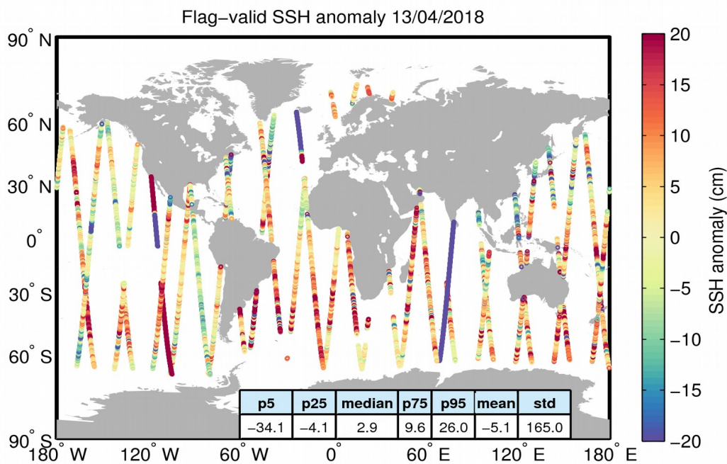
Figure 5. Geographical distribution of flag-valid 1-Hz SSH anomaly data over oceans and lakes for 13/04/2018. The statistical values shown in the table refer to the SSH anomaly in cm and are calculated over all measurements shown in the figure.
