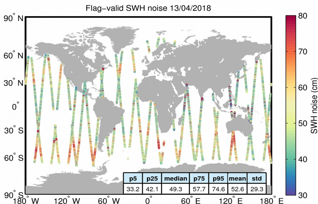
Figure 18. Geographical distribution of flag-valid 20-Hz SWH measurement noise over oceans and lakes for 13/04/2018. The statistical values shown in the table refer to the SWH noise and are calculated over all measurements shown in the figure.
