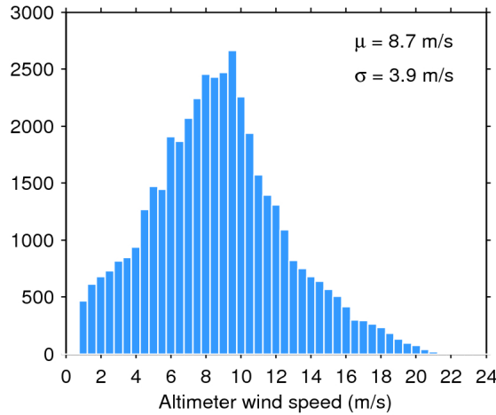
Figure 33. Histogram of flag-valid wind over oceans and lakes for 13/04/2018. The mean ( \mu ) and standard deviation ( \sigma ) are also shown. Note that values larger than 24 m/s are excluded from the histogram for the sake of readability but not from the computation of \mu and \sigma .
