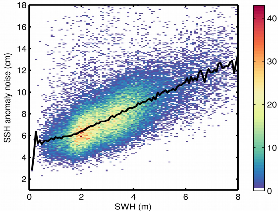
Figure 9. 2D histogram showing flag-valid SSH anomaly noise as a function of SWH for 13/04/2018. The black line denotes the median SSH anomaly noise as a function of SWH.
