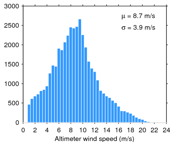
Figure 35. Histogram of science-valid wind over oceans and lakes for 13/04/2018. The mean ( \mu ) and standard deviation ( \sigma ) are also shown. Note that values larger than 24 m/s are excluded from the histogram for the sake of readability but not from the computation of \mu and \sigma .
