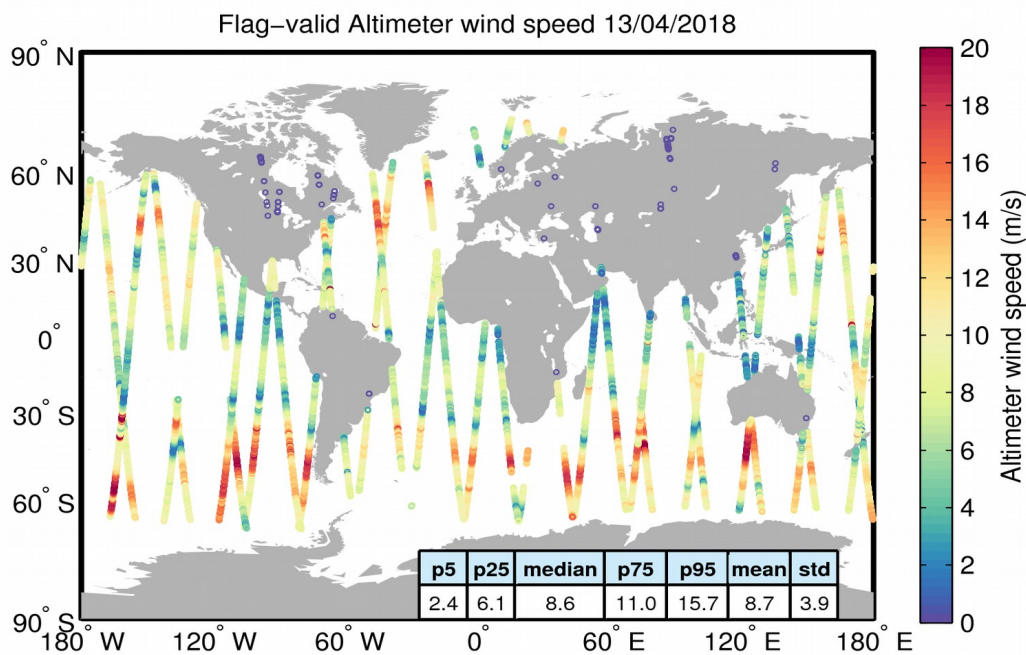
Figure 31. Geographical distribution of flag-valid wind data over oceans and lakes for 13/04/2018. The statistical values shown in the table refer to the wind in m/s and are calculated over all measurements shown in the figure.
