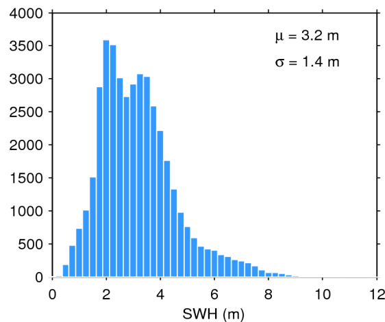
Figure 20. Histogram of science-valid SWH over oceans and lakes for 13/04/2018. The mean ( \mu ) and standard deviation ( \sigma ) are also shown. Note that values larger than 12 m are excluded from the histogram for the sake of readability but not from the computation of \mu and \sigma .
