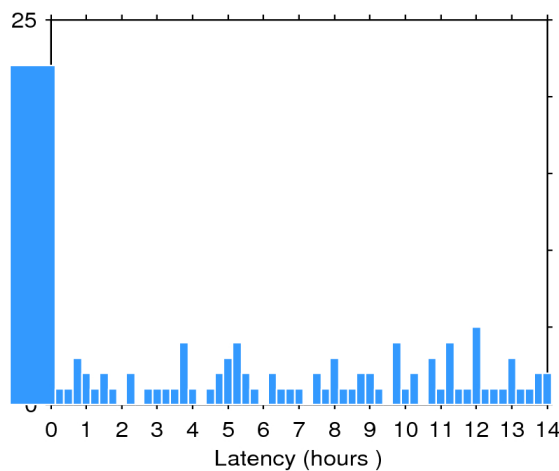
Figure 2. Histogram of the data latency for 13/04/2018. The y-axis denotes the number of files that are made available with a delay of x-hours with respect to the mean time of the records stored in the file.
