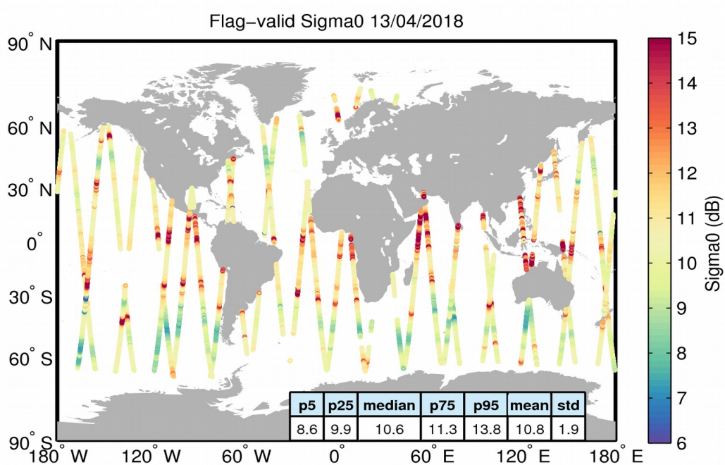
Figure 23. Geographical distribution of flag-valid sigma0 data over oceans and lakes for 13/04/2018. The statistical values shown in the table refer to the sigma0 in dB and are calculated over all measurements shown in the figure.
