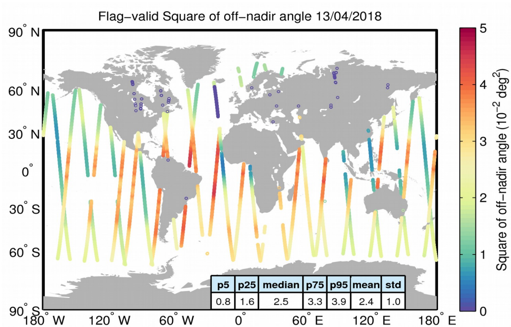
Figure 37. Geographical distribution of flag-valid mispointing data over oceans and lakes for 13/04/2018. The statistical values shown in the table refer to the mispointing in 10^{-2} \text{ deg}^2 and are calculated over all measurements shown in the figure.
