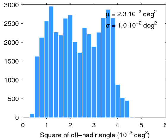
Figure 39. Histogram of flag-valid mispointing over oceans and lakes for 12/04/2018. The mean ( \mu ) and standard deviation ( \sigma ) are also shown. Note that values larger than 6 \cdot 10^{-2} \text{ deg}^2 are excluded from the histogram for the sake of readability but not from the computation of \mu and \sigma .
