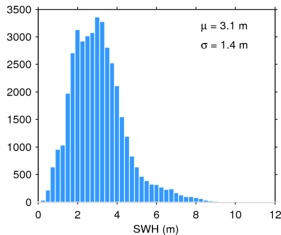
Figure 20. Histogram of science-valid SWH over oceans and lakes for 12/04/2018. The mean ( \mu ) and standard deviation ( \sigma ) are also shown. Note that values larger than 12 m are excluded from the histogram for the sake of readability but not from the computation of \mu and \sigma .
