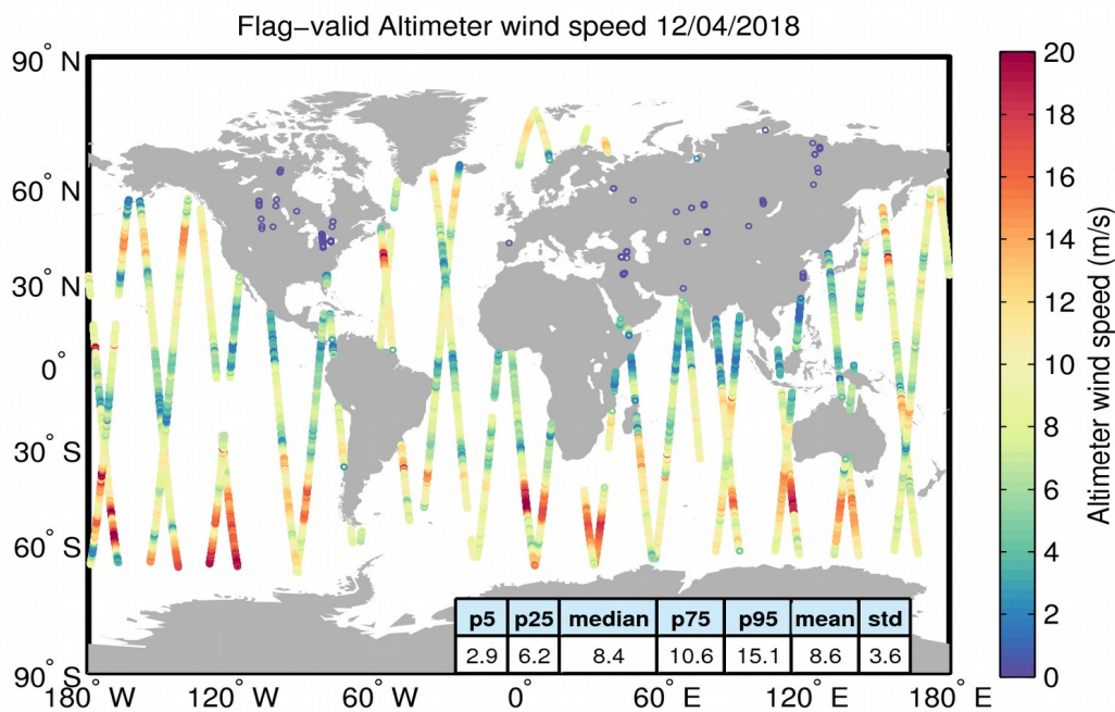
Figure 31. Geographical distribution of flag-valid wind data over oceans and lakes for 12/04/2018. The statistical values shown in the table refer to the wind in m/s and are calculated over all measurements shown in the figure.
