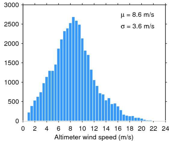
Figure 33. Histogram of flag-valid wind over oceans and lakes for 12/04/2018. The mean ( \mu ) and standard deviation ( \sigma ) are also shown. Note that values larger than 24 m/s are excluded from the histogram for the sake of readability but not from the computation of \mu and \sigma .
