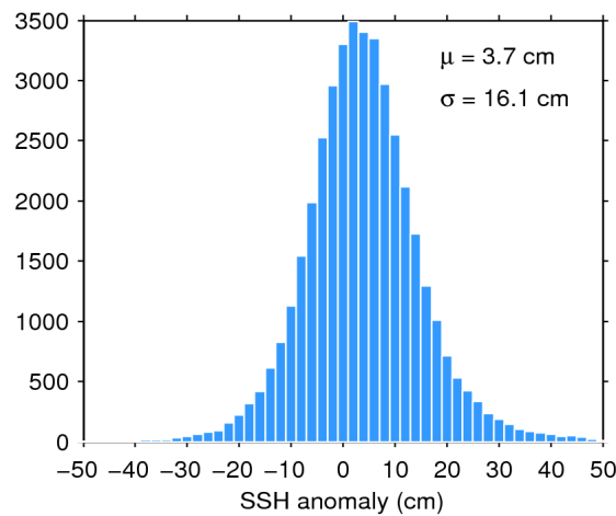
Figure 7. Histogram of flag-valid SSH anomaly over oceans and lakes for 12/04/2018. The mean ( \mu ) and standard deviation ( \sigma ) are also shown. Note that values outside [-50 50] cm are excluded from the histogram for the sake of readability but not from the computation of \mu and \sigma .
