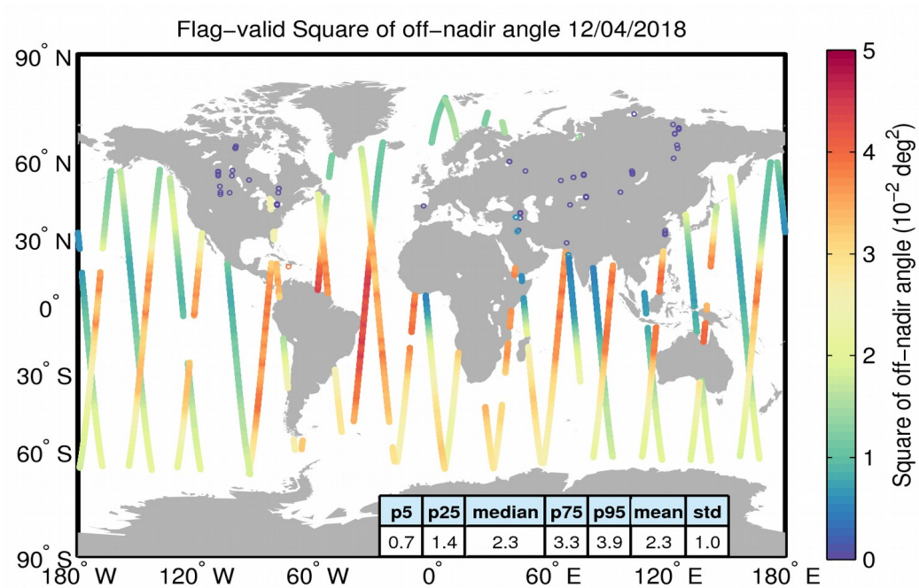
Figure 37. Geographical distribution of flag-valid mispointing data over oceans and lakes for 12/04/2018. The statistical values shown in the table refer to the mispointing in 10^{-2} deg 2 and are calculated over all measurements shown in the figure.
