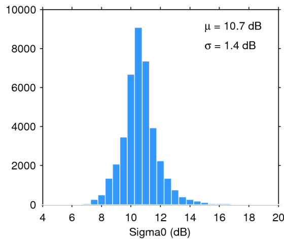
Figure 28. Histogram of science-valid sigma0 over oceans and lakes for 12/04/2018. The mean ( \mu ) and standard deviation ( \sigma ) are also shown. Note that values outside [4 20] dB are excluded from the histogram for the sake of readability but not from the computation of \mu and \sigma .
