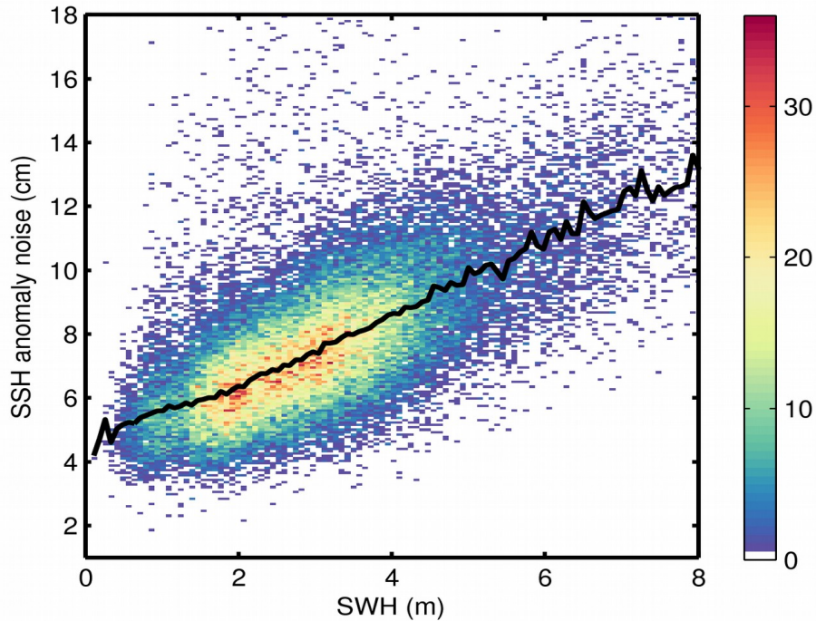
Figure 9. 2D histogram showing flag-valid SSH anomaly noise as a function of SWH for 12/04/2018. The black line denotes the median SSH anomaly noise as a function of SWH.
