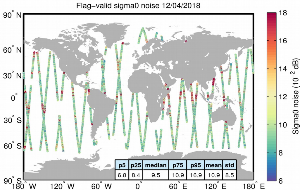
Figure 26. Geographical distribution of flag-valid 20-Hz sigma0 measurement noise over oceans and lakes for 12/04/2018. The statistical values shown in the table refer to the sigma0 noise and are calculated over all measurements shown in the figure.
