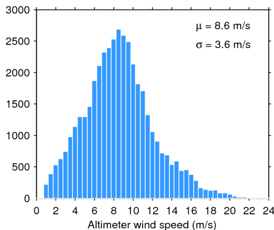
Figure 35. Histogram of science-valid wind over oceans and lakes for 12/04/2018. The mean ( \mu ) and standard deviation ( \sigma ) are also shown. Note that values larger than 24 m/s are excluded from the histogram for the sake of readability but not from the computation of \mu and \sigma .
