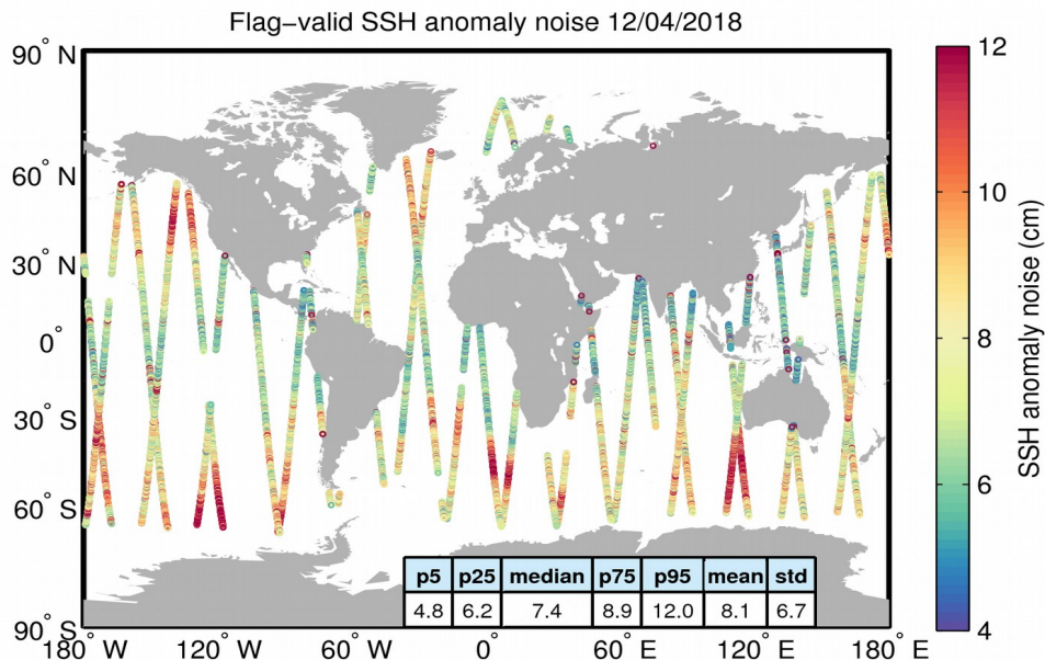
Figure 8. Geographical distribution of flag-valid 20-Hz SSH anomaly measurement noise over oceans and lakes for 12/04/2018. The statistical values shown in the table refer to the SSH anomaly noise and are calculated over all measurements shown in the figure.
