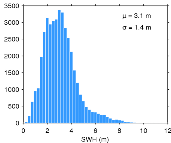
Figure 17. Histogram of flag-valid SWH over oceans and lakes for 12/04/2018. The mean ( \mu ) and standard deviation ( \sigma ) are also shown. Note that values larger than 12 m are excluded from the histogram for the sake of readability but not from the computation of \mu and \sigma .
