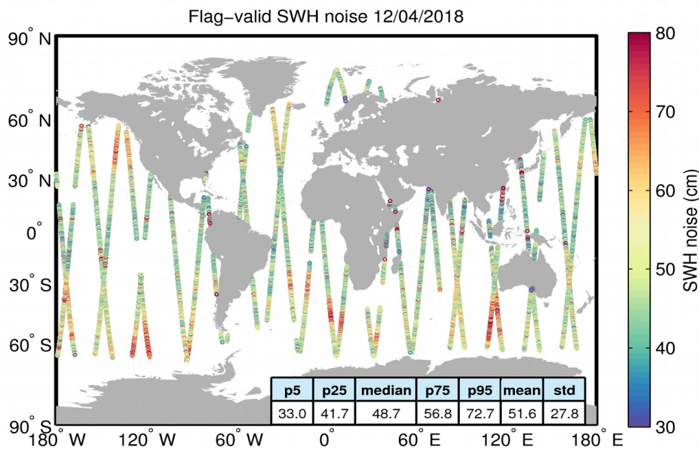
Figure 18. Geographical distribution of flag-valid 20-Hz SWH measurement noise over oceans and lakes for 12/04/2018. The statistical values shown in the table refer to the SWH noise and are calculated over all measurements shown in the figure.
