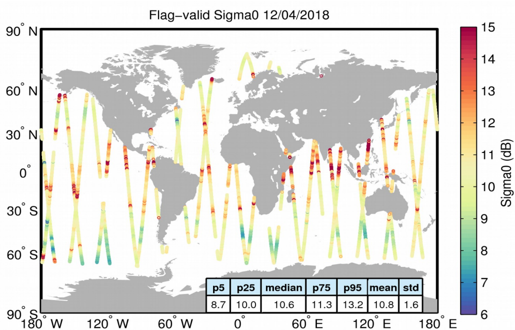
Figure 23. Geographical distribution of flag-valid sigma0 data over oceans and lakes for 12/04/2018. The statistical values shown in the table refer to the sigma0 in dB and are calculated over all measurements shown in the figure.
