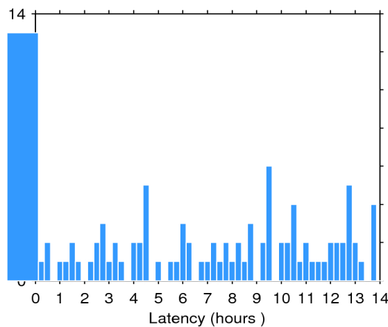
Figure 2. Histogram of the data latency for 12/04/2018. The y-axis denotes the number of files that are made available with a delay of x-hours with respect to the mean time of the records stored in the file.
