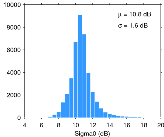
Figure 25. Histogram of flag-valid sigma0 over oceans and lakes for 12/04/2018. The mean ( \mu ) and standard deviation ( \sigma ) are also shown. Note that values outside [4 20] dB are excluded from the histogram for the sake of readability but not from the computation of \mu and \sigma .
