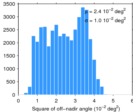
Figure 39. Histogram of flag-valid mispointing over oceans and lakes for 11/04/2018. The mean ( \mu ) and standard deviation ( \sigma ) are also shown. Note that values larger than 6 \cdot 10^{-2} \text{ deg}^2 are excluded from the histogram for the sake of readability but not from the computation of \mu and \sigma .
