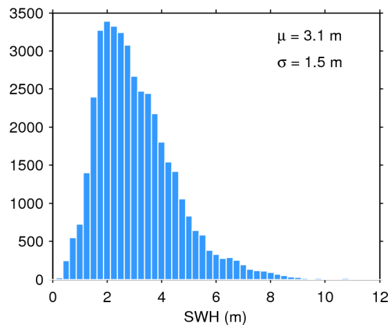
Figure 20. Histogram of science-valid SWH over oceans and lakes for 11/04/2018. The mean ( \mu ) and standard deviation ( \sigma ) are also shown. Note that values larger than 12 m are excluded from the histogram for the sake of readability but not from the computation of \mu and \sigma .
