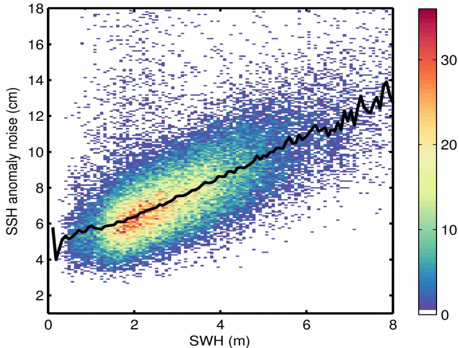
Figure 9. 2D histogram showing flag-valid SSH anomaly noise as a function of SWH for 11/04/2018. The black line denotes the median SSH anomaly noise as a function of SWH.
