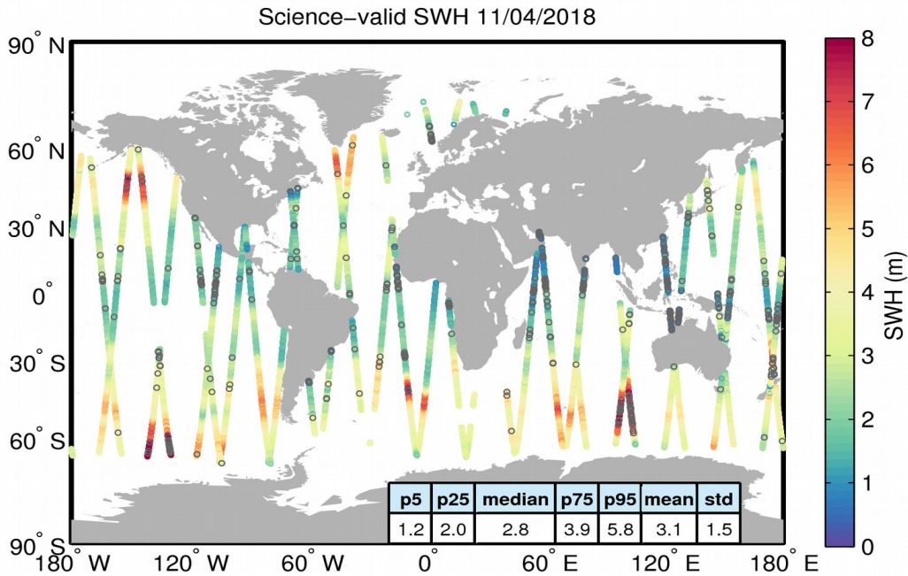
Figure 19. Geographical distribution of science-valid SWH data over oceans and lakes for 11/04/2018. The statistical values shown in the table refer to the SWH in m and are calculated over all measurements shown in the figure. Gray circles denote records that have been rejected based on the editing criteria described in Table 3.
