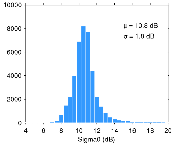
Figure 25. Histogram of flag-valid sigma0 over oceans and lakes for 11/04/2018. The mean ( \mu ) and standard deviation ( \sigma ) are also shown. Note that values outside [4 20] dB are excluded from the histogram for the sake of readability but not from the computation of \mu and \sigma .
