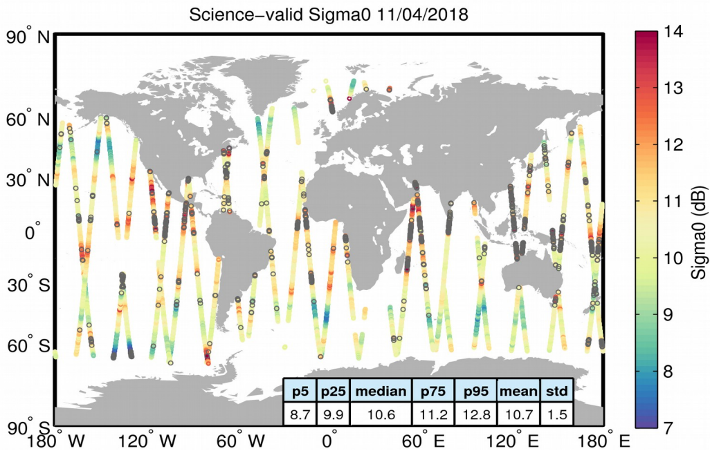
Figure 27. Geographical distribution of science-valid sigma0 data over oceans and lakes for 11/04/2018. The statistical values shown in the table refer to the sigma0 in dB and are calculated over all measurements shown in the figure. Gray circles denote records that have been rejected based on the editing criteria described in Table 4.
