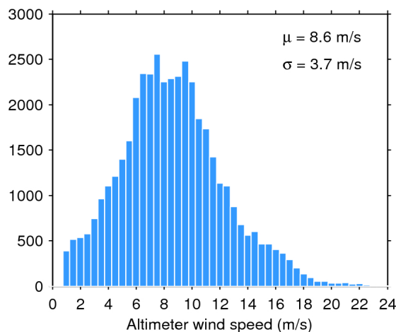
Figure 35. Histogram of science-valid wind over oceans and lakes for 11/04/2018. The mean ( \mu ) and standard deviation ( \sigma ) are also shown. Note that values larger than 24 m/s are excluded from the histogram for the sake of readability but not from the computation of \mu and \sigma .
