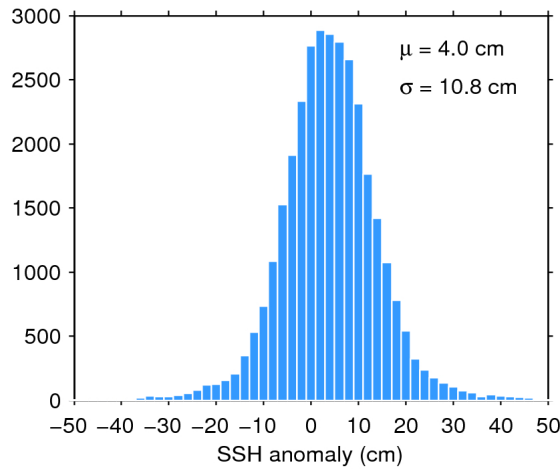
Figure 11. Histogram of science-valid SSH anomaly over oceans and lakes for 11/04/2018. The mean ( \mu ) and standard deviation ( \sigma ) are also shown. Note that values outside [-50 50] cm are excluded from the histogram for the sake of readability but not from the computation of \mu and \sigma .
