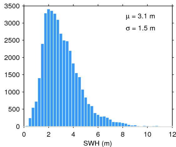
Figure 17. Histogram of flag-valid SWH over oceans and lakes for 11/04/2018. The mean ( \mu ) and standard deviation ( \sigma ) are also shown. Note that values larger than 12 m are excluded from the histogram for the sake of readability but not from the computation of \mu and \sigma .
