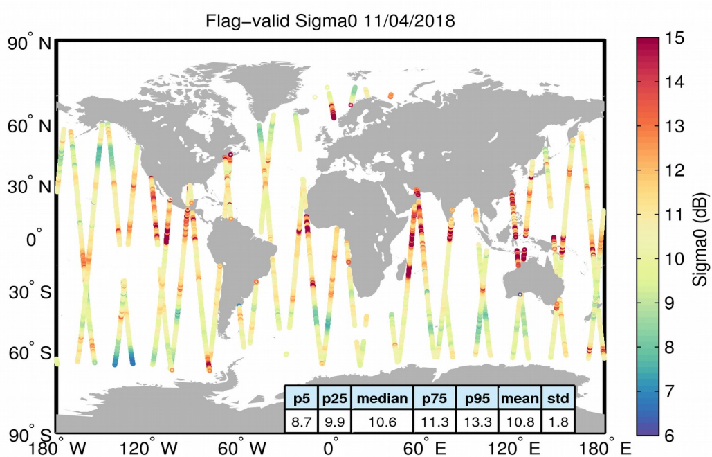
Figure 23. Geographical distribution of flag-valid sigma0 data over oceans and lakes for 11/04/2018. The statistical values shown in the table refer to the sigma0 in dB and are calculated over all measurements shown in the figure.
