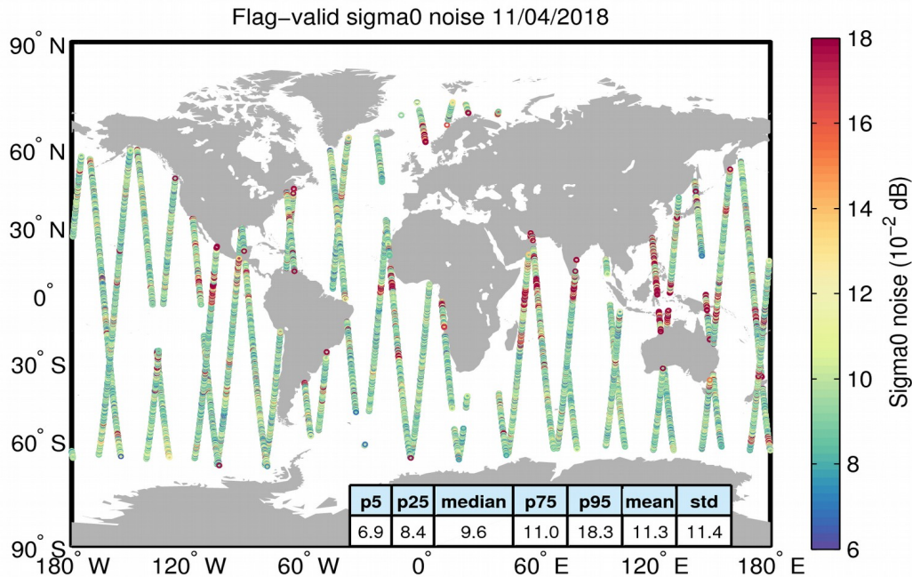
Figure 26. Geographical distribution of flag-valid 20-Hz sigma0 measurement noise over oceans and lakes for 11/04/2018. The statistical values shown in the table refer to the sigma0 noise and are calculated over all measurements shown in the figure.
