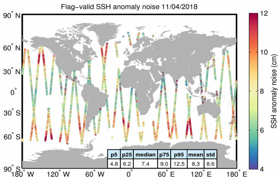
Figure 8. Geographical distribution of flag-valid 20-Hz SSH anomaly measurement noise over oceans and lakes for 11/04/2018. The statistical values shown in the table refer to the SSH anomaly noise and are calculated over all measurements shown in the figure.
