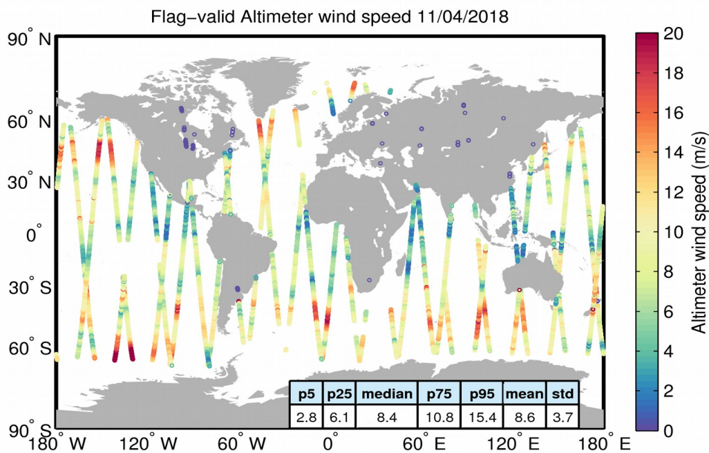
Figure 31. Geographical distribution of flag-valid wind data over oceans and lakes for 11/04/2018. The statistical values shown in the table refer to the wind in m/s and are calculated over all measurements shown in the figure.
