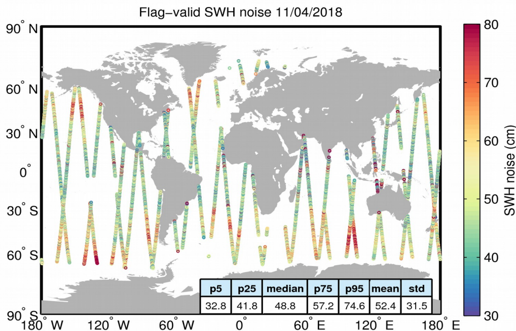
Figure 18. Geographical distribution of flag-valid 20-Hz SWH measurement noise over oceans and lakes for 11/04/2018. The statistical values shown in the figure refer to the SWH noise and are calculated over all measurements shown in the figure.
