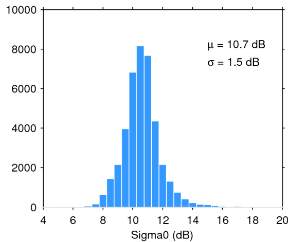
Figure 28. Histogram of science-valid sigma0 over oceans and lakes for 11/04/2018. The mean ( \mu ) and standard deviation ( \sigma ) are also shown. Note that values outside [4 20] dB are excluded from the histogram for the sake of readability but not from the computation of \mu and \sigma .
