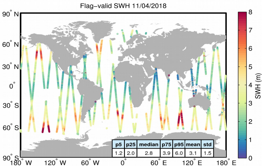
Figure 15. Geographical distribution of flag-valid SWH data over oceans and lakes for 11/04/2018. The statistical values shown in the table refer to the SWH in m and are calculated over all measurements shown in the figure.
