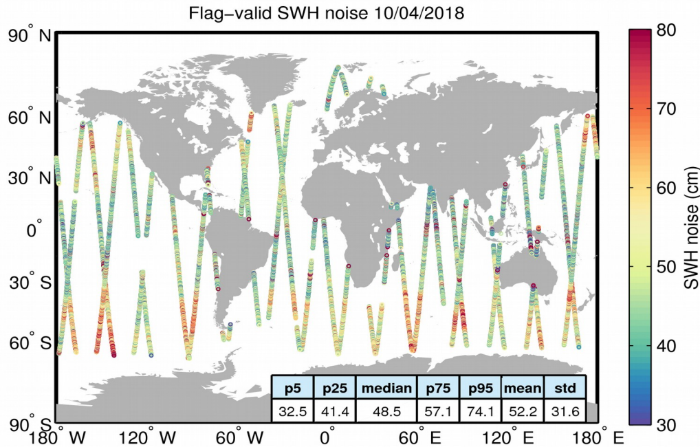
Figure 18. Geographical distribution of flag-valid 20-Hz SWH measurement noise over oceans and lakes for 10/04/2018. The statistical values shown in the table refer to the SWH noise and are calculated over all measurements shown in the figure.
