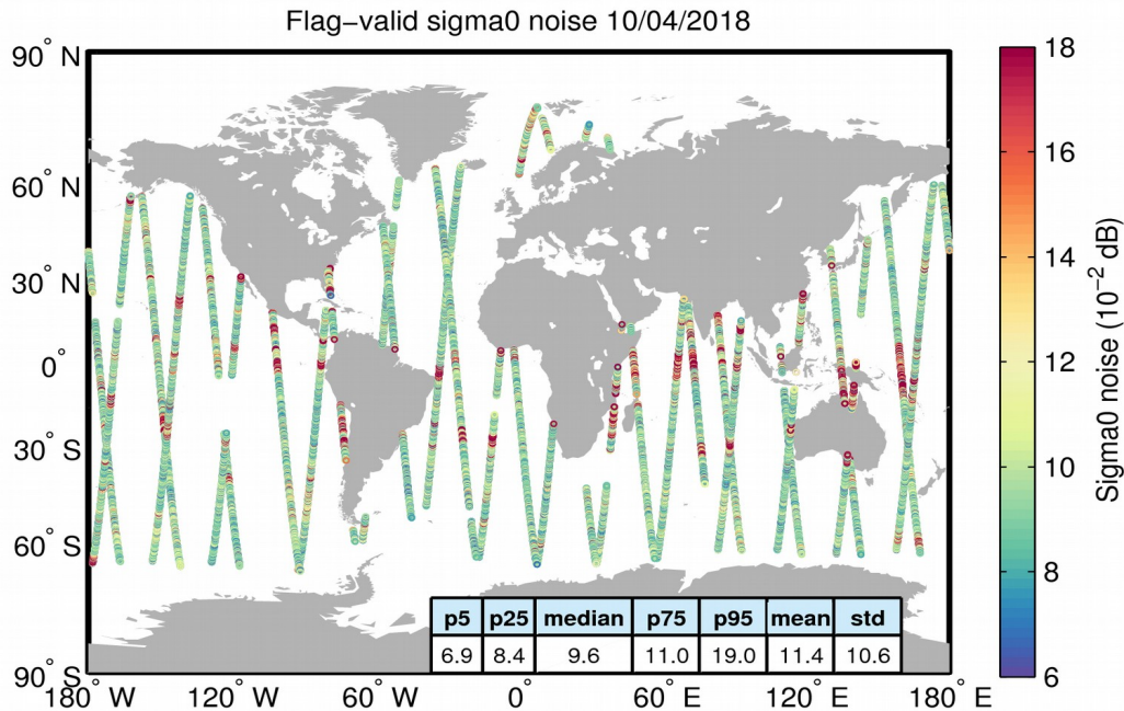
Figure 26. Geographical distribution of flag-valid 20-Hz sigma0 measurement noise over oceans and lakes for 10/04/2018. The statistical values shown in the table refer to the sigma0 noise and are calculated over all measurements shown in the figure.
