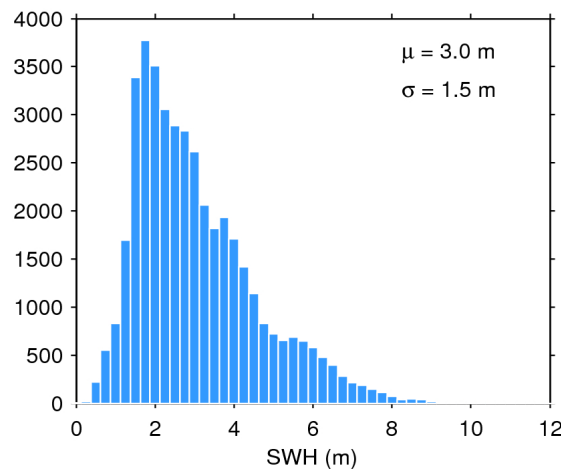
Figure 17. Histogram of flag-valid SWH over oceans and lakes for 10/04/2018. The mean ( \mu ) and standard deviation ( \sigma ) are also shown. Note that values larger than 12 m are excluded from the histogram for the sake of readability but not from the computation of \mu and \sigma .
