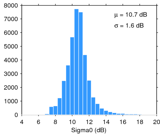
Figure 28. Histogram of science-valid sigma0 over oceans and lakes for 10/04/2018. The mean ( \mu ) and standard deviation ( \sigma ) are also shown. Note that values outside [4 20] dB are excluded from the histogram for the sake of readability but not from the computation of \mu and \sigma .
