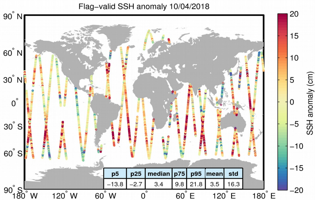
Figure 5. Geographical distribution of flag-valid 1-Hz SSH anomaly data over oceans and lakes for 10/04/2018. The statistical values shown in the table refer to the SSH anomaly in cm and are calculated over all measurements shown in the figure.
