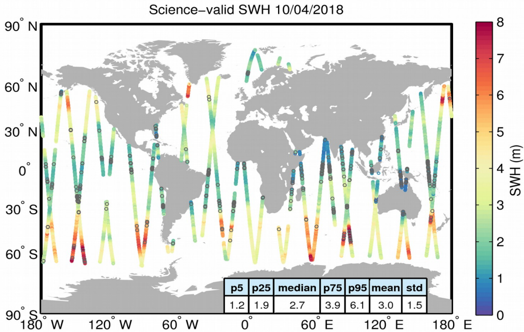
Figure 19. Geographical distribution of science-valid SWH data over oceans and lakes for 10/04/2018. The statistical values shown in the table refer to the SWH in m and are calculated over all measurements shown in the figure. Gray circles denote records that have been rejected based on the editing criteria described in Table 3.
