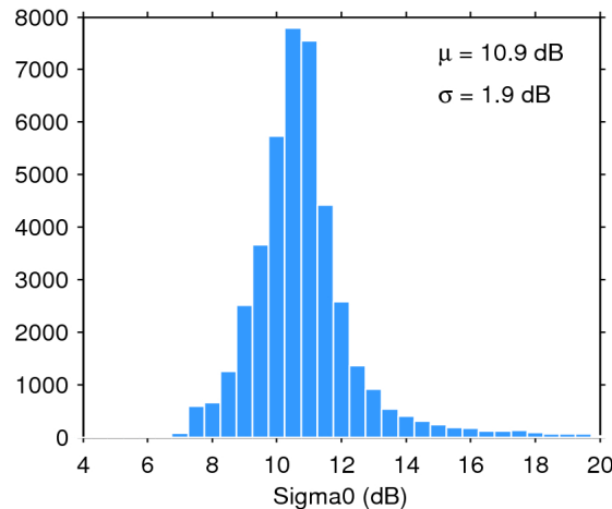
Figure 25. Histogram of flag-valid sigma0 over oceans and lakes for 10/04/2018. The mean ( \mu ) and standard deviation ( \sigma ) are also shown. Note that values outside [4 20] dB are excluded from the histogram for the sake of readability but not from the computation of \mu and \sigma .
