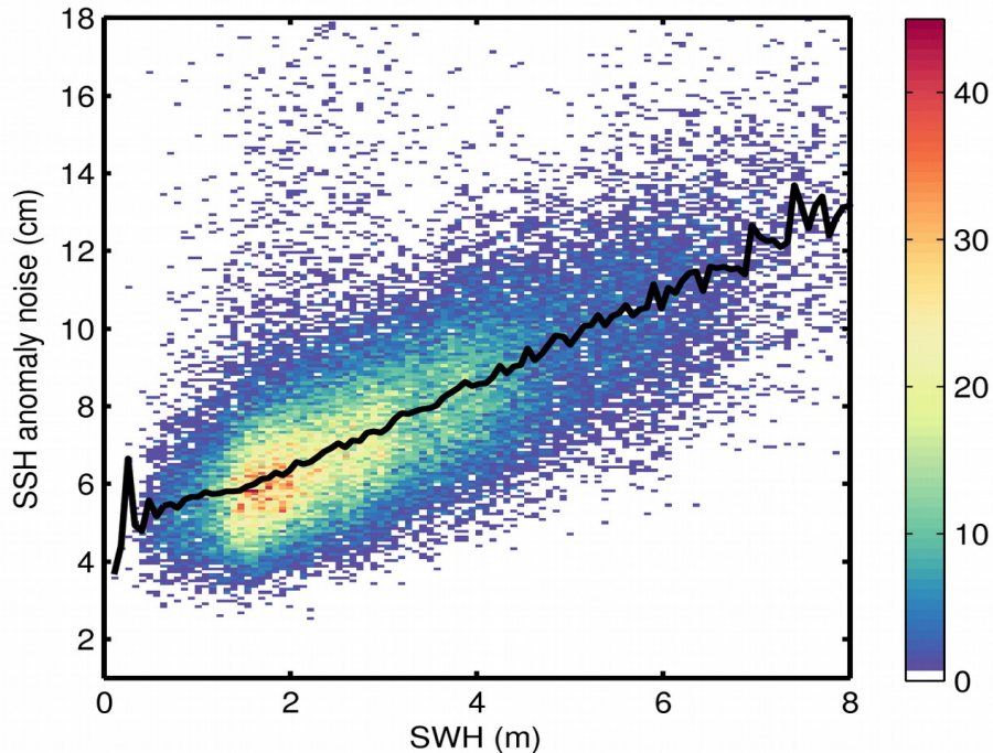
Figure 9. 2D histogram showing flag-valid SSH anomaly noise as a function of SWH for 10/04/2018. The black line denotes the median SSH anomaly noise as a function of SWH.
