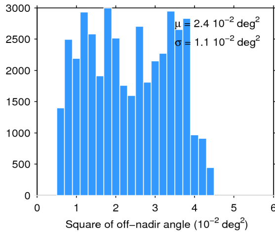
Figure 39. Histogram of flag-valid mispointing over oceans and lakes for 10/04/2018. The mean ( \mu ) and standard deviation ( \sigma ) are also shown. Note that values larger than 6 \cdot 10^{-2} \text{ deg}^2 are excluded from the histogram for the sake of readability but not from the computation of \mu and \sigma .
