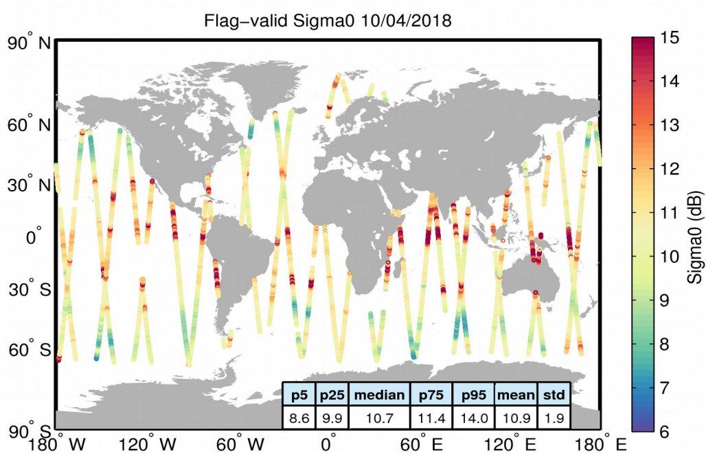
Figure 23. Geographical distribution of flag-valid sigma0 data over oceans and lakes for 10/04/2018. The statistical values shown in the table refer to the sigma0 in dB and are calculated over all measurements shown in the figure.
