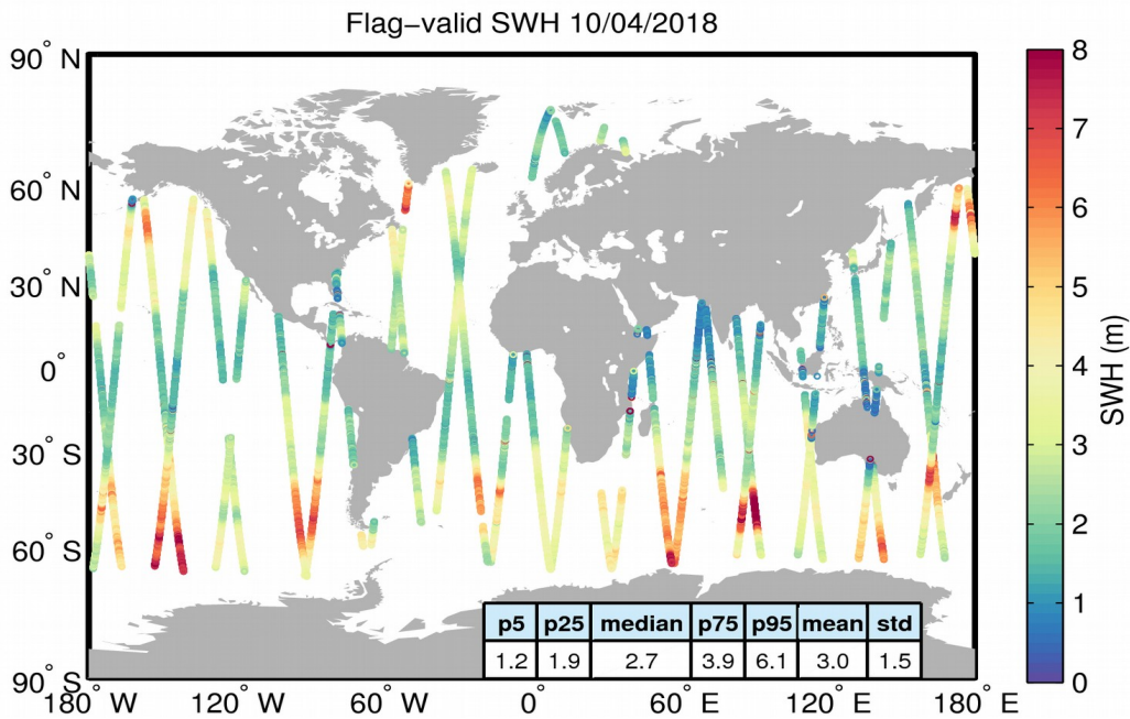
Figure 15. Geographical distribution of flag-valid SWH data over oceans and lakes for 10/04/2018. The statistical values shown in the table refer to the SWH in m and are calculated over all measurements shown in the figure.
