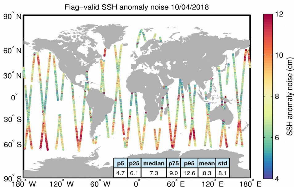
Figure 8. Geographical distribution of flag-valid 20-Hz SSH anomaly measurement noise over oceans and lakes for 10/04/2018. The statistical values shown in the table refer to the SSH anomaly noise and are calculated over all measurements shown in the figure.
