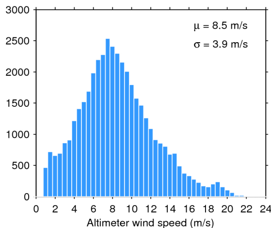
Figure 35. Histogram of science-valid wind over oceans and lakes for 10/04/2018. The mean ( \mu ) and standard deviation ( \sigma ) are also shown. Note that values larger than 24 m/s are excluded from the histogram for the sake of readability but not from the computation of \mu and \sigma .
