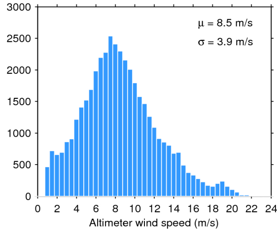
Figure 33. Histogram of flag-valid wind over oceans and lakes for 10/04/2018. The mean ( \mu ) and standard deviation ( \sigma ) are also shown. Note that values larger than 24 m/s are excluded from the histogram for the sake of readability but not from the computation of \mu and \sigma .
