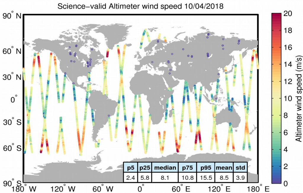
Figure 34. Geographical distribution of science-valid wind data over oceans and lakes for 10/04/2018. The statistical values shown in the table refer to the wind in m/s and are calculated over all measurements shown in the figure. Gray circles denote records that have been rejected based on the editing criteria described in Table 5.
