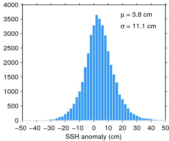
Figure 11. Histogram of science-valid SSH anomaly over oceans and lakes for 10/04/2018. The mean ( \mu ) and standard deviation ( \sigma ) are also shown. Note that values outside [-50 50] cm are excluded from the histogram for the sake of readability but not from the computation of \mu and \sigma .
