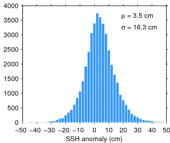
Figure 7. Histogram of flag-valid SSH anomaly over oceans and lakes for 10/04/2018. The mean ( \mu ) and standard deviation ( \sigma ) are also shown. Note that values outside [-50 50] cm are excluded from the histogram for the sake of readability but not from the computation of \mu and \sigma .
