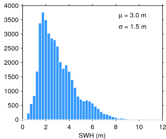
Figure 20. Histogram of science-valid SWH over oceans and lakes for 10/04/2018. The mean ( \mu ) and standard deviation ( \sigma ) are also shown. Note that values larger than 12 m are excluded from the histogram for the sake of readability but not from the computation of \mu and \sigma .
