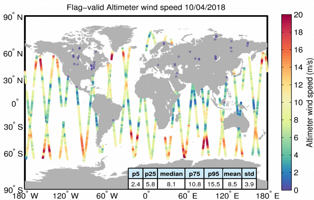
Figure 31. Geographical distribution of flag-valid wind data over oceans and lakes for 10/04/2018. The statistical values shown in the table refer to the wind in m/s and are calculated over all measurements shown in the figure.
