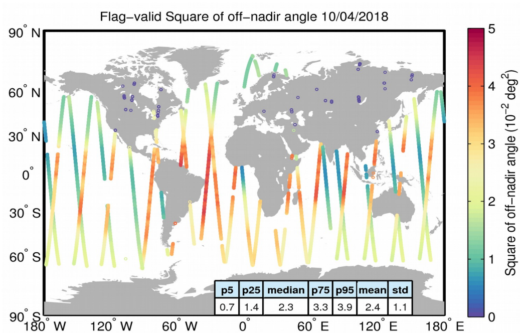
Figure 37. Geographical distribution of flag-valid mispointing data over oceans and lakes for 10/04/2018. The statistical values shown in the table refer to the mispointing in 10^{-2} deg 2 and are calculated over all measurements shown in the figure.
