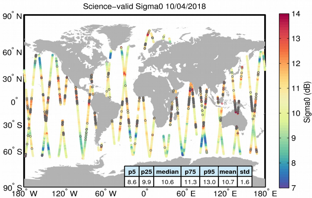
Figure 27. Geographical distribution of science-valid sigma0 data over oceans and lakes for 10/04/2018. The statistical values shown in the table refer to the sigma0 in dB and are calculated over all measurements shown in the figure. Gray circles denote records that have been rejected based on the editing criteria described in Table 4.
