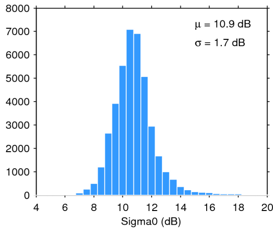
Figure 28. Histogram of science-valid sigma0 over oceans and lakes for 09/04/2018. The mean ( \mu ) and standard deviation ( \sigma ) are also shown. Note that values outside [4 20] dB are excluded from the histogram for the sake of readability but not from the computation of \mu and \sigma .
