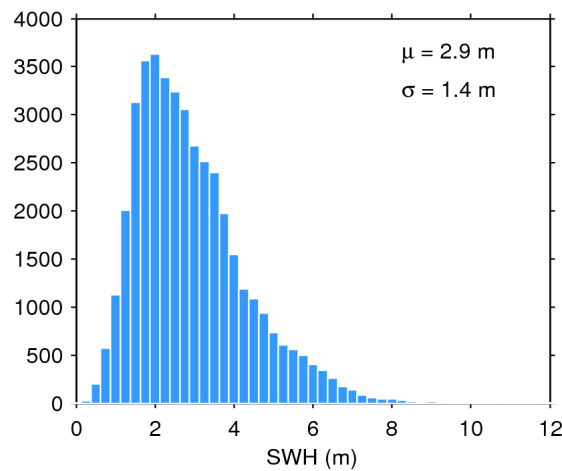
Figure 17. Histogram of flag-valid SWH over oceans and lakes for 09/04/2018. The mean ( \mu ) and standard deviation ( \sigma ) are also shown. Note that values larger than 12 m are excluded from the histogram for the sake of readability but not from the computation of \mu and \sigma .
