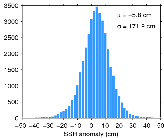
Figure 7. Histogram of flag-valid SSH anomaly over oceans and lakes for 09/04/2018. The mean ( \mu ) and standard deviation ( \sigma ) are also shown. Note that values outside [-50 50] cm are excluded from the histogram for the sake of readability but not from the computation of \mu and \sigma .
