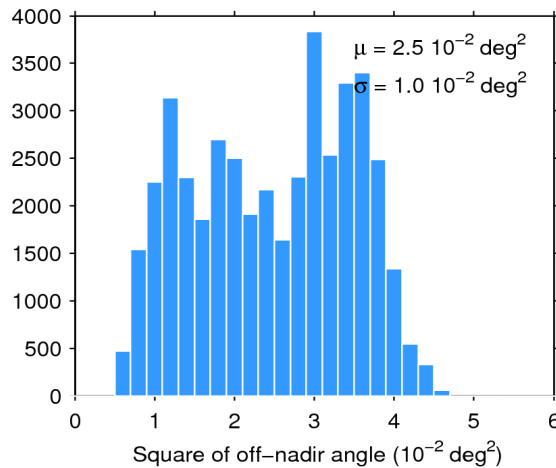
Figure 39. Histogram of flag-valid mispointing over oceans and lakes for 09/04/2018. The mean ( \mu ) and standard deviation ( \sigma ) are also shown. Note that values larger than 6 \cdot 10^{-2} \text{ deg}^2 are excluded from the histogram for the sake of readability but not from the computation of \mu and \sigma .
