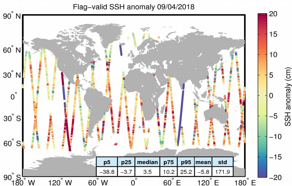
Figure 5. Geographical distribution of flag-valid 1-Hz SSH anomaly data over oceans and lakes for 09/04/2018. The statistical values shown in the table refer to the SSH anomaly in cm and are calculated over all measurements shown in the figure.
