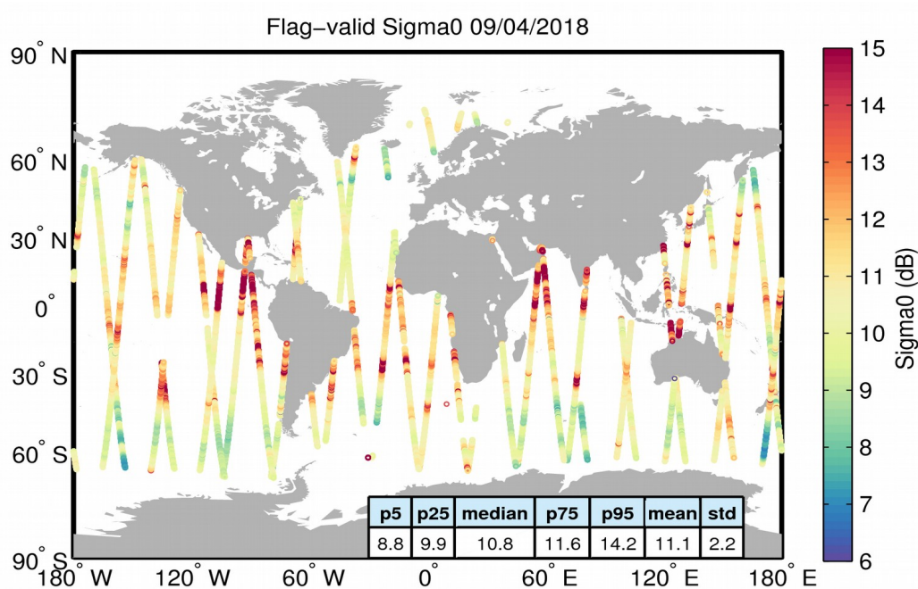
Figure 23. Geographical distribution of flag-valid sigma0 data over oceans and lakes for 09/04/2018. The statistical values shown in the table refer to the sigma0 in dB and are calculated over all measurements shown in the figure.
