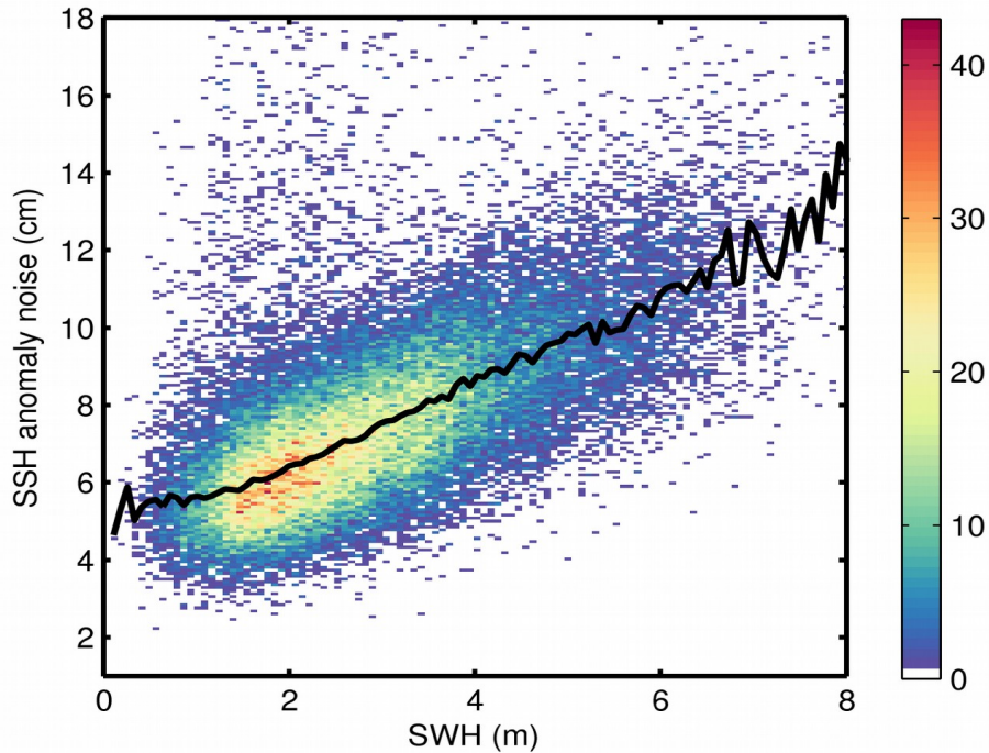
Figure 9. 2D histogram showing flag-valid SSH anomaly noise as a function of SWH for 09/04/2018. The black line denotes the median SSH anomaly noise as a function of SWH.
