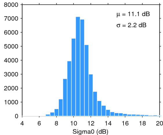
Figure 25. Histogram of flag-valid sigma0 over oceans and lakes for 09/04/2018. The mean ( \mu ) and standard deviation ( \sigma ) are also shown. Note that values outside [4 20] dB are excluded from the histogram for the sake of readability but not from the computation of \mu and \sigma .
