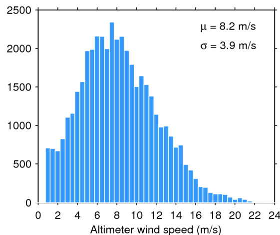
Figure 35. Histogram of science-valid wind over oceans and lakes for 09/04/2018. The mean ( \mu ) and standard deviation ( \sigma ) are also shown. Note that values larger than 24 m/s are excluded from the histogram for the sake of readability but not from the computation of \mu and \sigma .
