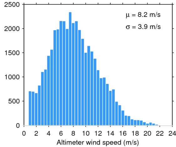
Figure 33. Histogram of flag-valid wind over oceans and lakes for 09/04/2018. The mean ( \mu ) and standard deviation ( \sigma ) are also shown. Note that values larger than 24 m/s are excluded from the histogram for the sake of readability but not from the computation of \mu and \sigma .
