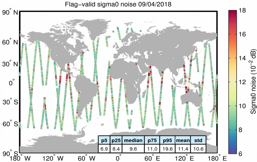
Figure 26. Geographical distribution of flag-valid 20-Hz sigma0 measurement noise over oceans and lakes for 09/04/2018. The statistical values shown in the table refer to the sigma0 noise and are calculated over all measurements shown in the figure.
