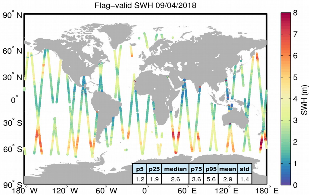
Figure 15. Geographical distribution of flag-valid SWH data over oceans and lakes for 09/04/2018. The statistical values shown in the table refer to the SWH in m and are calculated over all measurements shown in the figure.
