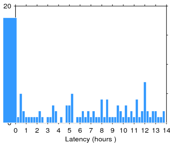
Figure 2. Histogram of the data latency for 09/04/2018. The y-axis denotes the number of files that are made available with a delay of x-hours with respect to the mean time of the records stored in the file.
