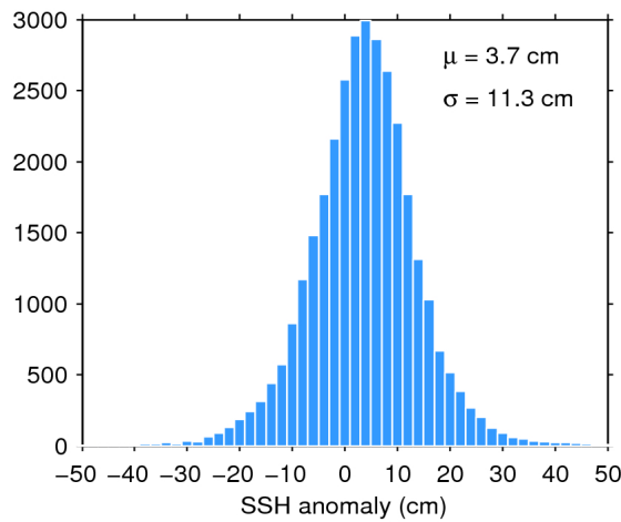
Figure 11. Histogram of science-valid SSH anomaly over oceans and lakes for 09/04/2018. The mean ( \mu ) and standard deviation ( \sigma ) are also shown. Note that values outside [-50 50] cm are excluded from the histogram for the sake of readability but not from the computation of \mu and \sigma .
