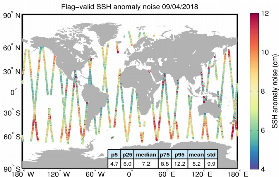
Figure 8. Geographical distribution of flag-valid 20-Hz SSH anomaly measurement noise over oceans and lakes for 09/04/2018. The statistical values shown in the table refer to the SSH anomaly noise and are calculated over all measurements shown in the figure.
