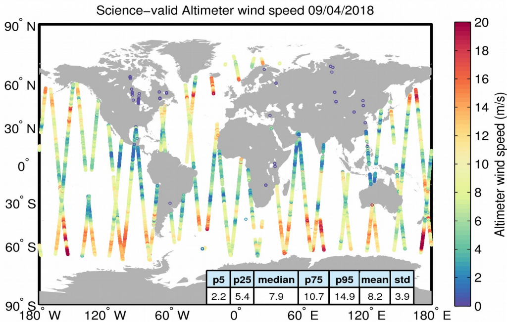
Figure 34. Geographical distribution of science-valid wind data over oceans and lakes for 09/04/2018. The statistical values shown in the table refer to the wind in m/s and are calculated over all measurements shown in the figure. Gray circles denote records that have been rejected based on the editing criteria described in Table 5.
