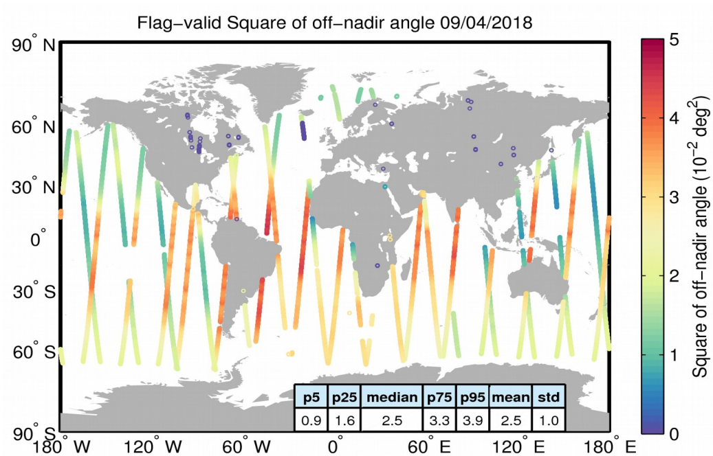
Figure 37. Geographical distribution of flag-valid mispointing data over oceans and lakes for 09/04/2018. The statistical values shown in the table refer to the mispointing in 10^{-2} \text{ deg}^2 and are calculated over all measurements shown in the figure.
