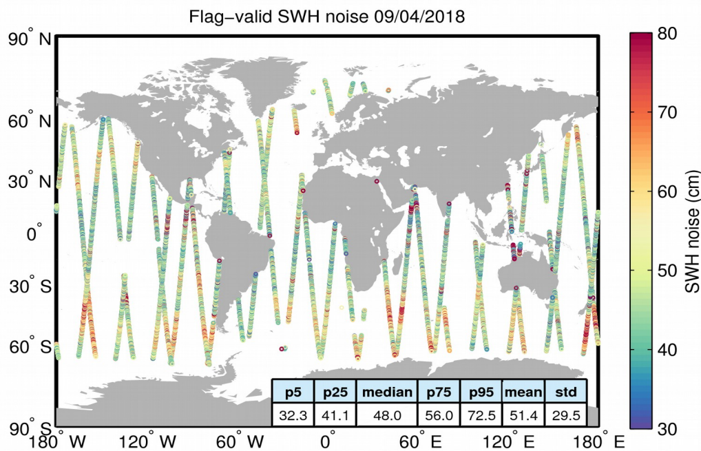
Figure 18. Geographical distribution of flag-valid 20-Hz SWH measurement noise over oceans and lakes for 09/04/2018. The statistical values shown in the table refer to the SWH noise and are calculated over all measurements shown in the figure.
