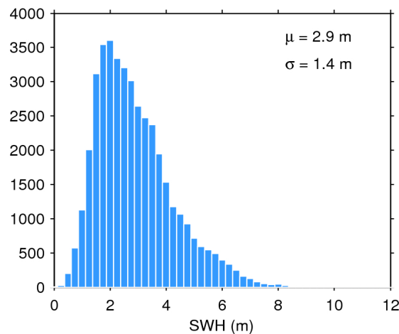
Figure 20. Histogram of science-valid SWH over oceans and lakes for 09/04/2018. The mean ( \mu ) and standard deviation ( \sigma ) are also shown. Note that values larger than 12 m are excluded from the histogram for the sake of readability but not from the computation of \mu and \sigma .
