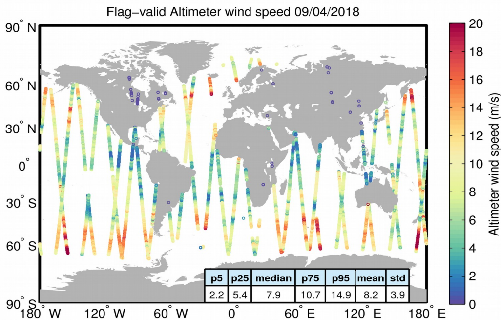
Figure 31. Geographical distribution of flag-valid wind data over oceans and lakes for 09/04/2018. The statistical values shown in the table refer to the wind in m/s and are calculated over all measurements shown in the figure.
