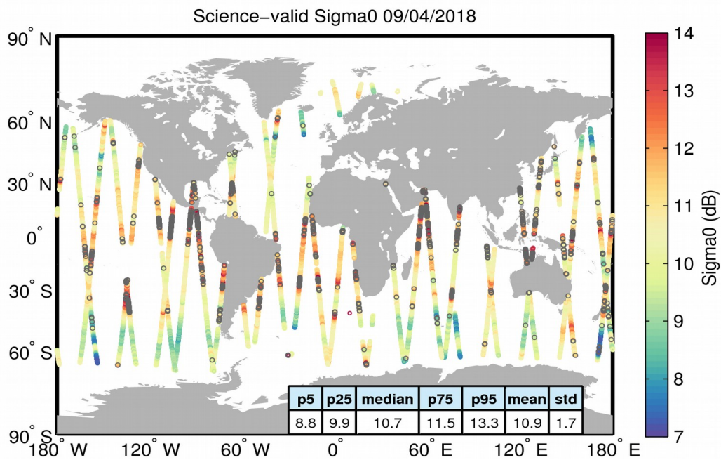
Figure 27. Geographical distribution of science-valid sigma0 data over oceans and lakes for 09/04/2018. The statistical values shown in the table refer to the sigma0 in dB and are calculated over all measurements shown in the figure. Gray circles denote records that have been rejected based on the editing criteria described in Table 4.
