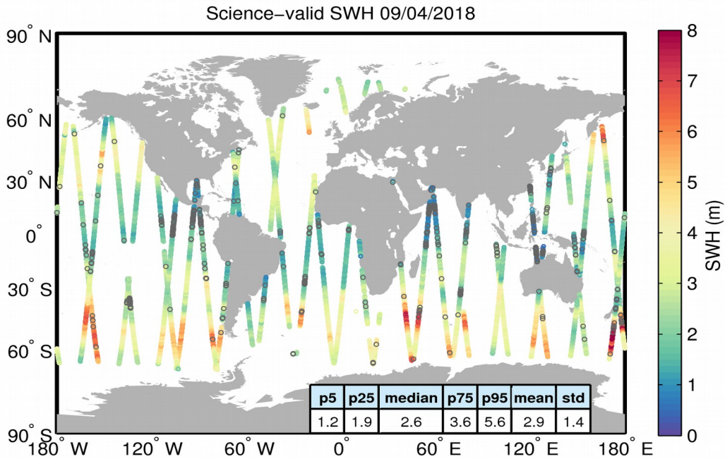
Figure 19. Geographical distribution of science-valid SWH data over oceans and lakes for 09/04/2018. The statistical values shown in the table refer to the SWH in m and are calculated over all measurements shown in the figure. Gray circles denote records that have been rejected based on the editing criteria described in Table 3.
