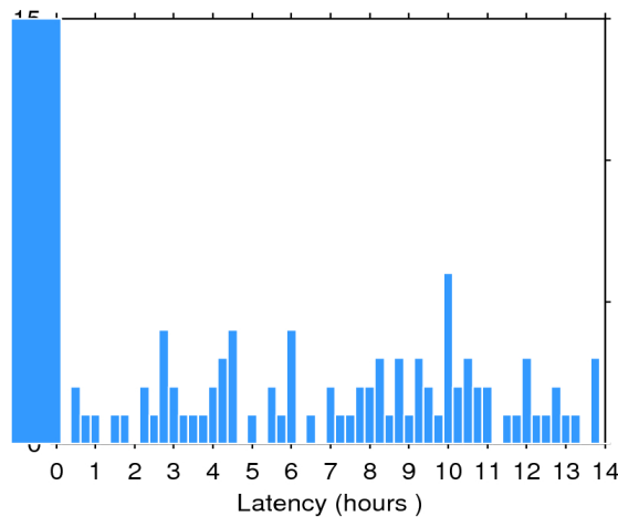
Figure 2. Histogram of the data latency for 08/04/2018. The y-axis denotes the number of files that are made available with a delay of x-hours with respect to the mean time of the records stored in the file.
