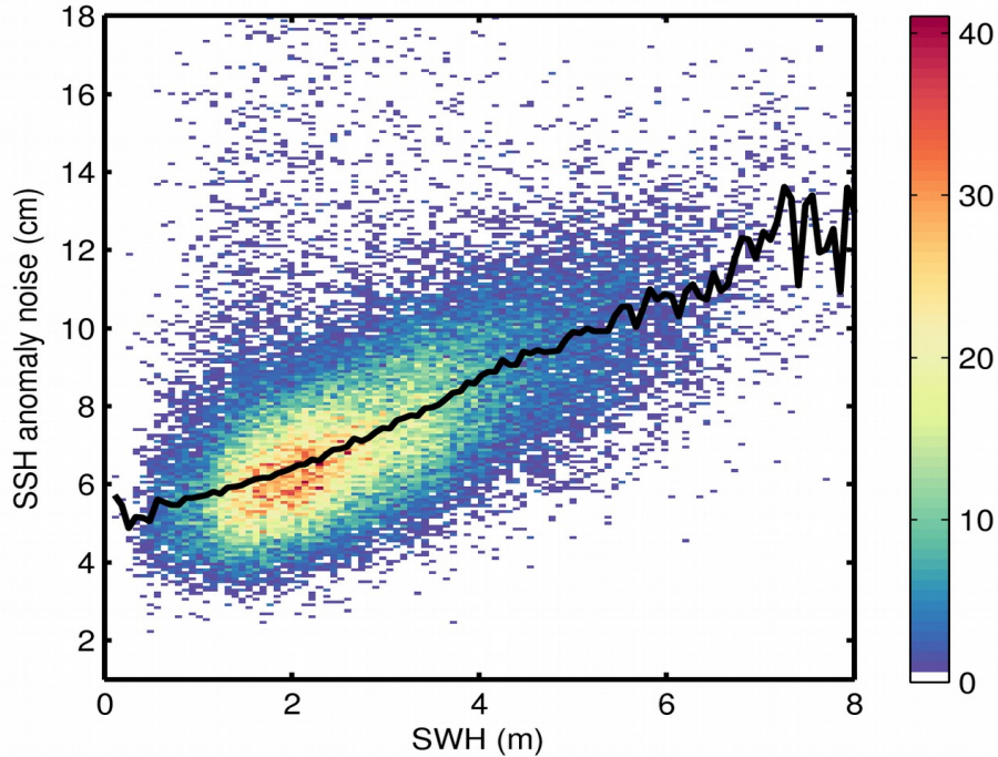
Figure 9. 2D histogram showing flag-valid SSH anomaly noise as a function of SWH for 08/04/2018. The black line denotes the median SSH anomaly noise as a function of SWH.
