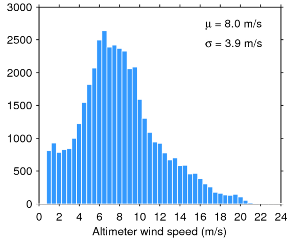
Figure 33. Histogram of flag-valid wind over oceans and lakes for 08/04/2018. The mean ( \mu ) and standard deviation ( \sigma ) are also shown. Note that values larger than 24 m/s are excluded from the histogram for the sake of readability but not from the computation of \mu and \sigma .
