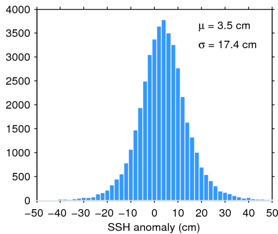
Figure 7. Histogram of flag-valid SSH anomaly over oceans and lakes for 08/04/2018. The mean ( \mu ) and standard deviation ( \sigma ) are also shown. Note that values outside [-50\ 50] cm are excluded from the histogram for the sake of readability but not from the computation of \mu and \sigma .
