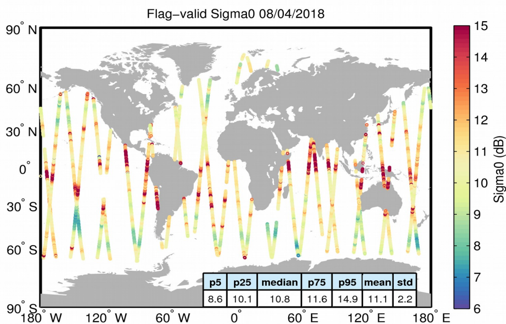
Figure 23. Geographical distribution of flag-valid sigma0 data over oceans and lakes for 08/04/2018. The statistical values shown in the table refer to the sigma0 in dB and are calculated over all measurements shown in the figure.
