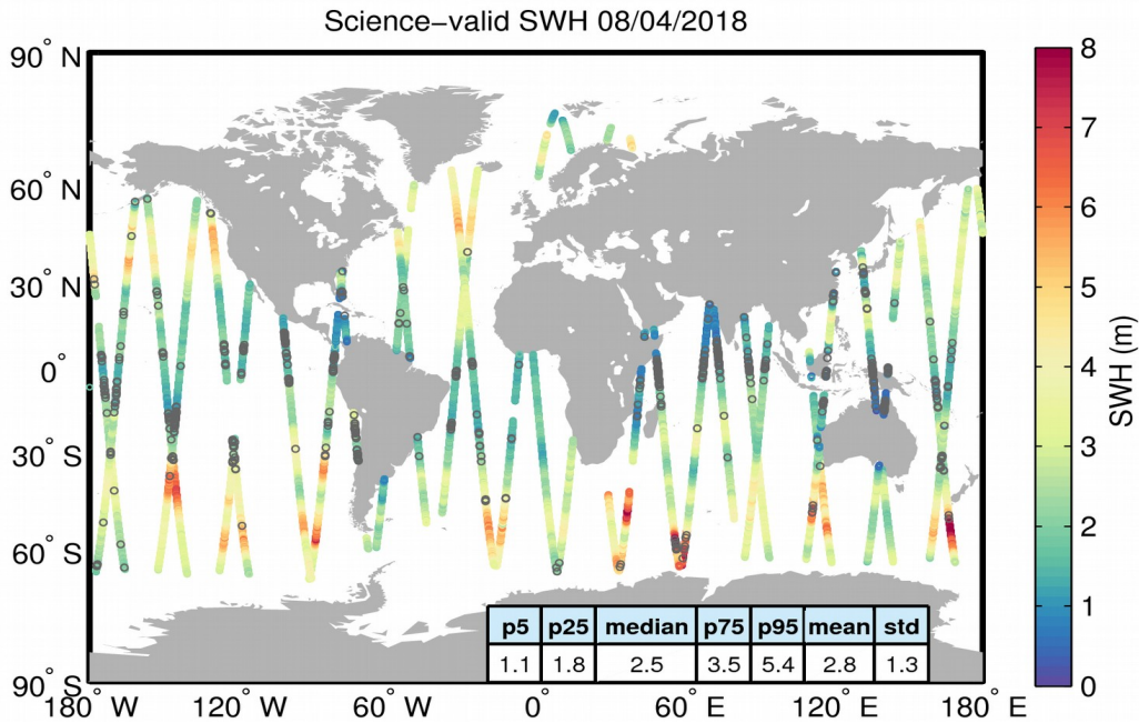
Figure 19. Geographical distribution of science-valid SWH data over oceans and lakes for 08/04/2018. The statistical values shown in the table refer to the SWH in m and are calculated over all measurements shown in the figure. Gray circles denote records that have been rejected based on the editing criteria described in Table 3.
