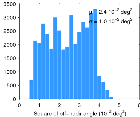
Figure 39. Histogram of flag-valid mispointing over oceans and lakes for 08/04/2018. The mean ( \mu ) and standard deviation ( \sigma ) are also shown. Note that values larger than 6 \cdot 10^{-2} \text{ deg}^2 are excluded from the histogram for the sake of readability but not from the computation of \mu and \sigma .
