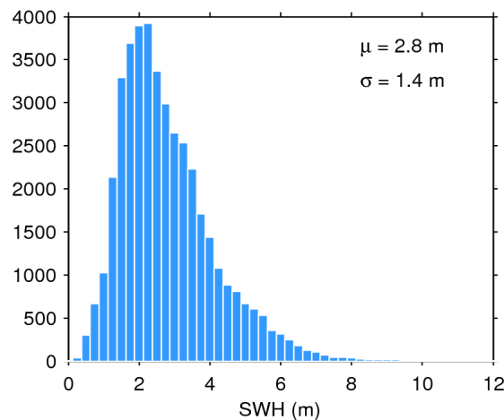
Figure 17. Histogram of flag-valid SWH over oceans and lakes for 08/04/2018. The mean ( \mu ) and standard deviation ( \sigma ) are also shown. Note that values larger than 12 m are excluded from the histogram for the sake of readability but not from the computation of \mu and \sigma .
