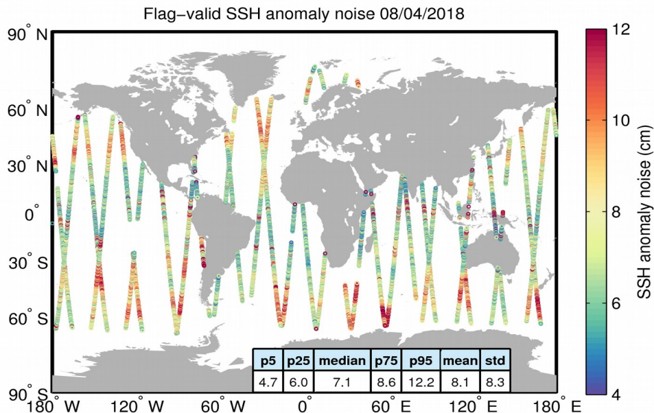
Figure 8. Geographical distribution of flag-valid 20-Hz SSH anomaly measurement noise over oceans and lakes for 08/04/2018. The statistical values shown in the table refer to the SSH anomaly noise and are calculated over all measurements shown in the figure.
