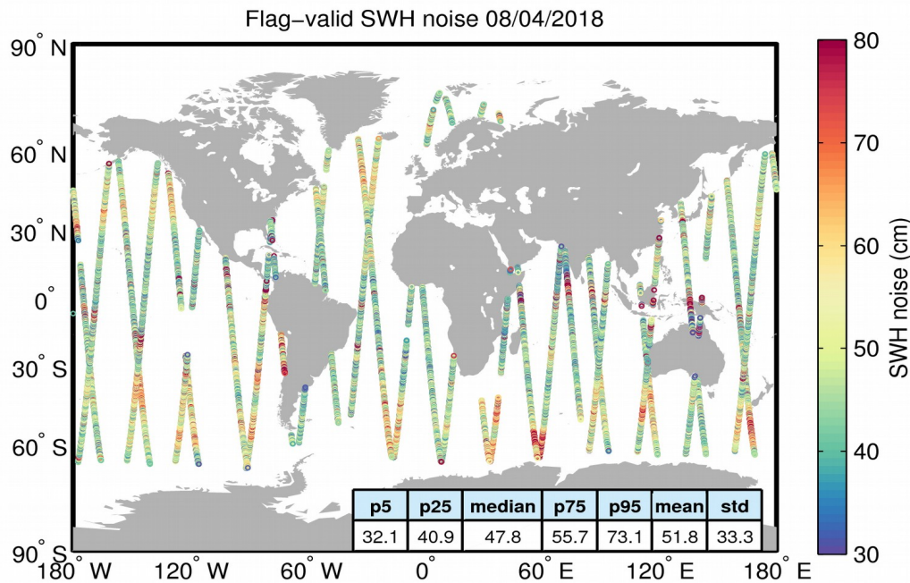
Figure 18. Geographical distribution of flag-valid 20-Hz SWH measurement noise over oceans and lakes for 08/04/2018. The statistical values shown in the figure refer to the SWH noise and are calculated over all measurements shown in the figure.
