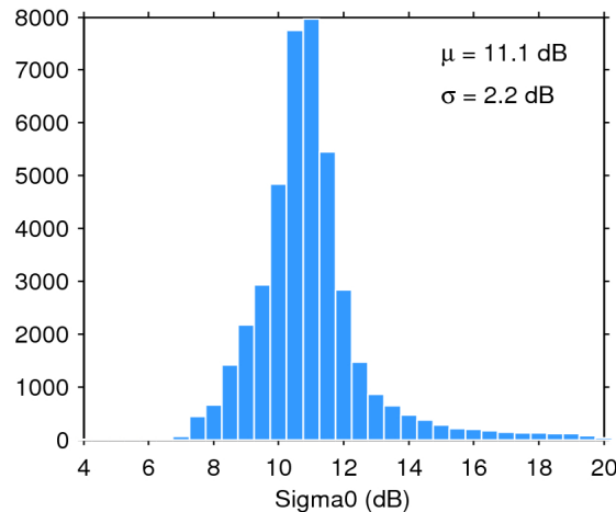
Figure 25. Histogram of flag-valid sigma0 over oceans and lakes for 08/04/2018. The mean ( \mu ) and standard deviation ( \sigma ) are also shown. Note that values outside [4 20] dB are excluded from the histogram for the sake of readability but not from the computation of \mu and \sigma .
