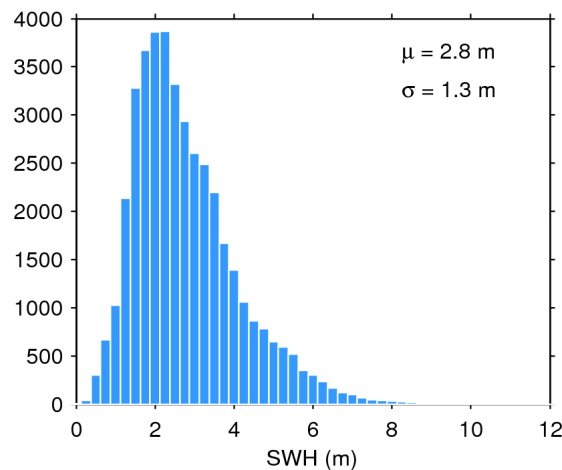
Figure 20. Histogram of science-valid SWH over oceans and lakes for 08/04/2018. The mean ( \mu ) and standard deviation ( \sigma ) are also shown. Note that values larger than 12 m are excluded from the histogram for the sake of readability but not from the computation of \mu and \sigma .
