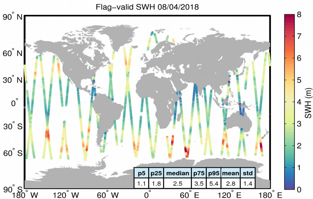
Figure 15. Geographical distribution of flag-valid SWH data over oceans and lakes for 08/04/2018. The statistical values shown in the table refer to the SWH in m and are calculated over all measurements shown in the figure.
