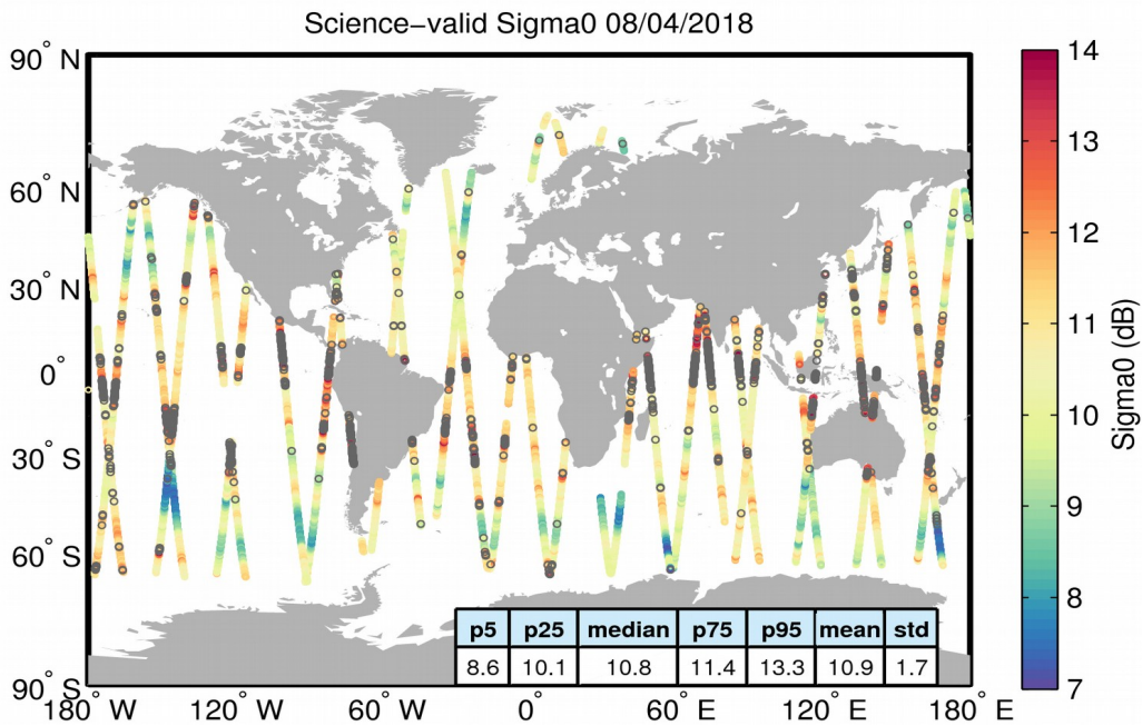
Figure 27. Geographical distribution of science-valid sigma0 data over oceans and lakes for 08/04/2018. The statistical values shown in the table refer to the sigma0 in dB and are calculated over all measurements shown in the figure. Gray circles denote records that have been rejected based on the editing criteria described in Table 4.
