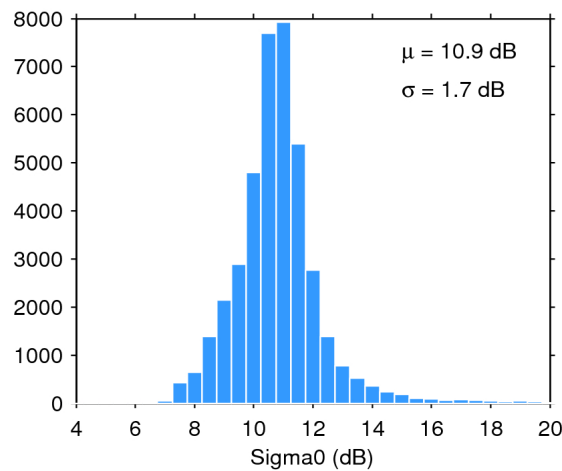
Figure 28. Histogram of science-valid sigma0 over oceans and lakes for 08/04/2018. The mean ( \mu ) and standard deviation ( \sigma ) are also shown. Note that values outside [4 20] dB are excluded from the histogram for the sake of readability but not from the computation of \mu and \sigma .
