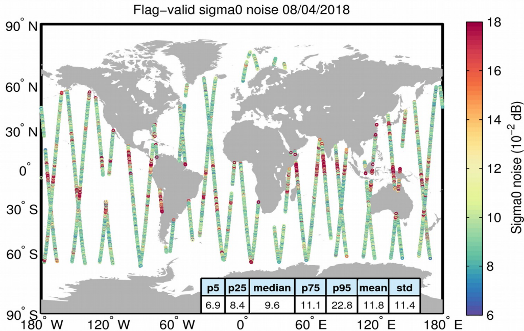
Figure 26. Geographical distribution of flag-valid 20-Hz sigma0 measurement noise over oceans and lakes for 08/04/2018. The statistical values shown in the table refer to the sigma0 noise and are calculated over all measurements shown in the figure.
