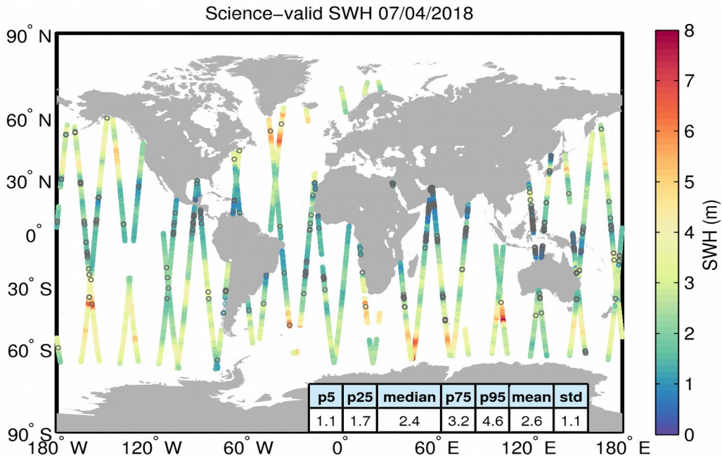
Figure 19. Geographical distribution of science-valid SWH data over oceans and lakes for 07/04/2018. The statistical values shown in the table refer to the SWH in m and are calculated over all measurements shown in the figure. Gray circles denote records that have been rejected based on the editing criteria described in Table 3.
