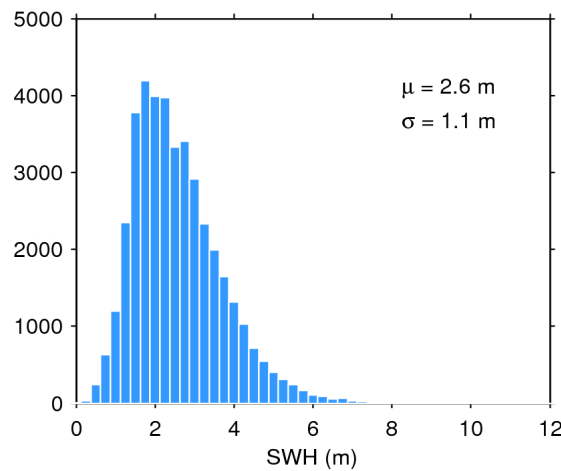
Figure 17. Histogram of flag-valid SWH over oceans and lakes for 07/04/2018. The mean ( \mu ) and standard deviation ( \sigma ) are also shown. Note that values larger than 12 m are excluded from the histogram for the sake of readability but not from the computation of \mu and \sigma .
