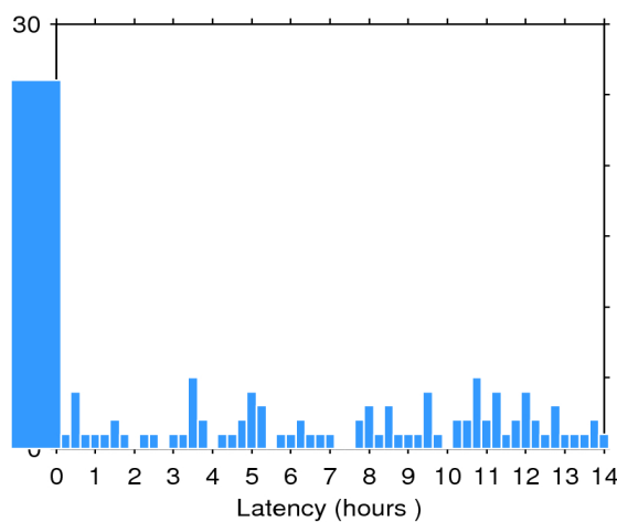
Figure 2. Histogram of the data latency for 07/04/2018. The y-axis denotes the number of files that are made available with a delay of x-hours with respect to the mean time of the records stored in the file.
