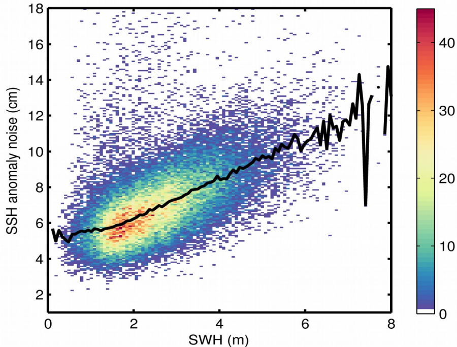
Figure 9. 2D histogram showing flag-valid SSH anomaly noise as a function of SWH for 07/04/2018. The black line denotes the median SSH anomaly noise as a function of SWH.
