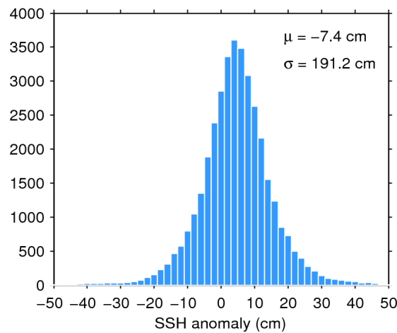
Figure 7. Histogram of flag-valid SSH anomaly over oceans and lakes for 07/04/2018. The mean ( \mu ) and standard deviation ( \sigma ) are also shown. Note that values outside [-50 50] cm are excluded from the histogram for the sake of readability but not from the computation of \mu and \sigma .
