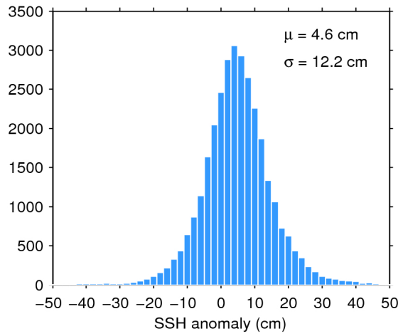
Figure 11. Histogram of science-valid SSH anomaly over oceans and lakes for 07/04/2018. The mean ( \mu ) and standard deviation ( \sigma ) are also shown. Note that values outside [-50 50] cm are excluded from the histogram for the sake of readability but not from the computation of \mu and \sigma .
