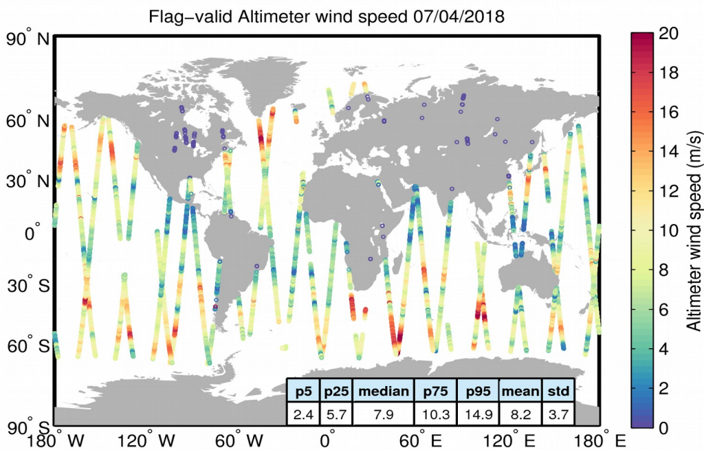
Figure 31. Geographical distribution of flag-valid wind data over oceans and lakes for 07/04/2018. The statistical values shown in the table refer to the wind in m/s and are calculated over all measurements shown in the figure.
