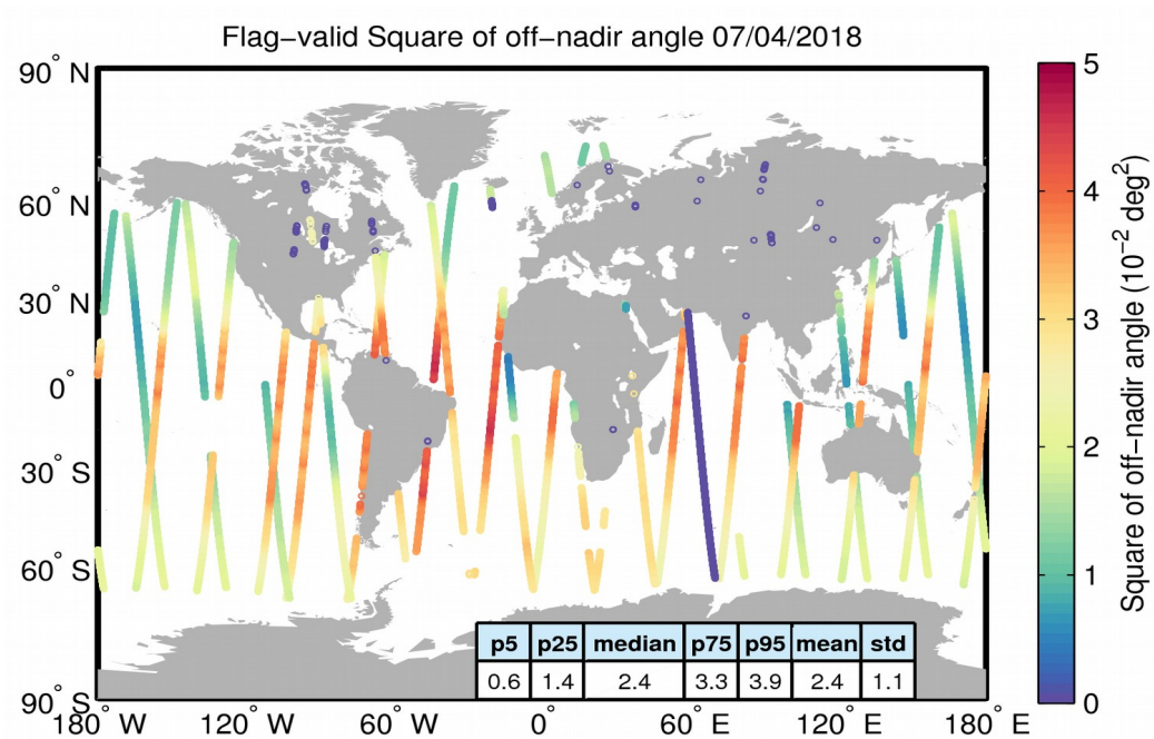
Figure 37. Geographical distribution of flag-valid mispointing data over oceans and lakes for 07/04/2018. The statistical values shown in the table refer to the mispointing in 10^{-2} \text{ deg}^2 and are calculated over all measurements shown in the figure.
