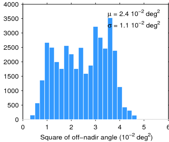
Figure 39. Histogram of flag-valid mispointing over oceans and lakes for 07/04/2018. The mean ( \mu ) and standard deviation ( \sigma ) are also shown. Note that values larger than 6 \cdot 10^{-2} \text{ deg}^2 are excluded from the histogram for the sake of readability but not from the computation of \mu and \sigma .
