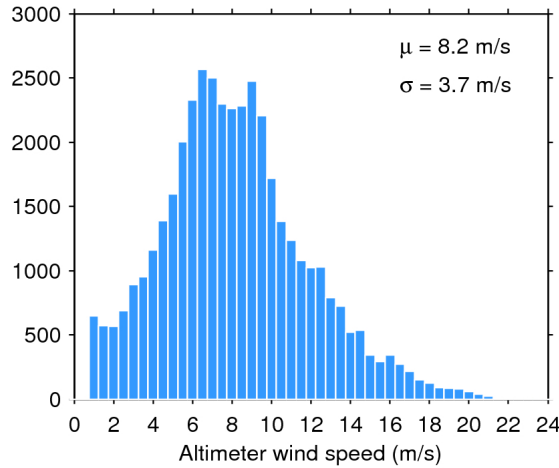
Figure 33. Histogram of flag-valid wind over oceans and lakes for 07/04/2018. The mean ( \mu ) and standard deviation ( \sigma ) are also shown. Note that values larger than 24 m/s are excluded from the histogram for the sake of readability but not from the computation of \mu and \sigma .
