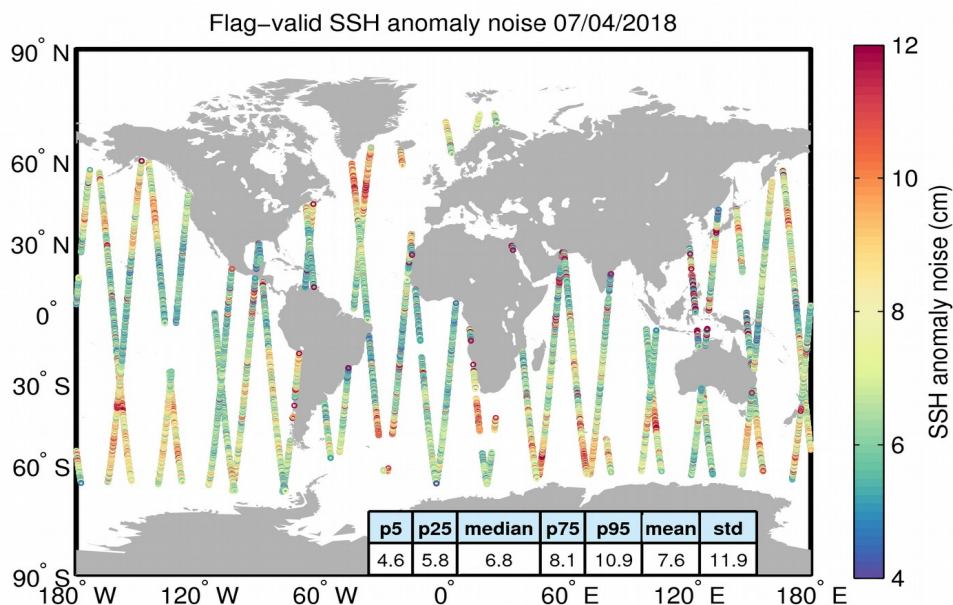
Figure 8. Geographical distribution of flag-valid 20-Hz SSH anomaly measurement noise over oceans and lakes for 07/04/2018. The statistical values shown in the table refer to the SSH anomaly noise and are calculated over all measurements shown in the figure.
