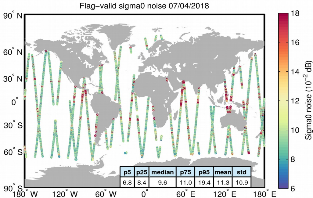
Figure 26. Geographical distribution of flag-valid 20-Hz sigma0 measurement noise over oceans and lakes for 07/04/2018. The statistical values shown in the table refer to the sigma0 noise and are calculated over all measurements shown in the figure.
