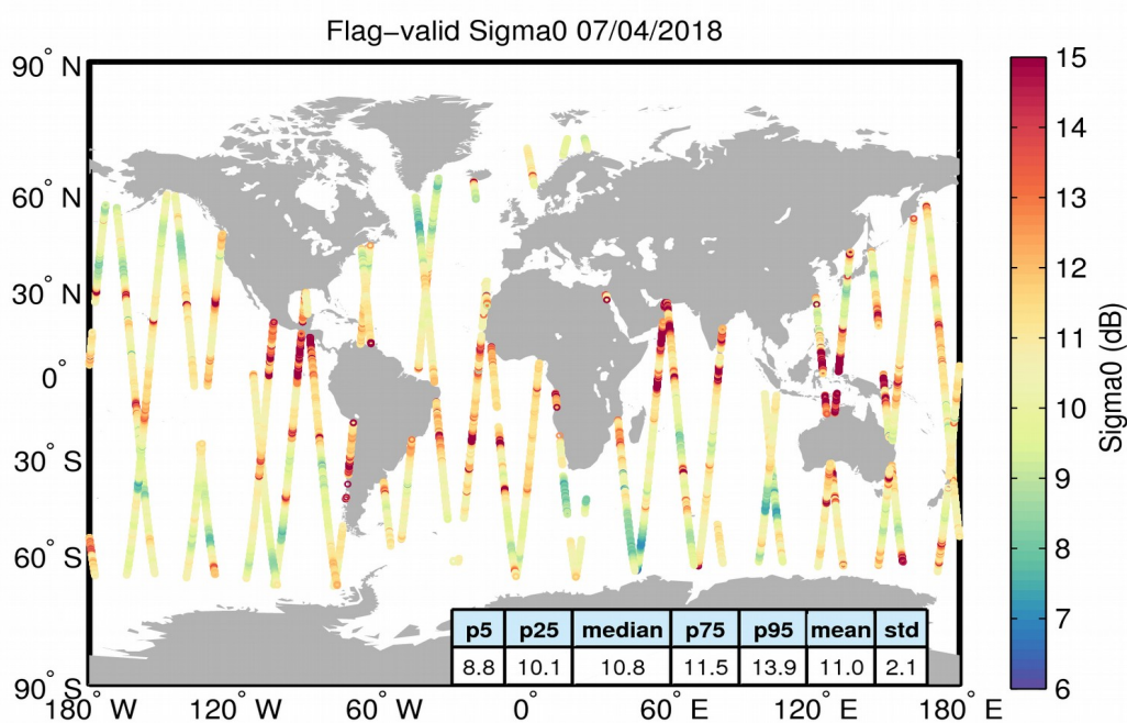
Figure 23. Geographical distribution of flag-valid sigma0 data over oceans and lakes for 07/04/2018. The statistical values shown in the table refer to the sigma0 in dB and are calculated over all measurements shown in the figure.
