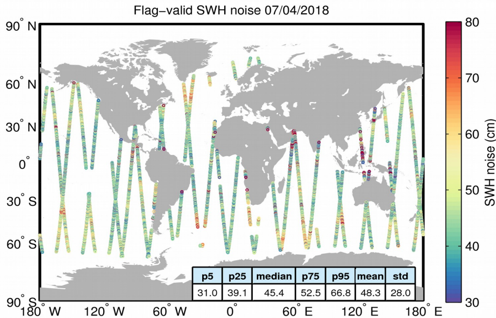
Figure 18. Geographical distribution of flag-valid 20-Hz SWH measurement noise over oceans and lakes for 07/04/2018. The statistical values shown in the figure refer to the SWH noise and are calculated over all measurements shown in the figure.
