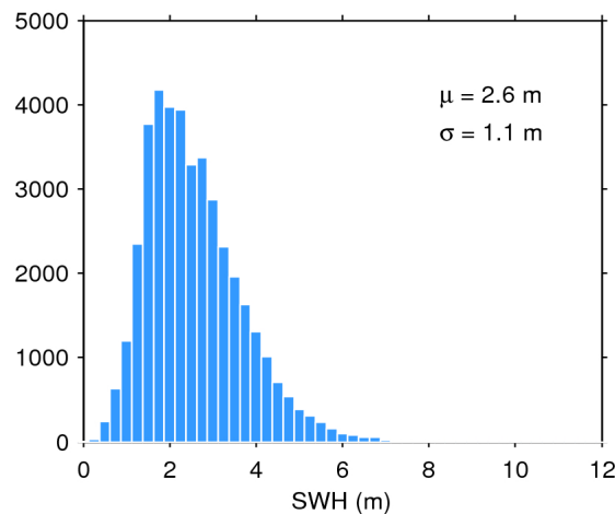
Figure 20. Histogram of science-valid SWH over oceans and lakes for 07/04/2018. The mean ( \mu ) and standard deviation ( \sigma ) are also shown. Note that values larger than 12 m are excluded from the histogram for the sake of readability but not from the computation of \mu and \sigma .
