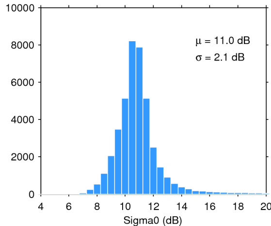
Figure 25. Histogram of flag-valid sigma0 over oceans and lakes for 07/04/2018. The mean ( \mu ) and standard deviation ( \sigma ) are also shown. Note that values outside [4 20] dB are excluded from the histogram for the sake of readability but not from the computation of \mu and \sigma .
