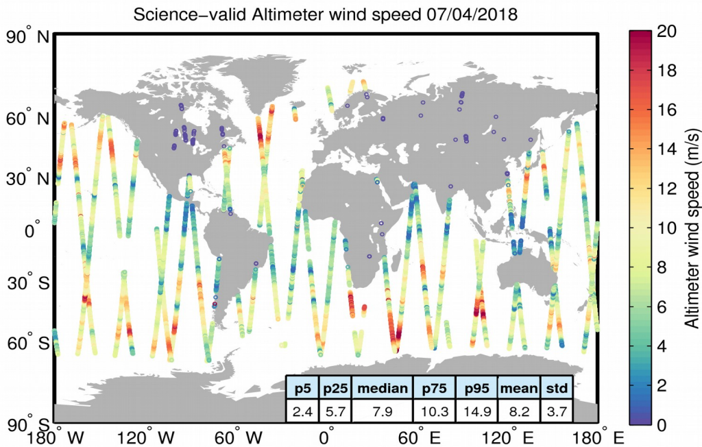
Figure 34. Geographical distribution of science-valid wind data over oceans and lakes for 07/04/2018. The statistical values shown in the table refer to the wind in m/s and are calculated over all measurements shown in the figure. Gray circles denote records that have been rejected based on the editing criteria described in Table 5.
