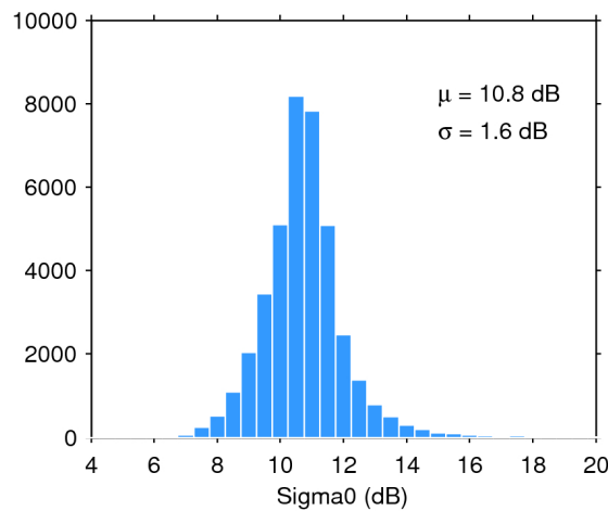
Figure 28. Histogram of science-valid sigma0 over oceans and lakes for 07/04/2018. The mean ( \mu ) and standard deviation ( \sigma ) are also shown. Note that values outside [4 20] dB are excluded from the histogram for the sake of readability but not from the computation of \mu and \sigma .
