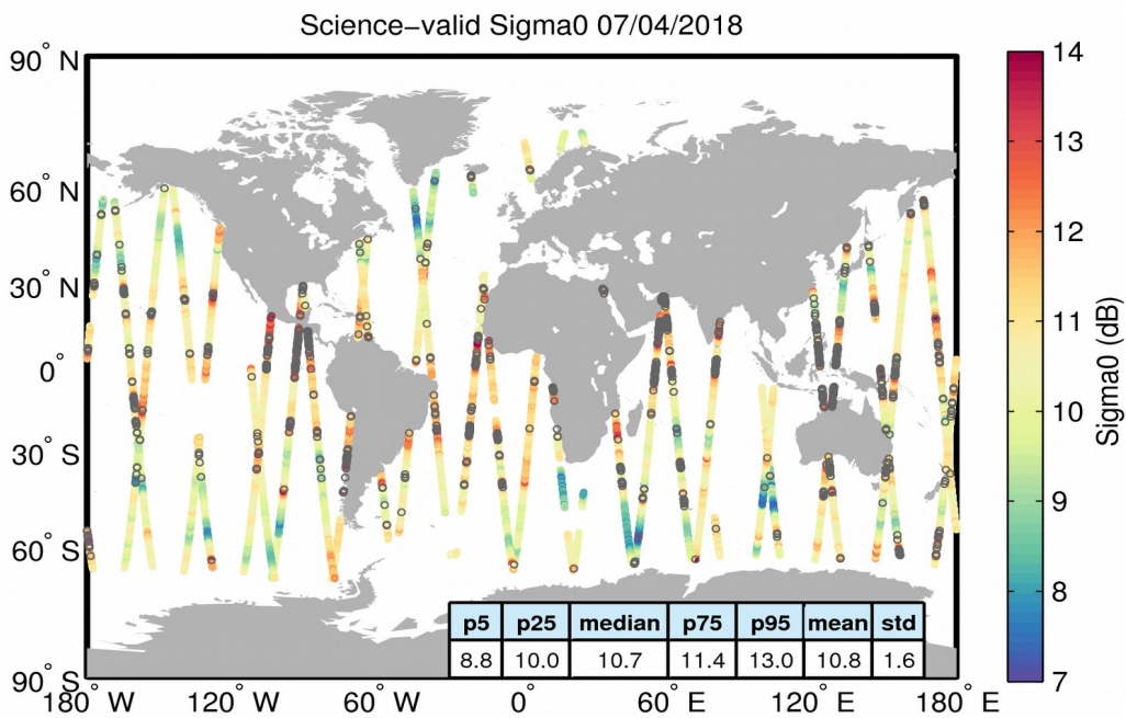
Figure 27. Geographical distribution of science-valid sigma0 data over oceans and lakes for 07/04/2018. The statistical values shown in the table refer to the sigma0 in dB and are calculated over all measurements shown in the figure. Gray circles denote records that have been rejected based on the editing criteria described in Table 4.
