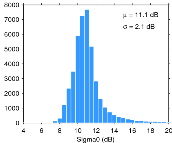
Figure 25. Histogram of flag-valid sigma0 over oceans and lakes for 06/04/2018. The mean ( \mu ) and standard deviation ( \sigma ) are also shown. Note that values outside [4 20] dB are excluded from the histogram for the sake of readability but not from the computation of \mu and \sigma .
