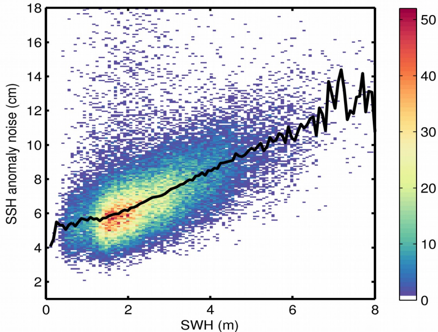
Figure 9. 2D histogram showing flag-valid SSH anomaly noise as a function of SWH for 06/04/2018. The black line denotes the median SSH anomaly noise as a function of SWH.
