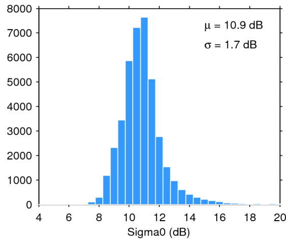
Figure 28. Histogram of science-valid sigma0 over oceans and lakes for 06/04/2018. The mean ( \mu ) and standard deviation ( \sigma ) are also shown. Note that values outside [4 20] dB are excluded from the histogram for the sake of readability but not from the computation of \mu and \sigma .
