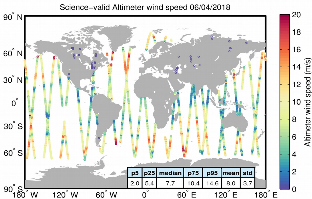
Figure 34. Geographical distribution of science-valid wind data over oceans and lakes for 06/04/2018. The statistical values shown in the table refer to the wind in m/s and are calculated over all measurements shown in the figure. Gray circles denote records that have been rejected based on the editing criteria described in Table 5.
