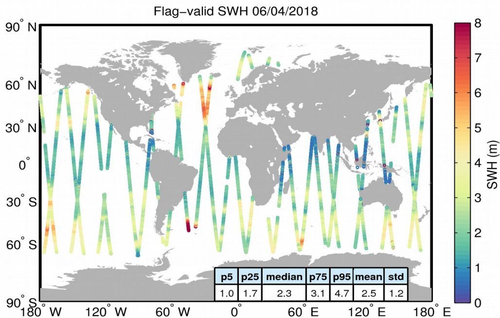
Figure 15. Geographical distribution of flag-valid SWH data over oceans and lakes for 06/04/2018. The statistical values shown in the table refer to the SWH in m and are calculated over all measurements shown in the figure.
