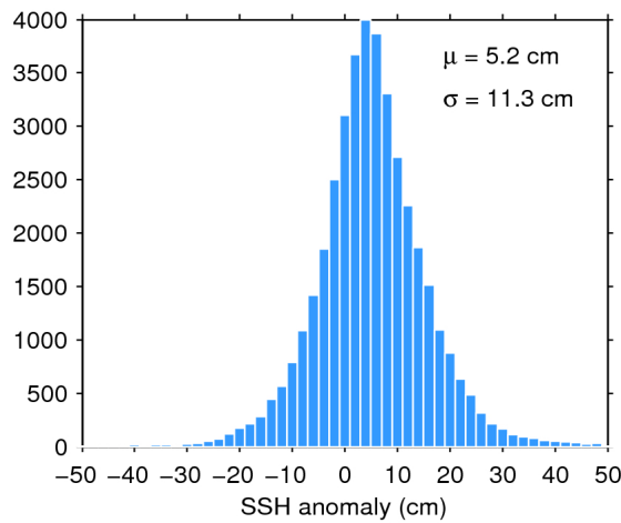
Figure 11. Histogram of science-valid SSH anomaly over oceans and lakes for 06/04/2018. The mean ( \mu ) and standard deviation ( \sigma ) are also shown. Note that values outside [-50 50] cm are excluded from the histogram for the sake of readability but not from the computation of \mu and \sigma .
