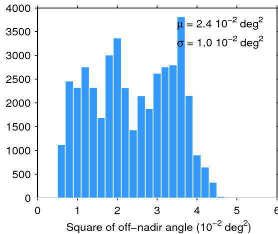
Figure 39. Histogram of flag-valid mispointing over oceans and lakes for 06/04/2018. The mean ( \mu ) and standard deviation ( \sigma ) are also shown. Note that values larger than 6 \cdot 10^{-2} \text{ deg}^2 are excluded from the histogram for the sake of readability but not from the computation of \mu and \sigma .
