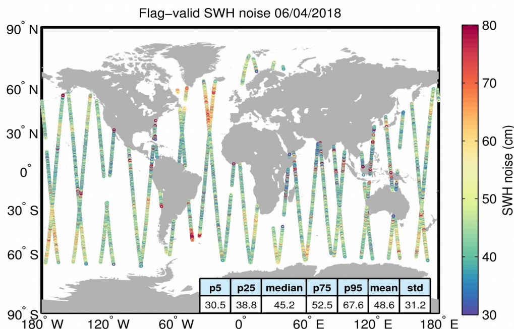
Figure 18. Geographical distribution of flag-valid 20-Hz SWH measurement noise over oceans and lakes for 06/04/2018. The statistical values shown in the figure refer to the SWH noise and are calculated over all measurements shown in the figure.
