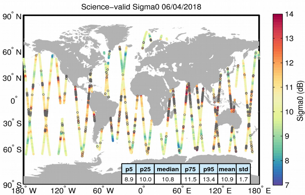
Figure 27. Geographical distribution of science-valid sigma0 data over oceans and lakes for 06/04/2018. The statistical values shown in the table refer to the sigma0 in dB and are calculated over all measurements shown in the figure. Gray circles denote records that have been rejected based on the editing criteria described in Table 4.
