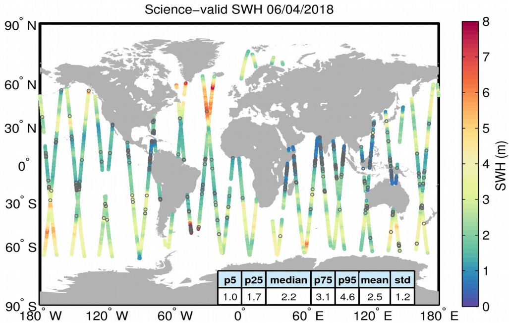
Figure 19. Geographical distribution of science-valid SWH data over oceans and lakes for 06/04/2018. The statistical values shown in the table refer to the SWH in m and are calculated over all measurements shown in the figure. Gray circles denote records that have been rejected based on the editing criteria described in Table 3.
