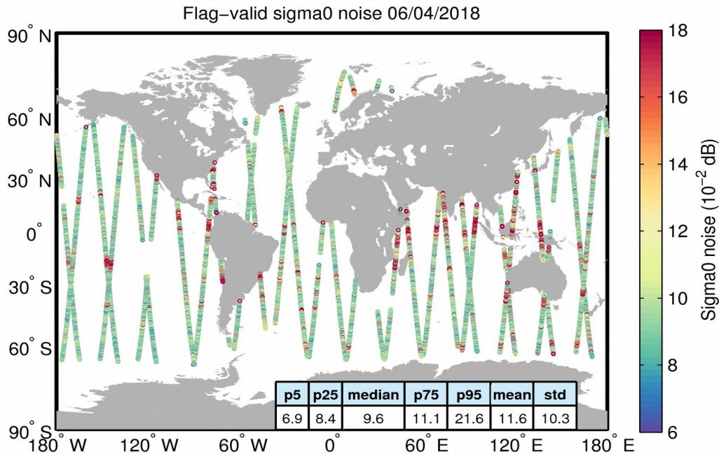
Figure 26. Geographical distribution of flag-valid 20-Hz sigma0 measurement noise over oceans and lakes for 06/04/2018. The statistical values shown in the table refer to the sigma0 noise and are calculated over all measurements shown in the figure.
