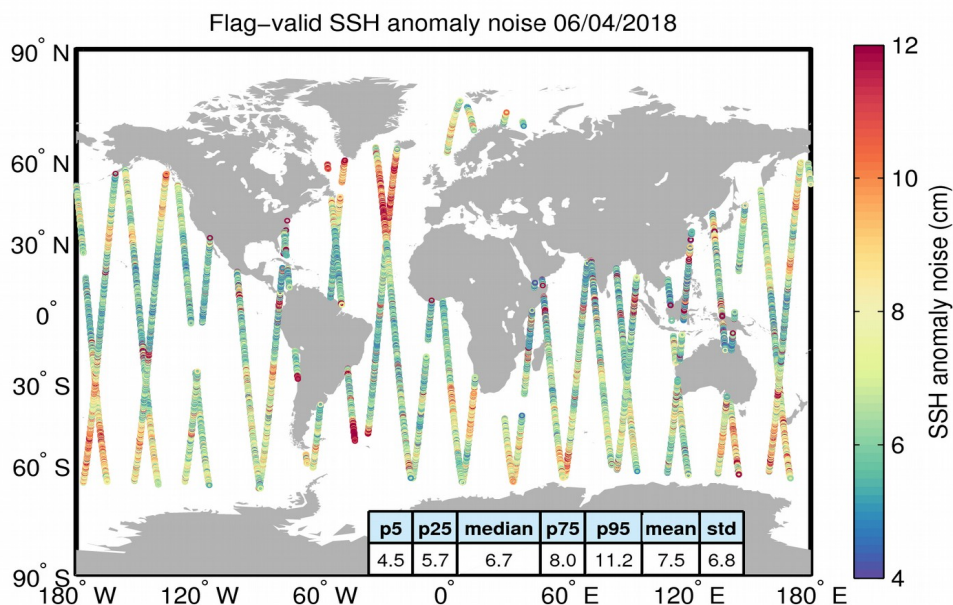
Figure 8. Geographical distribution of flag-valid 20-Hz SSH anomaly measurement noise over oceans and lakes for 06/04/2018. The statistical values shown in the table refer to the SSH anomaly noise and are calculated over all measurements shown in the figure.
