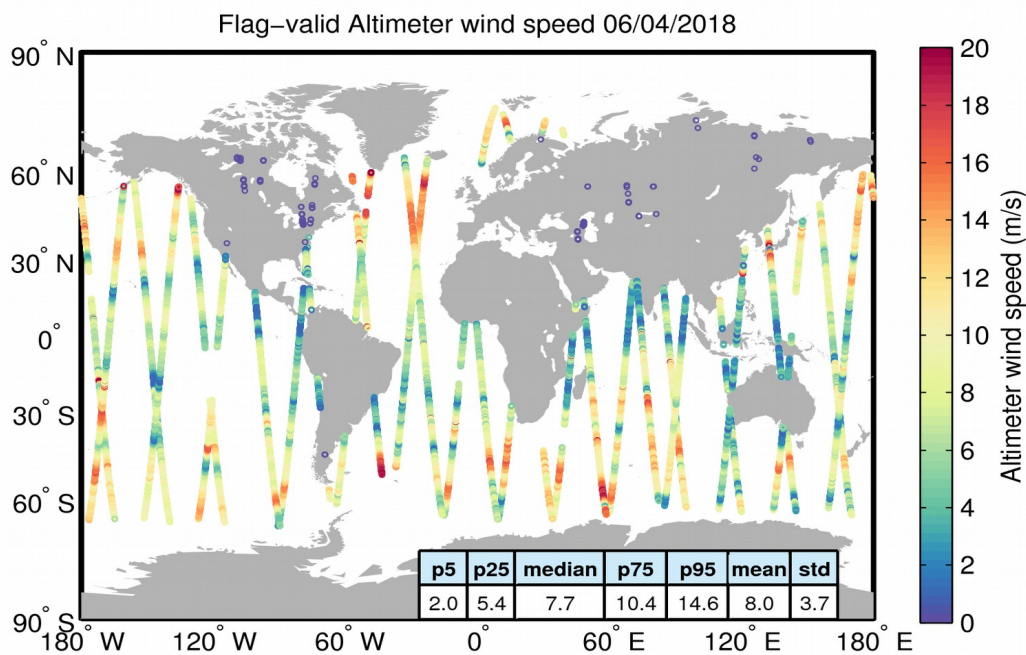
Figure 31. Geographical distribution of flag-valid wind data over oceans and lakes for 06/04/2018. The statistical values shown in the table refer to the wind in m/s and are calculated over all measurements shown in the figure.
