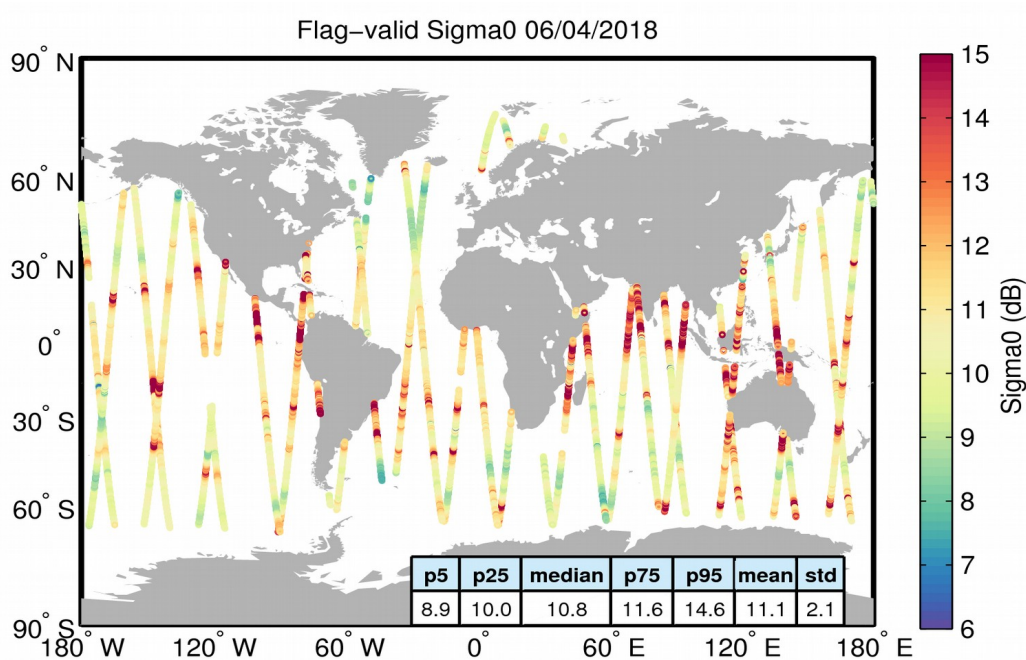
Figure 23. Geographical distribution of flag-valid sigma0 data over oceans and lakes for 06/04/2018. The statistical values shown in the table refer to the sigma0 in dB and are calculated over all measurements shown in the figure.
