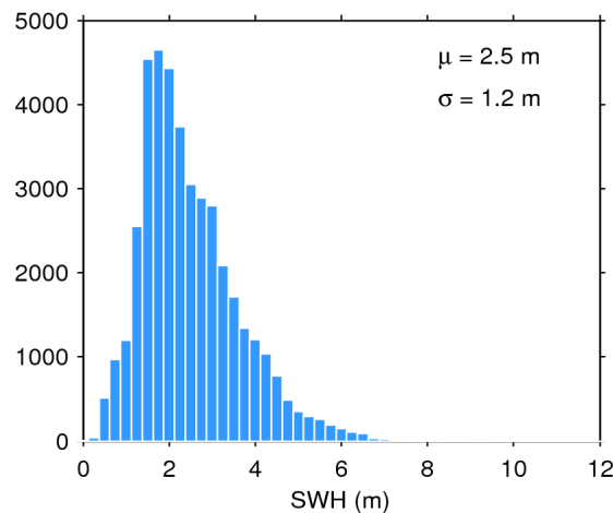
Figure 20. Histogram of science-valid SWH over oceans and lakes for 06/04/2018. The mean ( \mu ) and standard deviation ( \sigma ) are also shown. Note that values larger than 12 m are excluded from the histogram for the sake of readability but not from the computation of \mu and \sigma .
