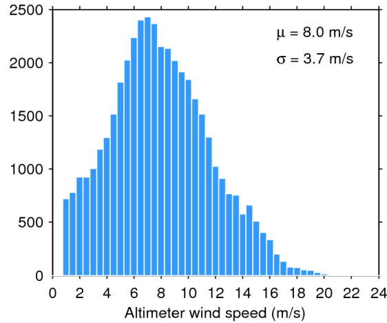
Figure 33. Histogram of flag-valid wind over oceans and lakes for 06/04/2018. The mean ( \mu ) and standard deviation ( \sigma ) are also shown. Note that values larger than 24 m/s are excluded from the histogram for the sake of readability but not from the computation of \mu and \sigma .
