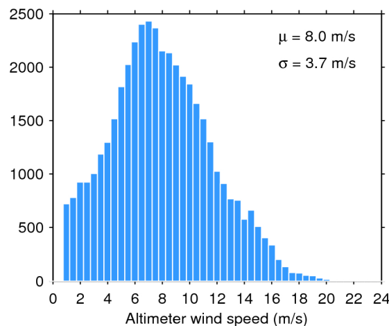
Figure 35. Histogram of science-valid wind over oceans and lakes for 06/04/2018. The mean ( \mu ) and standard deviation ( \sigma ) are also shown. Note that values larger than 24 m/s are excluded from the histogram for the sake of readability but not from the computation of \mu and \sigma .
