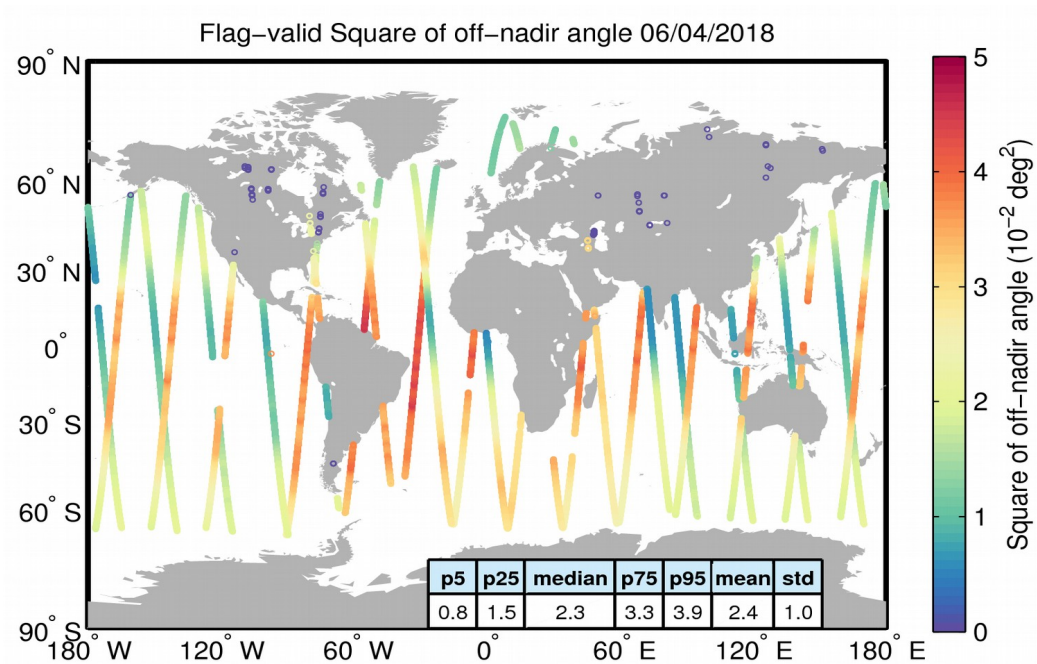
Figure 37. Geographical distribution of flag-valid mispointing data over oceans and lakes for 06/04/2018. The statistical values shown in the table refer to the mispointing in 10^{-2} deg 2 and are calculated over all measurements shown in the figure.
