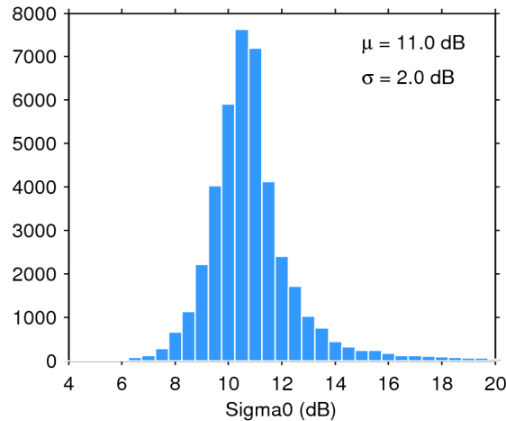
Figure 25. Histogram of flag-valid sigma0 over oceans and lakes for 05/04/2018. The mean ( \mu ) and standard deviation ( \sigma ) are also shown. Note that values outside [4 20] dB are excluded from the histogram for the sake of readability but not from the computation of \mu and \sigma .
