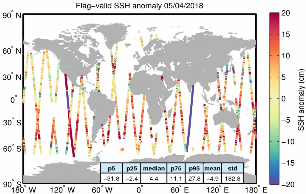
Figure 5. Geographical distribution of flag-valid 1-Hz SSH anomaly data over oceans and lakes for 05/04/2018. The statistical values shown in the table refer to the SSH anomaly in cm and are calculated over all measurements shown in the figure.
