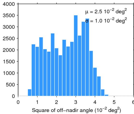
Figure 39. Histogram of flag-valid mispointing over oceans and lakes for 05/04/2018. The mean ( \mu ) and standard deviation ( \sigma ) are also shown. Note that values larger than 6 \cdot 10^{-2} \text{ deg}^2 are excluded from the histogram for the sake of readability but not from the computation of \mu and \sigma .
