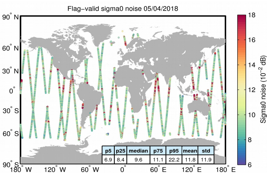
Figure 26. Geographical distribution of flag-valid 20-Hz sigma0 measurement noise over oceans and lakes for 05/04/2018. The statistical values shown in the table refer to the sigma0 noise and are calculated over all measurements shown in the figure.
