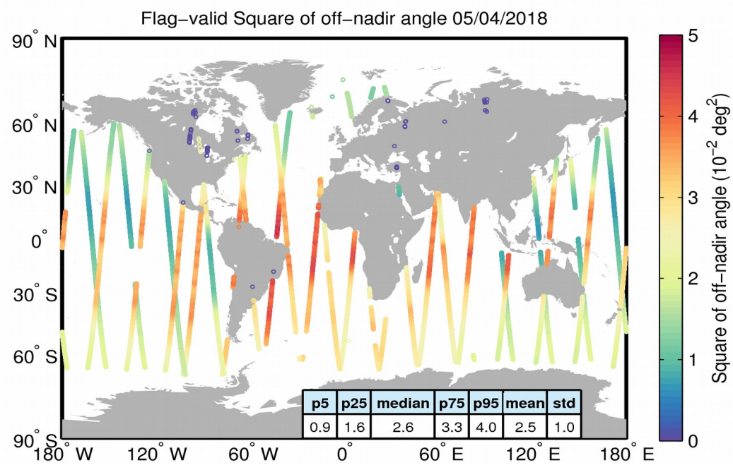
Figure 37. Geographical distribution of flag-valid mispointing data over oceans and lakes for 05/04/2018. The statistical values shown in the table refer to the mispointing in 10^{-2} \text{ deg}^2 and are calculated over all measurements shown in the figure.
