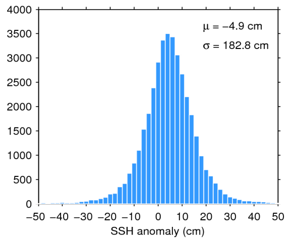
Figure 7. Histogram of flag-valid SSH anomaly over oceans and lakes for 05/04/2018. The mean ( \mu ) and standard deviation ( \sigma ) are also shown. Note that values outside [-50 50] cm are excluded from the histogram for the sake of readability but not from the computation of \mu and \sigma .
