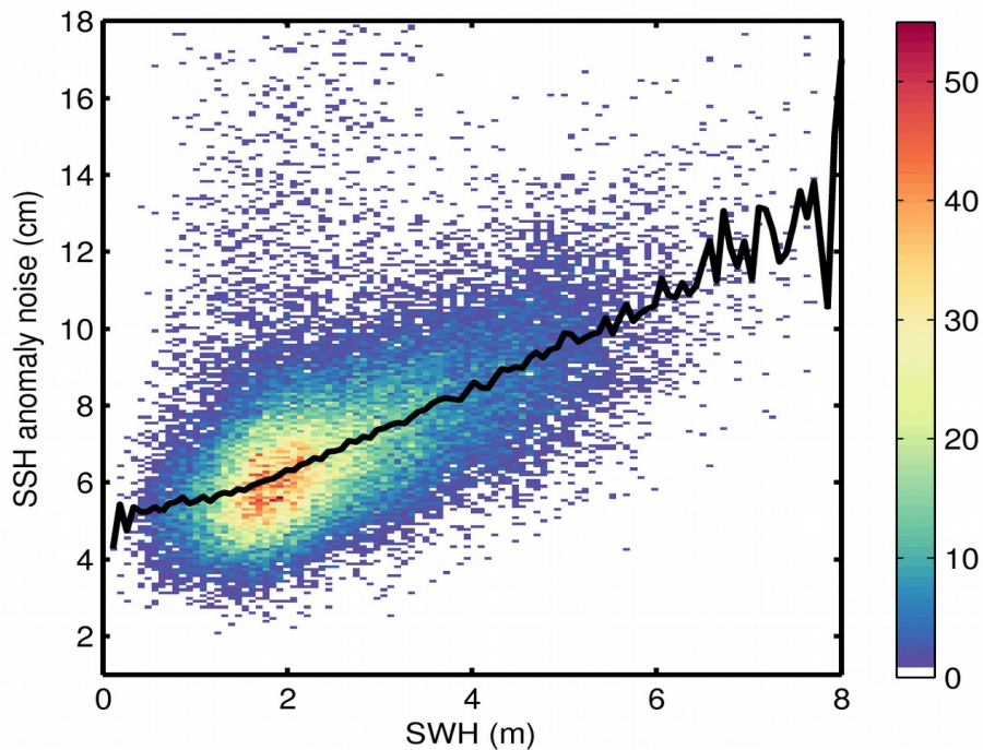
Figure 9. 2D histogram showing flag-valid SSH anomaly noise as a function of SWH for 05/04/2018. The black line denotes the median SSH anomaly noise as a function of SWH.
