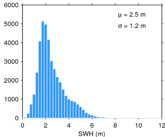
Figure 20. Histogram of science-valid SWH over oceans and lakes for 05/04/2018. The mean ( \mu ) and standard deviation ( \sigma ) are also shown. Note that values larger than 12 m are excluded from the histogram for the sake of readability but not from the computation of \mu and \sigma .
