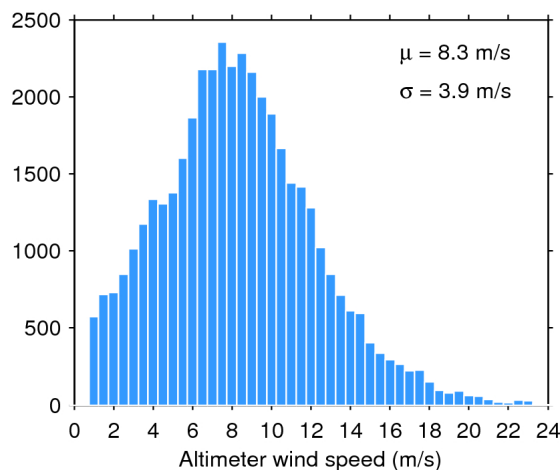
Figure 35. Histogram of science-valid wind over oceans and lakes for 05/04/2018. The mean ( \mu ) and standard deviation ( \sigma ) are also shown. Note that values larger than 24 m/s are excluded from the histogram for the sake of readability but not from the computation of \mu and \sigma .
