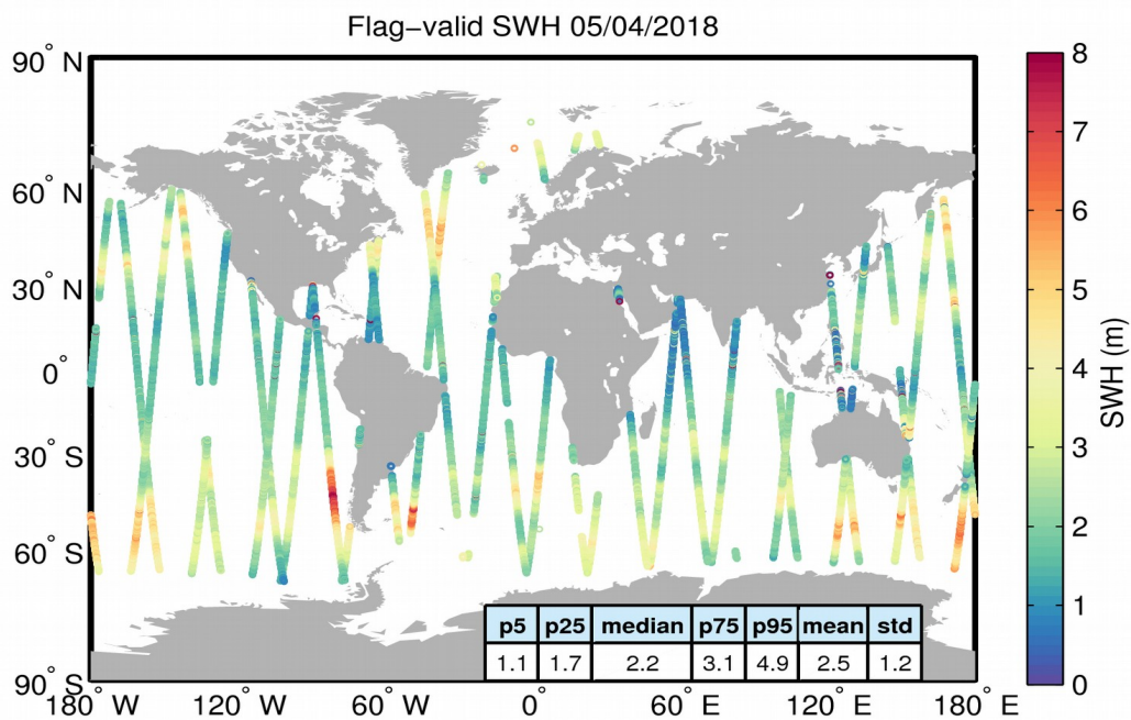
Figure 15. Geographical distribution of flag-valid SWH data over oceans and lakes for 05/04/2018. The statistical values shown in the table refer to the SWH in m and are calculated over all measurements shown in the figure.
