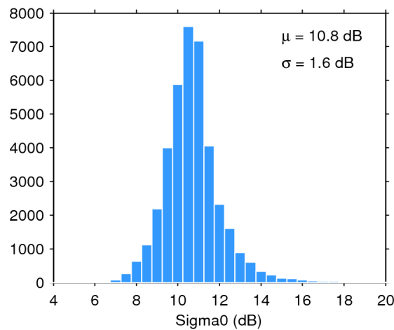
Figure 28. Histogram of science-valid sigma0 over oceans and lakes for 05/04/2018. The mean ( \mu ) and standard deviation ( \sigma ) are also shown. Note that values outside [4 20] dB are excluded from the histogram for the sake of readability but not from the computation of \mu and \sigma .
