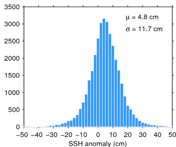
Figure 11. Histogram of science-valid SSH anomaly over oceans and lakes for 05/04/2018. The mean ( \mu ) and standard deviation ( \sigma ) are also shown. Note that values outside [-50 50] cm are excluded from the histogram for the sake of readability but not from the computation of \mu and \sigma .
