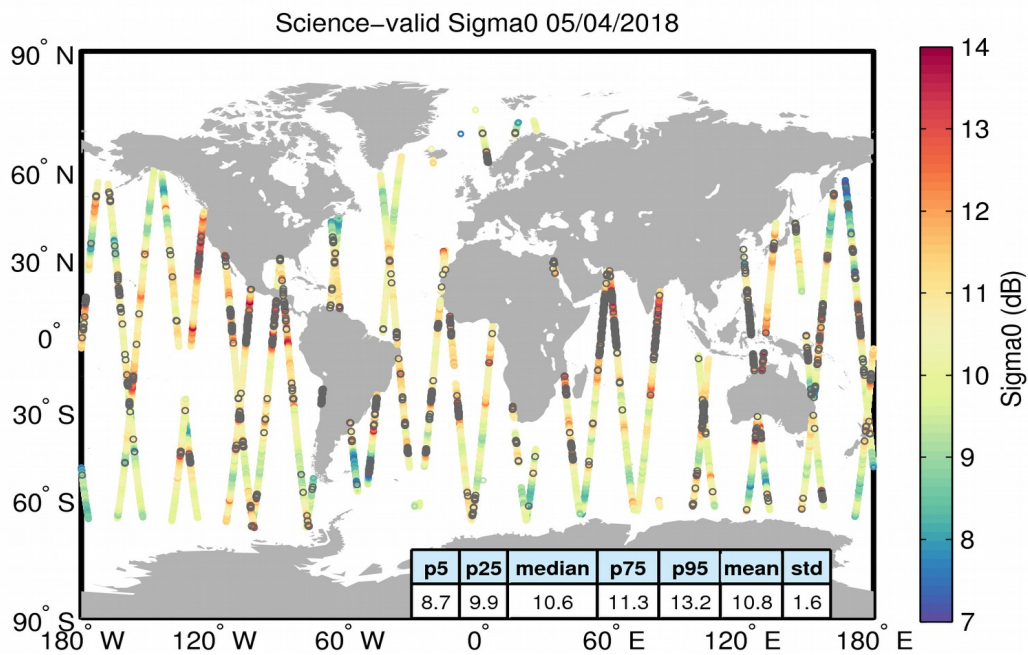
Figure 27. Geographical distribution of science-valid sigma0 data over oceans and lakes for 05/04/2018. The statistical values shown in the table refer to the sigma0 in dB and are calculated over all measurements shown in the figure. Gray circles denote records that have been rejected based on the editing criteria described in Table 4.
