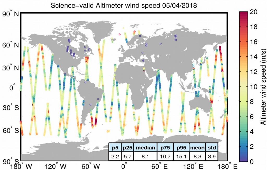
Figure 34. Geographical distribution of science-valid wind data over oceans and lakes for 05/04/2018. The statistical values shown in the table refer to the wind in m/s and are calculated over all measurements shown in the figure. Gray circles denote records that have been rejected based on the editing criteria described in Table 5.
