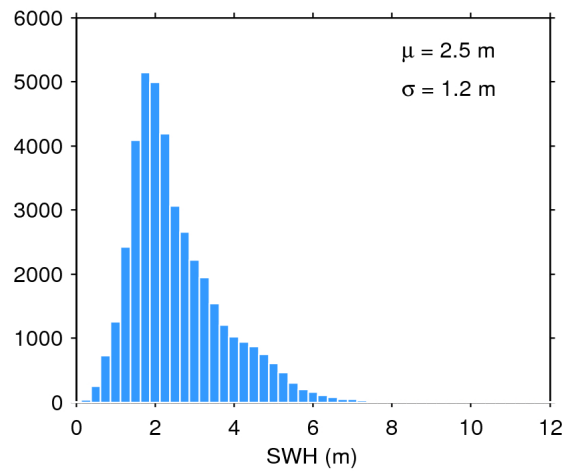
Figure 17. Histogram of flag-valid SWH over oceans and lakes for 05/04/2018. The mean ( \mu ) and standard deviation ( \sigma ) are also shown. Note that values larger than 12 m are excluded from the histogram for the sake of readability but not from the computation of \mu and \sigma .
