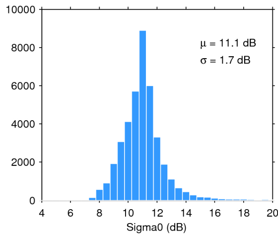
Figure 28. Histogram of science-valid sigma0 over oceans and lakes for 04/04/2018. The mean ( \mu ) and standard deviation ( \sigma ) are also shown. Note that values outside [4 20] dB are excluded from the histogram for the sake of readability but not from the computation of \mu and \sigma .
