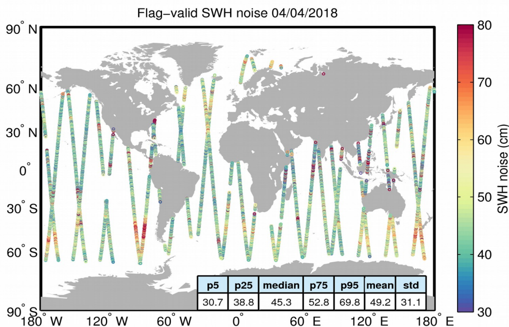
Figure 18. Geographical distribution of flag-valid 20-Hz SWH measurement noise over oceans and lakes for 04/04/2018. The statistical values shown in the figure refer to the SWH noise and are calculated over all measurements shown in the figure.
