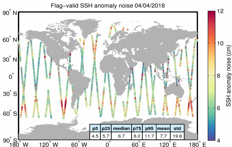
Figure 8. Geographical distribution of flag-valid 20-Hz SSH anomaly measurement noise over oceans and lakes for 04/04/2018. The statistical values shown in the table refer to the SSH anomaly noise and are calculated over all measurements shown in the figure.
