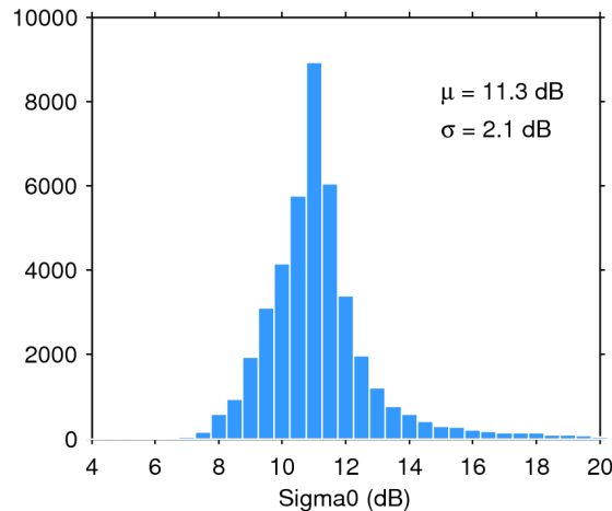
Figure 25. Histogram of flag-valid sigma0 over oceans and lakes for 04/04/2018. The mean ( \mu ) and standard deviation ( \sigma ) are also shown. Note that values outside [4 20] dB are excluded from the histogram for the sake of readability but not from the computation of \mu and \sigma .
