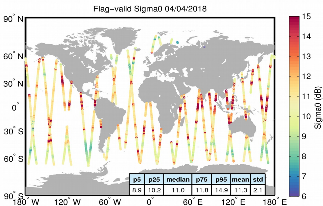
Figure 23. Geographical distribution of flag-valid sigma0 data over oceans and lakes for 04/04/2018. The statistical values shown in the table refer to the sigma0 in dB and are calculated over all measurements shown in the figure.
