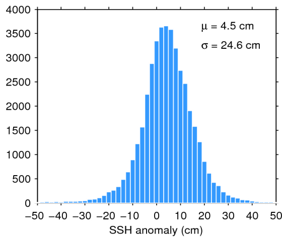
Figure 7. Histogram of flag-valid SSH anomaly over oceans and lakes for 04/04/2018. The mean ( \mu ) and standard deviation ( \sigma ) are also shown. Note that values outside [-50 50] cm are excluded from the histogram for the sake of readability but not from the computation of \mu and \sigma .
