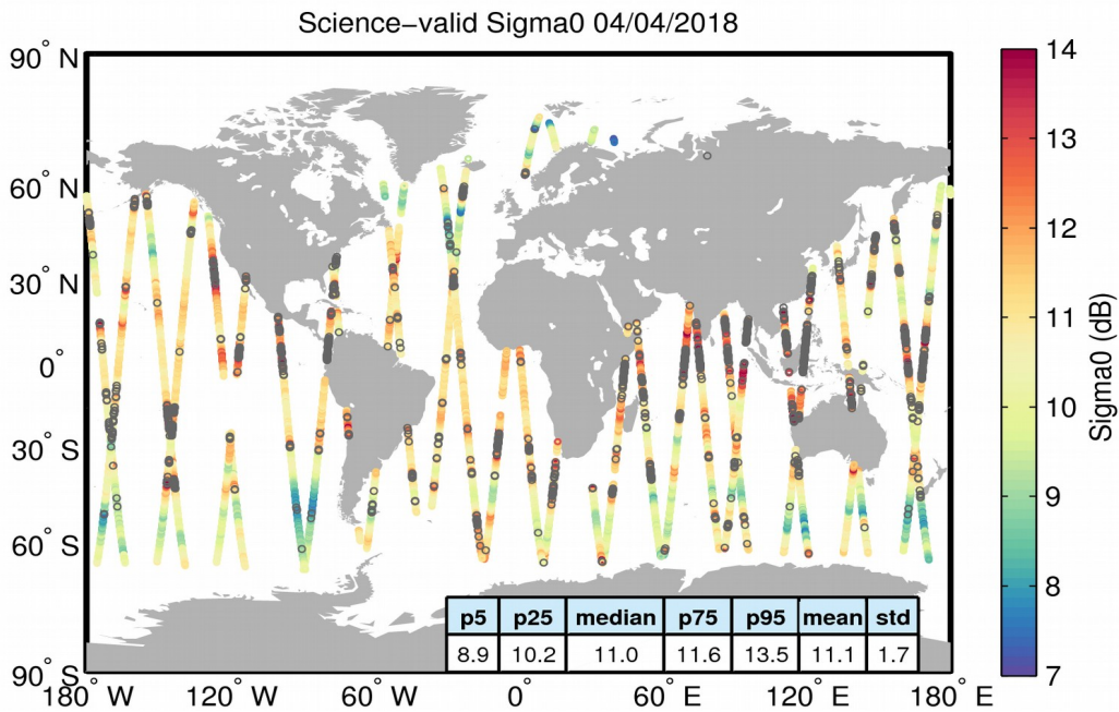
Figure 27. Geographical distribution of science-valid sigma0 data over oceans and lakes for 04/04/2018. The statistical values shown in the table refer to the sigma0 in dB and are calculated over all measurements shown in the figure. Gray circles denote records that have been rejected based on the editing criteria described in Table 4.
