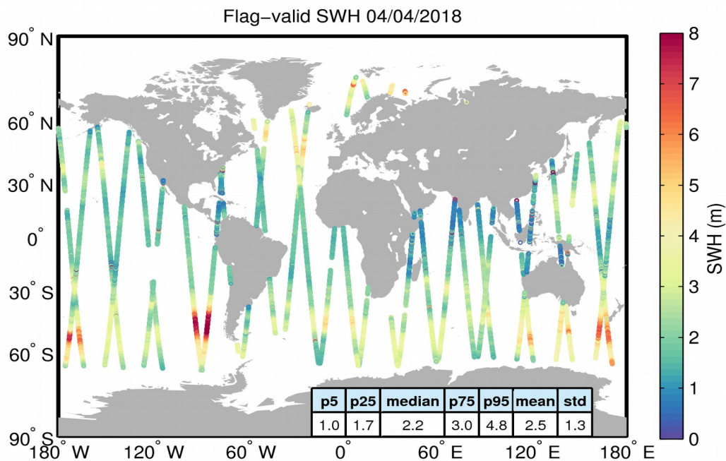
Figure 15. Geographical distribution of flag-valid SWH data over oceans and lakes for 04/04/2018. The statistical values shown in the table refer to the SWH in m and are calculated over all measurements shown in the figure.
