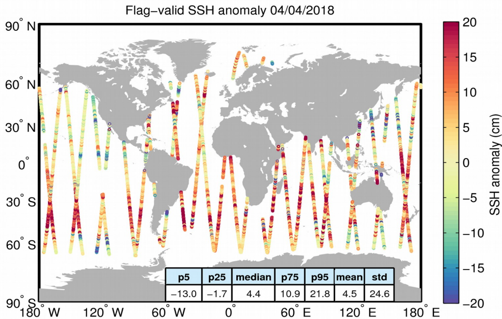
Figure 5. Geographical distribution of flag-valid 1-Hz SSH anomaly data over oceans and lakes for 04/04/2018. The statistical values shown in the table refer to the SSH anomaly in cm and are calculated over all measurements shown in the figure.
