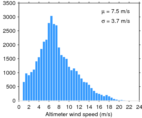
Figure 33. Histogram of flag-valid wind over oceans and lakes for 04/04/2018. The mean ( \mu ) and standard deviation ( \sigma ) are also shown. Note that values larger than 24 m/s are excluded from the histogram for the sake of readability but not from the computation of \mu and \sigma .
