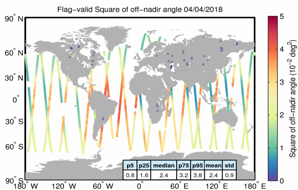
Figure 37. Geographical distribution of flag-valid mispointing data over oceans and lakes for 04/04/2018. The statistical values shown in the table refer to the mispointing in 10^{-2} \text{ deg}^2 and are calculated over all measurements shown in the figure.
