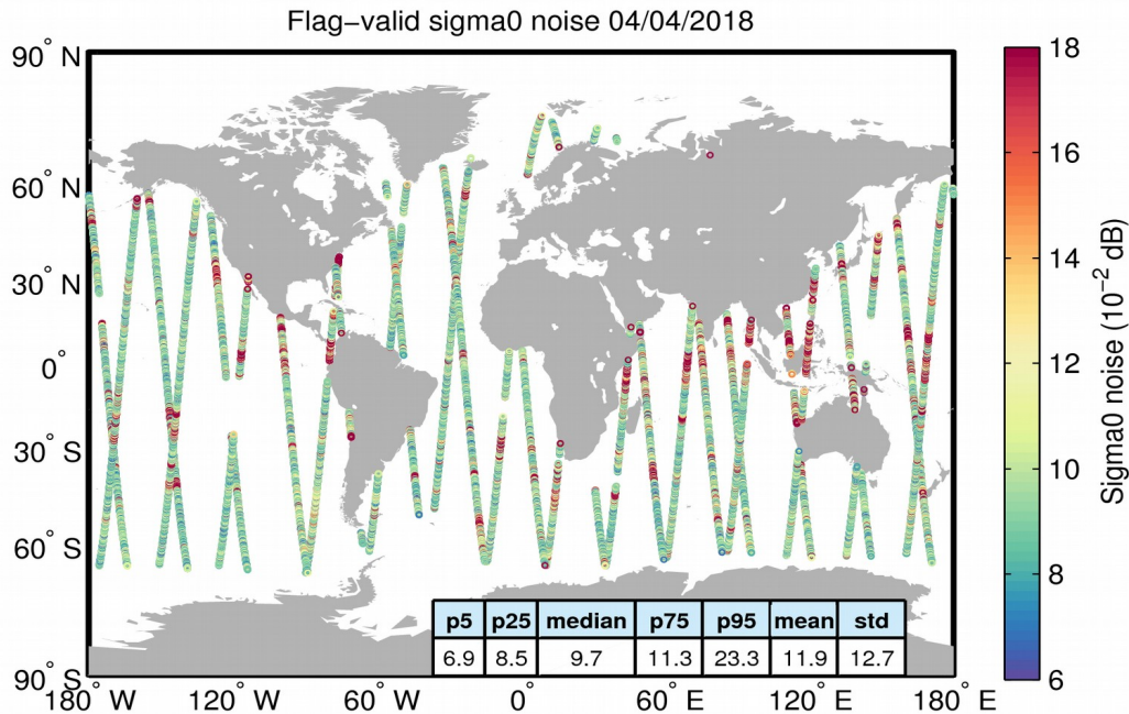
Figure 26. Geographical distribution of flag-valid 20-Hz sigma0 measurement noise over oceans and lakes for 04/04/2018. The statistical values shown in the table refer to the sigma0 noise and are calculated over all measurements shown in the figure.
