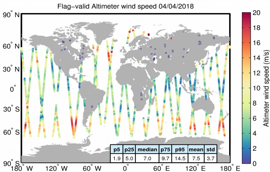
Figure 31. Geographical distribution of flag-valid wind data over oceans and lakes for 04/04/2018. The statistical values shown in the table refer to the wind in m/s and are calculated over all measurements shown in the figure.
