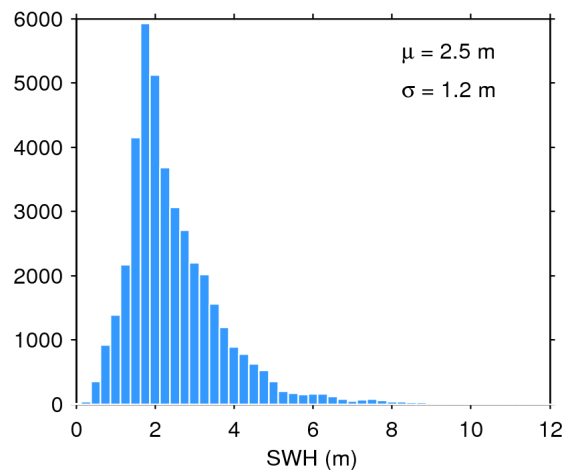
Figure 20. Histogram of science-valid SWH over oceans and lakes for 04/04/2018. The mean ( \mu ) and standard deviation ( \sigma ) are also shown. Note that values larger than 12 m are excluded from the histogram for the sake of readability but not from the computation of \mu and \sigma .
