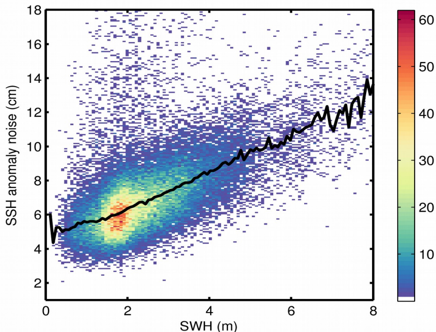
Figure 9. 2D histogram showing flag-valid SSH anomaly noise as a function of SWH for 04/04/2018. The black line denotes the median SSH anomaly noise as a function of SWH.
