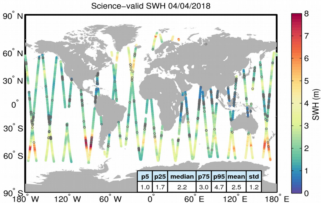
Figure 19. Geographical distribution of science-valid SWH data over oceans and lakes for 04/04/2018. The statistical values shown in the table refer to the SWH in m and are calculated over all measurements shown in the figure. Gray circles denote records that have been rejected based on the editing criteria described in Table 3.
