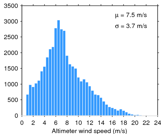
Figure 35. Histogram of science-valid wind over oceans and lakes for 04/04/2018. The mean ( \mu ) and standard deviation ( \sigma ) are also shown. Note that values larger than 24 m/s are excluded from the histogram for the sake of readability but not from the computation of \mu and \sigma .
