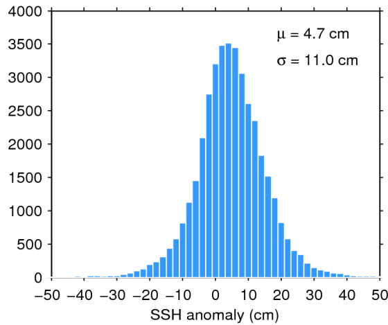
Figure 11. Histogram of science-valid SSH anomaly over oceans and lakes for 04/04/2018. The mean ( \mu ) and standard deviation ( \sigma ) are also shown. Note that values outside [-50 50] cm are excluded from the histogram for the sake of readability but not from the computation of \mu and \sigma .
