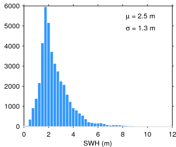
Figure 17. Histogram of flag-valid SWH over oceans and lakes for 04/04/2018. The mean ( \mu ) and standard deviation ( \sigma ) are also shown. Note that values larger than 12 m are excluded from the histogram for the sake of readability but not from the computation of \mu and \sigma .
