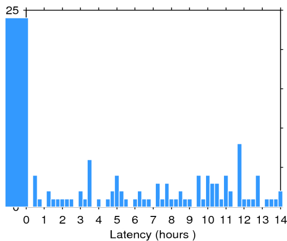
Figure 2. Histogram of the data latency for 03/04/2018. The y-axis denotes the number of files that are made available with a delay of x-hours with respect to the mean time of the records stored in the file.
