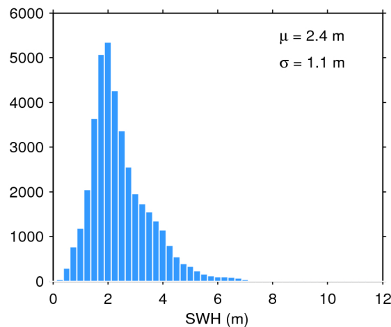
Figure 20. Histogram of science-valid SWH over oceans and lakes for 03/04/2018. The mean ( \mu ) and standard deviation ( \sigma ) are also shown. Note that values larger than 12 m are excluded from the histogram for the sake of readability but not from the computation of \mu and \sigma .
