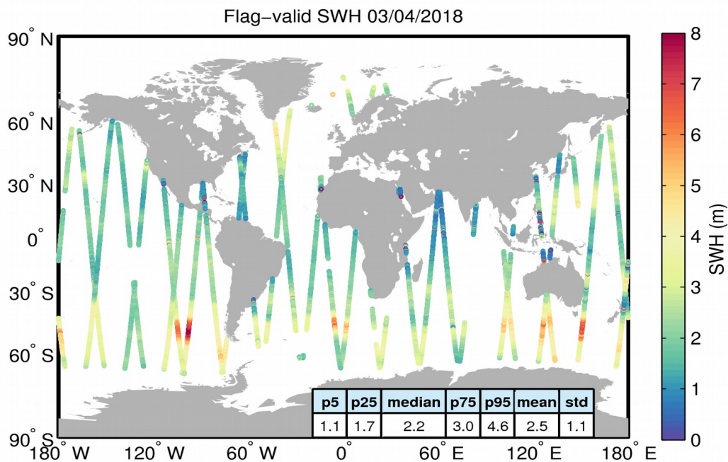
Figure 15. Geographical distribution of flag-valid SWH data over oceans and lakes for 03/04/2018. The statistical values shown in the table refer to the SWH in m and are calculated over all measurements shown in the figure.
