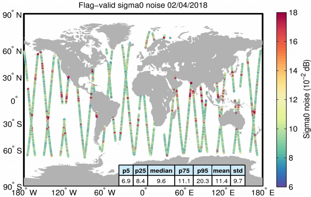
Figure 26. Geographical distribution of flag-valid 20-Hz sigma0 measurement noise over oceans and lakes for 02/04/2018. The statistical values shown in the table refer to the sigma0 noise and are calculated over all measurements shown in the figure.
