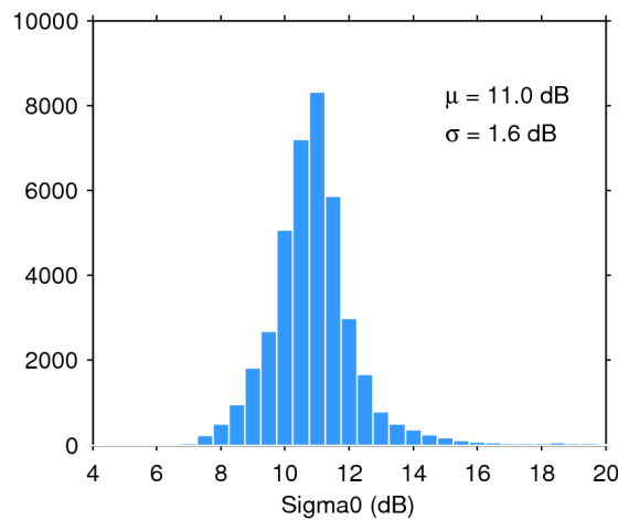
Figure 28. Histogram of science-valid sigma0 over oceans and lakes for 02/04/2018. The mean ( \mu ) and standard deviation ( \sigma ) are also shown. Note that values outside [4 20] dB are excluded from the histogram for the sake of readability but not from the computation of \mu and \sigma .
