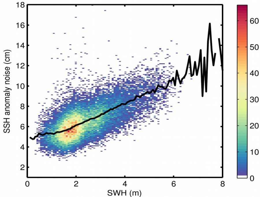
Figure 9. 2D histogram showing flag-valid SSH anomaly noise as a function of SWH for 02/04/2018. The black line denotes the median SSH anomaly noise as a function of SWH.
