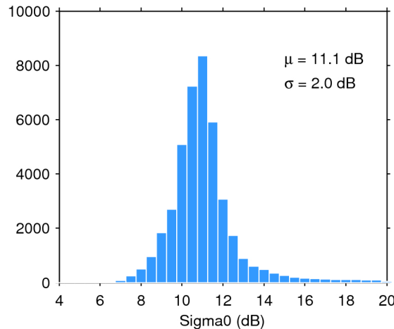
Figure 25. Histogram of flag-valid sigma0 over oceans and lakes for 02/04/2018. The mean ( \mu ) and standard deviation ( \sigma ) are also shown. Note that values outside [4 20] dB are excluded from the histogram for the sake of readability but not from the computation of \mu and \sigma .
