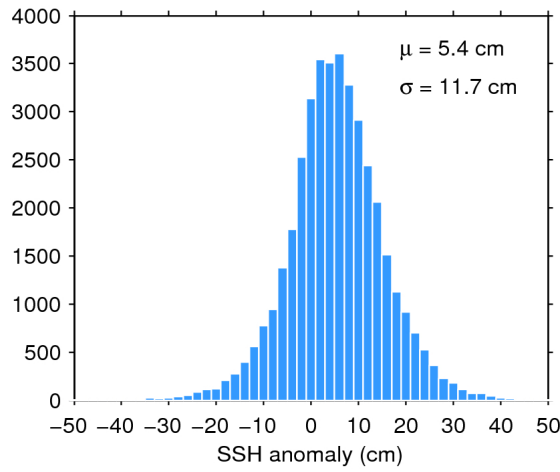
Figure 11. Histogram of science-valid SSH anomaly over oceans and lakes for 02/04/2018. The mean ( \mu ) and standard deviation ( \sigma ) are also shown. Note that values outside [-50 50] cm are excluded from the histogram for the sake of readability but not from the computation of \mu and \sigma .
