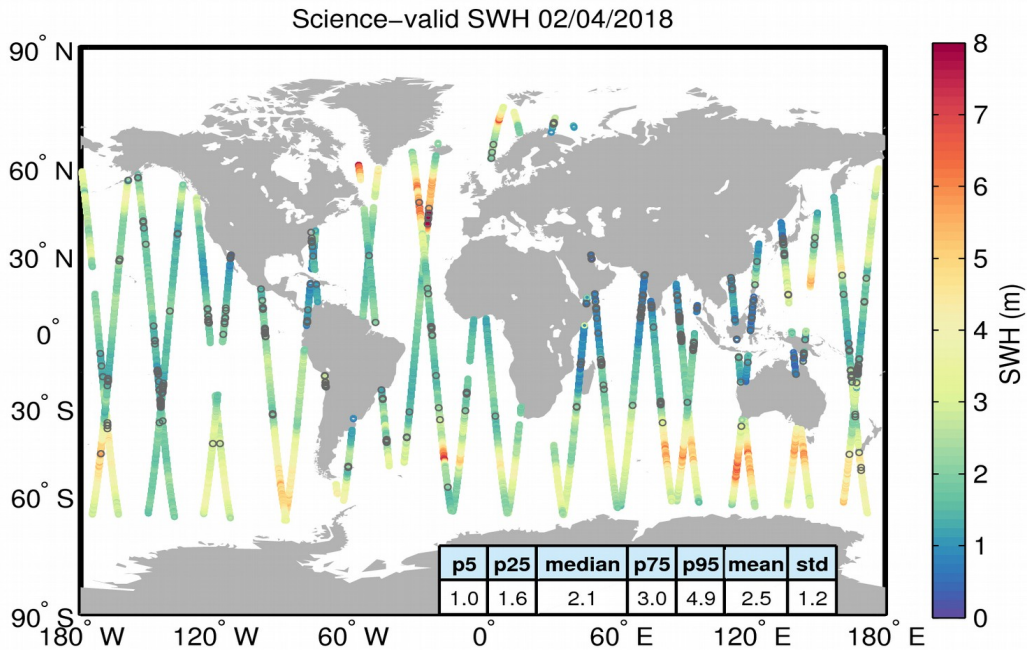
Figure 19. Geographical distribution of science-valid SWH data over oceans and lakes for 02/04/2018. The statistical values shown in the table refer to the SWH in m and are calculated over all measurements shown in the figure. Gray circles denote records that have been rejected based on the editing criteria described in Table 3.
