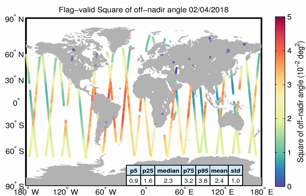
Figure 37. Geographical distribution of flag-valid mispointing data over oceans and lakes for 02/04/2018. The statistical values shown in the table refer to the mispointing in 10^{-2} deg 2 and are calculated over all measurements shown in the figure.
