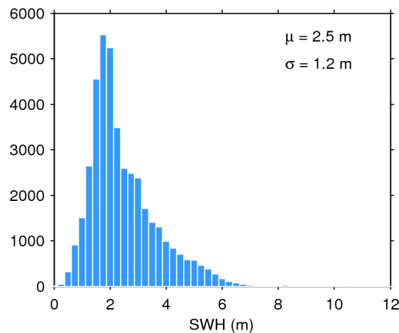
Figure 17. Histogram of flag-valid SWH over oceans and lakes for 02/04/2018. The mean ( \mu ) and standard deviation ( \sigma ) are also shown. Note that values larger than 12 m are excluded from the histogram for the sake of readability but not from the computation of \mu and \sigma .
