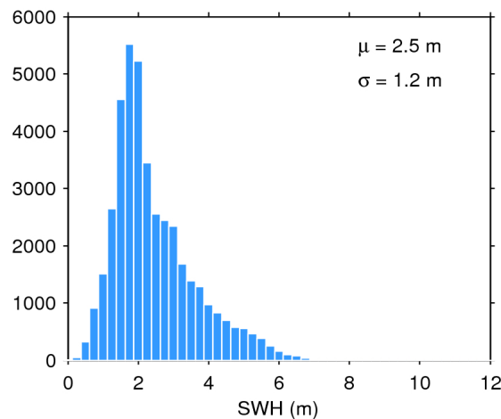
Figure 20. Histogram of science-valid SWH over oceans and lakes for 02/04/2018. The mean ( \mu ) and standard deviation ( \sigma ) are also shown. Note that values larger than 12 m are excluded from the histogram for the sake of readability but not from the computation of \mu and \sigma .
