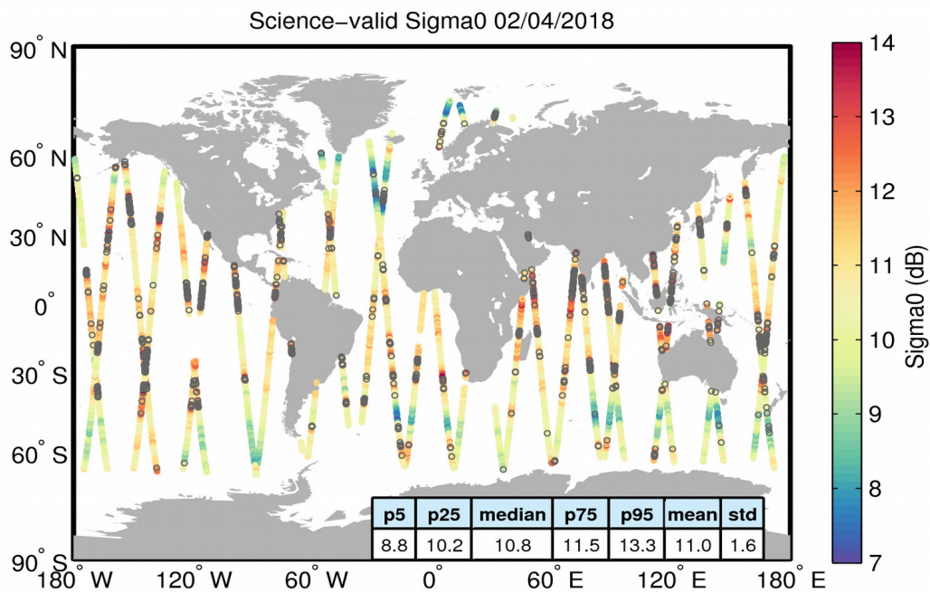
Figure 27. Geographical distribution of science-valid sigma0 data over oceans and lakes for 02/04/2018. The statistical values shown in the table refer to the sigma0 in dB and are calculated over all measurements shown in the figure. Gray circles denote records that have been rejected based on the editing criteria described in Table 4.
