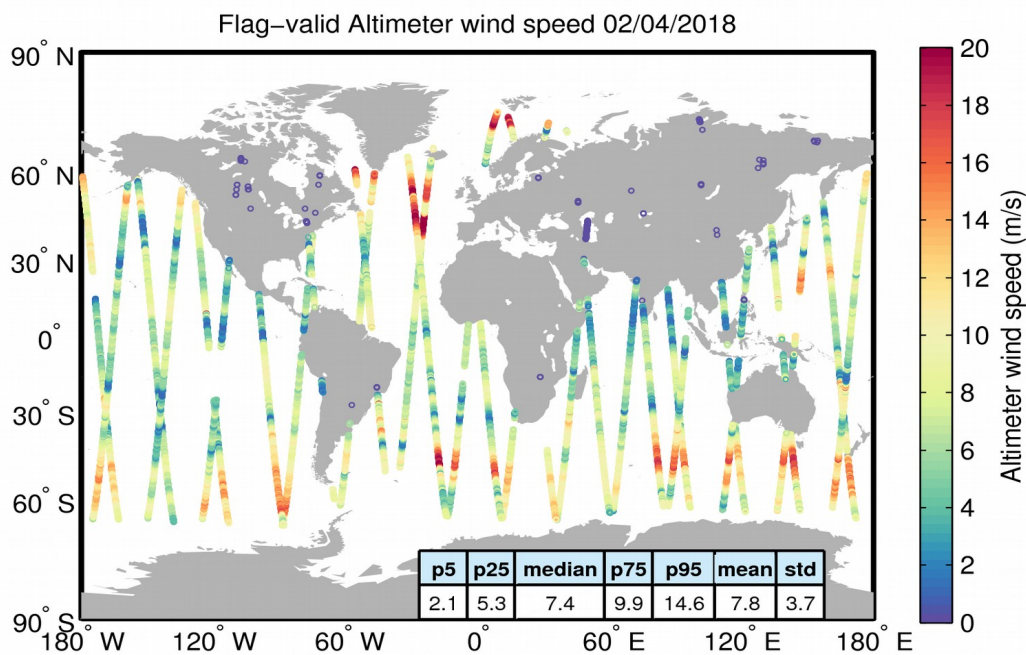
Figure 31. Geographical distribution of flag-valid wind data over oceans and lakes for 02/04/2018. The statistical values shown in the table refer to the wind in m/s and are calculated over all measurements shown in the figure.
