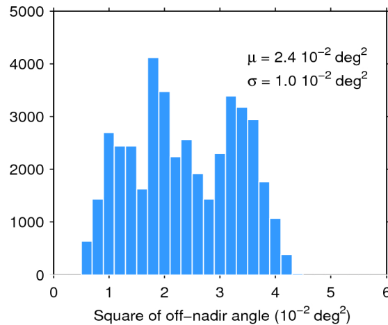
Figure 39. Histogram of flag-valid mispointing over oceans and lakes for 02/04/2018. The mean ( \mu ) and standard deviation ( \sigma ) are also shown. Note that values larger than 6 \cdot 10^{-2} \text{ deg}^2 are excluded from the histogram for the sake of readability but not from the computation of \mu and \sigma .
