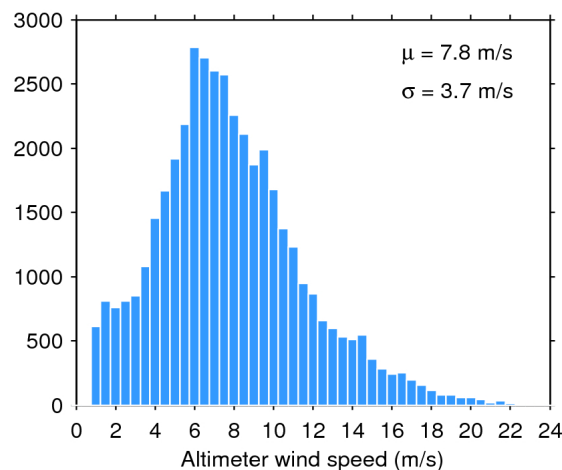
Figure 35. Histogram of science-valid wind over oceans and lakes for 02/04/2018. The mean ( \mu ) and standard deviation ( \sigma ) are also shown. Note that values larger than 24 m/s are excluded from the histogram for the sake of readability but not from the computation of \mu and \sigma .
