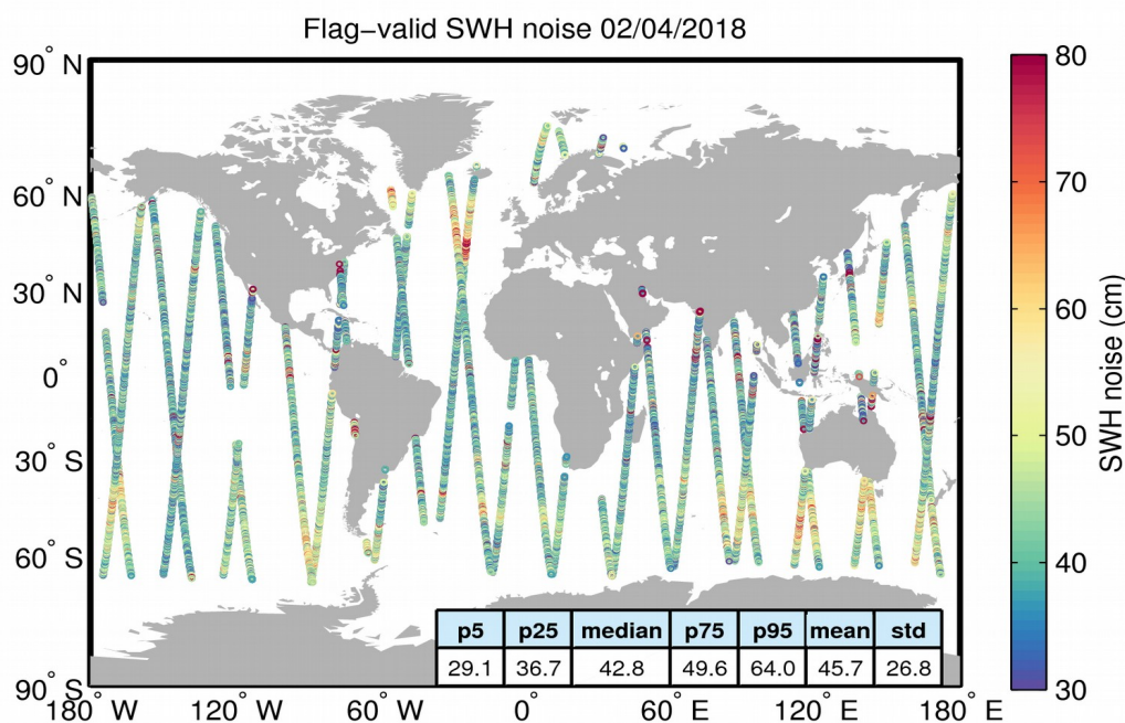
Figure 18. Geographical distribution of flag-valid 20-Hz SWH measurement noise over oceans and lakes for 02/04/2018. The statistical values shown in the figure refer to the SWH noise and are calculated over all measurements shown in the figure.
