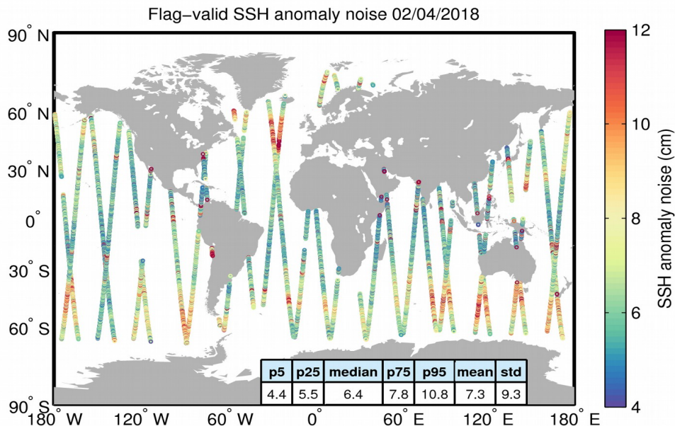
Figure 8. Geographical distribution of flag-valid 20-Hz SSH anomaly measurement noise over oceans and lakes for 02/04/2018. The statistical values shown in the table refer to the SSH anomaly noise and are calculated over all measurements shown in the figure.
