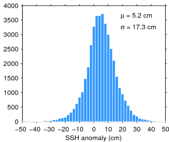
Figure 7. Histogram of flag-valid SSH anomaly over oceans and lakes for 02/04/2018. The mean ( \mu ) and standard deviation ( \sigma ) are also shown. Note that values outside [-50\ 50] cm are excluded from the histogram for the sake of readability but not from the computation of \mu and \sigma .
