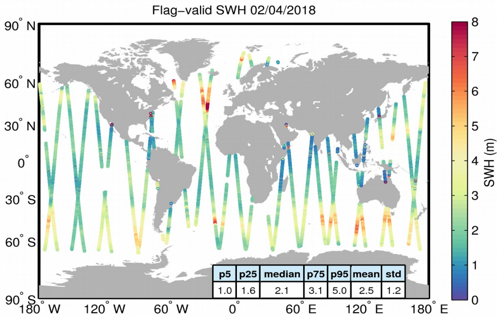
Figure 15. Geographical distribution of flag-valid SWH data over oceans and lakes for 02/04/2018. The statistical values shown in the table refer to the SWH in m and are calculated over all measurements shown in the figure.
