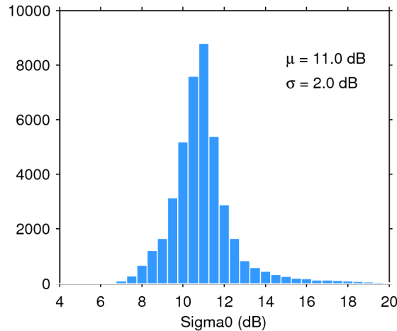
Figure 25. Histogram of flag-valid sigma0 over oceans and lakes for 01/04/2018. The mean ( \mu ) and standard deviation ( \sigma ) are also shown. Note that values outside [4 20] dB are excluded from the histogram for the sake of readability but not from the computation of \mu and \sigma .
