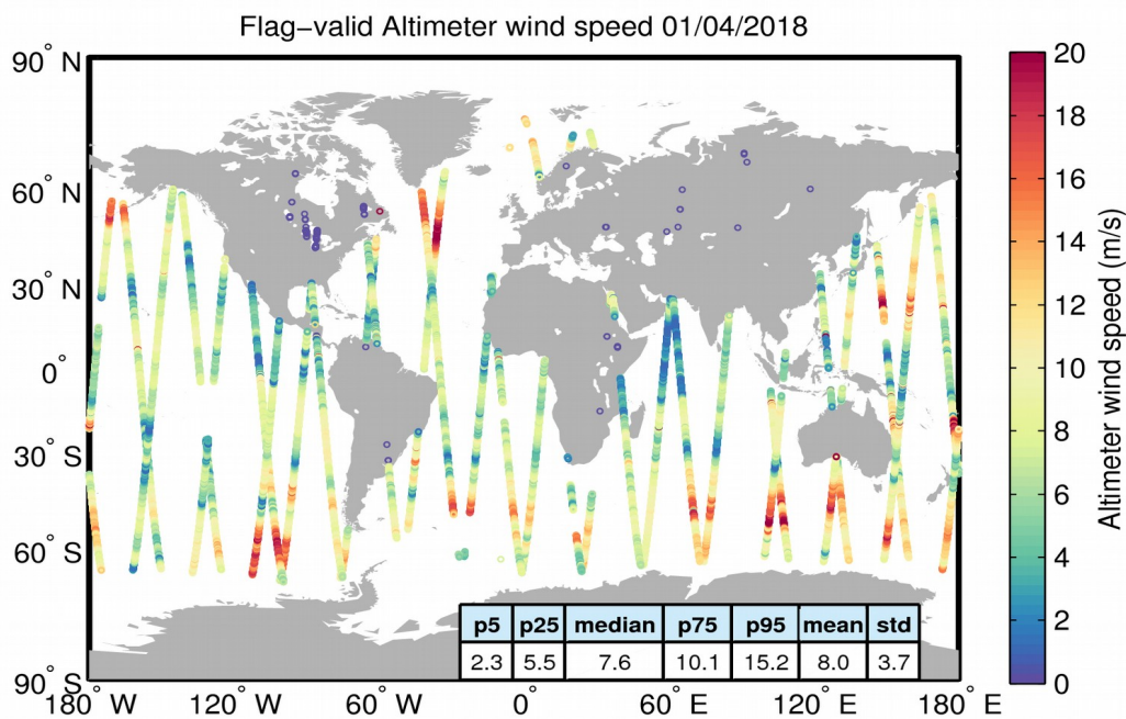
Figure 31. Geographical distribution of flag-valid wind data over oceans and lakes for 01/04/2018. The statistical values shown in the table refer to the wind in m/s and are calculated over all measurements shown in the figure.
