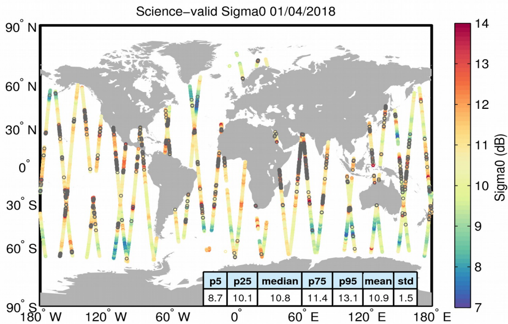
Figure 27. Geographical distribution of science-valid sigma0 data over oceans and lakes for 01/04/2018. The statistical values shown in the table refer to the sigma0 in dB and are calculated over all measurements shown in the figure. Gray circles denote records that have been rejected based on the editing criteria described in Table 4.
