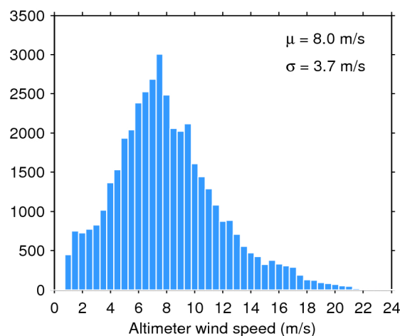
Figure 35. Histogram of science-valid wind over oceans and lakes for 01/04/2018. The mean ( \mu ) and standard deviation ( \sigma ) are also shown. Note that values larger than 24 m/s are excluded from the histogram for the sake of readability but not from the computation of \mu and \sigma .
