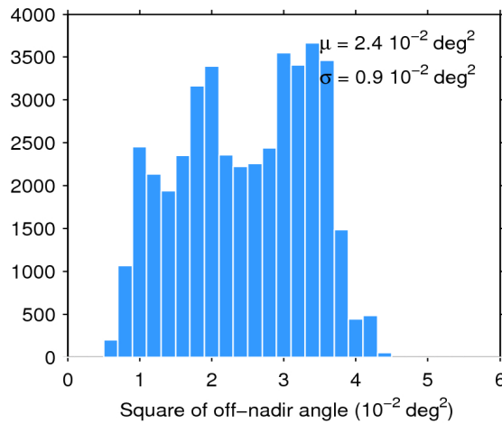
Figure 39. Histogram of flag-valid mispointing over oceans and lakes for 01/04/2018. The mean ( \mu ) and standard deviation ( \sigma ) are also shown. Note that values larger than 6 \cdot 10^{-2} \text{ deg}^2 are excluded from the histogram for the sake of readability but not from the computation of \mu and \sigma .
