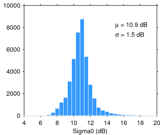
Figure 28. Histogram of science-valid sigma0 over oceans and lakes for 01/04/2018. The mean ( \mu ) and standard deviation ( \sigma ) are also shown. Note that values outside [4 20] dB are excluded from the histogram for the sake of readability but not from the computation of \mu and \sigma .
