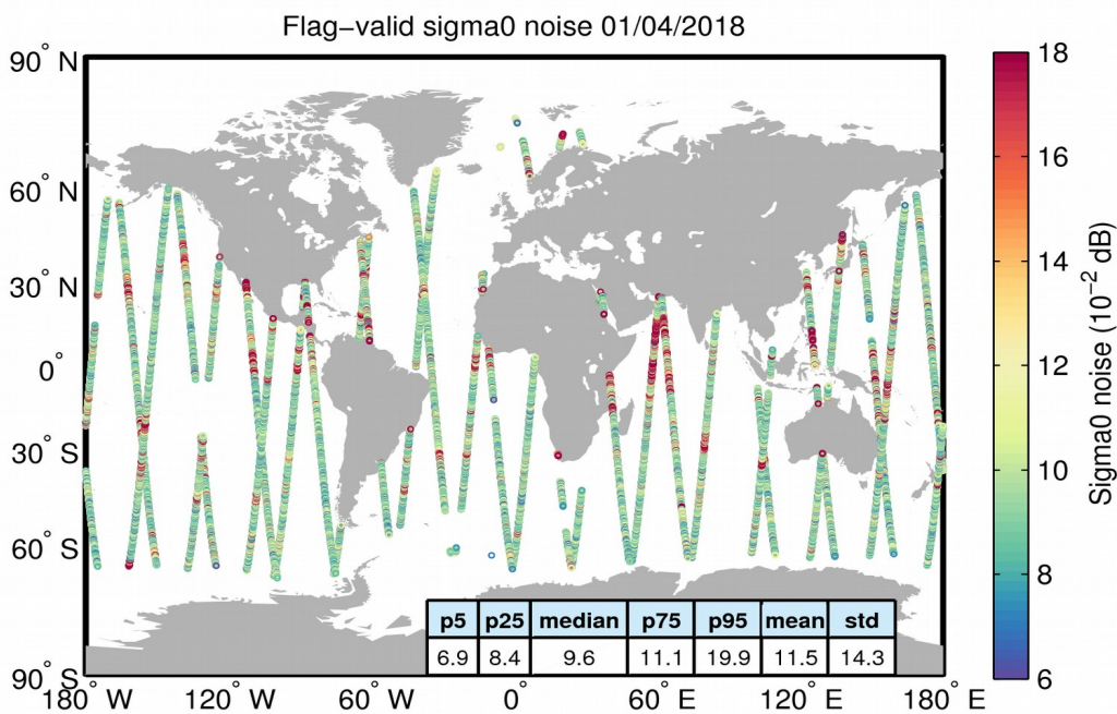
Figure 26. Geographical distribution of flag-valid 20-Hz sigma0 measurement noise over oceans and lakes for 01/04/2018. The statistical values shown in the table refer to the sigma0 noise and are calculated over all measurements shown in the figure.
