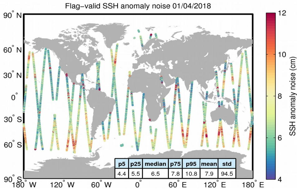
Figure 8. Geographical distribution of flag-valid 20-Hz SSH anomaly measurement noise over oceans and lakes for 01/04/2018. The statistical values shown in the table refer to the SSH anomaly noise and are calculated over all measurements shown in the figure.
