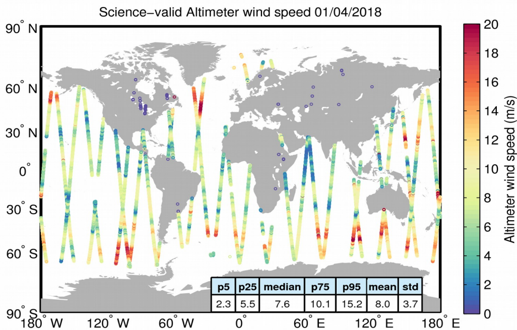
Figure 34. Geographical distribution of science-valid wind data over oceans and lakes for 01/04/2018. The statistical values shown in the table refer to the wind in m/s and are calculated over all measurements shown in the figure. Gray circles denote records that have been rejected based on the editing criteria described in Table 5.
