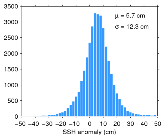
Figure 11. Histogram of science-valid SSH anomaly over oceans and lakes for 01/04/2018. The mean ( \mu ) and standard deviation ( \sigma ) are also shown. Note that values outside [-50 50] cm are excluded from the histogram for the sake of readability but not from the computation of \mu and \sigma .
