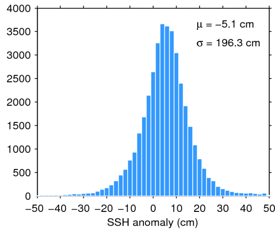
Figure 7. Histogram of flag-valid SSH anomaly over oceans and lakes for 01/04/2018. The mean ( \mu ) and standard deviation ( \sigma ) are also shown. Note that values outside [-50 50] cm are excluded from the histogram for the sake of readability but not from the computation of \mu and \sigma .
