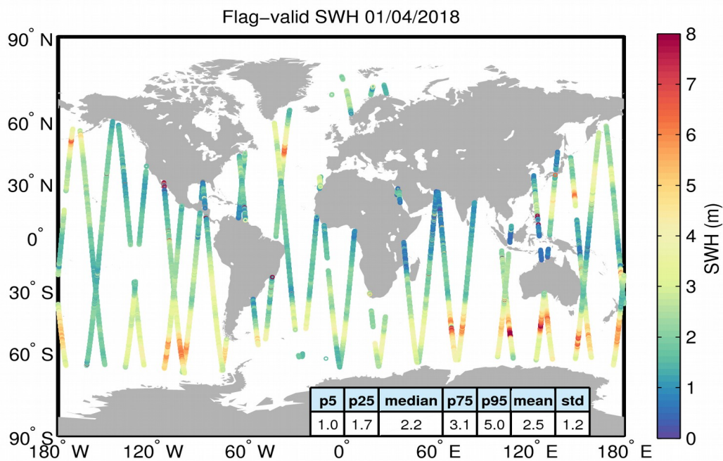
Figure 15. Geographical distribution of flag-valid SWH data over oceans and lakes for 01/04/2018. The statistical values shown in the table refer to the SWH in m and are calculated over all measurements shown in the figure.
