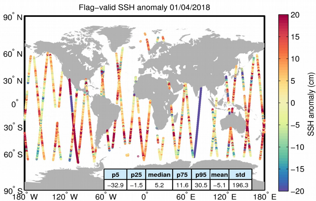
Figure 5. Geographical distribution of flag-valid 1-Hz SSH anomaly data over oceans and lakes for 01/04/2018. The statistical values shown in the table refer to the SSH anomaly in cm and are calculated over all measurements shown in the figure.
