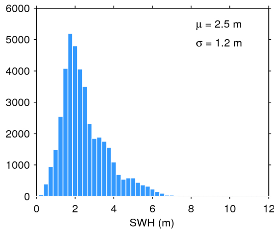
Figure 20. Histogram of science-valid SWH over oceans and lakes for 01/04/2018. The mean ( \mu ) and standard deviation ( \sigma ) are also shown. Note that values larger than 12 m are excluded from the histogram for the sake of readability but not from the computation of \mu and \sigma .
