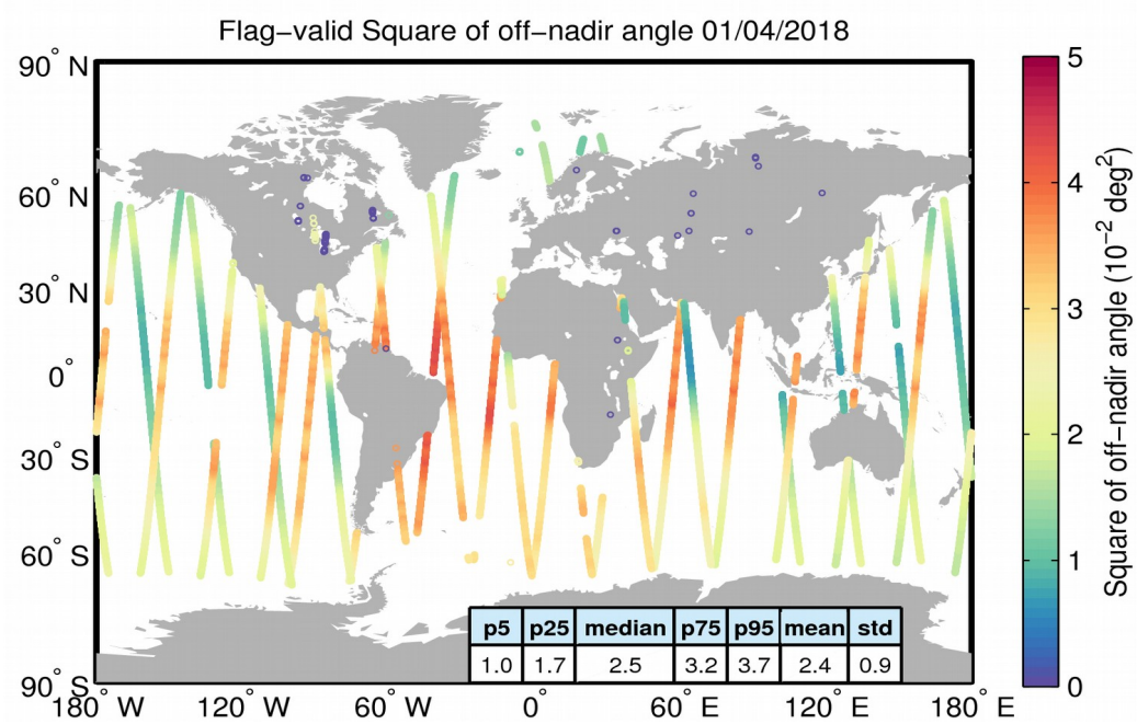
Figure 37. Geographical distribution of flag-valid mispointing data over oceans and lakes for 01/04/2018. The statistical values shown in the table refer to the mispointing in 10^{-2} \text{ deg}^2 and are calculated over all measurements shown in the figure.
