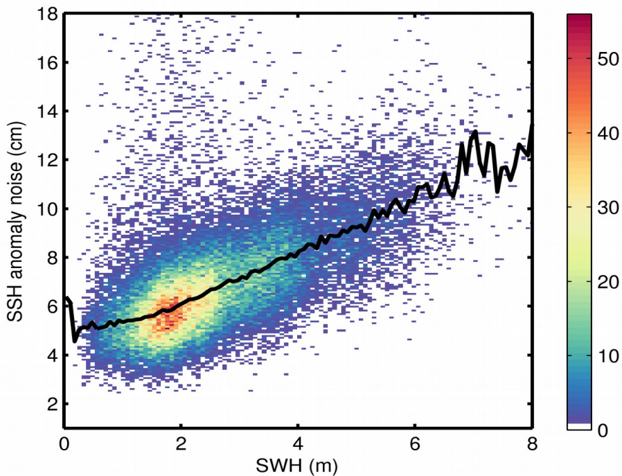
Figure 9. 2D histogram showing flag-valid SSH anomaly noise as a function of SWH for 01/04/2018. The black line denotes the median SSH anomaly noise as a function of SWH.
