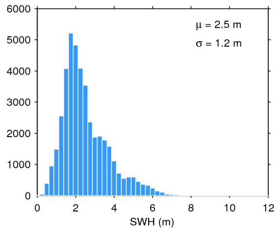
Figure 17. Histogram of flag-valid SWH over oceans and lakes for 01/04/2018. The mean ( \mu ) and standard deviation ( \sigma ) are also shown. Note that values larger than 12 m are excluded from the histogram for the sake of readability but not from the computation of \mu and \sigma .
