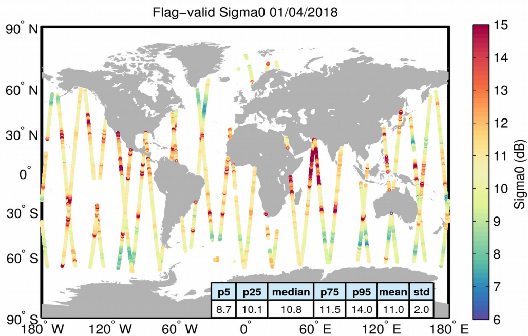
Figure 23. Geographical distribution of flag-valid sigma0 data over oceans and lakes for 01/04/2018. The statistical values shown in the table refer to the sigma0 in dB and are calculated over all measurements shown in the figure.
