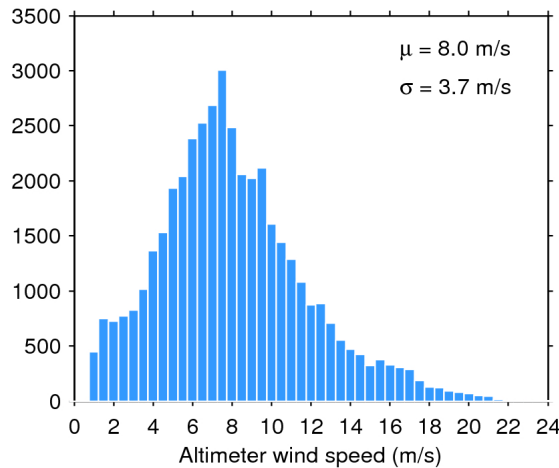
Figure 33. Histogram of flag-valid wind over oceans and lakes for 01/04/2018. The mean ( \mu ) and standard deviation ( \sigma ) are also shown. Note that values larger than 24 m/s are excluded from the histogram for the sake of readability but not from the computation of \mu and \sigma .
