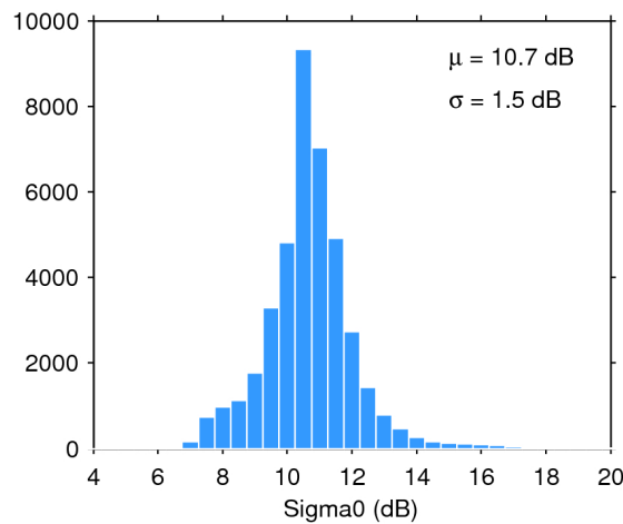
Figure 28. Histogram of science-valid sigma0 over oceans and lakes for 18/03/2018. The mean ( \mu ) and standard deviation ( \sigma ) are also shown. Note that values outside [4 20] dB are excluded from the histogram for the sake of readability but not from the computation of \mu and \sigma .
