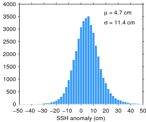
Figure 11. Histogram of science-valid SSH anomaly over oceans and lakes for 18/03/2018. The mean ( \mu ) and standard deviation ( \sigma ) are also shown. Note that values outside [-50 50] cm are excluded from the histogram for the sake of readability but not from the computation of \mu and \sigma .
