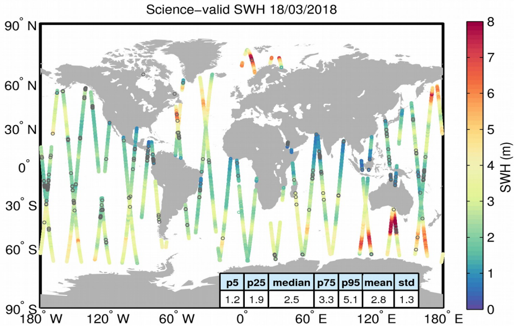
Figure 19. Geographical distribution of science-valid SWH data over oceans and lakes for 18/03/2018. The statistical values shown in the table refer to the SWH in m and are calculated over all measurements shown in the figure. Gray circles denote records that have been rejected based on the editing criteria described in Table 3.
