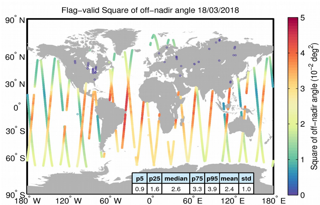
Figure 37. Geographical distribution of flag-valid mispointing data over oceans and lakes for 18/03/2018. The statistical values shown in the table refer to the mispointing in 10^{-2} \text{ deg}^2 and are calculated over all measurements shown in the figure.
