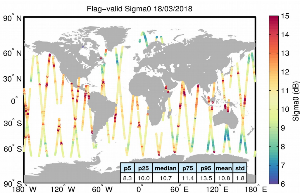
Figure 23. Geographical distribution of flag-valid sigma0 data over oceans and lakes for 18/03/2018. The statistical values shown in the table refer to the sigma0 in dB and are calculated over all measurements shown in the figure.
