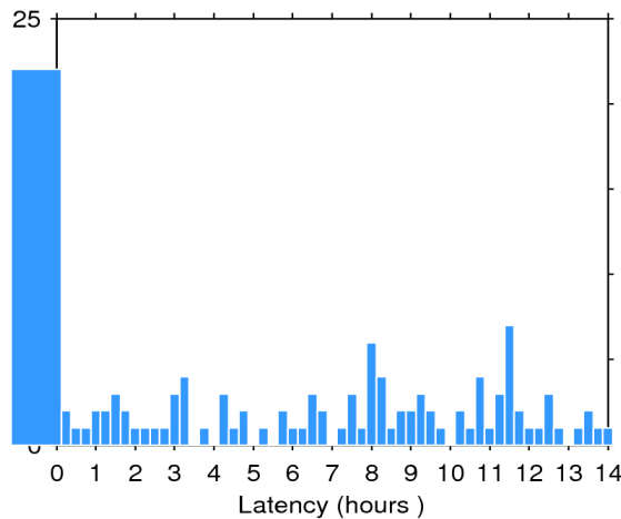
Figure 2. Histogram of the data latency for 18/03/2018. The y-axis denotes the number of files that are made available with a delay of x-hours with respect to the mean time of the records stored in the file.
