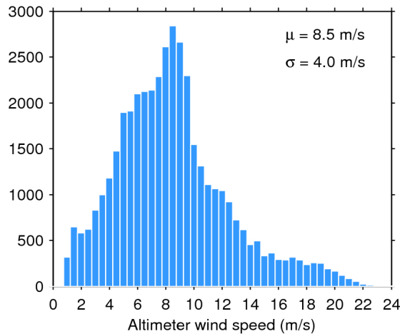
Figure 33. Histogram of flag-valid wind over oceans and lakes for 18/03/2018. The mean ( \mu ) and standard deviation ( \sigma ) are also shown. Note that values larger than 24 m/s are excluded from the histogram for the sake of readability but not from the computation of \mu and \sigma .
