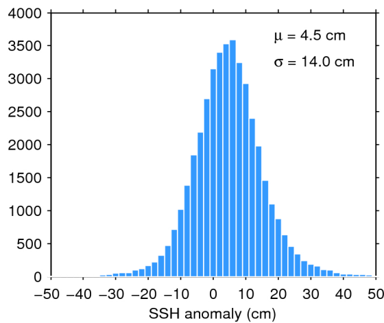
Figure 7. Histogram of flag-valid SSH anomaly over oceans and lakes for 18/03/2018. The mean ( \mu ) and standard deviation ( \sigma ) are also shown. Note that values outside [-50 50] cm are excluded from the histogram for the sake of readability but not from the computation of \mu and \sigma .
