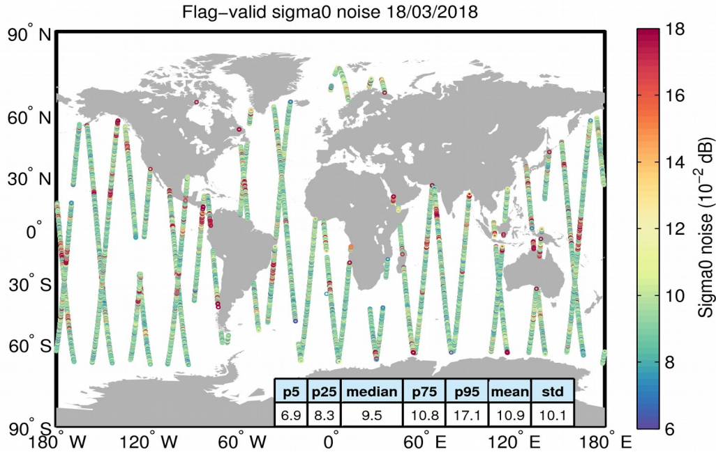
Figure 26. Geographical distribution of flag-valid 20-Hz sigma0 measurement noise over oceans and lakes for 18/03/2018. The statistical values shown in the table refer to the sigma0 noise and are calculated over all measurements shown in the figure.
