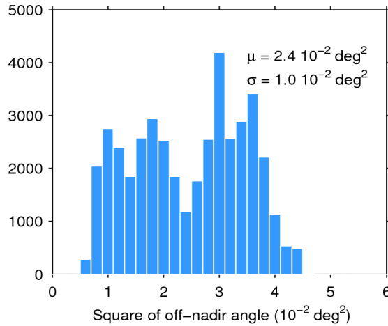
Figure 39. Histogram of flag-valid mispointing over oceans and lakes for 18/03/2018. The mean ( \mu ) and standard deviation ( \sigma ) are also shown. Note that values larger than 6 \cdot 10^{-2} \text{ deg}^2 are excluded from the histogram for the sake of readability but not from the computation of \mu and \sigma .
