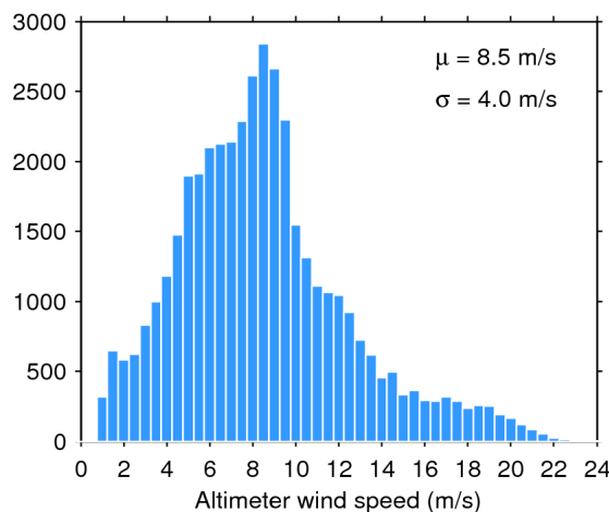
Figure 35. Histogram of science-valid wind over oceans and lakes for 18/03/2018. The mean ( \mu ) and standard deviation ( \sigma ) are also shown. Note that values larger than 24 m/s are excluded from the histogram for the sake of readability but not from the computation of \mu and \sigma .
