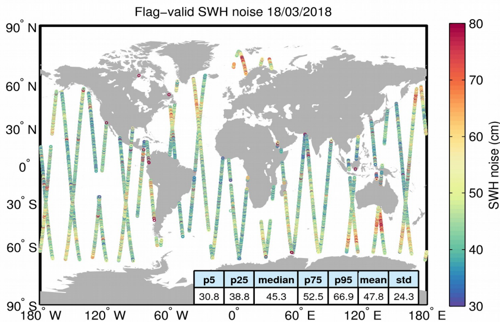
Figure 18. Geographical distribution of flag-valid 20-Hz SWH measurement noise over oceans and lakes for 18/03/2018. The statistical values shown in the figure refer to the SWH noise and are calculated over all measurements shown in the figure.
