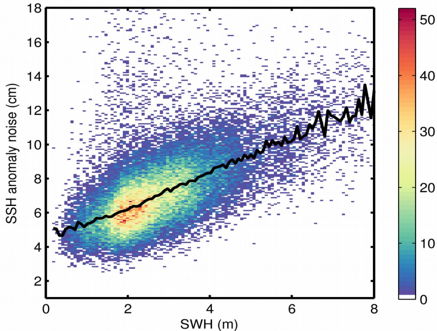
Figure 9. 2D histogram showing flag-valid SSH anomaly noise as a function of SWH for 18/03/2018. The black line denotes the median SSH anomaly noise as a function of SWH.
