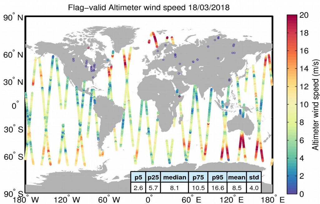
Figure 31. Geographical distribution of flag-valid wind data over oceans and lakes for 18/03/2018. The statistical values shown in the table refer to the wind in m/s and are calculated over all measurements shown in the figure.
