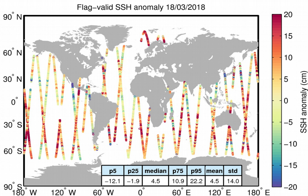
Figure 5. Geographical distribution of flag-valid 1-Hz SSH anomaly data over oceans and lakes for 18/03/2018. The statistical values shown in the table refer to the SSH anomaly in cm and are calculated over all measurements shown in the figure.
