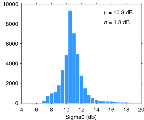
Figure 25. Histogram of flag-valid sigma0 over oceans and lakes for 18/03/2018. The mean ( \mu ) and standard deviation ( \sigma ) are also shown. Note that values outside [4 20] dB are excluded from the histogram for the sake of readability but not from the computation of \mu and \sigma .
