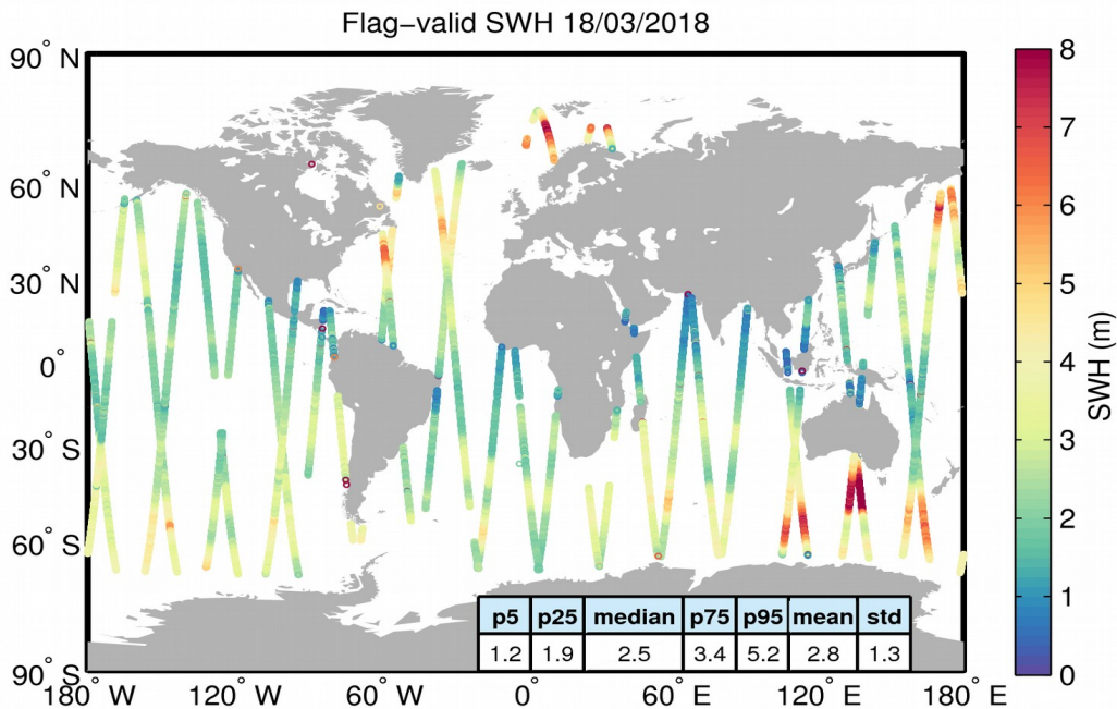
Figure 15. Geographical distribution of flag-valid SWH data over oceans and lakes for 18/03/2018. The statistical values shown in the table refer to the SWH in m and are calculated over all measurements shown in the figure.
