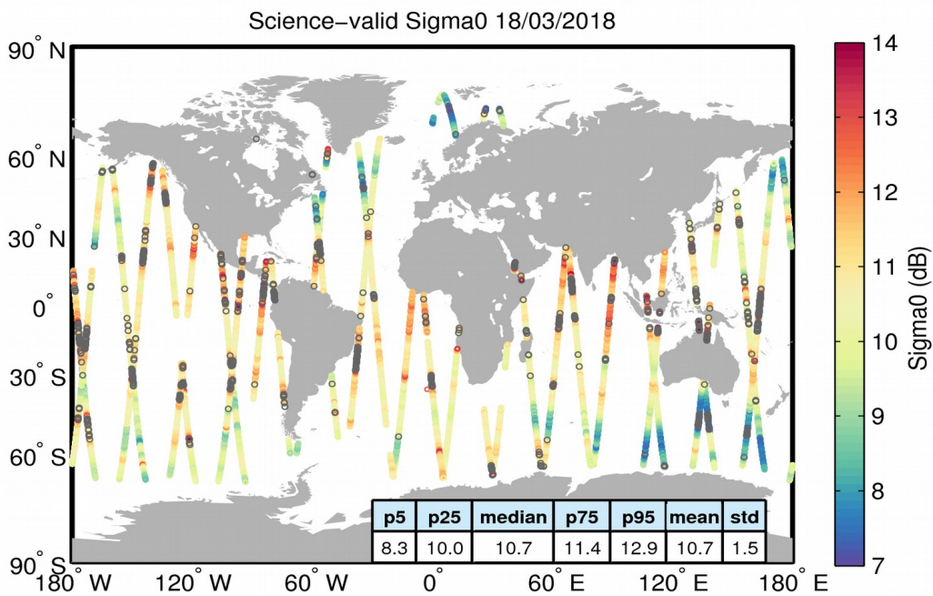
Figure 27. Geographical distribution of science-valid sigma0 data over oceans and lakes for 18/03/2018. The statistical values shown in the table refer to the sigma0 in dB and are calculated over all measurements shown in the figure. Gray circles denote records that have been rejected based on the editing criteria described in Table 4.
