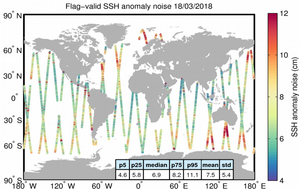
Figure 8. Geographical distribution of flag-valid 20-Hz SSH anomaly measurement noise over oceans and lakes for 18/03/2018. The statistical values shown in the table refer to the SSH anomaly noise and are calculated over all measurements shown in the figure.
