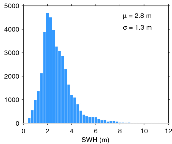
Figure 17. Histogram of flag-valid SWH over oceans and lakes for 18/03/2018. The mean ( \mu ) and standard deviation ( \sigma ) are also shown. Note that values larger than 12 m are excluded from the histogram for the sake of readability but not from the computation of \mu and \sigma .
