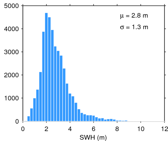
Figure 20. Histogram of science-valid SWH over oceans and lakes for 18/03/2018. The mean ( \mu ) and standard deviation ( \sigma ) are also shown. Note that values larger than 12 m are excluded from the histogram for the sake of readability but not from the computation of \mu and \sigma .
