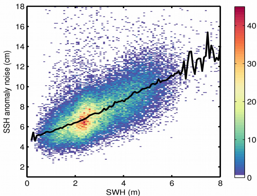
Figure 9. 2D histogram showing flag-valid SSH anomaly noise as a function of SWH for 16/03/2018. The black line denotes the median SSH anomaly noise as a function of SWH.
