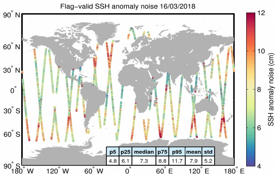
Figure 8. Geographical distribution of flag-valid 20-Hz SSH anomaly measurement noise over oceans and lakes for 16/03/2018. The statistical values shown in the table refer to the SSH anomaly noise and are calculated over all measurements shown in the figure.
