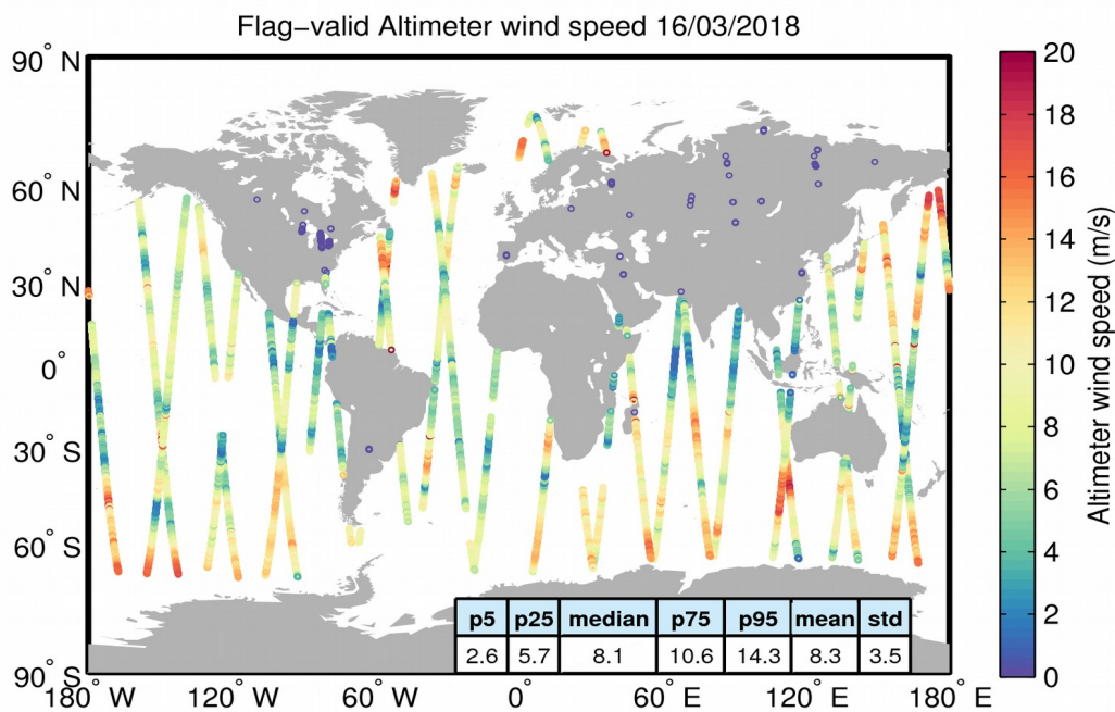
Figure 31. Geographical distribution of flag-valid wind data over oceans and lakes for 16/03/2018. The statistical values shown in the table refer to the wind in m/s and are calculated over all measurements shown in the figure.
