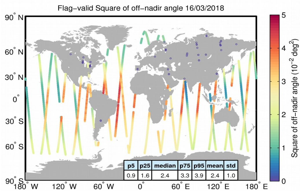
Figure 37. Geographical distribution of flag-valid mispointing data over oceans and lakes for 16/03/2018. The statistical values shown in the table refer to the mispointing in 10^{-2} \text{ deg}^2 and are calculated over all measurements shown in the figure.
