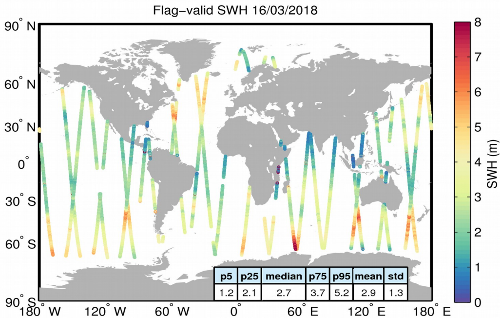
Figure 15. Geographical distribution of flag-valid SWH data over oceans and lakes for 16/03/2018. The statistical values shown in the table refer to the SWH in m and are calculated over all measurements shown in the figure.
