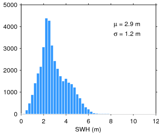
Figure 20. Histogram of science-valid SWH over oceans and lakes for 16/03/2018. The mean ( \mu ) and standard deviation ( \sigma ) are also shown. Note that values larger than 12 m are excluded from the histogram for the sake of readability but not from the computation of \mu and \sigma .
