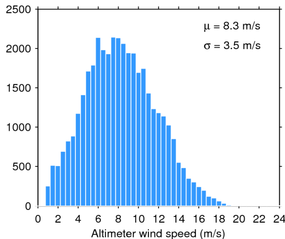
Figure 35. Histogram of science-valid wind over oceans and lakes for 16/03/2018. The mean ( \mu ) and standard deviation ( \sigma ) are also shown. Note that values larger than 24 m/s are excluded from the histogram for the sake of readability but not from the computation of \mu and \sigma .
