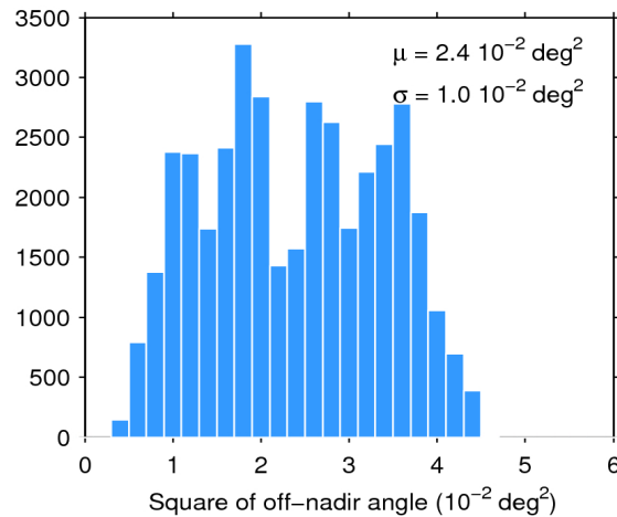
Figure 39. Histogram of flag-valid mispointing over oceans and lakes for 16/03/2018. The mean ( \mu ) and standard deviation ( \sigma ) are also shown. Note that values larger than 6 \cdot 10^{-2} \text{ deg}^2 are excluded from the histogram for the sake of readability but not from the computation of \mu and \sigma .
