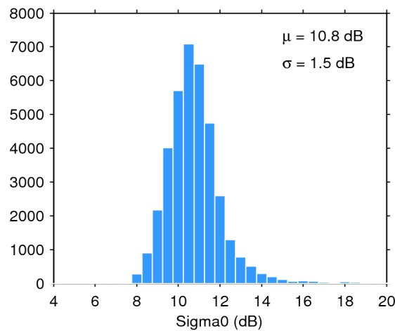
Figure 28. Histogram of science-valid sigma0 over oceans and lakes for 16/03/2018. The mean ( \mu ) and standard deviation ( \sigma ) are also shown. Note that values outside [4 20] dB are excluded from the histogram for the sake of readability but not from the computation of \mu and \sigma .
