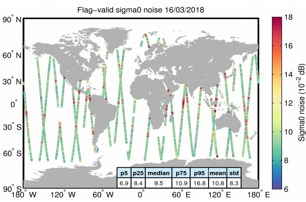
Figure 26. Geographical distribution of flag-valid 20-Hz sigma0 measurement noise over oceans and lakes for 16/03/2018. The statistical values shown in the table refer to the sigma0 noise and are calculated over all measurements shown in the figure.
