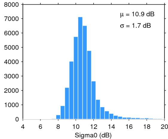
Figure 25. Histogram of flag-valid sigma0 over oceans and lakes for 16/03/2018. The mean ( \mu ) and standard deviation ( \sigma ) are also shown. Note that values outside [4 20] dB are excluded from the histogram for the sake of readability but not from the computation of \mu and \sigma .
