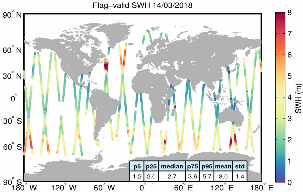
Figure 15. Geographical distribution of flag-valid SWH data over oceans and lakes for 14/03/2018. The statistical values shown in the table refer to the SWH in m and are calculated over all measurements shown in the figure.
