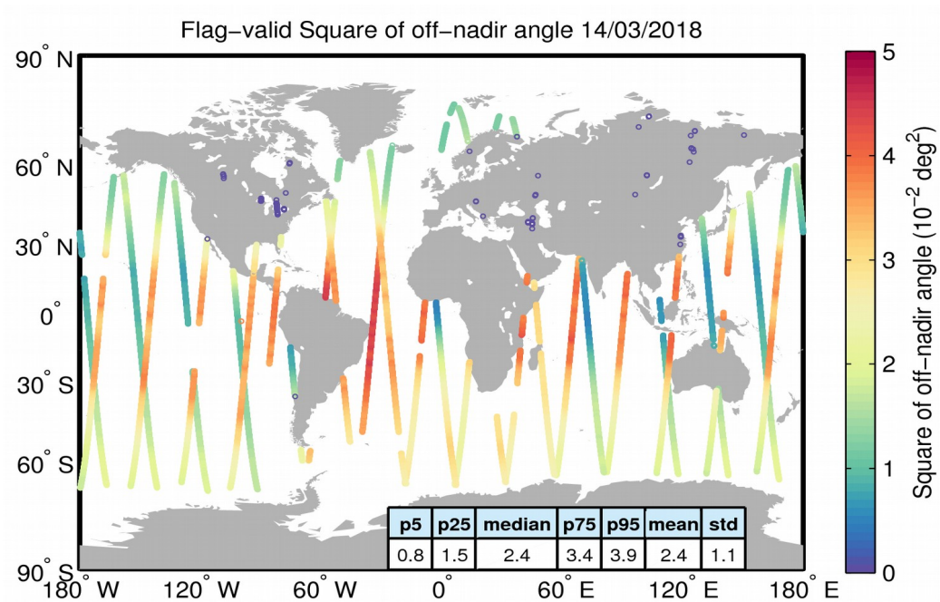
Figure 37. Geographical distribution of flag-valid mispointing data over oceans and lakes for 14/03/2018. The statistical values shown in the table refer to the mispointing in 10^{-2} deg 2 and are calculated over all measurements shown in the figure.
