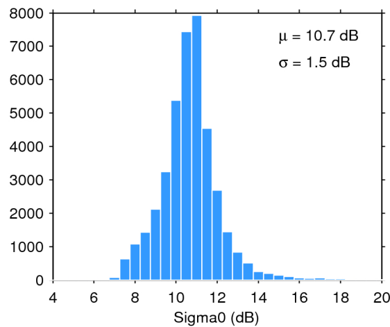
Figure 28. Histogram of science-valid sigma0 over oceans and lakes for 14/03/2018. The mean ( \mu ) and standard deviation ( \sigma ) are also shown. Note that values outside [4 20] dB are excluded from the histogram for the sake of readability but not from the computation of \mu and \sigma .
