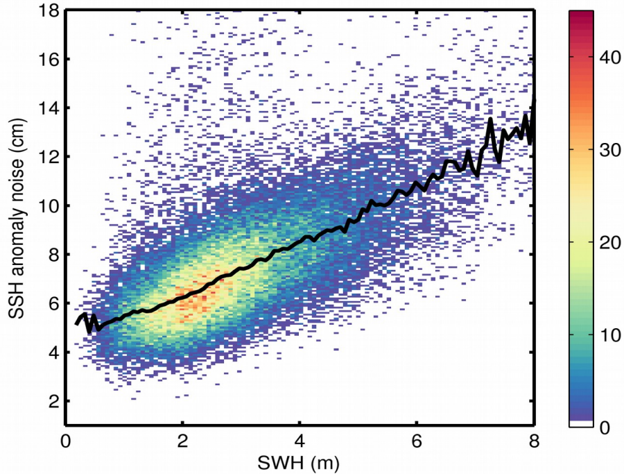
Figure 9. 2D histogram showing flag-valid SSH anomaly noise as a function of SWH for 14/03/2018. The black line denotes the median SSH anomaly noise as a function of SWH.
