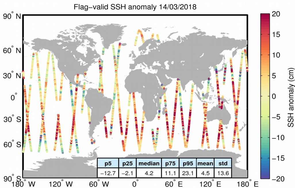
Figure 5. Geographical distribution of flag-valid 1-Hz SSH anomaly data over oceans and lakes for 14/03/2018. The statistical values shown in the table refer to the SSH anomaly in cm and are calculated over all measurements shown in the figure.
