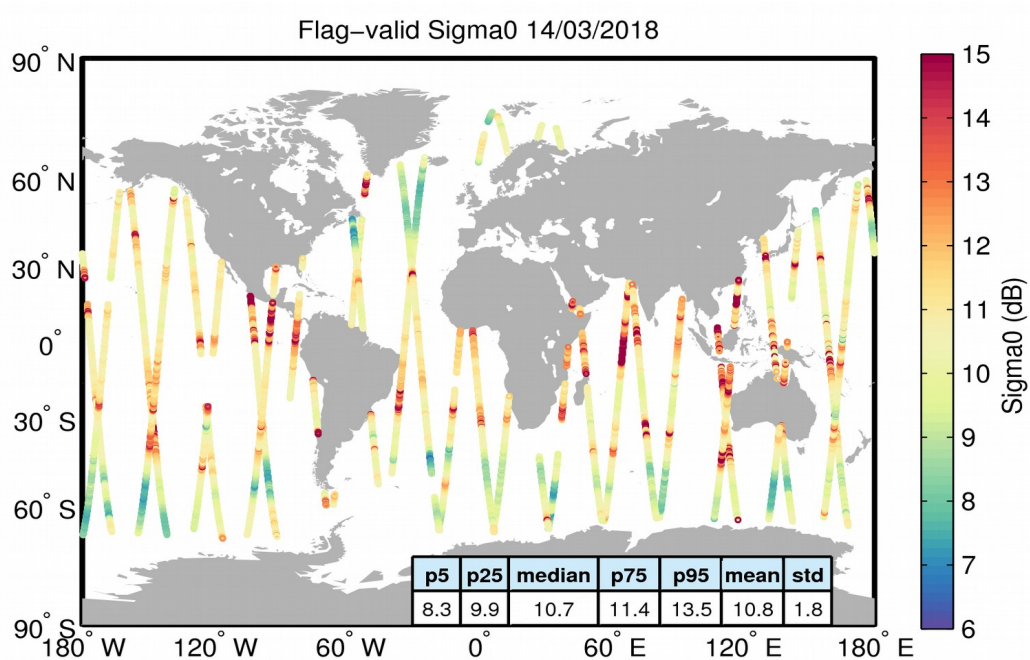
Figure 23. Geographical distribution of flag-valid sigma0 data over oceans and lakes for 14/03/2018. The statistical values shown in the table refer to the sigma0 in dB and are calculated over all measurements shown in the figure.
