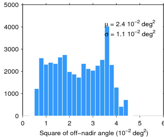
Figure 39. Histogram of flag-valid mispointing over oceans and lakes for 14/03/2018. The mean ( \mu ) and standard deviation ( \sigma ) are also shown. Note that values larger than 6 \cdot 10^{-2} \text{ deg}^2 are excluded from the histogram for the sake of readability but not from the computation of \mu and \sigma .
