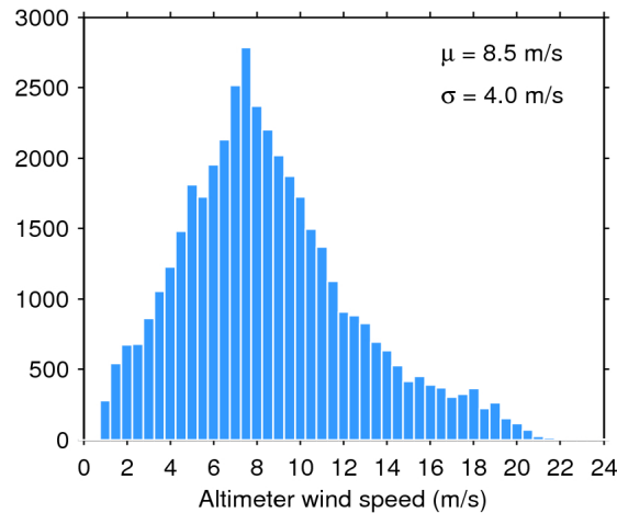
Figure 33. Histogram of flag-valid wind over oceans and lakes for 14/03/2018. The mean ( \mu ) and standard deviation ( \sigma ) are also shown. Note that values larger than 24 m/s are excluded from the histogram for the sake of readability but not from the computation of \mu and \sigma .
