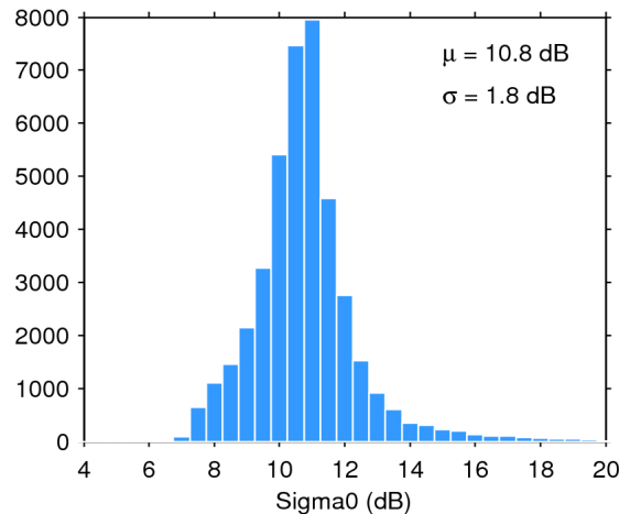
Figure 25. Histogram of flag-valid sigma0 over oceans and lakes for 14/03/2018. The mean ( \mu ) and standard deviation ( \sigma ) are also shown. Note that values outside [4 20] dB are excluded from the histogram for the sake of readability but not from the computation of \mu and \sigma .
