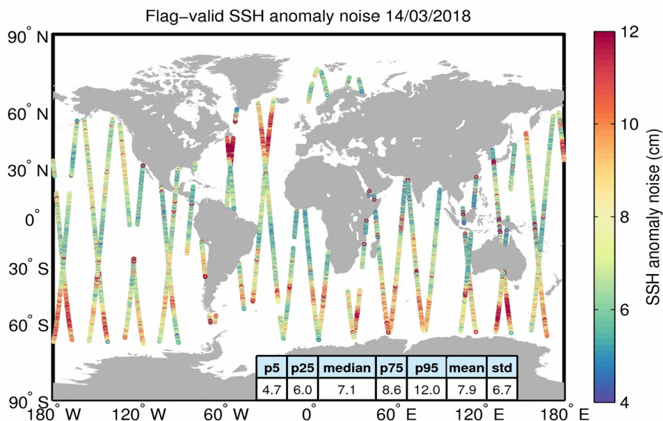
Figure 8. Geographical distribution of flag-valid 20-Hz SSH anomaly measurement noise over oceans and lakes for 14/03/2018. The statistical values shown in the table refer to the SSH anomaly noise and are calculated over all measurements shown in the figure.
