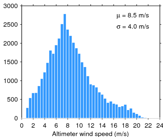
Figure 35. Histogram of science-valid wind over oceans and lakes for 14/03/2018. The mean ( \mu ) and standard deviation ( \sigma ) are also shown. Note that values larger than 24 m/s are excluded from the histogram for the sake of readability but not from the computation of \mu and \sigma .
