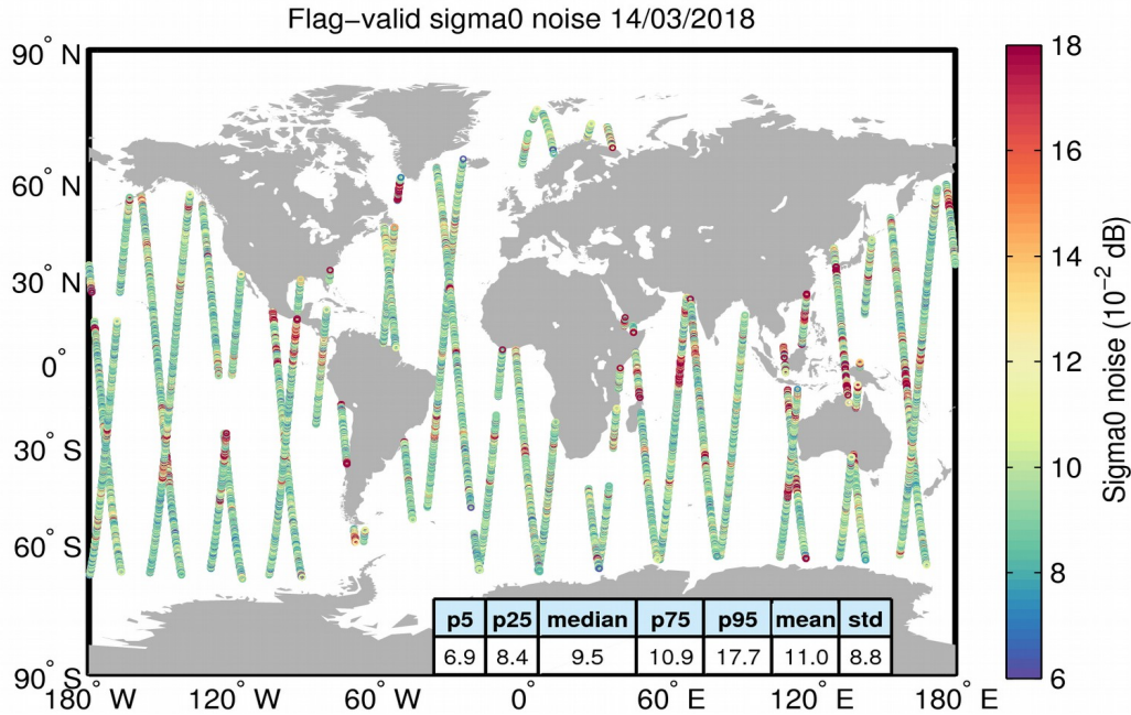
Figure 26. Geographical distribution of flag-valid 20-Hz sigma0 measurement noise over oceans and lakes for 14/03/2018. The statistical values shown in the table refer to the sigma0 noise and are calculated over all measurements shown in the figure.
