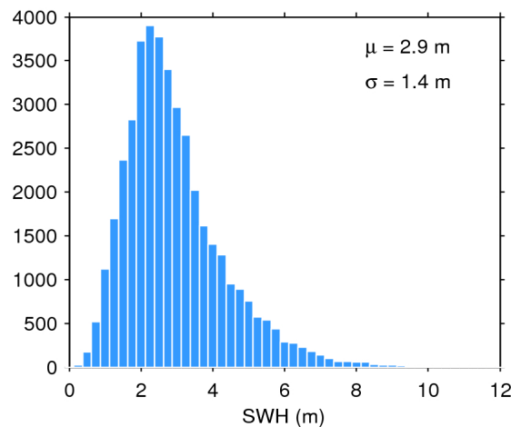
Figure 20. Histogram of science-valid SWH over oceans and lakes for 14/03/2018. The mean ( \mu ) and standard deviation ( \sigma ) are also shown. Note that values larger than 12 m are excluded from the histogram for the sake of readability but not from the computation of \mu and \sigma .
