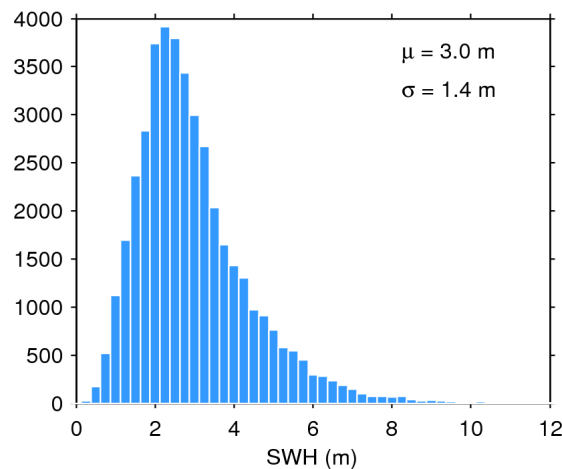
Figure 17. Histogram of flag-valid SWH over oceans and lakes for 14/03/2018. The mean ( \mu ) and standard deviation ( \sigma ) are also shown. Note that values larger than 12 m are excluded from the histogram for the sake of readability but not from the computation of \mu and \sigma .
