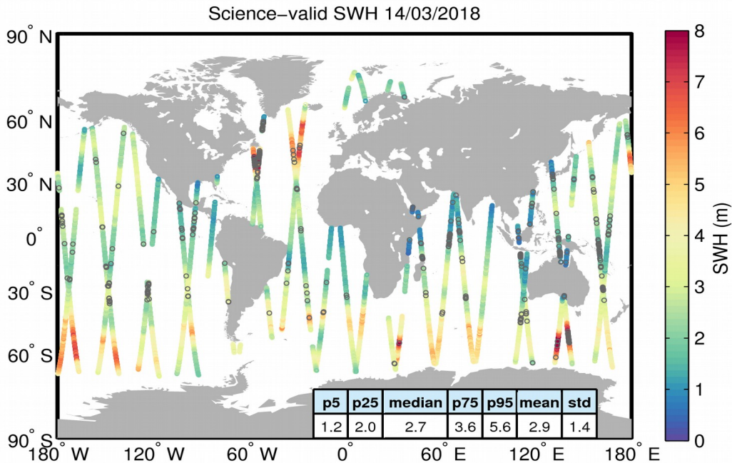
Figure 19. Geographical distribution of science-valid SWH data over oceans and lakes for 14/03/2018. The statistical values shown in the table refer to the SWH in m and are calculated over all measurements shown in the figure. Gray circles denote records that have been rejected based on the editing criteria described in Table 3.
