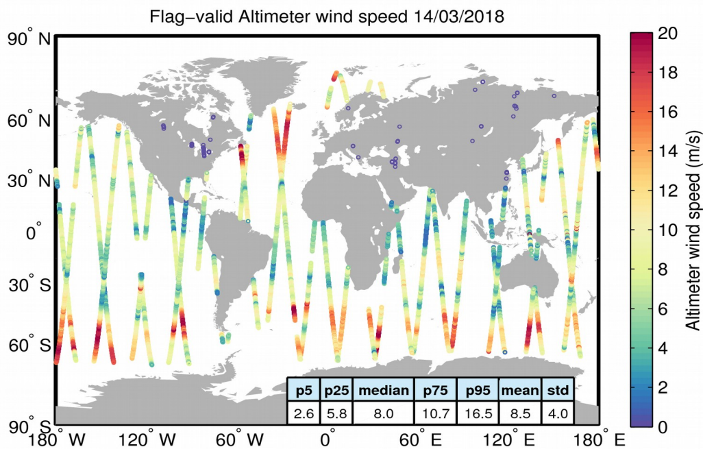
Figure 31. Geographical distribution of flag-valid wind data over oceans and lakes for 14/03/2018. The statistical values shown in the table refer to the wind in m/s and are calculated over all measurements shown in the figure.
