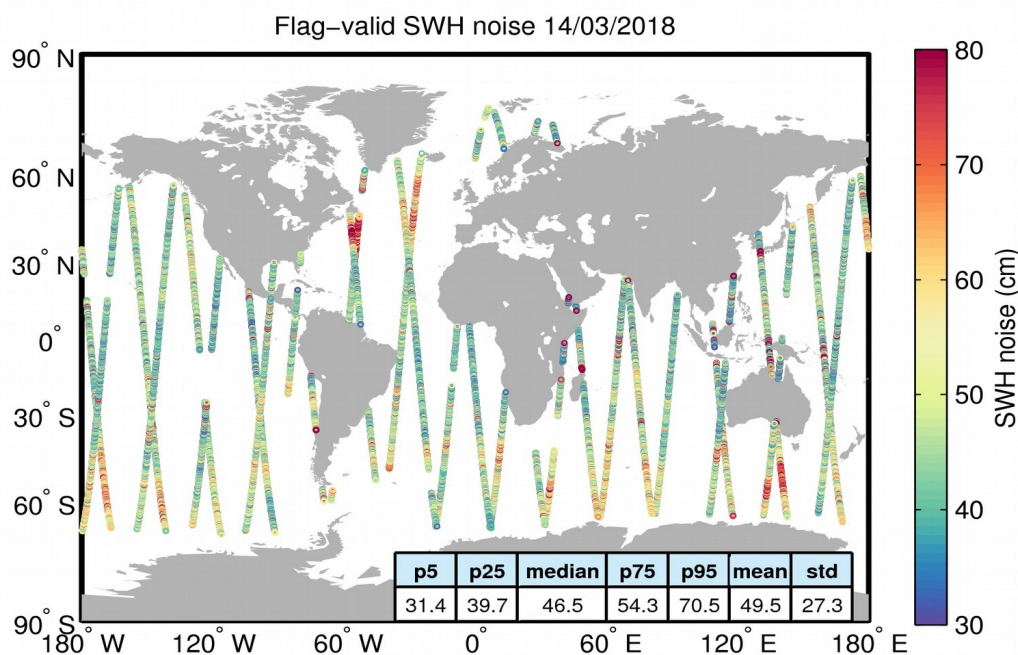
Figure 18. Geographical distribution of flag-valid 20-Hz SWH measurement noise over oceans and lakes for 14/03/2018. The statistical values shown in the figure refer to the SWH noise and are calculated over all measurements shown in the figure.
