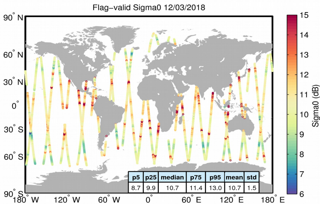
Figure 23. Geographical distribution of flag-valid sigma0 data over oceans and lakes for 12/03/2018. The statistical values shown in the table refer to the sigma0 in dB and are calculated over all measurements shown in the figure.
