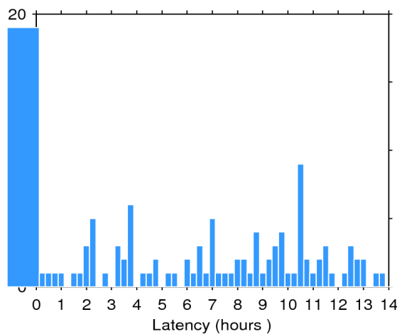
Figure 2. Histogram of the data latency for 09/03/2018. The y-axis denotes the number of files that are made available with a delay of x-hours with respect to the mean time of the records stored in the file.
