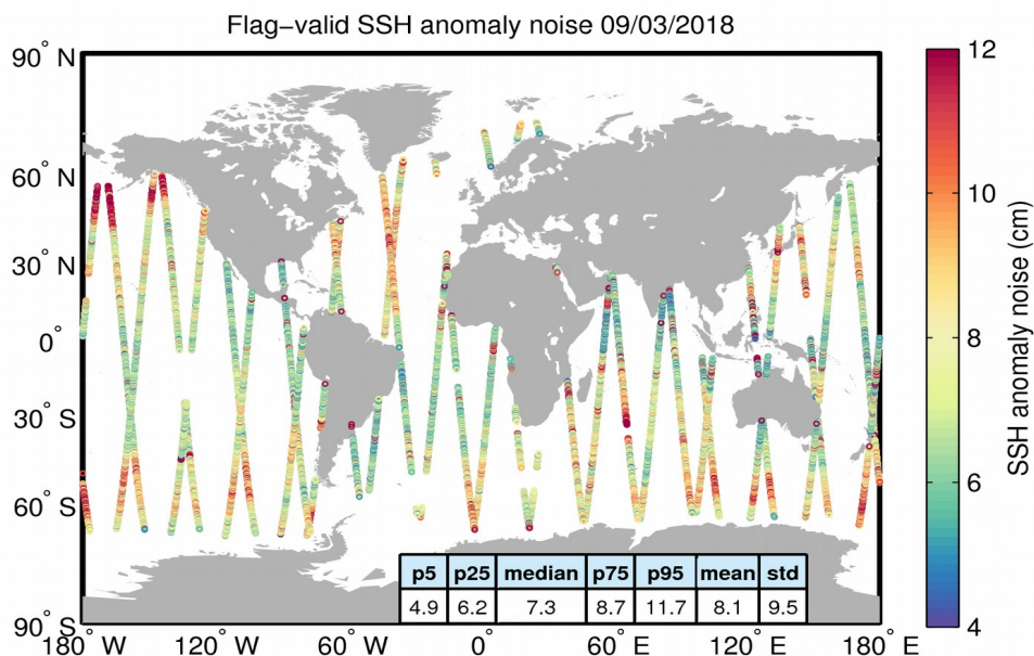
Figure 8. Geographical distribution of flag-valid 20-Hz SSH anomaly measurement noise over oceans and lakes for 09/03/2018. The statistical values shown in the table refer to the SSH anomaly noise and are calculated over all measurements shown in the figure.
