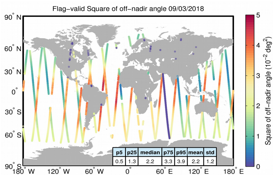
Figure 37. Geographical distribution of flag-valid mispointing data over oceans and lakes for 09/03/2018. The statistical values shown in the table refer to the mispointing in 10^{-2} \text{ deg}^2 and are calculated over all measurements shown in the figure.
