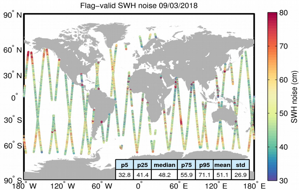
Figure 18. Geographical distribution of flag-valid 20-Hz SWH measurement noise over oceans and lakes for 09/03/2018. The statistical values shown in the table refer to the SWH noise and are calculated over all measurements shown in the figure.
