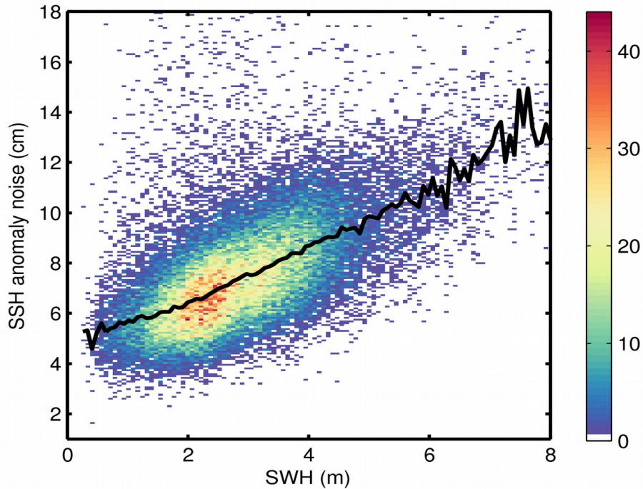
Figure 9. 2D histogram showing flag-valid SSH anomaly noise as a function of SWH for 09/03/2018. The black line denotes the median SSH anomaly noise as a function of SWH.
