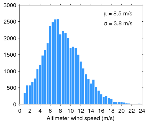
Figure 35. Histogram of science-valid wind over oceans and lakes for 09/03/2018. The mean ( \mu ) and standard deviation ( \sigma ) are also shown. Note that values larger than 24 m/s are excluded from the histogram for the sake of readability but not from the computation of \mu and \sigma .
