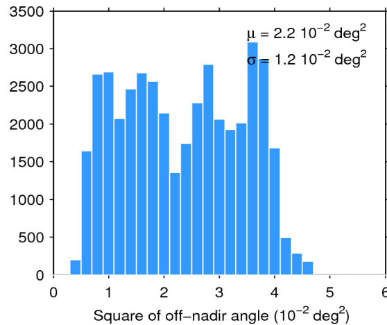
Figure 39. Histogram of flag-valid mispointing over oceans and lakes for 09/03/2018. The mean ( \mu ) and standard deviation ( \sigma ) are also shown. Note that values larger than 6 \cdot 10^{-2} \text{ deg}^2 are excluded from the histogram for the sake of readability but not from the computation of \mu and \sigma .
