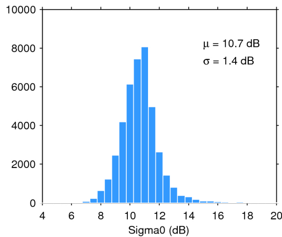
Figure 28. Histogram of science-valid sigma0 over oceans and lakes for 09/03/2018. The mean ( \mu ) and standard deviation ( \sigma ) are also shown. Note that values outside [4 20] dB are excluded from the histogram for the sake of readability but not from the computation of \mu and \sigma .
