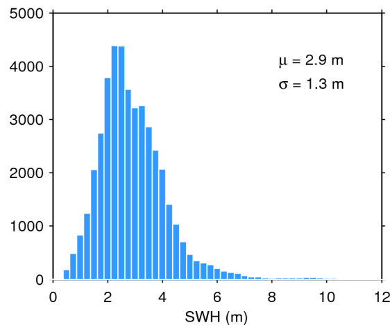
Figure 17. Histogram of flag-valid SWH over oceans and lakes for 09/03/2018. The mean ( \mu ) and standard deviation ( \sigma ) are also shown. Note that values larger than 12 m are excluded from the histogram for the sake of readability but not from the computation of \mu and \sigma .
