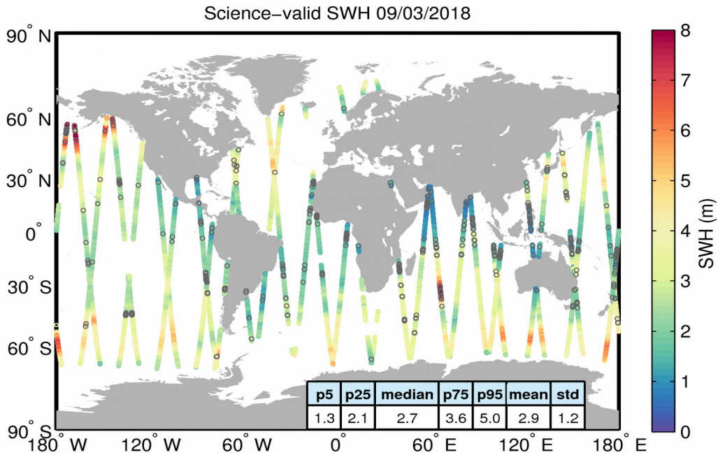
Figure 19. Geographical distribution of science-valid SWH data over oceans and lakes for 09/03/2018. The statistical values shown in the table refer to the SWH in m and are calculated over all measurements shown in the figure. Gray circles denote records that have been rejected based on the editing criteria described in Table 3.
