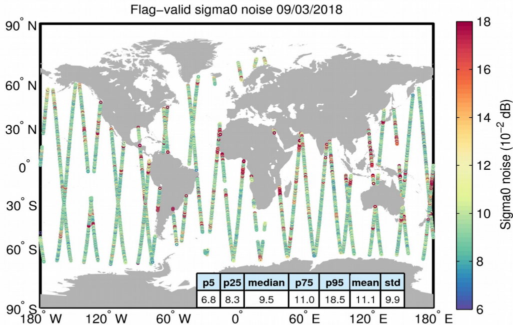
Figure 26. Geographical distribution of flag-valid 20-Hz sigma0 measurement noise over oceans and lakes for 09/03/2018. The statistical values shown in the table refer to the sigma0 noise and are calculated over all measurements shown in the figure.
