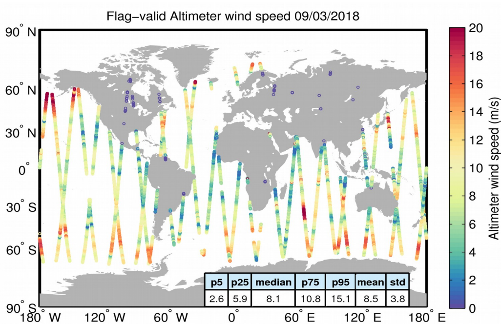
Figure 31. Geographical distribution of flag-valid wind data over oceans and lakes for 09/03/2018. The statistical values shown in the table refer to the wind in m/s and are calculated over all measurements shown in the figure.
