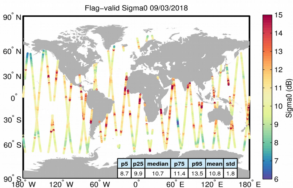
Figure 23. Geographical distribution of flag-valid sigma0 data over oceans and lakes for 09/03/2018. The statistical values shown in the table refer to the sigma0 in dB and are calculated over all measurements shown in the figure.
