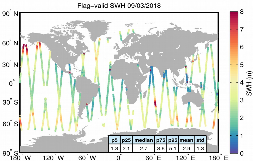
Figure 15. Geographical distribution of flag-valid SWH data over oceans and lakes for 09/03/2018. The statistical values shown in the table refer to the SWH in m and are calculated over all measurements shown in the figure.
