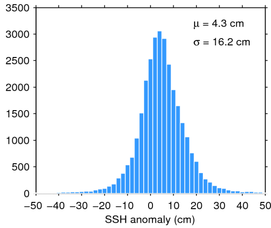
Figure 11. Histogram of science-valid SSH anomaly over oceans and lakes for 09/03/2018. The mean ( \mu ) and standard deviation ( \sigma ) are also shown. Note that values outside [-50 50] cm are excluded from the histogram for the sake of readability but not from the computation of \mu and \sigma .
