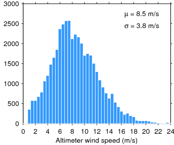
Figure 33. Histogram of flag-valid wind over oceans and lakes for 09/03/2018. The mean ( \mu ) and standard deviation ( \sigma ) are also shown. Note that values larger than 24 m/s are excluded from the histogram for the sake of readability but not from the computation of \mu and \sigma .
