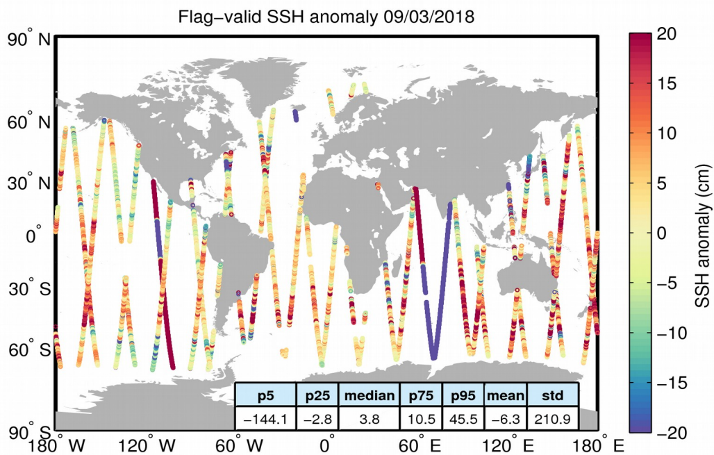
Figure 5. Geographical distribution of flag-valid 1-Hz SSH anomaly data over oceans and lakes for 09/03/2018. The statistical values shown in the table refer to the SSH anomaly in cm and are calculated over all measurements shown in the figure.
