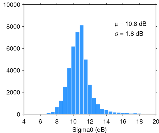
Figure 25. Histogram of flag-valid sigma0 over oceans and lakes for 09/03/2018. The mean ( \mu ) and standard deviation ( \sigma ) are also shown. Note that values outside [4 20] dB are excluded from the histogram for the sake of readability but not from the computation of \mu and \sigma .
