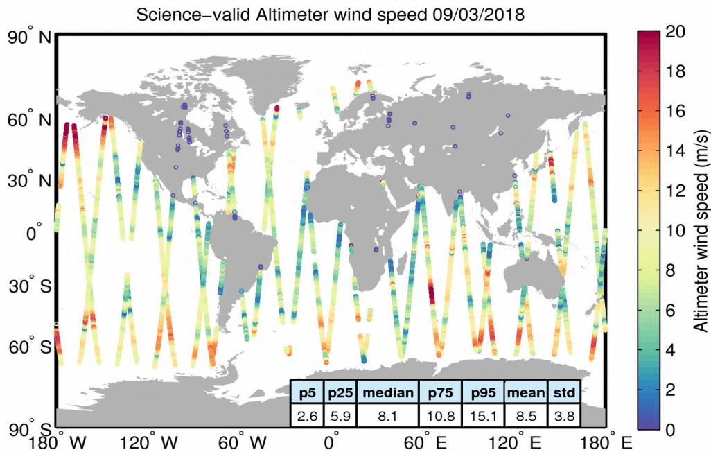
Figure 34. Geographical distribution of science-valid wind data over oceans and lakes for 09/03/2018. The statistical values shown in the table refer to the wind in m/s and are calculated over all measurements shown in the figure. Gray circles denote records that have been rejected based on the editing criteria described in Table 5.
