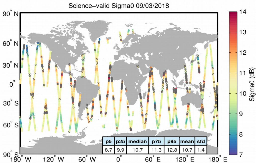
Figure 27. Geographical distribution of science-valid sigma0 data over oceans and lakes for 09/03/2018. The statistical values shown in the table refer to the sigma0 in dB and are calculated over all measurements shown in the figure. Gray circles denote records that have been rejected based on the editing criteria described in Table 4.
