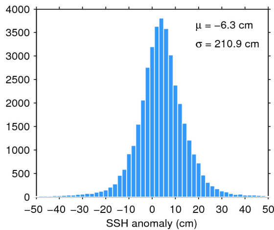
Figure 7. Histogram of flag-valid SSH anomaly over oceans and lakes for 09/03/2018. The mean ( \mu ) and standard deviation ( \sigma ) are also shown. Note that values outside [-50\ 50] cm are excluded from the histogram for the sake of readability but not from the computation of \mu and \sigma .
