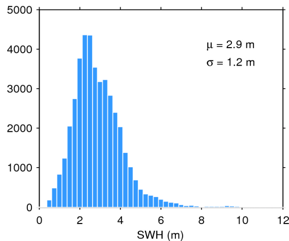
Figure 20. Histogram of science-valid SWH over oceans and lakes for 09/03/2018. The mean ( \mu ) and standard deviation ( \sigma ) are also shown. Note that values larger than 12 m are excluded from the histogram for the sake of readability but not from the computation of \mu and \sigma .
