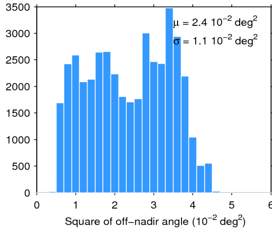
Figure 39. Histogram of flag-valid mispointing over oceans and lakes for 08/03/2018. The mean ( \mu ) and standard deviation ( \sigma ) are also shown. Note that values larger than 6 \cdot 10^{-2} \text{ deg}^2 are excluded from the histogram for the sake of readability but not from the computation of \mu and \sigma .
