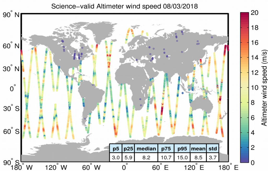
Figure 34. Geographical distribution of science-valid wind data over oceans and lakes for 08/03/2018. The statistical values shown in the table refer to the wind in m/s and are calculated over all measurements shown in the figure. Gray circles denote records that have been rejected based on the editing criteria described in Table 5.
