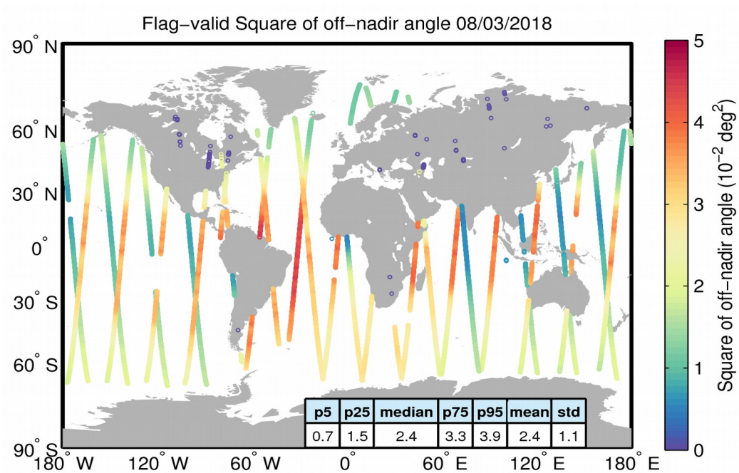
Figure 37. Geographical distribution of flag-valid mispointing data over oceans and lakes for 08/03/2018. The statistical values shown in the table refer to the mispointing in 10^{-2} \text{ deg}^2 and are calculated over all measurements shown in the figure.
