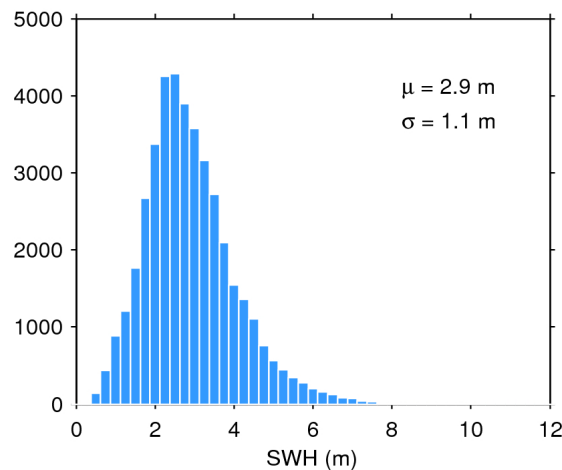
Figure 20. Histogram of science-valid SWH over oceans and lakes for 08/03/2018. The mean ( \mu ) and standard deviation ( \sigma ) are also shown. Note that values larger than 12 m are excluded from the histogram for the sake of readability but not from the computation of \mu and \sigma .
