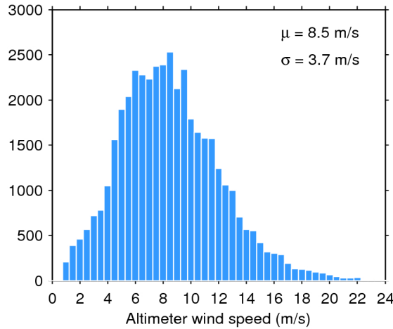
Figure 33. Histogram of flag-valid wind over oceans and lakes for 08/03/2018. The mean ( \mu ) and standard deviation ( \sigma ) are also shown. Note that values larger than 24 m/s are excluded from the histogram for the sake of readability but not from the computation of \mu and \sigma .
