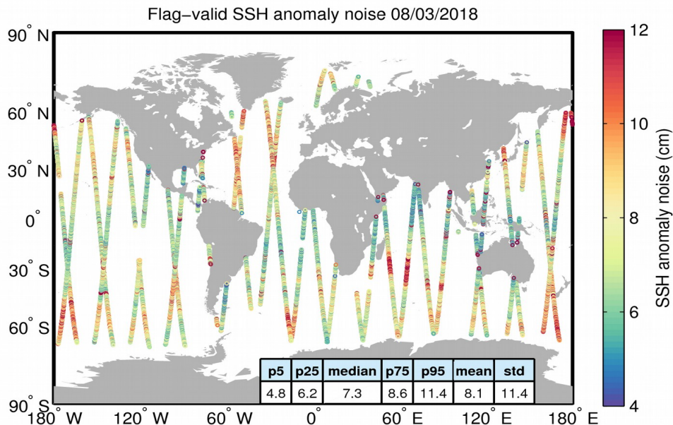
Figure 8. Geographical distribution of flag-valid 20-Hz SSH anomaly measurement noise over oceans and lakes for 08/03/2018. The statistical values shown in the table refer to the SSH anomaly noise and are calculated over all measurements shown in the figure.
