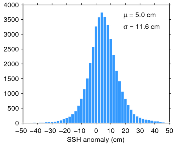
Figure 11. Histogram of science-valid SSH anomaly over oceans and lakes for 08/03/2018. The mean ( \mu ) and standard deviation ( \sigma ) are also shown. Note that values outside [-50 50] cm are excluded from the histogram for the sake of readability but not from the computation of \mu and \sigma .
