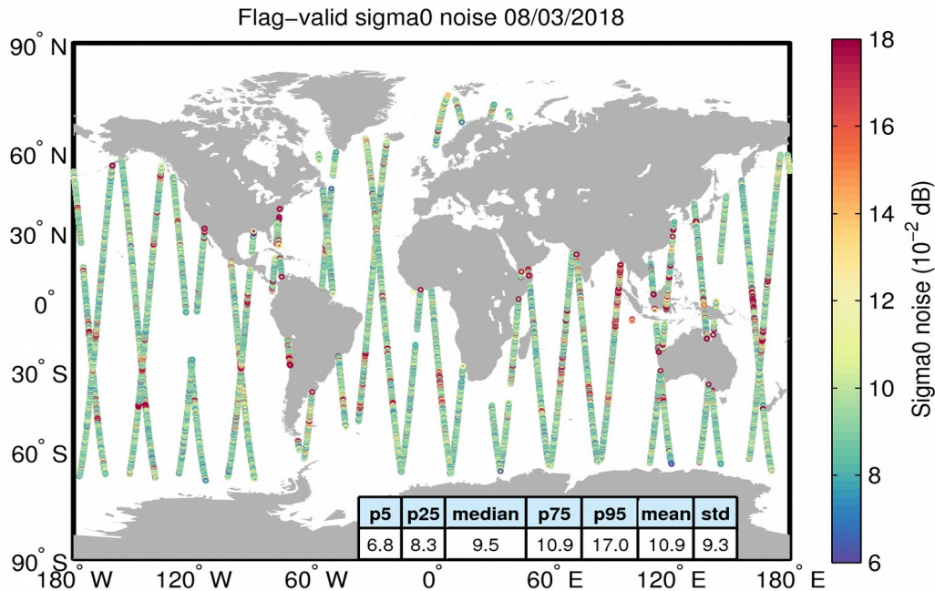
Figure 26. Geographical distribution of flag-valid 20-Hz sigma0 measurement noise over oceans and lakes for 08/03/2018. The statistical values shown in the table refer to the sigma0 noise and are calculated over all measurements shown in the figure.
