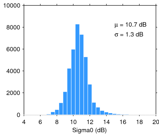
Figure 28. Histogram of science-valid sigma0 over oceans and lakes for 08/03/2018. The mean ( \mu ) and standard deviation ( \sigma ) are also shown. Note that values outside [4 20] dB are excluded from the histogram for the sake of readability but not from the computation of \mu and \sigma .
