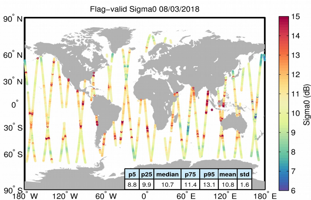
Figure 23. Geographical distribution of flag-valid sigma0 data over oceans and lakes for 08/03/2018. The statistical values shown in the table refer to the sigma0 in dB and are calculated over all measurements shown in the figure.
