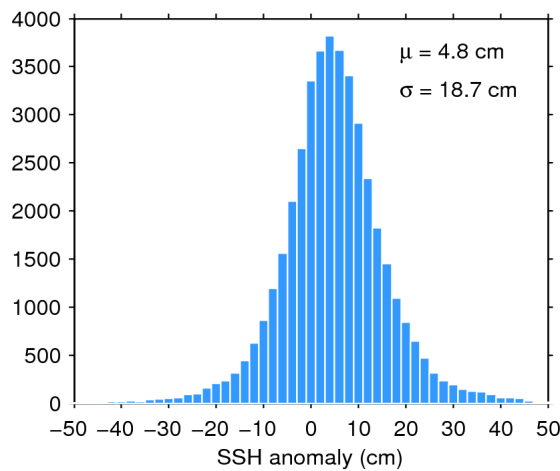
Figure 7. Histogram of flag-valid SSH anomaly over oceans and lakes for 08/03/2018. The mean ( \mu ) and standard deviation ( \sigma ) are also shown. Note that values outside [-50\ 50] cm are excluded from the histogram for the sake of readability but not from the computation of \mu and \sigma .
