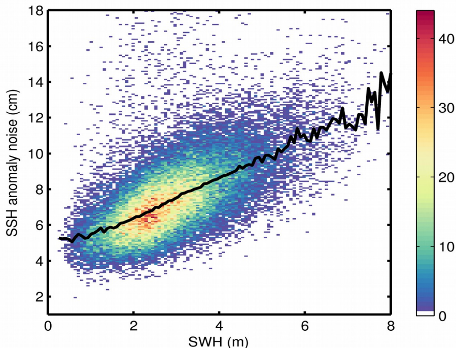
Figure 9. 2D histogram showing flag-valid SSH anomaly noise as a function of SWH for 08/03/2018. The black line denotes the median SSH anomaly noise as a function of SWH.
