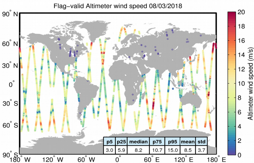
Figure 31. Geographical distribution of flag-valid wind data over oceans and lakes for 08/03/2018. The statistical values shown in the table refer to the wind in m/s and are calculated over all measurements shown in the figure.
