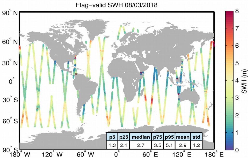
Figure 15. Geographical distribution of flag-valid SWH data over oceans and lakes for 08/03/2018. The statistical values shown in the table refer to the SWH in m and are calculated over all measurements shown in the figure.
