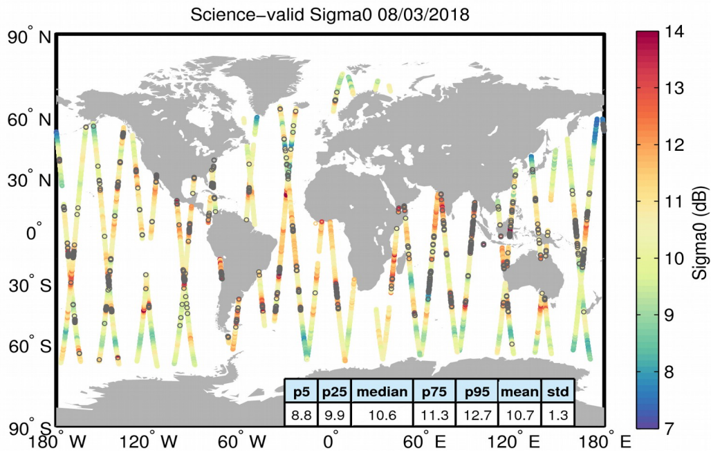
Figure 27. Geographical distribution of science-valid sigma0 data over oceans and lakes for 08/03/2018. The statistical values shown in the table refer to the sigma0 in dB and are calculated over all measurements shown in the figure. Gray circles denote records that have been rejected based on the editing criteria described in Table 4.
