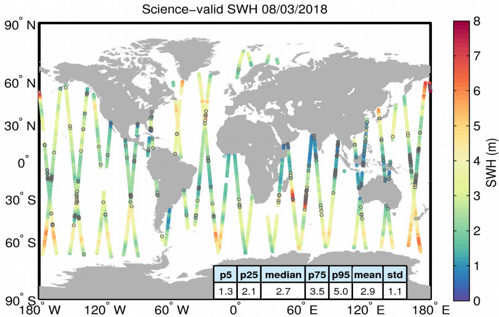
Figure 19. Geographical distribution of science-valid SWH data over oceans and lakes for 08/03/2018. The statistical values shown in the table refer to the SWH in m and are calculated over all measurements shown in the figure. Gray circles denote records that have been rejected based on the editing criteria described in Table 3.
