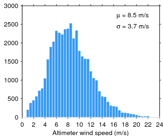
Figure 35. Histogram of science-valid wind over oceans and lakes for 08/03/2018. The mean ( \mu ) and standard deviation ( \sigma ) are also shown. Note that values larger than 24 m/s are excluded from the histogram for the sake of readability but not from the computation of \mu and \sigma .
