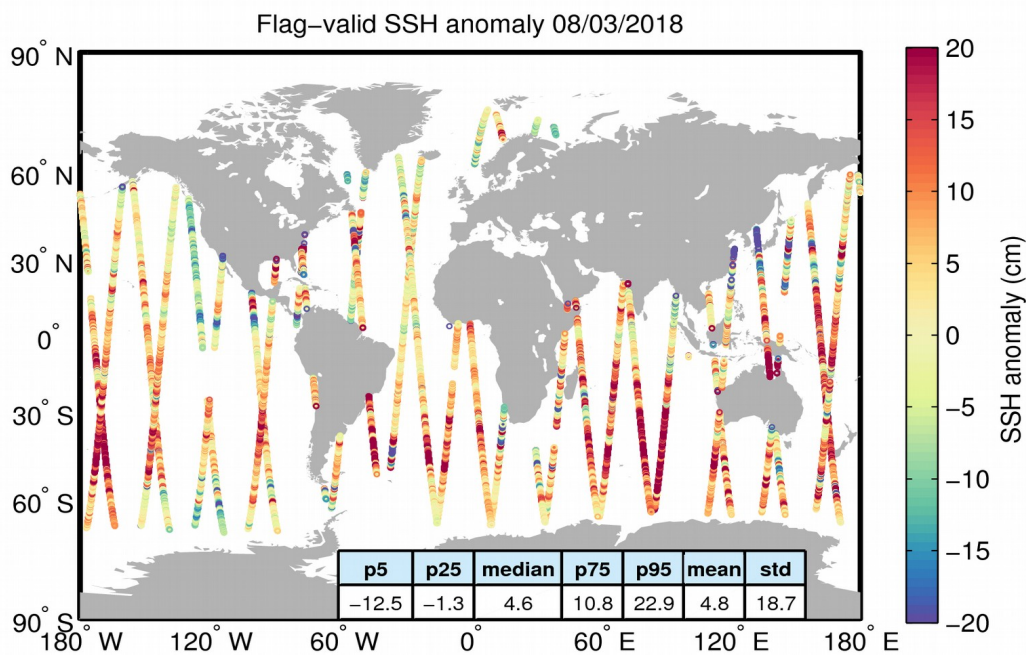
Figure 5. Geographical distribution of flag-valid 1-Hz SSH anomaly data over oceans and lakes for 08/03/2018. The statistical values shown in the table refer to the SSH anomaly in cm and are calculated over all measurements shown in the figure.
