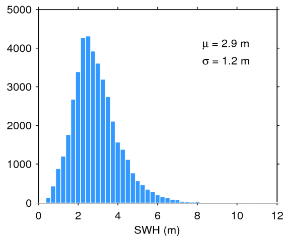
Figure 17. Histogram of flag-valid SWH over oceans and lakes for 08/03/2018. The mean ( \mu ) and standard deviation ( \sigma ) are also shown. Note that values larger than 12 m are excluded from the histogram for the sake of readability but not from the computation of \mu and \sigma .
