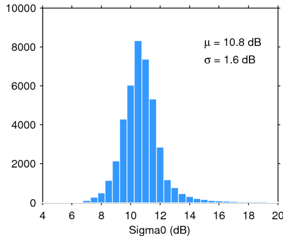
Figure 25. Histogram of flag-valid sigma0 over oceans and lakes for 08/03/2018. The mean ( \mu ) and standard deviation ( \sigma ) are also shown. Note that values outside [4 20] dB are excluded from the histogram for the sake of readability but not from the computation of \mu and \sigma .
