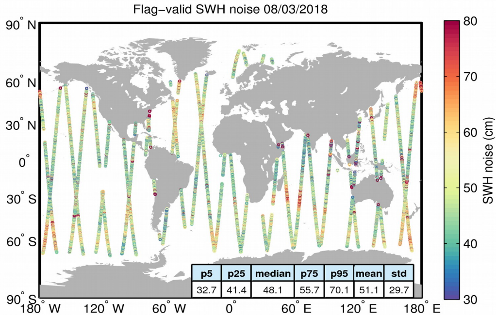
Figure 18. Geographical distribution of flag-valid 20-Hz SWH measurement noise over oceans and lakes for 08/03/2018. The statistical values shown in the figure refer to the SWH noise and are calculated over all measurements shown in the figure.
