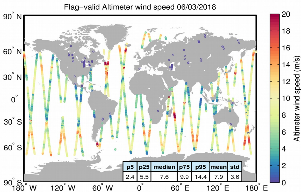
Figure 31. Geographical distribution of flag-valid wind data over oceans and lakes for 06/03/2018. The statistical values shown in the table refer to the wind in m/s and are calculated over all measurements shown in the figure.
