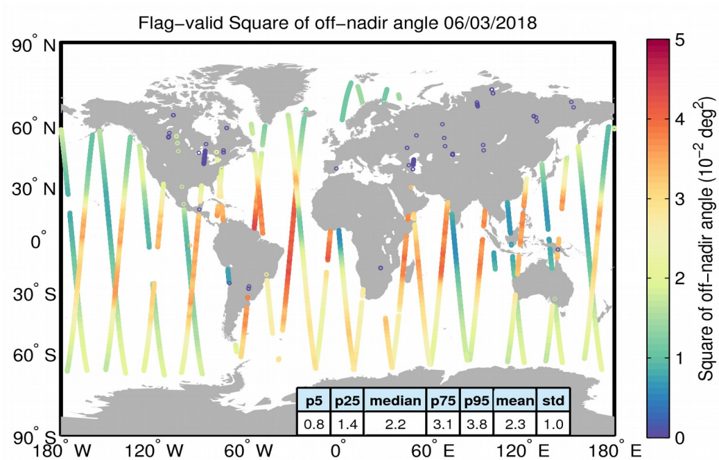
Figure 37. Geographical distribution of flag-valid mispointing data over oceans and lakes for 06/03/2018. The statistical values shown in the table refer to the mispointing in 10^{-2} \text{ deg}^2 and are calculated over all measurements shown in the figure.
