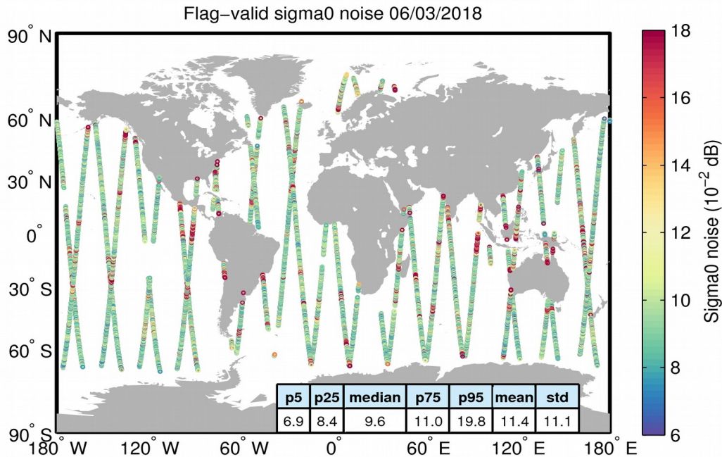
Figure 26. Geographical distribution of flag-valid 20-Hz sigma0 measurement noise over oceans and lakes for 06/03/2018. The statistical values shown in the table refer to the sigma0 noise and are calculated over all measurements shown in the figure.
