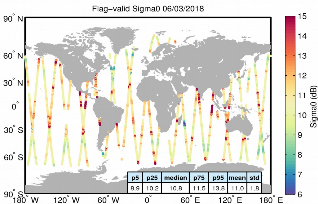
Figure 23. Geographical distribution of flag-valid sigma0 data over oceans and lakes for 06/03/2018. The statistical values shown in the table refer to the sigma0 in dB and are calculated over all measurements shown in the figure.
