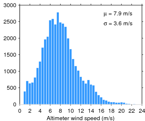
Figure 35. Histogram of science-valid wind over oceans and lakes for 06/03/2018. The mean ( \mu ) and standard deviation ( \sigma ) are also shown. Note that values larger than 24 m/s are excluded from the histogram for the sake of readability but not from the computation of \mu and \sigma .
