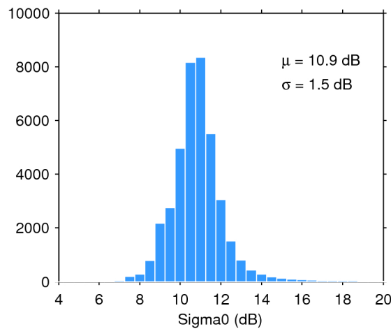
Figure 28. Histogram of science-valid sigma0 over oceans and lakes for 06/03/2018. The mean ( \mu ) and standard deviation ( \sigma ) are also shown. Note that values outside [4 20] dB are excluded from the histogram for the sake of readability but not from the computation of \mu and \sigma .
