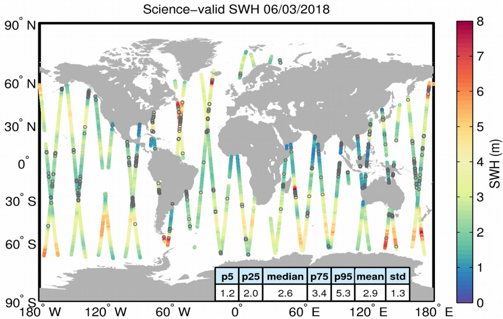
Figure 19. Geographical distribution of science-valid SWH data over oceans and lakes for 06/03/2018. The statistical values shown in the table refer to the SWH in m and are calculated over all measurements shown in the figure. Gray circles denote records that have been rejected based on the editing criteria described in Table 3.
