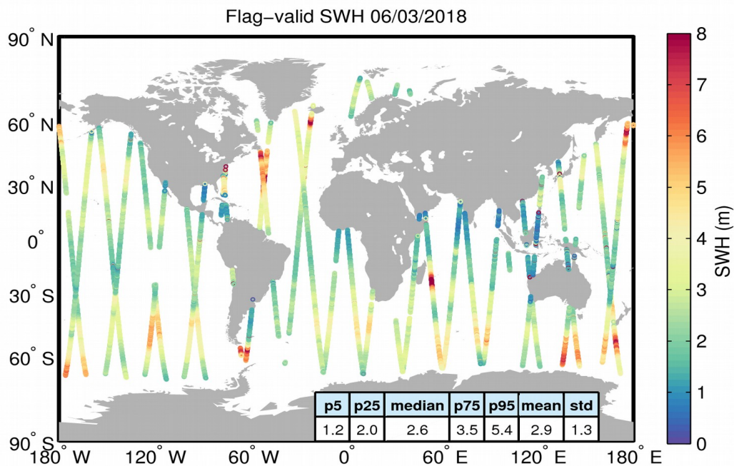
Figure 15. Geographical distribution of flag-valid SWH data over oceans and lakes for 06/03/2018. The statistical values shown in the table refer to the SWH in m and are calculated over all measurements shown in the figure.
