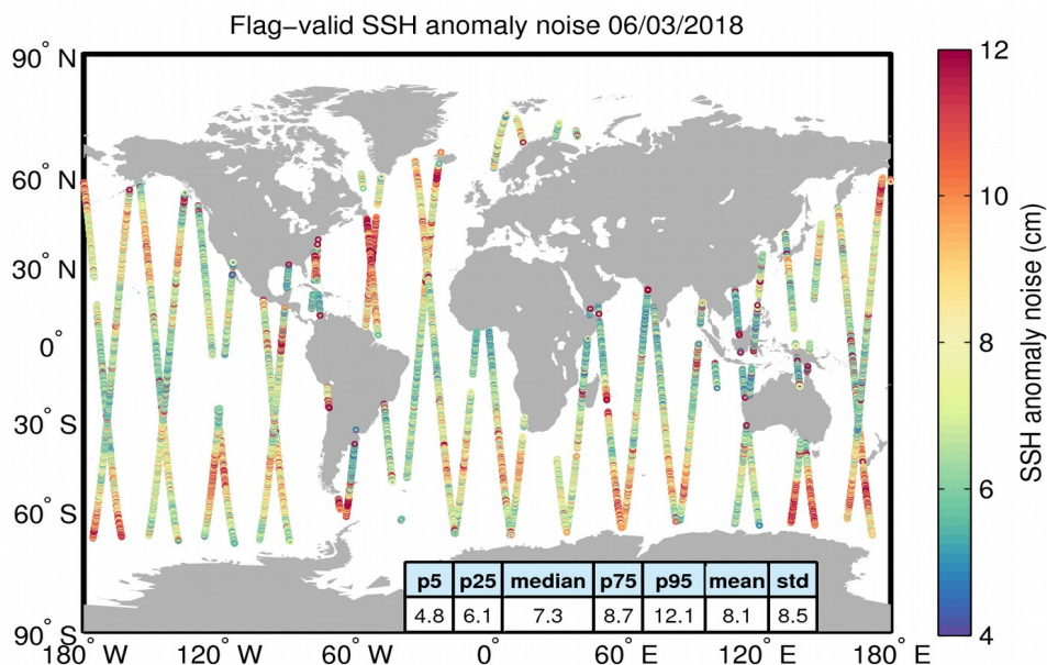
Figure 8. Geographical distribution of flag-valid 20-Hz SSH anomaly measurement noise over oceans and lakes for 06/03/2018. The statistical values shown in the table refer to the SSH anomaly noise and are calculated over all measurements shown in the figure.
