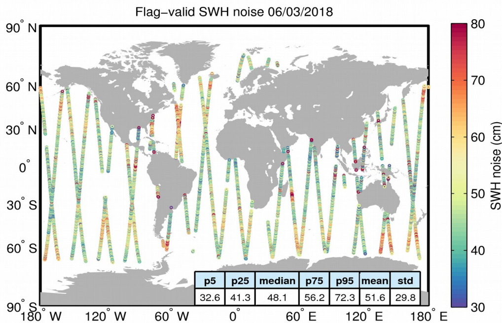
Figure 18. Geographical distribution of flag-valid 20-Hz SWH measurement noise over oceans and lakes for 06/03/2018. The statistical values shown in the table refer to the SWH noise and are calculated over all measurements shown in the figure.
