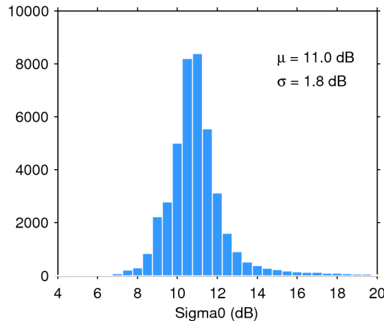
Figure 25. Histogram of flag-valid sigma0 over oceans and lakes for 06/03/2018. The mean ( \mu ) and standard deviation ( \sigma ) are also shown. Note that values outside [4 20] dB are excluded from the histogram for the sake of readability but not from the computation of \mu and \sigma .
