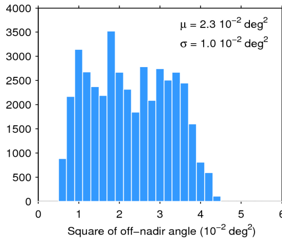
Figure 39. Histogram of flag-valid mispointing over oceans and lakes for 06/03/2018. The mean ( \mu ) and standard deviation ( \sigma ) are also shown. Note that values larger than 6 \cdot 10^{-2} \text{ deg}^2 are excluded from the histogram for the sake of readability but not from the computation of \mu and \sigma .
