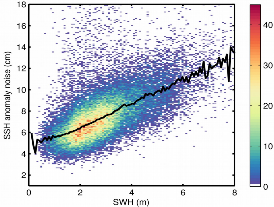
Figure 9. 2D histogram showing flag-valid SSH anomaly noise as a function of SWH for 06/03/2018. The black line denotes the median SSH anomaly noise as a function of SWH.
