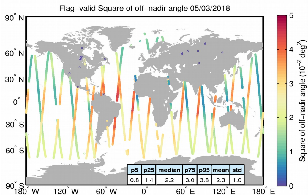
Figure 37. Geographical distribution of flag-valid mispointing data over oceans and lakes for 05/03/2018. The statistical values shown in the table refer to the mispointing in 10^{-2} \text{ deg}^2 and are calculated over all measurements shown in the figure.
