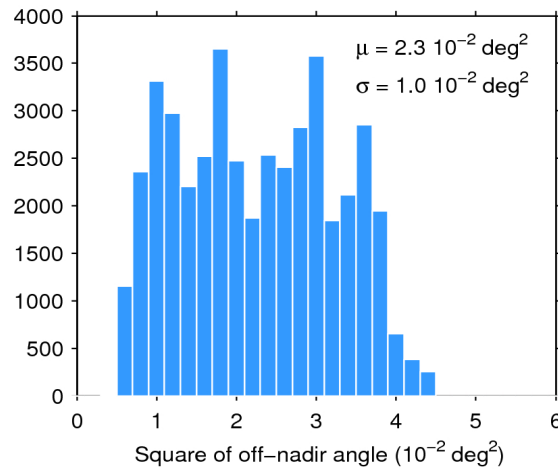
Figure 39. Histogram of flag-valid mispointing over oceans and lakes for 05/03/2018. The mean ( \mu ) and standard deviation ( \sigma ) are also shown. Note that values larger than 6 \cdot 10^{-2} \text{ deg}^2 are excluded from the histogram for the sake of readability but not from the computation of \mu and \sigma .
