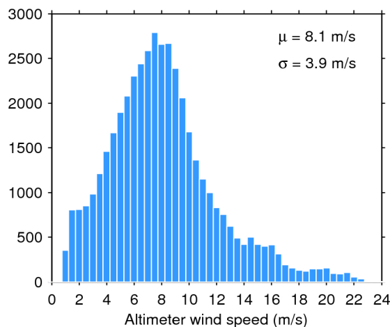
Figure 35. Histogram of science-valid wind over oceans and lakes for 05/03/2018. The mean ( \mu ) and standard deviation ( \sigma ) are also shown. Note that values larger than 24 m/s are excluded from the histogram for the sake of readability but not from the computation of \mu and \sigma .
