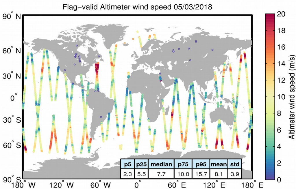
Figure 31. Geographical distribution of flag-valid wind data over oceans and lakes for 05/03/2018. The statistical values shown in the table refer to the wind in m/s and are calculated over all measurements shown in the figure.
