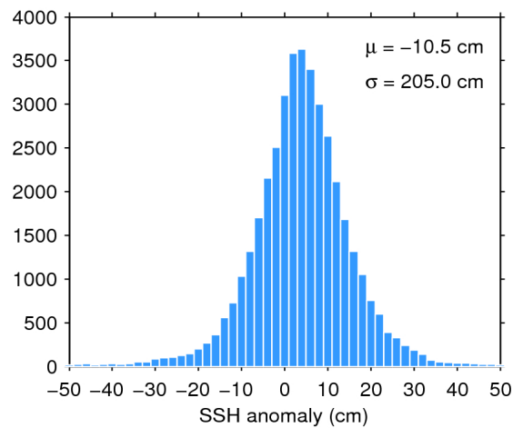
Figure 7. Histogram of flag-valid SSH anomaly over oceans and lakes for 05/03/2018. The mean ( \mu ) and standard deviation ( \sigma ) are also shown. Note that values outside [-50 50] cm are excluded from the histogram for the sake of readability but not from the computation of \mu and \sigma .
