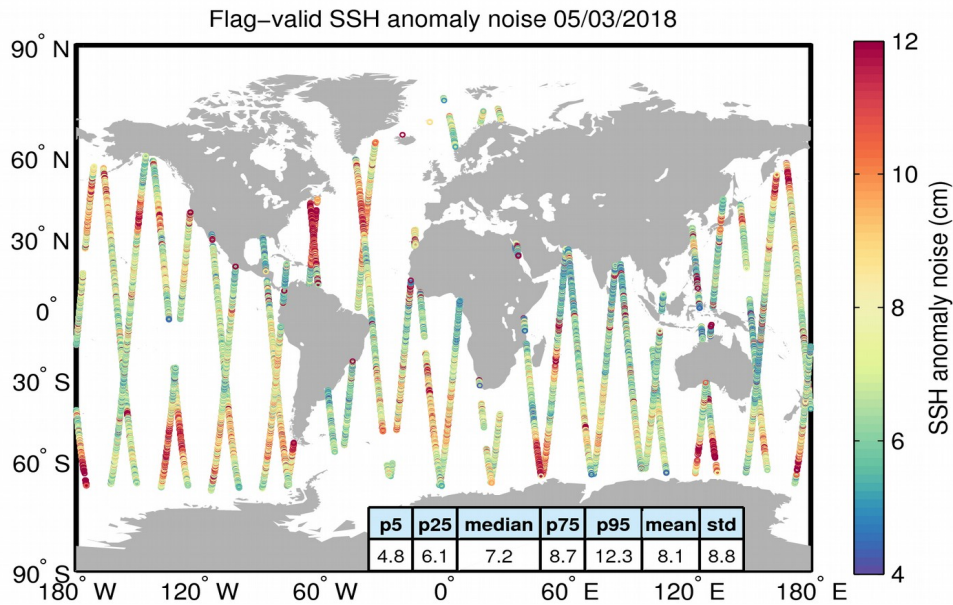
Figure 8. Geographical distribution of flag-valid 20-Hz SSH anomaly measurement noise over oceans and lakes for 05/03/2018. The statistical values shown in the table refer to the SSH anomaly noise and are calculated over all measurements shown in the figure.
