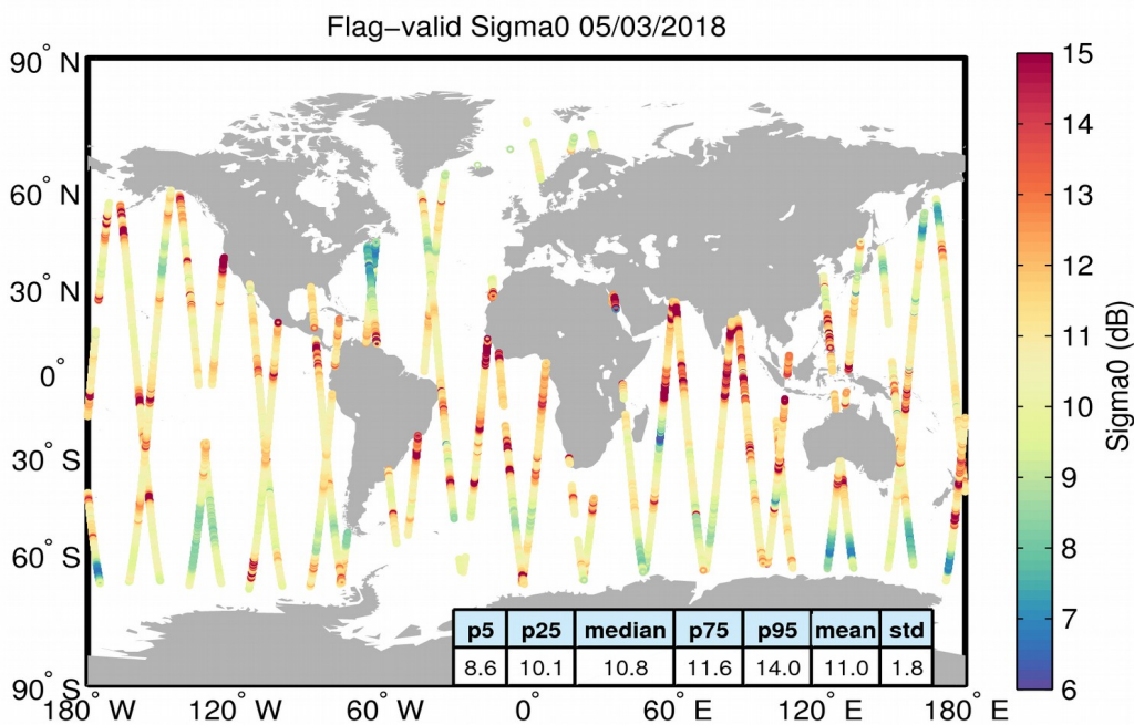
Figure 23. Geographical distribution of flag-valid sigma0 data over oceans and lakes for 05/03/2018. The statistical values shown in the table refer to the sigma0 in dB and are calculated over all measurements shown in the figure.
