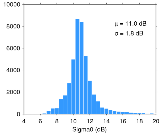
Figure 25. Histogram of flag-valid sigma0 over oceans and lakes for 05/03/2018. The mean ( \mu ) and standard deviation ( \sigma ) are also shown. Note that values outside [4 20] dB are excluded from the histogram for the sake of readability but not from the computation of \mu and \sigma .
