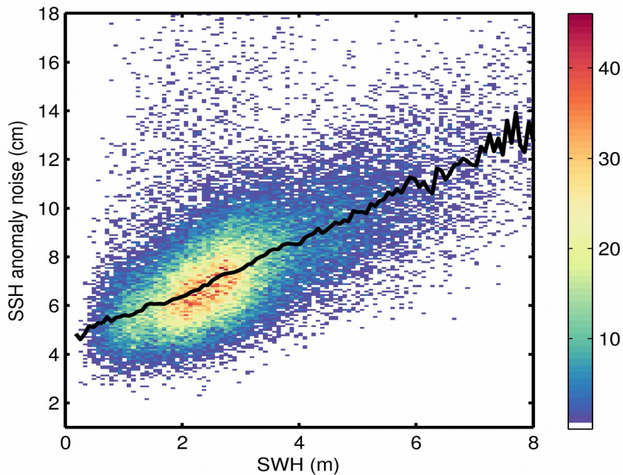
Figure 9. 2D histogram showing flag-valid SSH anomaly noise as a function of SWH for 05/03/2018. The black line denotes the median SSH anomaly noise as a function of SWH.
