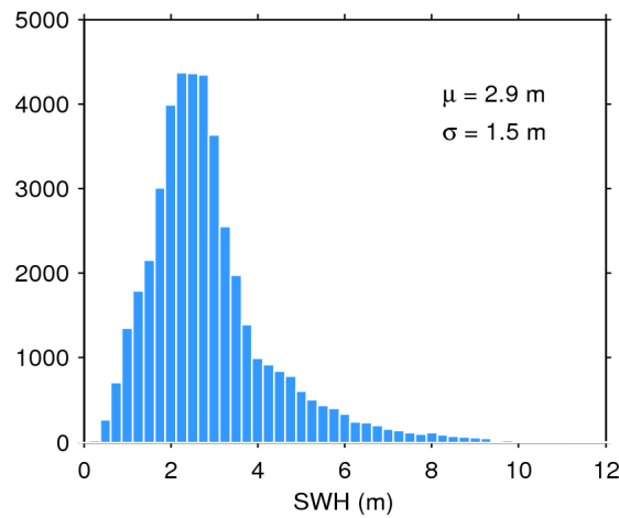
Figure 17. Histogram of flag-valid SWH over oceans and lakes for 05/03/2018. The mean ( \mu ) and standard deviation ( \sigma ) are also shown. Note that values larger than 12 m are excluded from the histogram for the sake of readability but not from the computation of \mu and \sigma .
