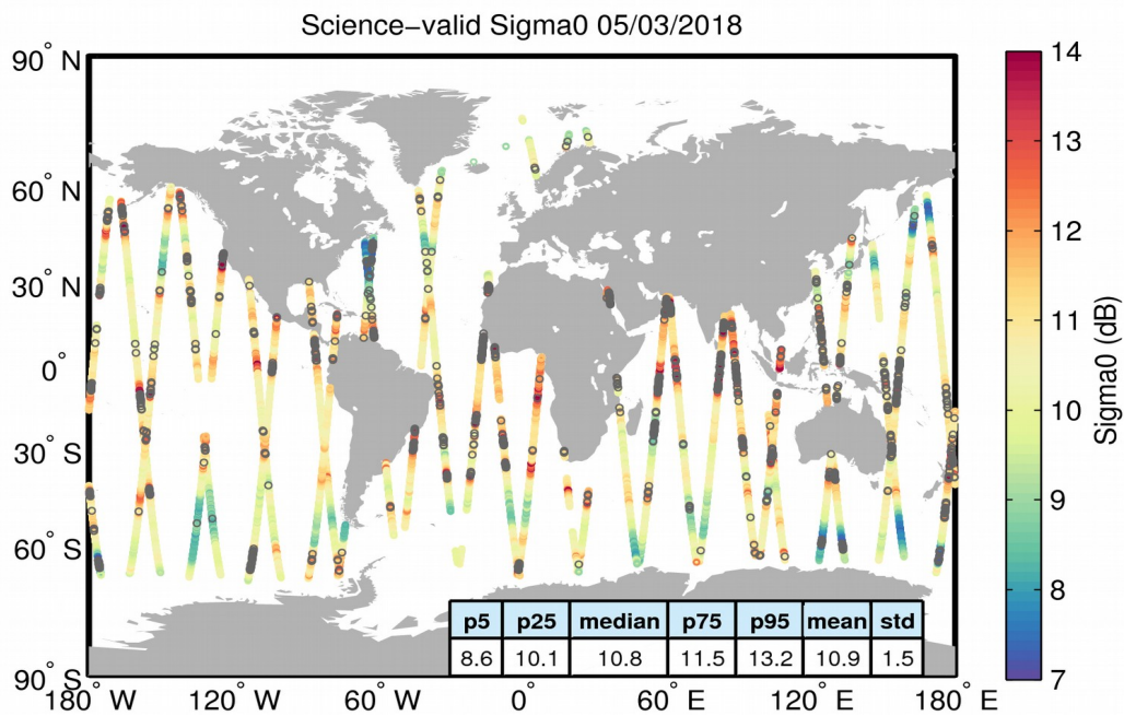
Figure 27. Geographical distribution of science-valid sigma0 data over oceans and lakes for 05/03/2018. The statistical values shown in the table refer to the sigma0 in dB and are calculated over all measurements shown in the figure. Gray circles denote records that have been rejected based on the editing criteria described in Table 4.
