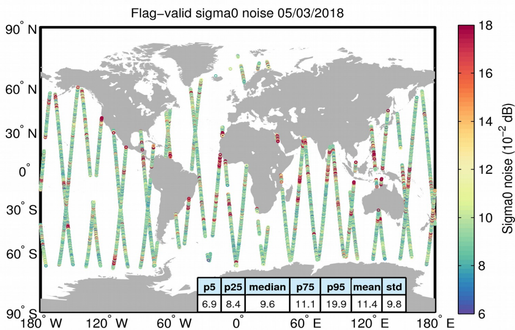
Figure 26. Geographical distribution of flag-valid 20-Hz sigma0 measurement noise over oceans and lakes for 05/03/2018. The statistical values shown in the table refer to the sigma0 noise and are calculated over all measurements shown in the figure.
