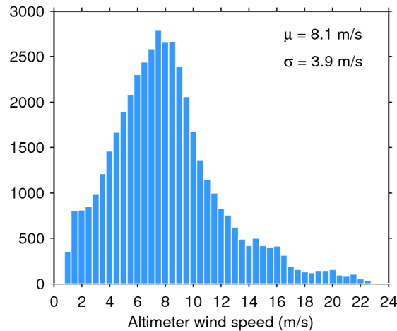
Figure 33. Histogram of flag-valid wind over oceans and lakes for 05/03/2018. The mean ( \mu ) and standard deviation ( \sigma ) are also shown. Note that values larger than 24 m/s are excluded from the histogram for the sake of readability but not from the computation of \mu and \sigma .
