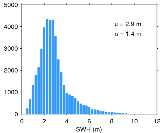
Figure 20. Histogram of science-valid SWH over oceans and lakes for 05/03/2018. The mean ( \mu ) and standard deviation ( \sigma ) are also shown. Note that values larger than 12 m are excluded from the histogram for the sake of readability but not from the computation of \mu and \sigma .
