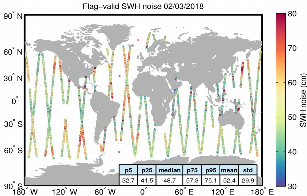
Figure 18. Geographical distribution of flag-valid 20-Hz SWH measurement noise over oceans and lakes for 02/03/2018. The statistical values shown in the figure refer to the SWH noise and are calculated over all measurements shown in the figure.
