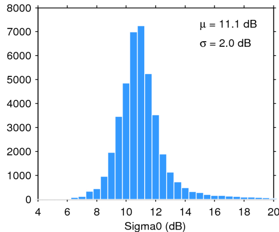
Figure 25. Histogram of flag-valid sigma0 over oceans and lakes for 02/03/2018. The mean ( \mu ) and standard deviation ( \sigma ) are also shown. Note that values outside [4 20] dB are excluded from the histogram for the sake of readability but not from the computation of \mu and \sigma .
