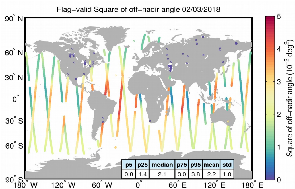
Figure 37. Geographical distribution of flag-valid mispointing data over oceans and lakes for 02/03/2018. The statistical values shown in the table refer to the mispointing in 10^{-2} deg 2 and are calculated over all measurements shown in the figure.
