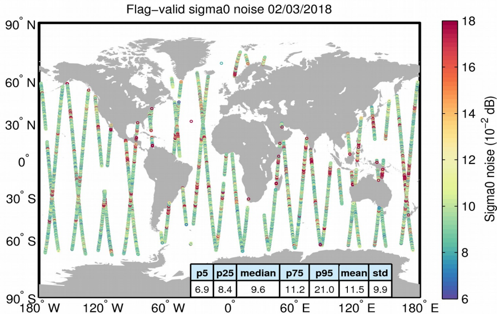
Figure 26. Geographical distribution of flag-valid 20-Hz sigma0 measurement noise over oceans and lakes for 02/03/2018. The statistical values shown in the table refer to the sigma0 noise and are calculated over all measurements shown in the figure.
