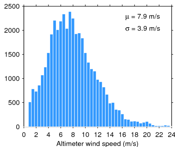
Figure 35. Histogram of science-valid wind over oceans and lakes for 02/03/2018. The mean ( \mu ) and standard deviation ( \sigma ) are also shown. Note that values larger than 24 m/s are excluded from the histogram for the sake of readability but not from the computation of \mu and \sigma .
