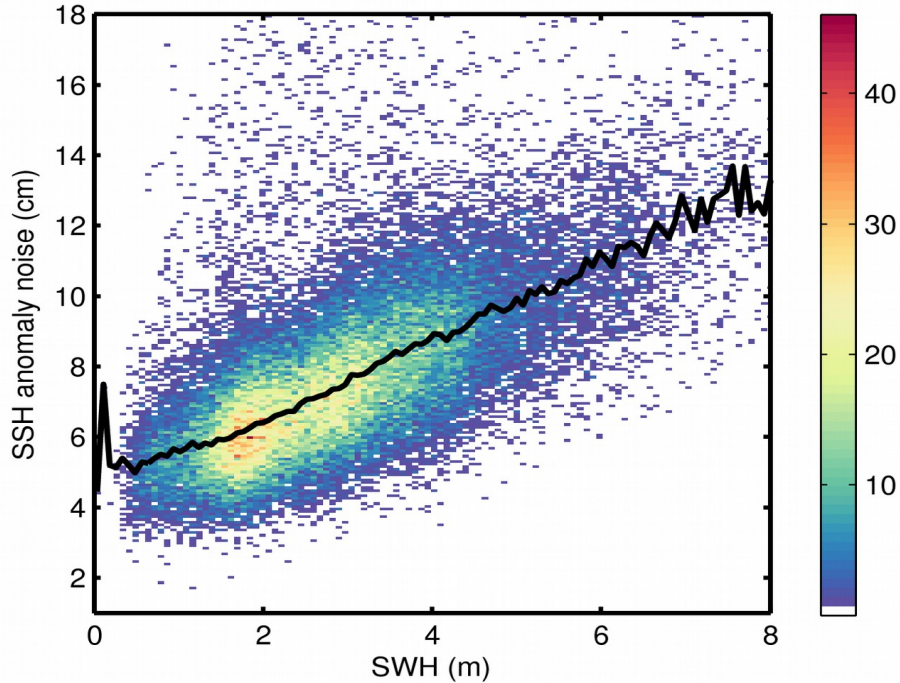
Figure 9. 2D histogram showing flag-valid SSH anomaly noise as a function of SWH for 02/03/2018. The black line denotes the median SSH anomaly noise as a function of SWH.
