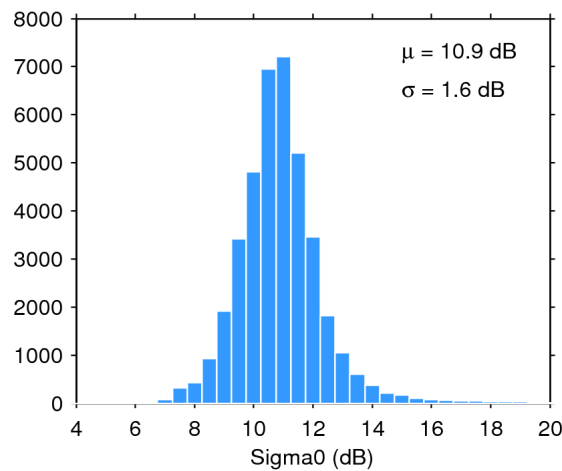
Figure 28. Histogram of science-valid sigma0 over oceans and lakes for 02/03/2018. The mean ( \mu ) and standard deviation ( \sigma ) are also shown. Note that values outside [4 20] dB are excluded from the histogram for the sake of readability but not from the computation of \mu and \sigma .
