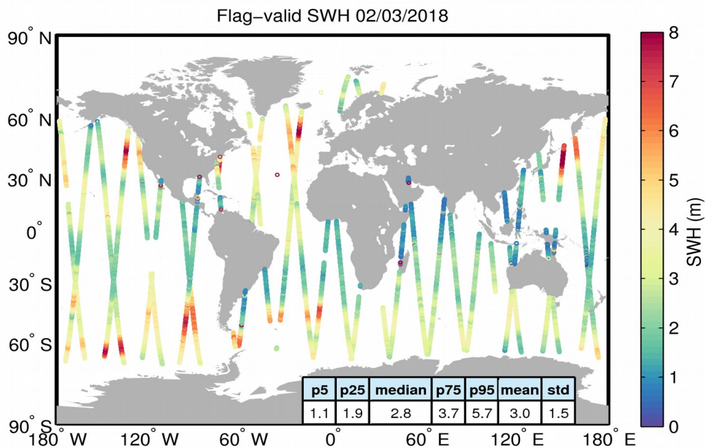
Figure 15. Geographical distribution of flag-valid SWH data over oceans and lakes for 02/03/2018. The statistical values shown in the table refer to the SWH in m and are calculated over all measurements shown in the figure.
