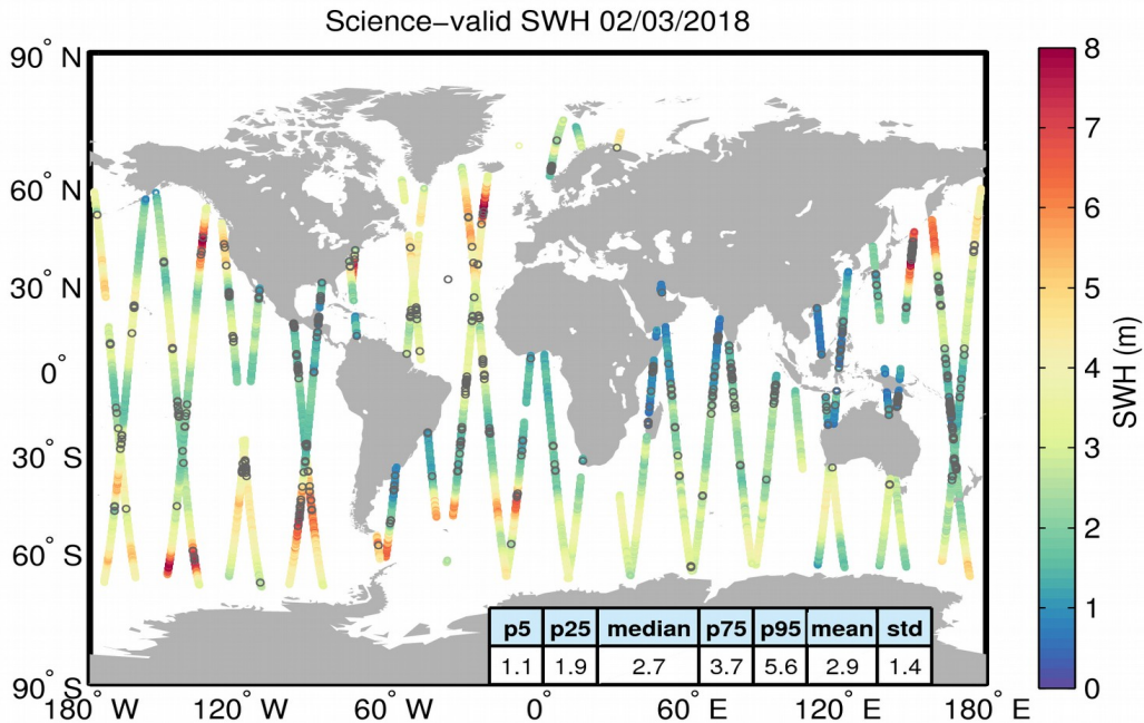
Figure 19. Geographical distribution of science-valid SWH data over oceans and lakes for 02/03/2018. The statistical values shown in the table refer to the SWH in m and are calculated over all measurements shown in the figure. Gray circles denote records that have been rejected based on the editing criteria described in Table 3.
