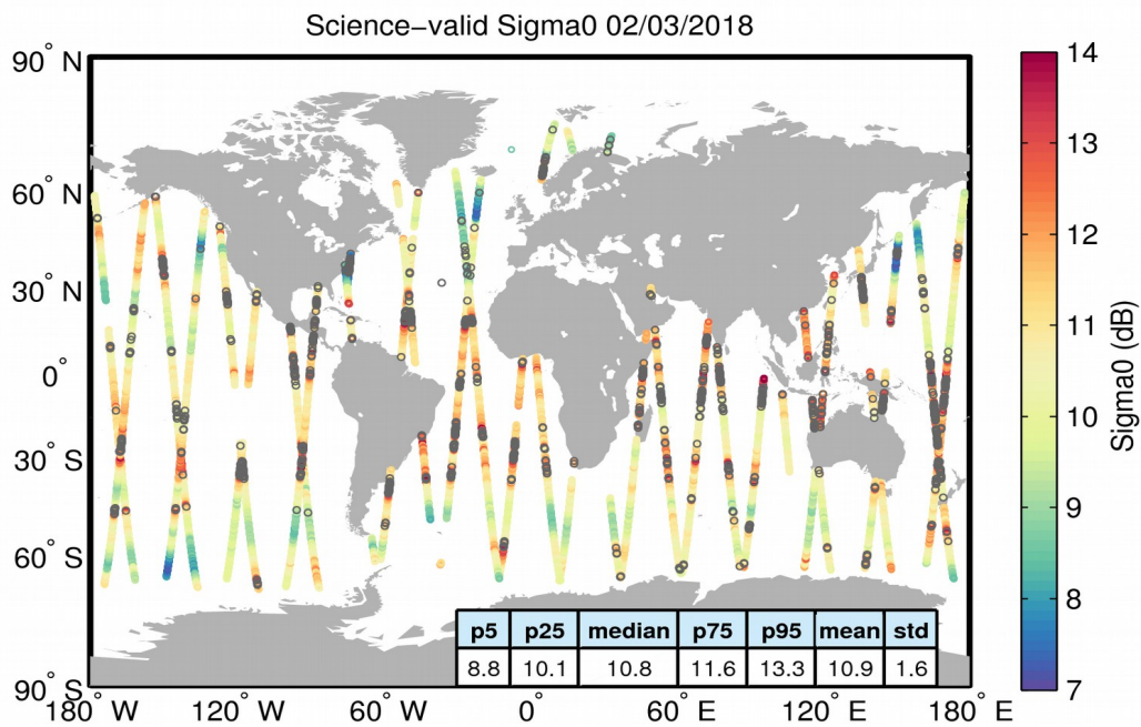
Figure 27. Geographical distribution of science-valid sigma0 data over oceans and lakes for 02/03/2018. The statistical values shown in the table refer to the sigma0 in dB and are calculated over all measurements shown in the figure. Gray circles denote records that have been rejected based on the editing criteria described in Table 4.
