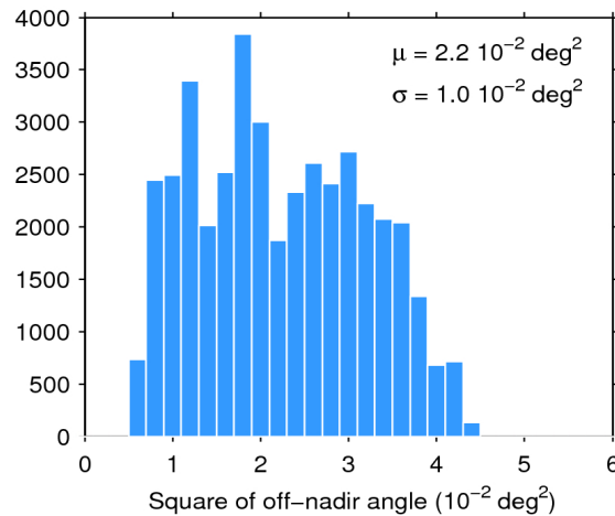
Figure 39. Histogram of flag-valid mispointing over oceans and lakes for 02/03/2018. The mean ( \mu ) and standard deviation ( \sigma ) are also shown. Note that values larger than 6 \cdot 10^{-2} \text{ deg}^2 are excluded from the histogram for the sake of readability but not from the computation of \mu and \sigma .
