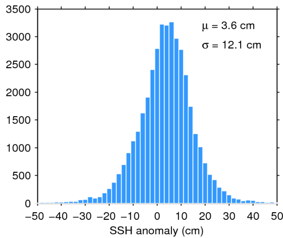
Figure 11. Histogram of science-valid SSH anomaly over oceans and lakes for 02/03/2018. The mean ( \mu ) and standard deviation ( \sigma ) are also shown. Note that values outside [-50 50] cm are excluded from the histogram for the sake of readability but not from the computation of \mu and \sigma .
