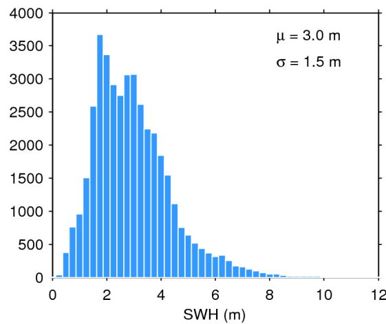
Figure 17. Histogram of flag-valid SWH over oceans and lakes for 02/03/2018. The mean ( \mu ) and standard deviation ( \sigma ) are also shown. Note that values larger than 12 m are excluded from the histogram for the sake of readability but not from the computation of \mu and \sigma .
