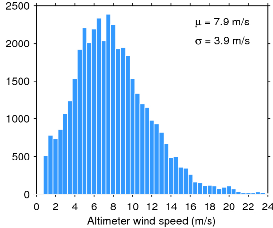
Figure 33. Histogram of flag-valid wind over oceans and lakes for 02/03/2018. The mean ( \mu ) and standard deviation ( \sigma ) are also shown. Note that values larger than 24 m/s are excluded from the histogram for the sake of readability but not from the computation of \mu and \sigma .
