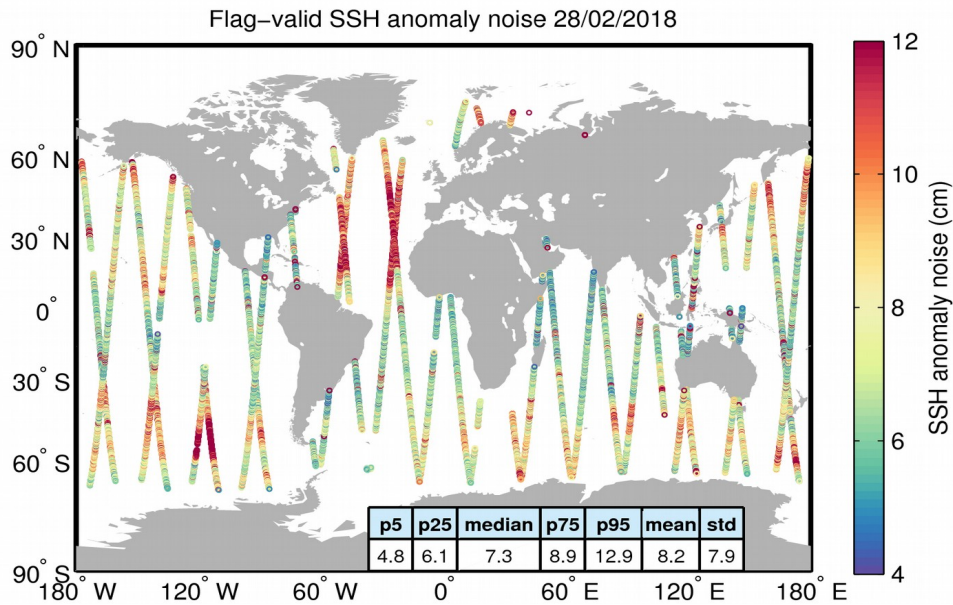
Figure 8. Geographical distribution of flag-valid 20-Hz SSH anomaly measurement noise over oceans and lakes for 28/02/2018. The statistical values shown in the table refer to the SSH anomaly noise and are calculated over all measurements shown in the figure.
