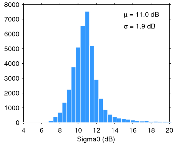
Figure 25. Histogram of flag-valid sigma0 over oceans and lakes for 28/02/2018. The mean ( \mu ) and standard deviation ( \sigma ) are also shown. Note that values outside [4 20] dB are excluded from the histogram for the sake of readability but not from the computation of \mu and \sigma .
