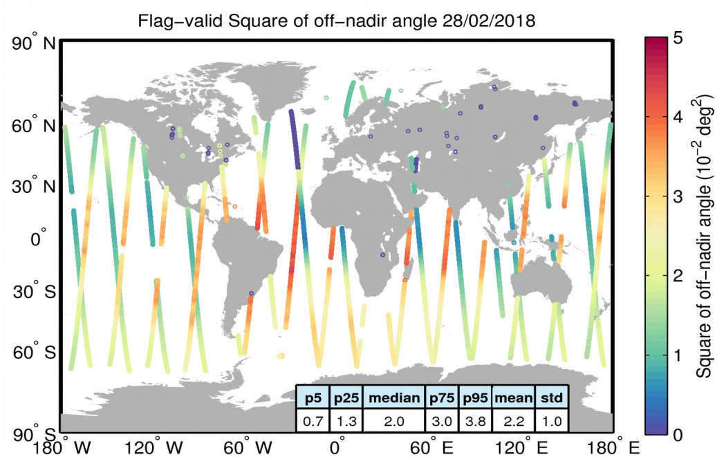
Figure 37. Geographical distribution of flag-valid mispointing data over oceans and lakes for 28/02/2018. The statistical values shown in the table refer to the mispointing in 10^{-2} deg 2 and are calculated over all measurements shown in the figure.
