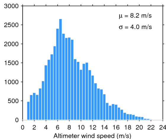
Figure 35. Histogram of science-valid wind over oceans and lakes for 28/02/2018. The mean ( \mu ) and standard deviation ( \sigma ) are also shown. Note that values larger than 24 m/s are excluded from the histogram for the sake of readability but not from the computation of \mu and \sigma .
