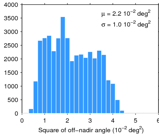
Figure 39. Histogram of flag-valid mispointing over oceans and lakes for 28/02/2018. The mean ( \mu ) and standard deviation ( \sigma ) are also shown. Note that values larger than 6 \cdot 10^{-2} \text{ deg}^2 are excluded from the histogram for the sake of readability but not from the computation of \mu and \sigma .
