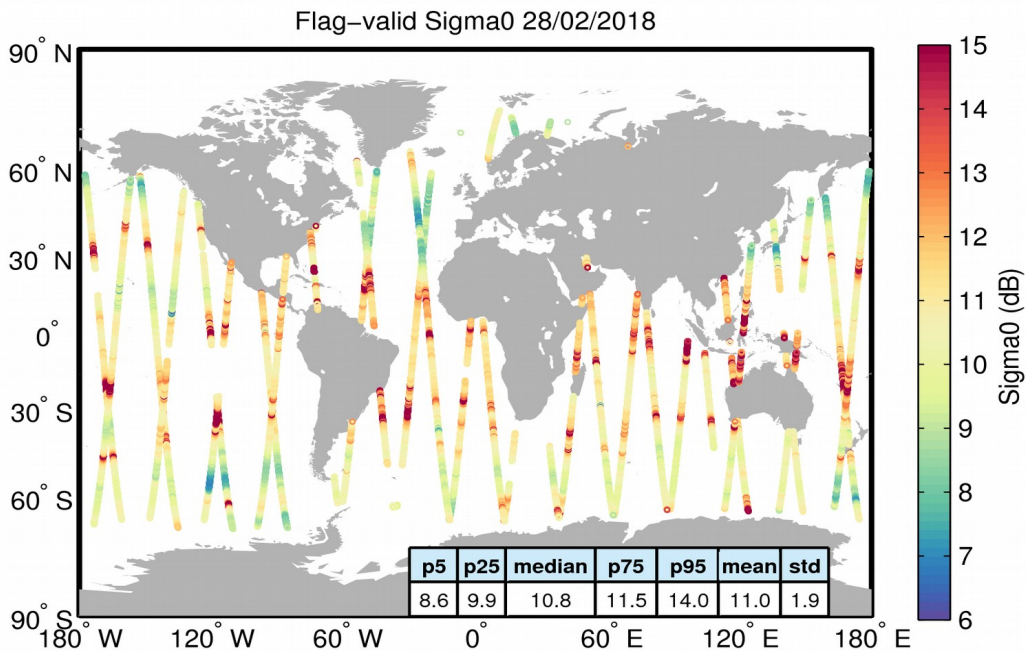
Figure 23. Geographical distribution of flag-valid sigma0 data over oceans and lakes for 28/02/2018. The statistical values shown in the table refer to the sigma0 in dB and are calculated over all measurements shown in the figure.
