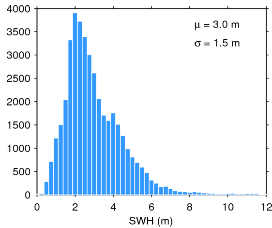
Figure 17. Histogram of flag-valid SWH over oceans and lakes for 28/02/2018. The mean ( \mu ) and standard deviation ( \sigma ) are also shown. Note that values larger than 12 m are excluded from the histogram for the sake of readability but not from the computation of \mu and \sigma .
