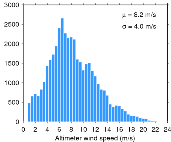
Figure 33. Histogram of flag-valid wind over oceans and lakes for 28/02/2018. The mean ( \mu ) and standard deviation ( \sigma ) are also shown. Note that values larger than 24 m/s are excluded from the histogram for the sake of readability but not from the computation of \mu and \sigma .
