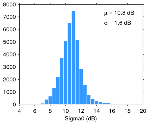
Figure 28. Histogram of science-valid sigma0 over oceans and lakes for 28/02/2018. The mean ( \mu ) and standard deviation ( \sigma ) are also shown. Note that values outside [4 20] dB are excluded from the histogram for the sake of readability but not from the computation of \mu and \sigma .
