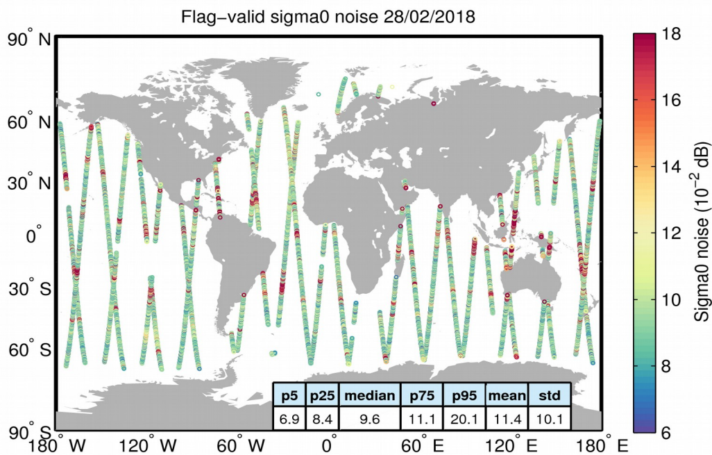
Figure 26. Geographical distribution of flag-valid 20-Hz sigma0 measurement noise over oceans and lakes for 28/02/2018. The statistical values shown in the table refer to the sigma0 noise and are calculated over all measurements shown in the figure.
