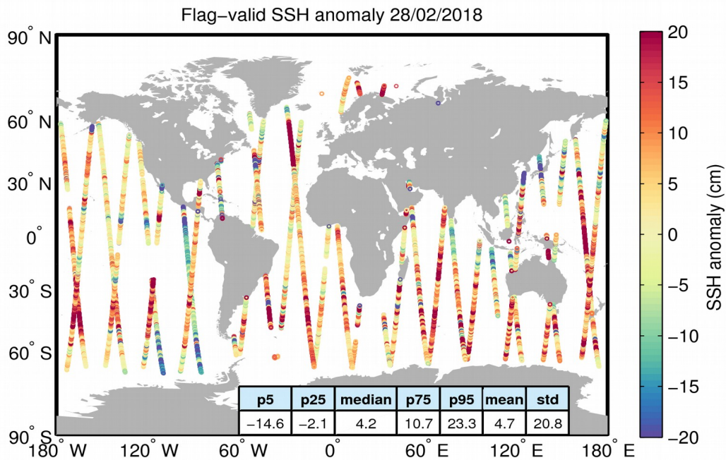
Figure 5. Geographical distribution of flag-valid 1-Hz SSH anomaly data over oceans and lakes for 28/02/2018. The statistical values shown in the table refer to the SSH anomaly in cm and are calculated over all measurements shown in the figure.
