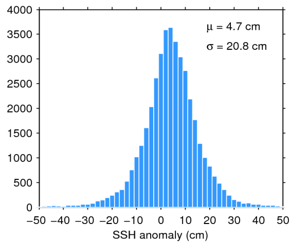
Figure 7. Histogram of flag-valid SSH anomaly over oceans and lakes for 28/02/2018. The mean ( \mu ) and standard deviation ( \sigma ) are also shown. Note that values outside [-50 50] cm are excluded from the histogram for the sake of readability but not from the computation of \mu and \sigma .
