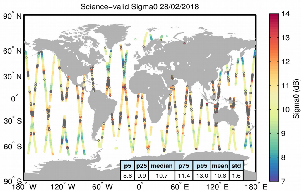
Figure 27. Geographical distribution of science-valid sigma0 data over oceans and lakes for 28/02/2018. The statistical values shown in the table refer to the sigma0 in dB and are calculated over all measurements shown in the figure. Gray circles denote records that have been rejected based on the editing criteria described in Table 4.
