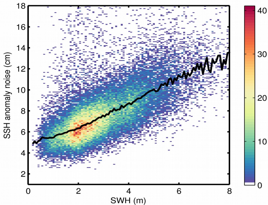
Figure 9. 2D histogram showing flag-valid SSH anomaly noise as a function of SWH for 28/02/2018. The black line denotes the median SSH anomaly noise as a function of SWH.
