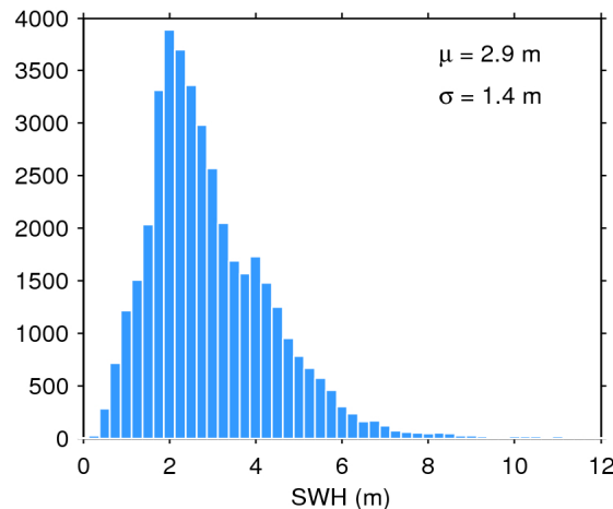
Figure 20. Histogram of science-valid SWH over oceans and lakes for 28/02/2018. The mean ( \mu ) and standard deviation ( \sigma ) are also shown. Note that values larger than 12 m are excluded from the histogram for the sake of readability but not from the computation of \mu and \sigma .
