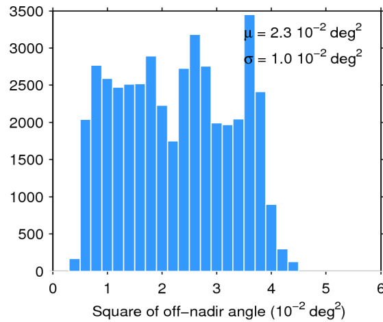
Figure 39. Histogram of flag-valid mispointing over oceans and lakes for 27/02/2018. The mean ( \mu ) and standard deviation ( \sigma ) are also shown. Note that values larger than 6 \cdot 10^{-2} \text{ deg}^2 are excluded from the histogram for the sake of readability but not from the computation of \mu and \sigma .
