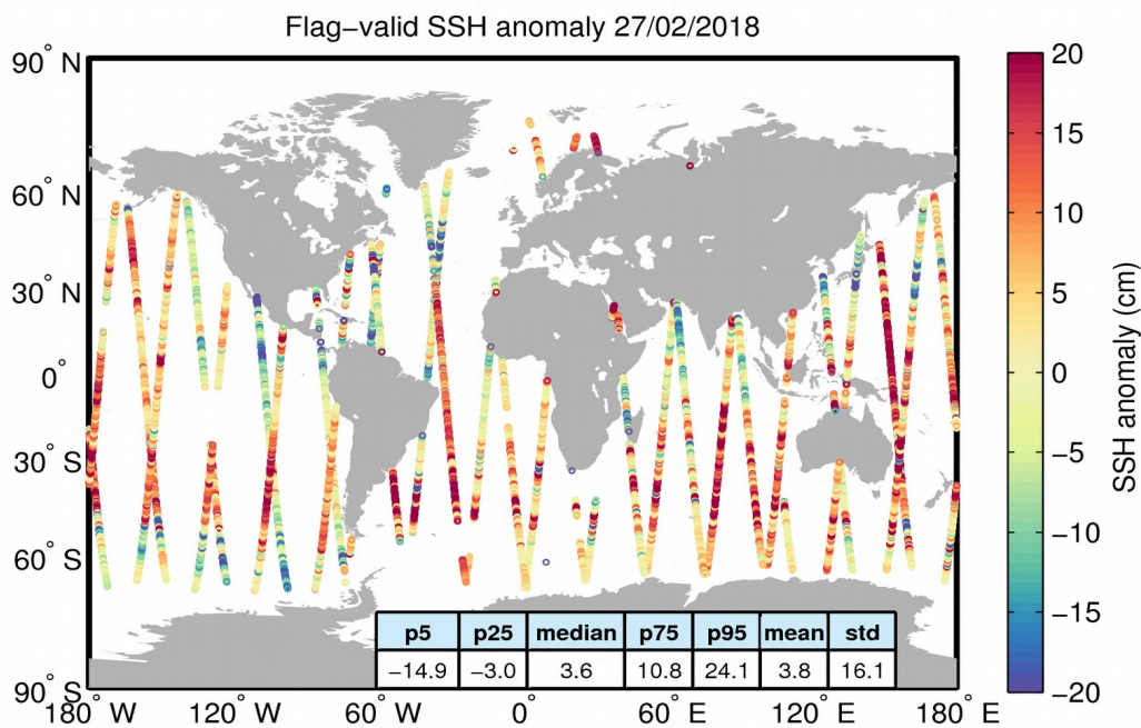
Figure 5. Geographical distribution of flag-valid 1-Hz SSH anomaly data over oceans and lakes for 27/02/2018. The statistical values shown in the table refer to the SSH anomaly in cm and are calculated over all measurements shown in the figure.
