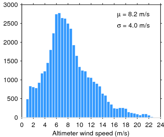
Figure 33. Histogram of flag-valid wind over oceans and lakes for 27/02/2018. The mean ( \mu ) and standard deviation ( \sigma ) are also shown. Note that values larger than 24 m/s are excluded from the histogram for the sake of readability but not from the computation of \mu and \sigma .
