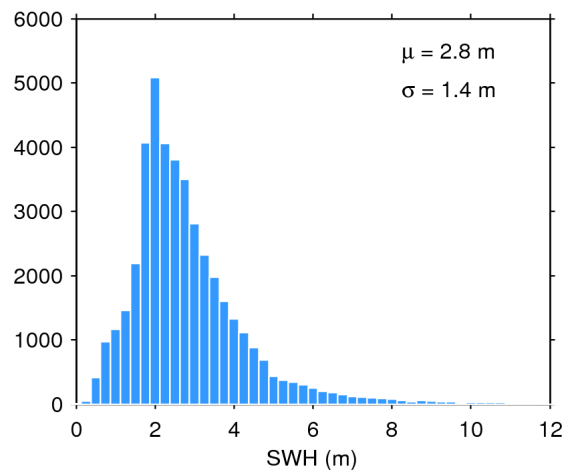
Figure 20. Histogram of science-valid SWH over oceans and lakes for 27/02/2018. The mean ( \mu ) and standard deviation ( \sigma ) are also shown. Note that values larger than 12 m are excluded from the histogram for the sake of readability but not from the computation of \mu and \sigma .
