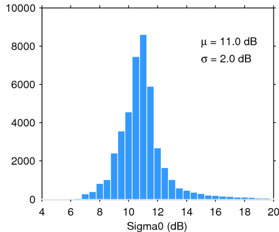
Figure 25. Histogram of flag-valid sigma0 over oceans and lakes for 27/02/2018. The mean ( \mu ) and standard deviation ( \sigma ) are also shown. Note that values outside [4 20] dB are excluded from the histogram for the sake of readability but not from the computation of \mu and \sigma .
