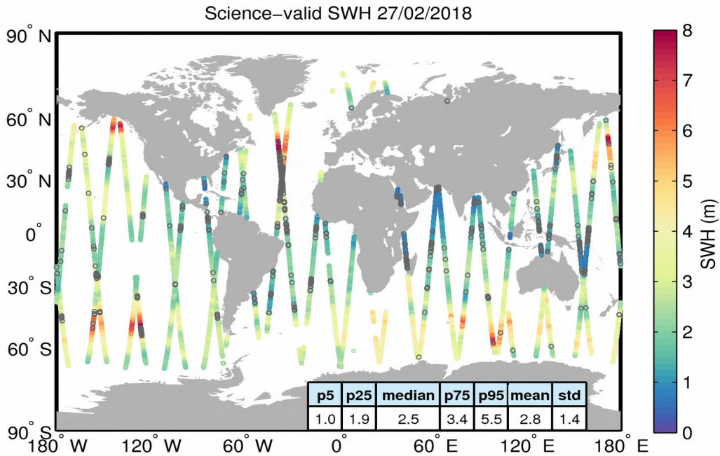
Figure 19. Geographical distribution of science-valid SWH data over oceans and lakes for 27/02/2018. The statistical values shown in the table refer to the SWH in m and are calculated over all measurements shown in the figure. Gray circles denote records that have been rejected based on the editing criteria described in Table 3.
