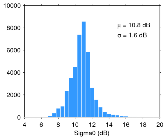
Figure 28. Histogram of science-valid sigma0 over oceans and lakes for 27/02/2018. The mean ( \mu ) and standard deviation ( \sigma ) are also shown. Note that values outside [4 20] dB are excluded from the histogram for the sake of readability but not from the computation of \mu and \sigma .
