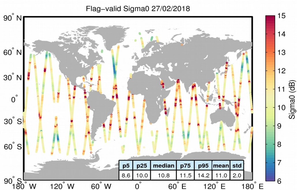
Figure 23. Geographical distribution of flag-valid sigma0 data over oceans and lakes for 27/02/2018. The statistical values shown in the table refer to the sigma0 in dB and are calculated over all measurements shown in the figure.
