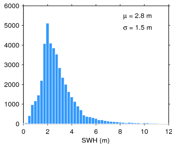
Figure 17. Histogram of flag-valid SWH over oceans and lakes for 27/02/2018. The mean ( \mu ) and standard deviation ( \sigma ) are also shown. Note that values larger than 12 m are excluded from the histogram for the sake of readability but not from the computation of \mu and \sigma .
