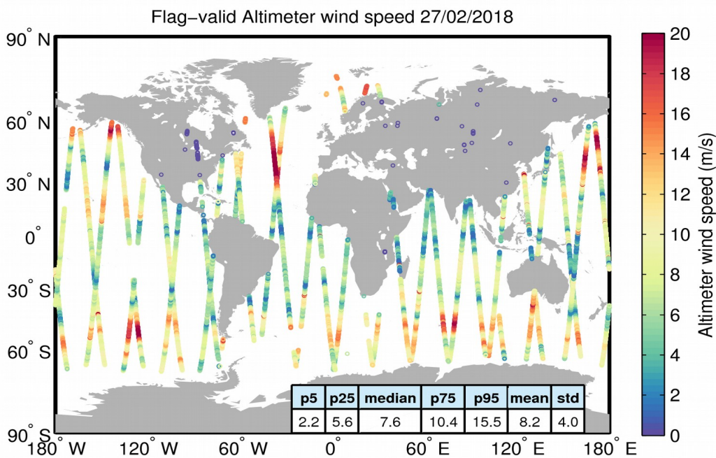
Figure 31. Geographical distribution of flag-valid wind data over oceans and lakes for 27/02/2018. The statistical values shown in the table refer to the wind in m/s and are calculated over all measurements shown in the figure.
