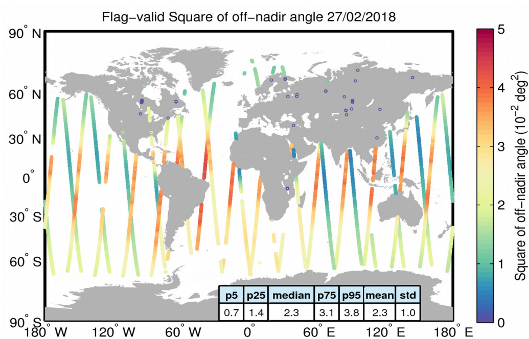
Figure 37. Geographical distribution of flag-valid mispointing data over oceans and lakes for 27/02/2018. The statistical values shown in the table refer to the mispointing in 10^{-2} \text{ deg}^2 and are calculated over all measurements shown in the figure.
