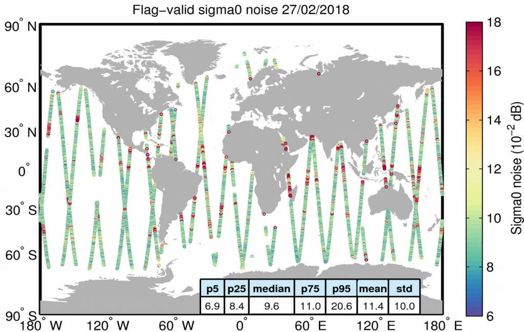
Figure 26. Geographical distribution of flag-valid 20-Hz sigma0 measurement noise over oceans and lakes for 27/02/2018. The statistical values shown in the table refer to the sigma0 noise and are calculated over all measurements shown in the figure.
