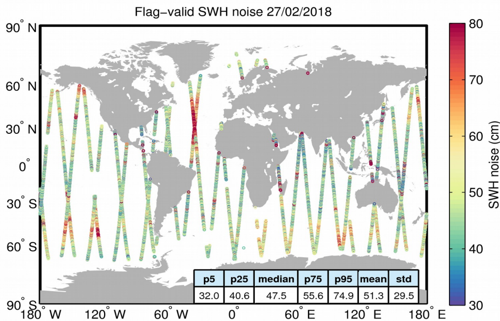
Figure 18. Geographical distribution of flag-valid 20-Hz SWH measurement noise over oceans and lakes for 27/02/2018. The statistical values shown in the figure refer to the SWH noise and are calculated over all measurements shown in the figure.
