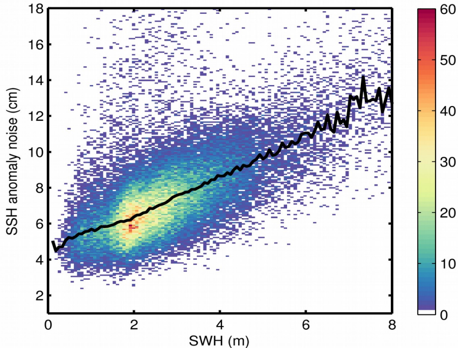
Figure 9. 2D histogram showing flag-valid SSH anomaly noise as a function of SWH for 27/02/2018. The black line denotes the median SSH anomaly noise as a function of SWH.
