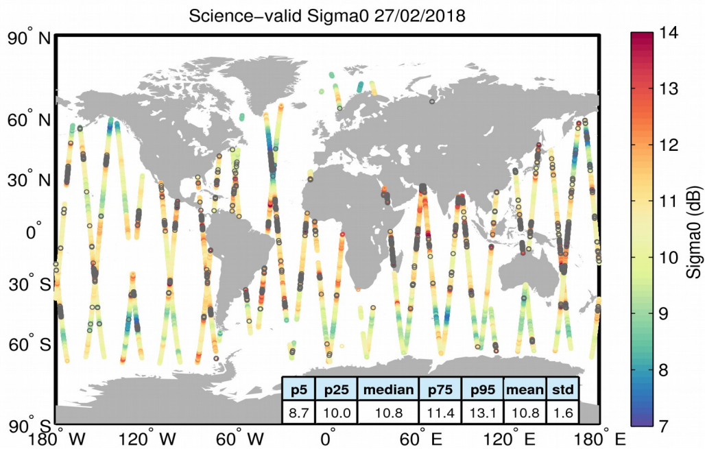
Figure 27. Geographical distribution of science-valid sigma0 data over oceans and lakes for 27/02/2018. The statistical values shown in the table refer to the sigma0 in dB and are calculated over all measurements shown in the figure. Gray circles denote records that have been rejected based on the editing criteria described in Table 4.
