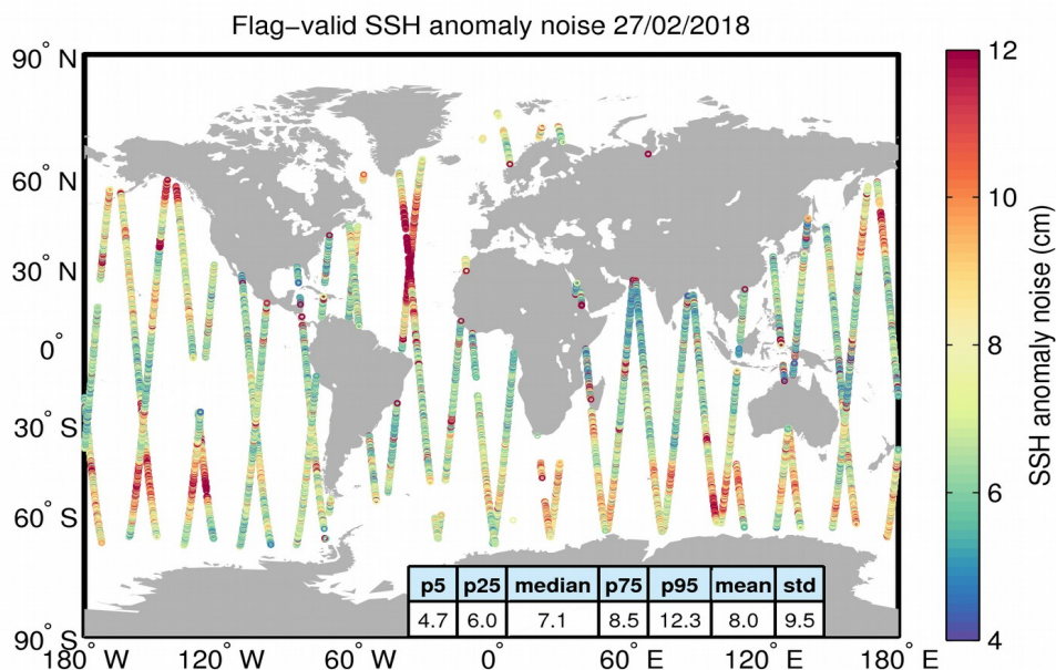
Figure 8. Geographical distribution of flag-valid 20-Hz SSH anomaly measurement noise over oceans and lakes for 27/02/2018. The statistical values shown in the table refer to the SSH anomaly noise and are calculated over all measurements shown in the figure.
