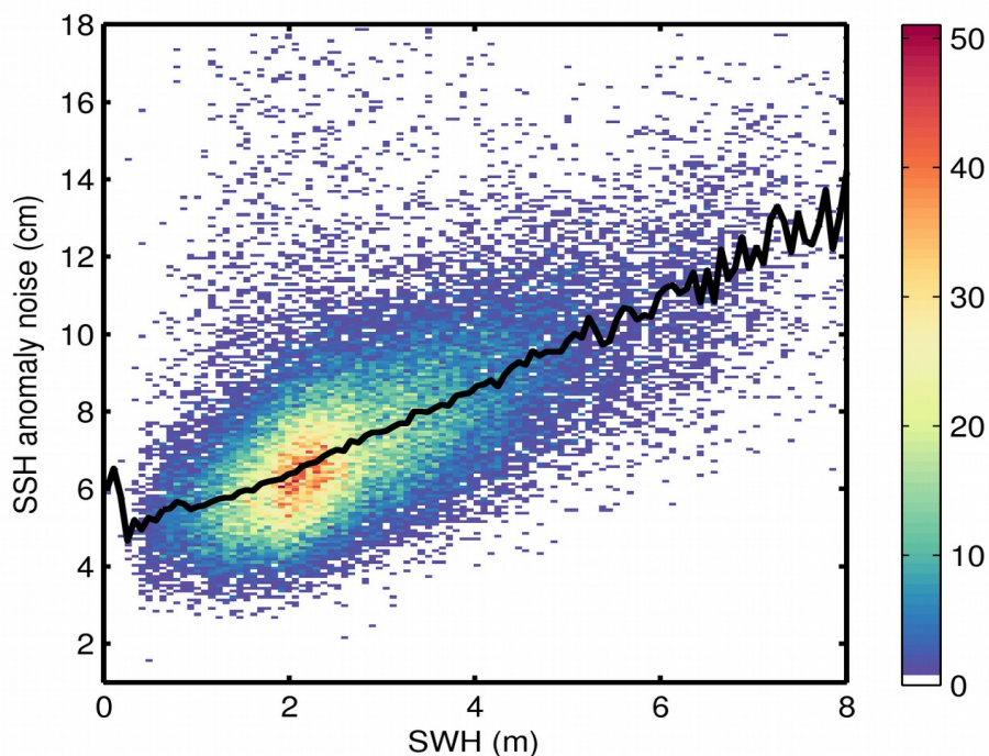
Figure 9. 2D histogram showing flag-valid SSH anomaly noise as a function of SWH for 26/02/2018. The black line denotes the median SSH anomaly noise as a function of SWH.
