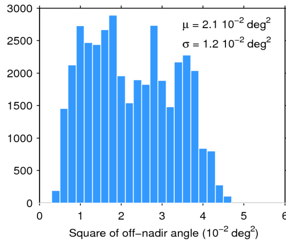
Figure 39. Histogram of flag-valid mispointing over oceans and lakes for 26/02/2018. The mean ( \mu ) and standard deviation ( \sigma ) are also shown. Note that values larger than 6 \cdot 10^{-2} \text{ deg}^2 are excluded from the histogram for the sake of readability but not from the computation of \mu and \sigma .
