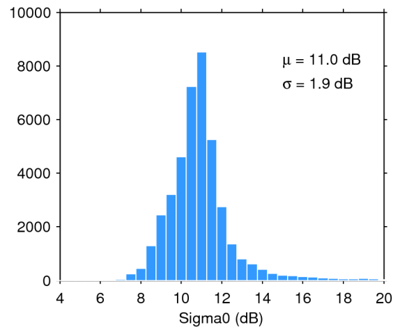
Figure 25. Histogram of flag-valid sigma0 over oceans and lakes for 26/02/2018. The mean ( \mu ) and standard deviation ( \sigma ) are also shown. Note that values outside [4 20] dB are excluded from the histogram for the sake of readability but not from the computation of \mu and \sigma .
