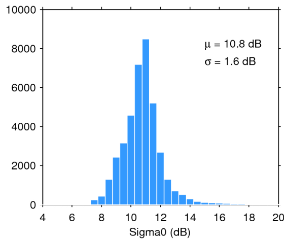
Figure 28. Histogram of science-valid sigma0 over oceans and lakes for 26/02/2018. The mean ( \mu ) and standard deviation ( \sigma ) are also shown. Note that values outside [4 20] dB are excluded from the histogram for the sake of readability but not from the computation of \mu and \sigma .
