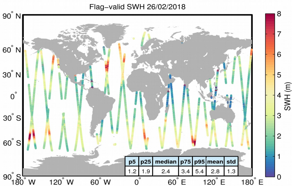
Figure 15. Geographical distribution of flag-valid SWH data over oceans and lakes for 26/02/2018. The statistical values shown in the table refer to the SWH in m and are calculated over all measurements shown in the figure.
