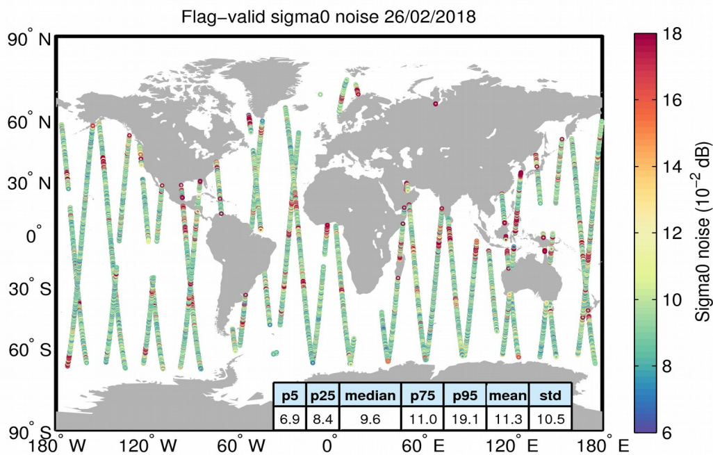
Figure 26. Geographical distribution of flag-valid 20-Hz sigma0 measurement noise over oceans and lakes for 26/02/2018. The statistical values shown in the table refer to the sigma0 noise and are calculated over all measurements shown in the figure.
