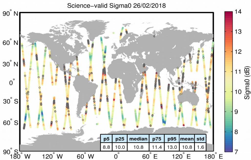
Figure 27. Geographical distribution of science-valid sigma0 data over oceans and lakes for 26/02/2018. The statistical values shown in the table refer to the sigma0 in dB and are calculated over all measurements shown in the figure. Gray circles denote records that have been rejected based on the editing criteria described in Table 4.
