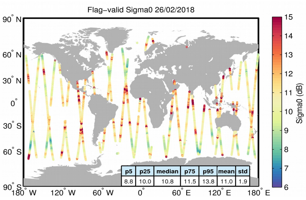
Figure 23. Geographical distribution of flag-valid sigma0 data over oceans and lakes for 26/02/2018. The statistical values shown in the table refer to the sigma0 in dB and are calculated over all measurements shown in the figure.
