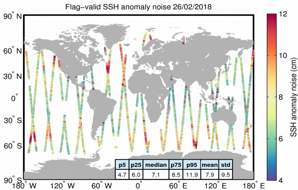
Figure 8. Geographical distribution of flag-valid 20-Hz SSH anomaly measurement noise over oceans and lakes for 26/02/2018. The statistical values shown in the table refer to the SSH anomaly noise and are calculated over all measurements shown in the figure.
