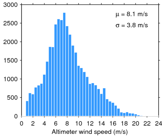
Figure 33. Histogram of flag-valid wind over oceans and lakes for 26/02/2018. The mean ( \mu ) and standard deviation ( \sigma ) are also shown. Note that values larger than 24 m/s are excluded from the histogram for the sake of readability but not from the computation of \mu and \sigma .
