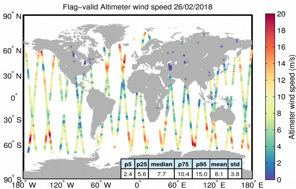
Figure 31. Geographical distribution of flag-valid wind data over oceans and lakes for 26/02/2018. The statistical values shown in the table refer to the wind in m/s and are calculated over all measurements shown in the figure.
