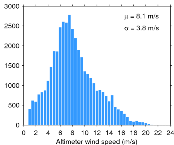
Figure 35. Histogram of science-valid wind over oceans and lakes for 26/02/2018. The mean ( \mu ) and standard deviation ( \sigma ) are also shown. Note that values larger than 24 m/s are excluded from the histogram for the sake of readability but not from the computation of \mu and \sigma .
