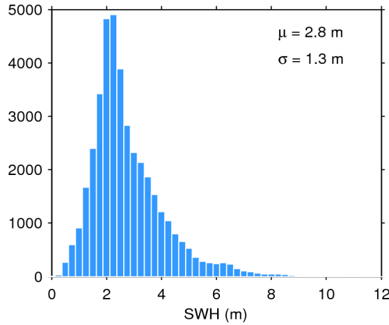
Figure 20. Histogram of science-valid SWH over oceans and lakes for 26/02/2018. The mean ( \mu ) and standard deviation ( \sigma ) are also shown. Note that values larger than 12 m are excluded from the histogram for the sake of readability but not from the computation of \mu and \sigma .
