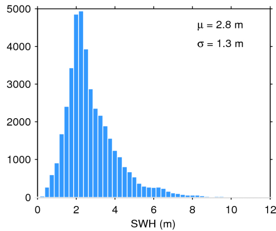
Figure 17. Histogram of flag-valid SWH over oceans and lakes for 26/02/2018. The mean ( \mu ) and standard deviation ( \sigma ) are also shown. Note that values larger than 12 m are excluded from the histogram for the sake of readability but not from the computation of \mu and \sigma .
