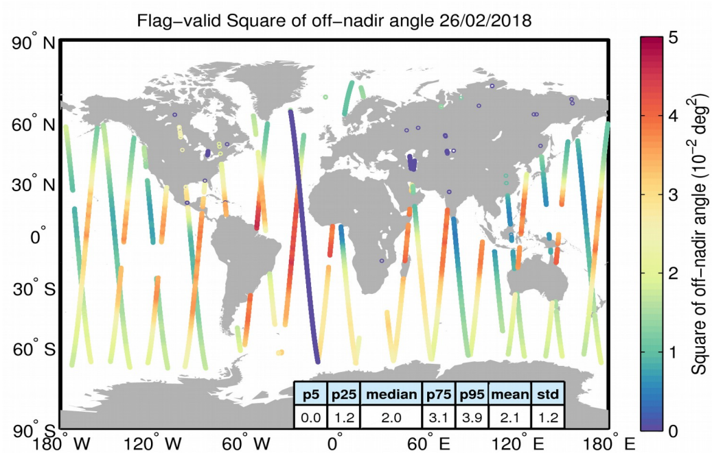
Figure 37. Geographical distribution of flag-valid mispointing data over oceans and lakes for 26/02/2018. The statistical values shown in the table refer to the mispointing in 10^{-2} \text{ deg}^2 and are calculated over all measurements shown in the figure.
