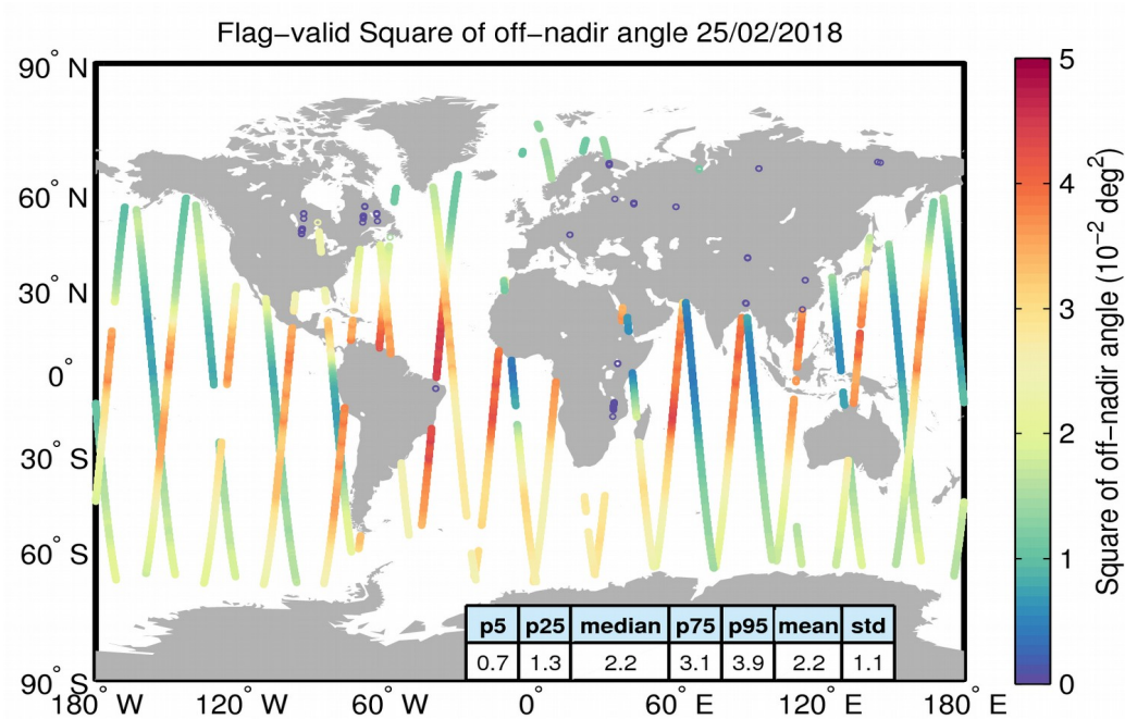
Figure 37. Geographical distribution of flag-valid mispointing data over oceans and lakes for 25/02/2018. The statistical values shown in the table refer to the mispointing in 10^{-2} \text{ deg}^2 and are calculated over all measurements shown in the figure.
