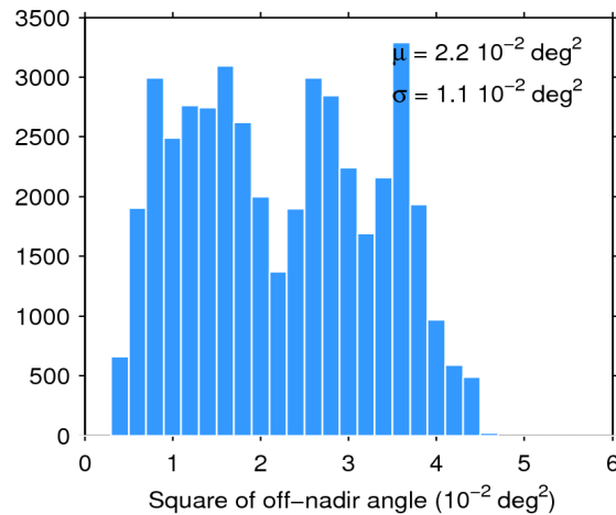
Figure 39. Histogram of flag-valid mispointing over oceans and lakes for 25/02/2018. The mean ( \mu ) and standard deviation ( \sigma ) are also shown. Note that values larger than 6 \cdot 10^{-2} \text{ deg}^2 are excluded from the histogram for the sake of readability but not from the computation of \mu and \sigma .
