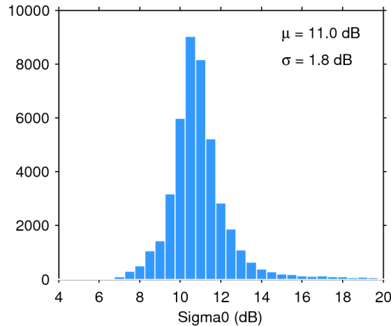
Figure 25. Histogram of flag-valid sigma0 over oceans and lakes for 25/02/2018. The mean ( \mu ) and standard deviation ( \sigma ) are also shown. Note that values outside [4 20] dB are excluded from the histogram for the sake of readability but not from the computation of \mu and \sigma .
