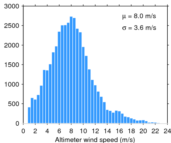
Figure 35. Histogram of science-valid wind over oceans and lakes for 25/02/2018. The mean ( \mu ) and standard deviation ( \sigma ) are also shown. Note that values larger than 24 m/s are excluded from the histogram for the sake of readability but not from the computation of \mu and \sigma .
