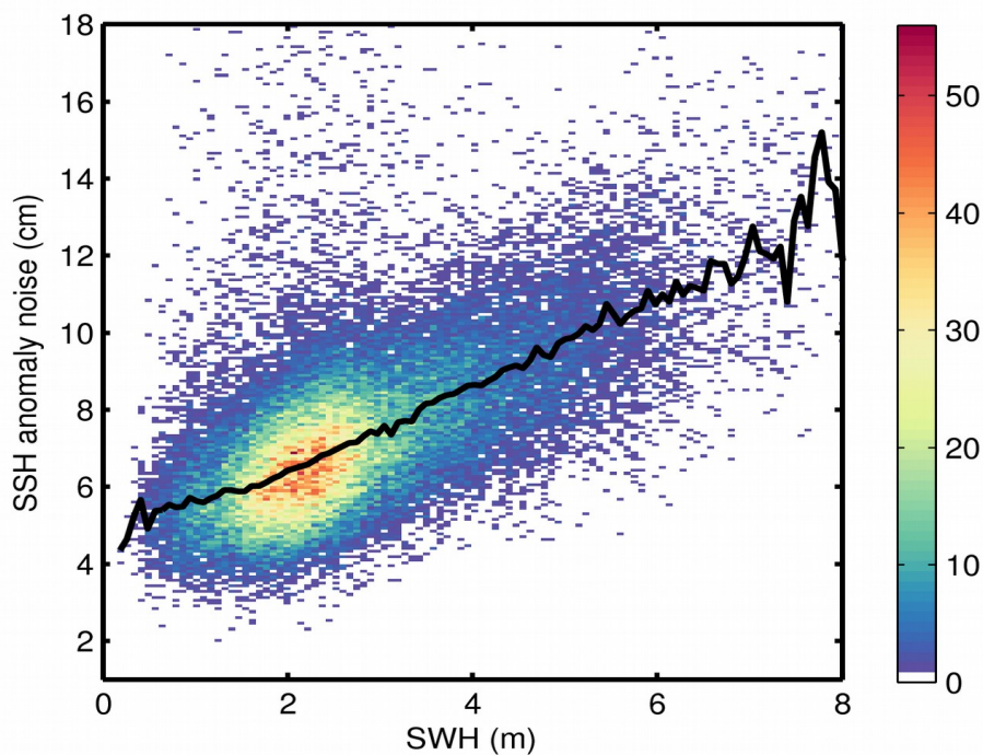
Figure 9. 2D histogram showing flag-valid SSH anomaly noise as a function of SWH for 25/02/2018. The black line denotes the median SSH anomaly noise as a function of SWH.
