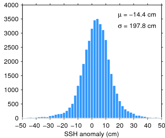
Figure 7. Histogram of flag-valid SSH anomaly over oceans and lakes for 25/02/2018. The mean ( \mu ) and standard deviation ( \sigma ) are also shown. Note that values outside [-50 50] cm are excluded from the histogram for the sake of readability but not from the computation of \mu and \sigma .
