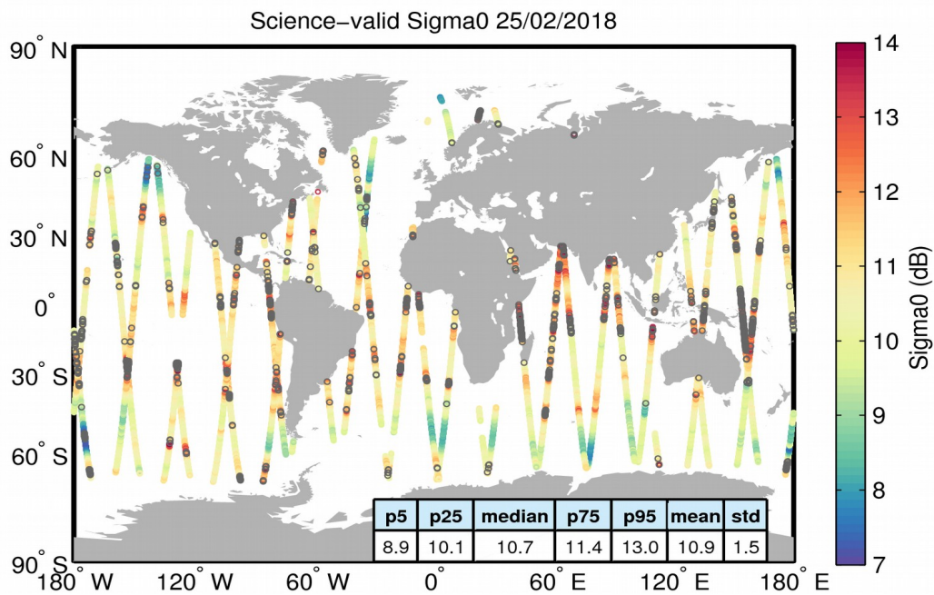
Figure 27. Geographical distribution of science-valid sigma0 data over oceans and lakes for 25/02/2018. The statistical values shown in the table refer to the sigma0 in dB and are calculated over all measurements shown in the figure. Gray circles denote records that have been rejected based on the editing criteria described in Table 4.
