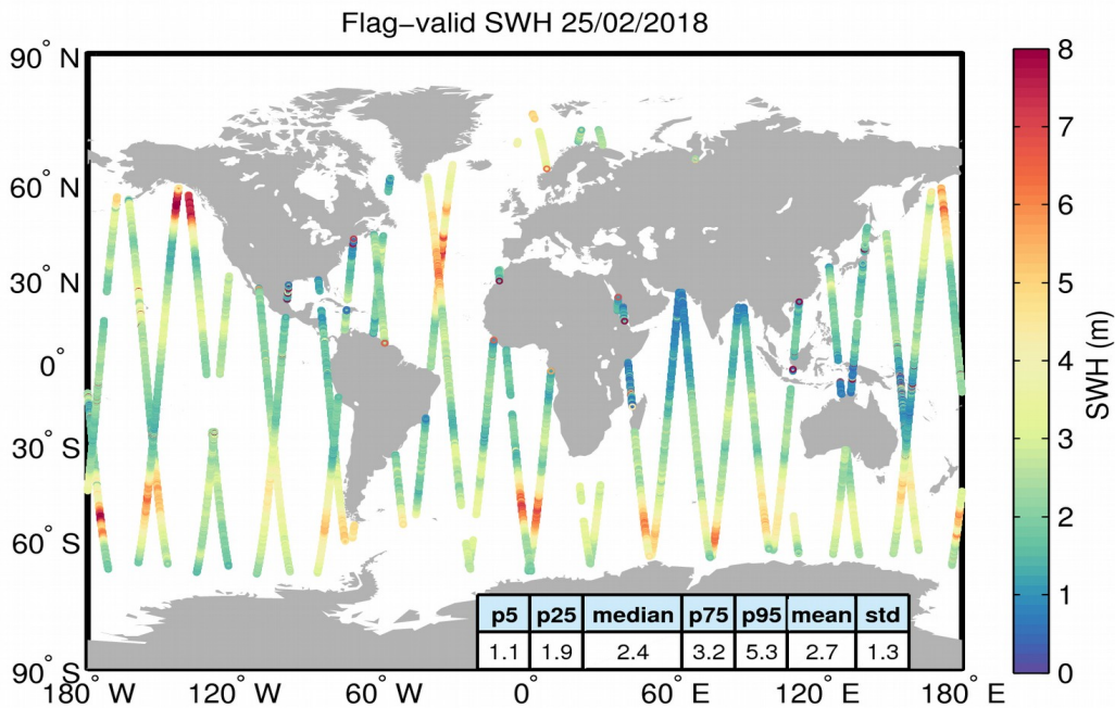
Figure 15. Geographical distribution of flag-valid SWH data over oceans and lakes for 25/02/2018. The statistical values shown in the table refer to the SWH in m and are calculated over all measurements shown in the figure.
