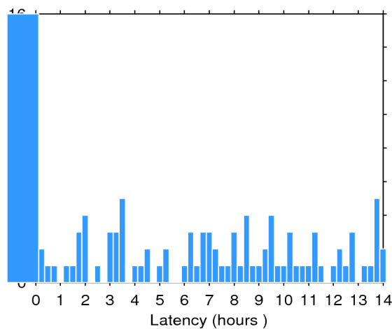
Figure 2. Histogram of the data latency for 25/02/2018. The y-axis denotes the number of files that are made available with a delay of x-hours with respect to the mean time of the records stored in the file.
