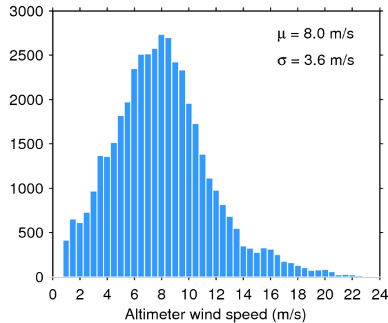
Figure 33. Histogram of flag-valid wind over oceans and lakes for 25/02/2018. The mean ( \mu ) and standard deviation ( \sigma ) are also shown. Note that values larger than 24 m/s are excluded from the histogram for the sake of readability but not from the computation of \mu and \sigma .
