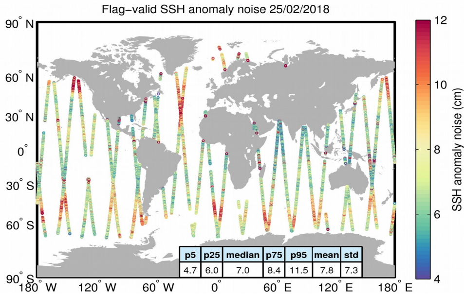
Figure 8. Geographical distribution of flag-valid 20-Hz SSH anomaly measurement noise over oceans and lakes for 25/02/2018. The statistical values shown in the table refer to the SSH anomaly noise and are calculated over all measurements shown in the figure.
