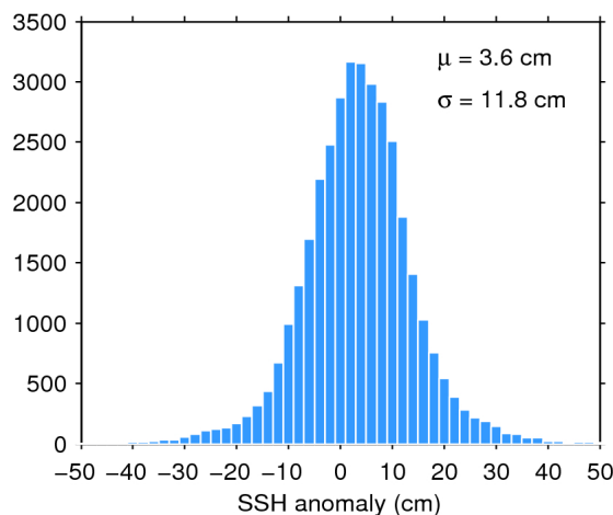
Figure 11. Histogram of science-valid SSH anomaly over oceans and lakes for 25/02/2018. The mean ( \mu ) and standard deviation ( \sigma ) are also shown. Note that values outside [-50 50] cm are excluded from the histogram for the sake of readability but not from the computation of \mu and \sigma .
