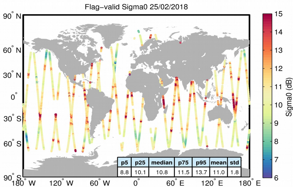
Figure 23. Geographical distribution of flag-valid sigma0 data over oceans and lakes for 25/02/2018. The statistical values shown in the table refer to the sigma0 in dB and are calculated over all measurements shown in the figure.
