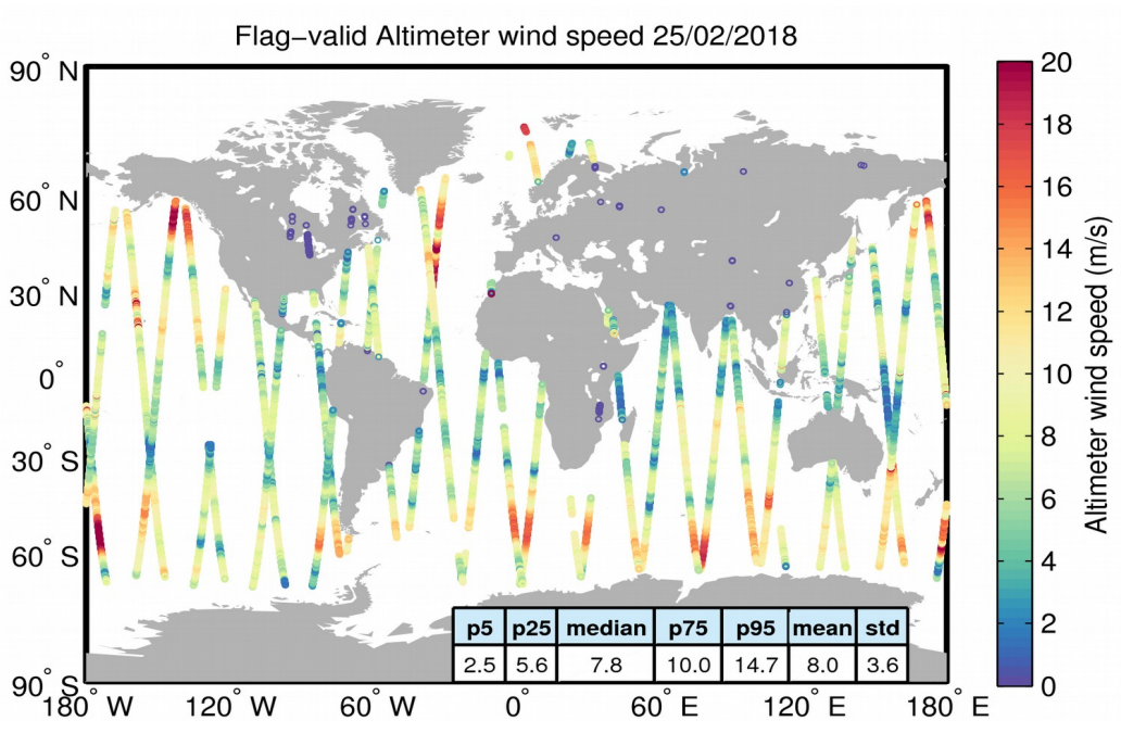
Figure 31. Geographical distribution of flag-valid wind data over oceans and lakes for 25/02/2018. The statistical values shown in the table refer to the wind in m/s and are calculated over all measurements shown in the figure.
