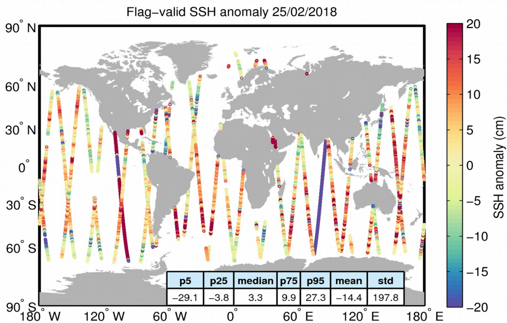
Figure 5. Geographical distribution of flag-valid 1-Hz SSH anomaly data over oceans and lakes for 25/02/2018. The statistical values shown in the table refer to the SSH anomaly in cm and are calculated over all measurements shown in the figure.
