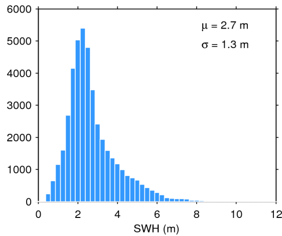
Figure 17. Histogram of flag-valid SWH over oceans and lakes for 25/02/2018. The mean ( \mu ) and standard deviation ( \sigma ) are also shown. Note that values larger than 12 m are excluded from the histogram for the sake of readability but not from the computation of \mu and \sigma .
