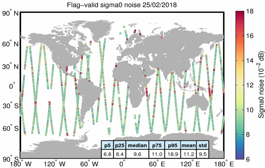
Figure 26. Geographical distribution of flag-valid 20-Hz sigma0 measurement noise over oceans and lakes for 25/02/2018. The statistical values shown in the table refer to the sigma0 noise and are calculated over all measurements shown in the figure.
