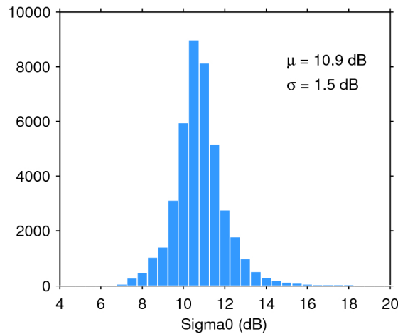
Figure 28. Histogram of science-valid sigma0 over oceans and lakes for 25/02/2018. The mean ( \mu ) and standard deviation ( \sigma ) are also shown. Note that values outside [4 20] dB are excluded from the histogram for the sake of readability but not from the computation of \mu and \sigma .
