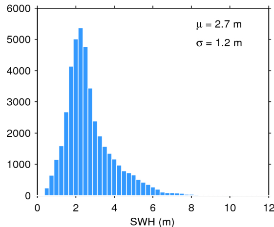
Figure 20. Histogram of science-valid SWH over oceans and lakes for 25/02/2018. The mean ( \mu ) and standard deviation ( \sigma ) are also shown. Note that values larger than 12 m are excluded from the histogram for the sake of readability but not from the computation of \mu and \sigma .
