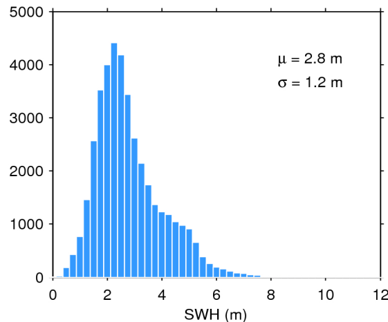
Figure 20. Histogram of science-valid SWH over oceans and lakes for 24/02/2018. The mean ( \mu ) and standard deviation ( \sigma ) are also shown. Note that values larger than 12 m are excluded from the histogram for the sake of readability but not from the computation of \mu and \sigma .
