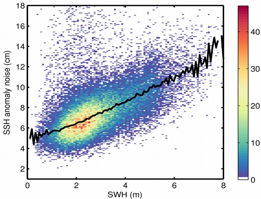
Figure 9. 2D histogram showing flag-valid SSH anomaly noise as a function of SWH for 24/02/2018. The black line denotes the median SSH anomaly noise as a function of SWH.
