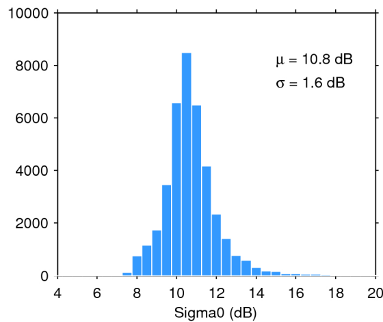
Figure 28. Histogram of science-valid sigma0 over oceans and lakes for 24/02/2018. The mean ( \mu ) and standard deviation ( \sigma ) are also shown. Note that values outside [4 20] dB are excluded from the histogram for the sake of readability but not from the computation of \mu and \sigma .
