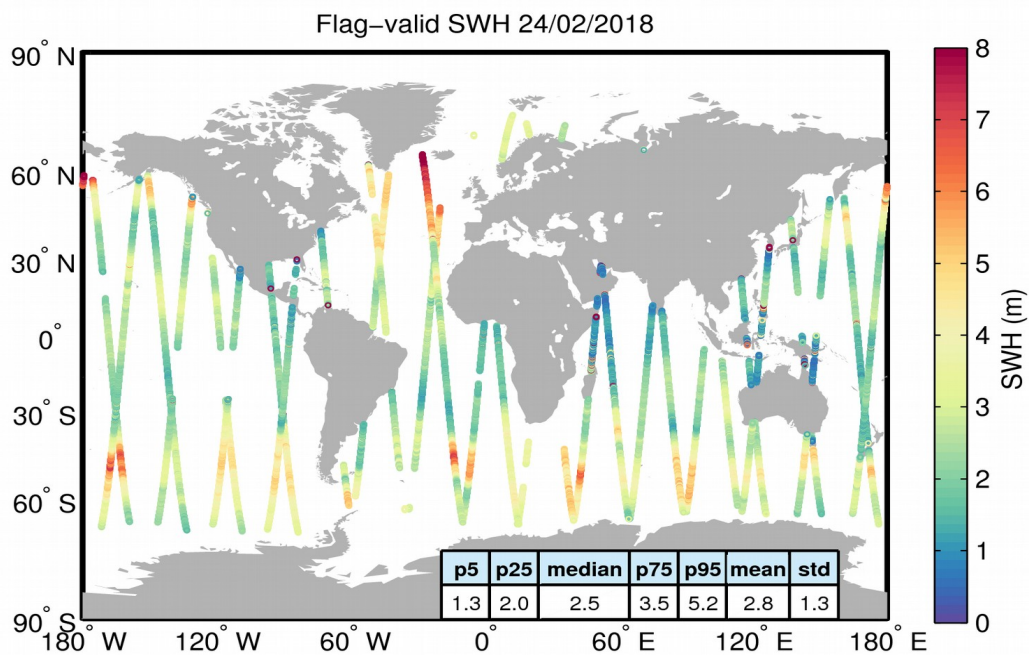
Figure 15. Geographical distribution of flag-valid SWH data over oceans and lakes for 24/02/2018. The statistical values shown in the table refer to the SWH in m and are calculated over all measurements shown in the figure.
