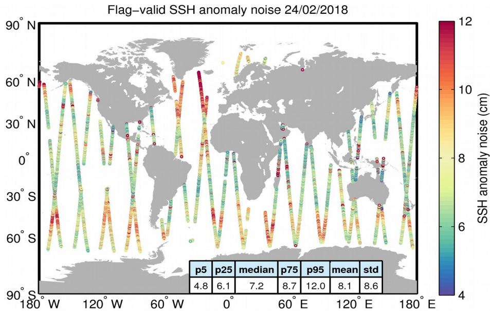
Figure 8. Geographical distribution of flag-valid 20-Hz SSH anomaly measurement noise over oceans and lakes for 24/02/2018. The statistical values shown in the table refer to the SSH anomaly noise and are calculated over all measurements shown in the figure.
