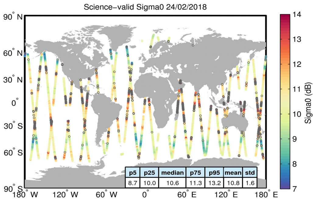
Figure 27. Geographical distribution of science-valid sigma0 data over oceans and lakes for 24/02/2018. The statistical values shown in the table refer to the sigma0 in dB and are calculated over all measurements shown in the figure. Gray circles denote records that have been rejected based on the editing criteria described in Table 4.
