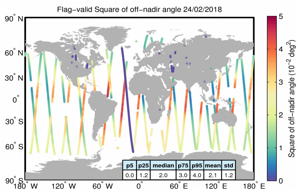
Figure 37. Geographical distribution of flag-valid mispointing data over oceans and lakes for 24/02/2018. The statistical values shown in the table refer to the mispointing in 10^{-2} \text{ deg}^2 and are calculated over all measurements shown in the figure.
