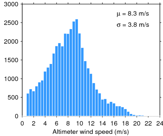
Figure 33. Histogram of flag-valid wind over oceans and lakes for 24/02/2018. The mean ( \mu ) and standard deviation ( \sigma ) are also shown. Note that values larger than 24 m/s are excluded from the histogram for the sake of readability but not from the computation of \mu and \sigma .
