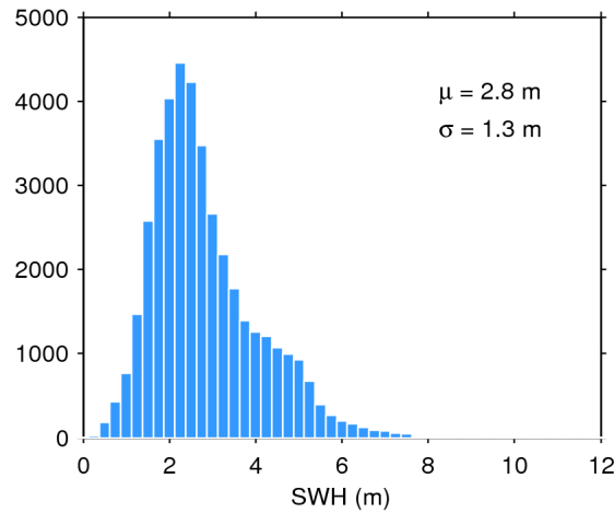
Figure 17. Histogram of flag-valid SWH over oceans and lakes for 24/02/2018. The mean ( \mu ) and standard deviation ( \sigma ) are also shown. Note that values larger than 12 m are excluded from the histogram for the sake of readability but not from the computation of \mu and \sigma .
