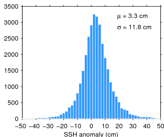
Figure 11. Histogram of science-valid SSH anomaly over oceans and lakes for 24/02/2018. The mean ( \mu ) and standard deviation ( \sigma ) are also shown. Note that values outside [-50 50] cm are excluded from the histogram for the sake of readability but not from the computation of \mu and \sigma .
