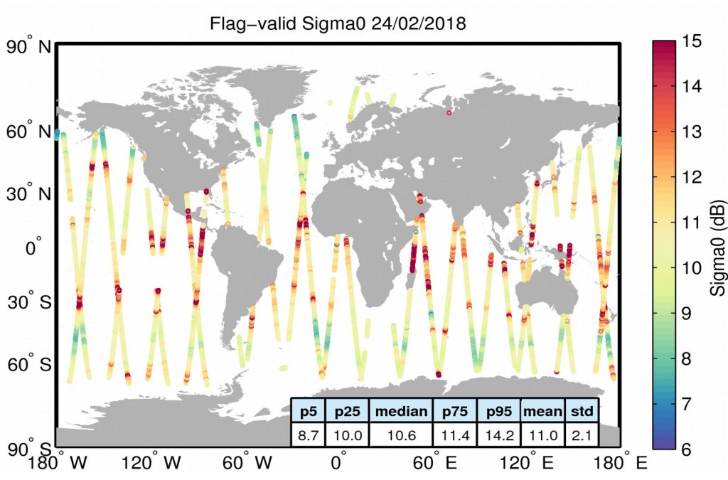
Figure 23. Geographical distribution of flag-valid sigma0 data over oceans and lakes for 24/02/2018. The statistical values shown in the table refer to the sigma0 in dB and are calculated over all measurements shown in the figure.
