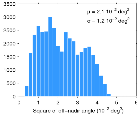
Figure 39. Histogram of flag-valid mispointing over oceans and lakes for 24/02/2018. The mean ( \mu ) and standard deviation ( \sigma ) are also shown. Note that values larger than 6 \cdot 10^{-2} \text{ deg}^2 are excluded from the histogram for the sake of readability but not from the computation of \mu and \sigma .
