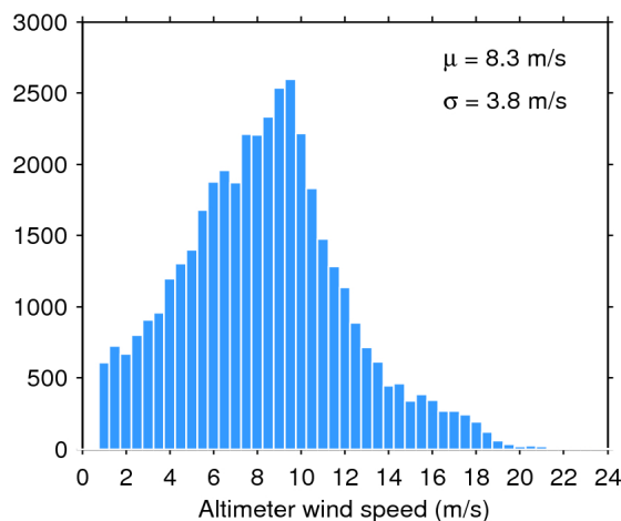
Figure 35. Histogram of science-valid wind over oceans and lakes for 24/02/2018. The mean ( \mu ) and standard deviation ( \sigma ) are also shown. Note that values larger than 24 m/s are excluded from the histogram for the sake of readability but not from the computation of \mu and \sigma .
