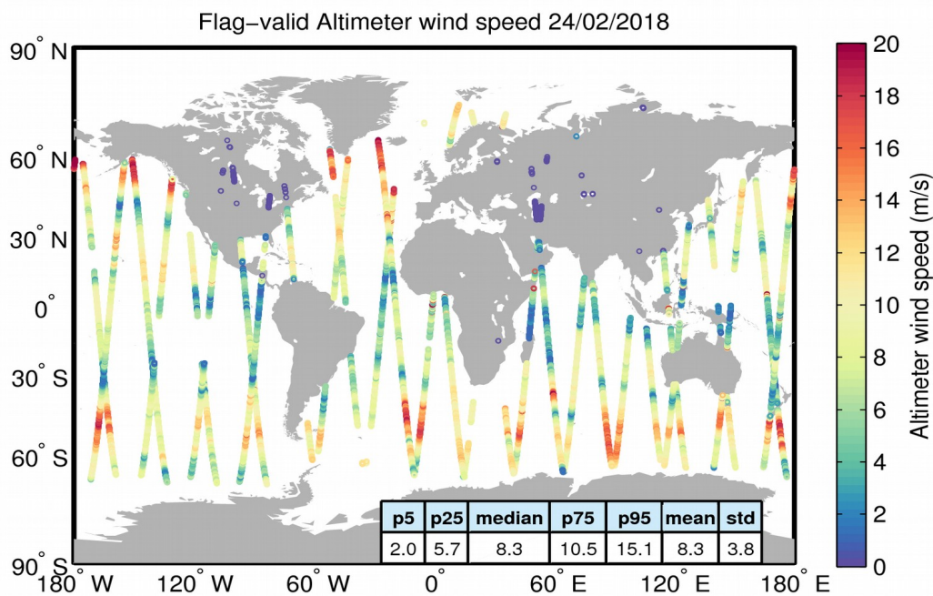
Figure 31. Geographical distribution of flag-valid wind data over oceans and lakes for 24/02/2018. The statistical values shown in the table refer to the wind in m/s and are calculated over all measurements shown in the figure.
