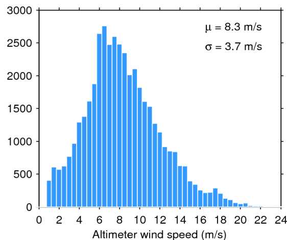
Figure 35. Histogram of science-valid wind over oceans and lakes for 23/02/2018. The mean ( \mu ) and standard deviation ( \sigma ) are also shown. Note that values larger than 24 m/s are excluded from the histogram for the sake of readability but not from the computation of \mu and \sigma .
