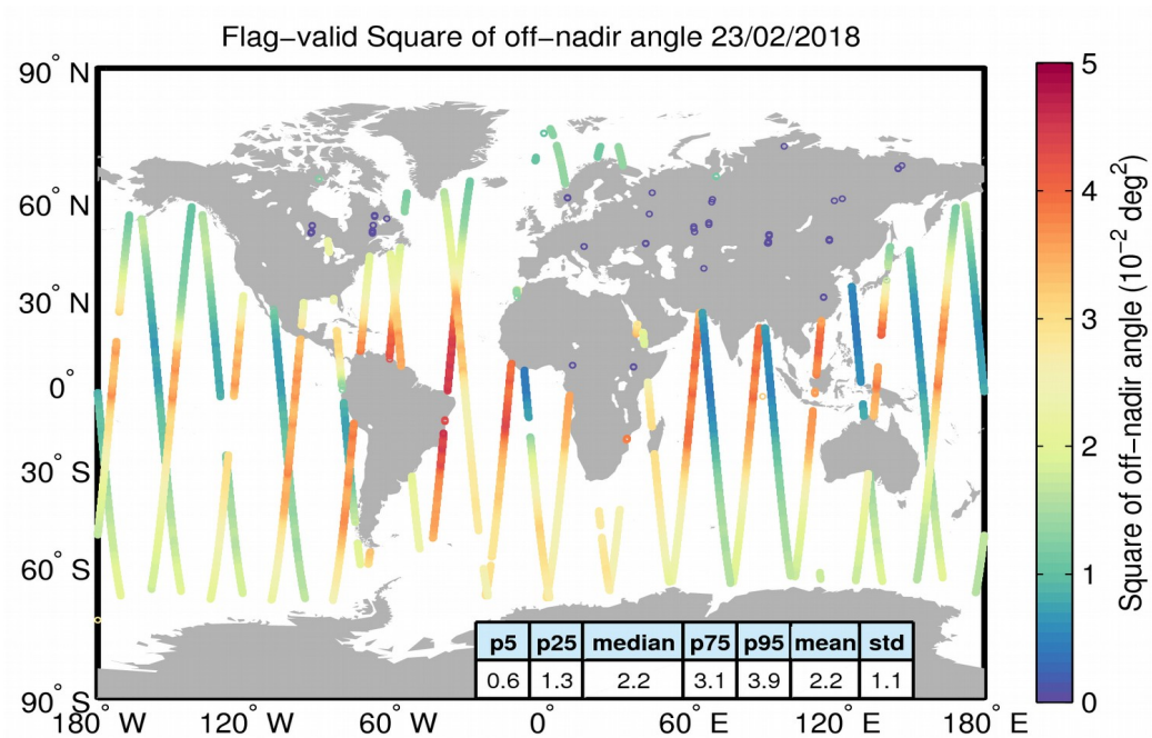
Figure 37. Geographical distribution of flag-valid mispointing data over oceans and lakes for 23/02/2018. The statistical values shown in the table refer to the mispointing in 10^{-2} \text{deg}^2 and are calculated over all measurements shown in the figure.
