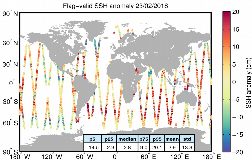
Figure 5. Geographical distribution of flag-valid 1-Hz SSH anomaly data over oceans and lakes for 23/02/2018. The statistical values shown in the table refer to the SSH anomaly in cm and are calculated over all measurements shown in the figure.
