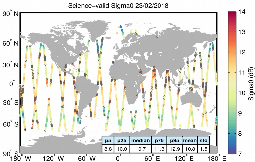
Figure 27. Geographical distribution of science-valid sigma0 data over oceans and lakes for 23/02/2018. The statistical values shown in the table refer to the sigma0 in dB and are calculated over all measurements shown in the figure. Gray circles denote records that have been rejected based on the editing criteria described in Table 4.
