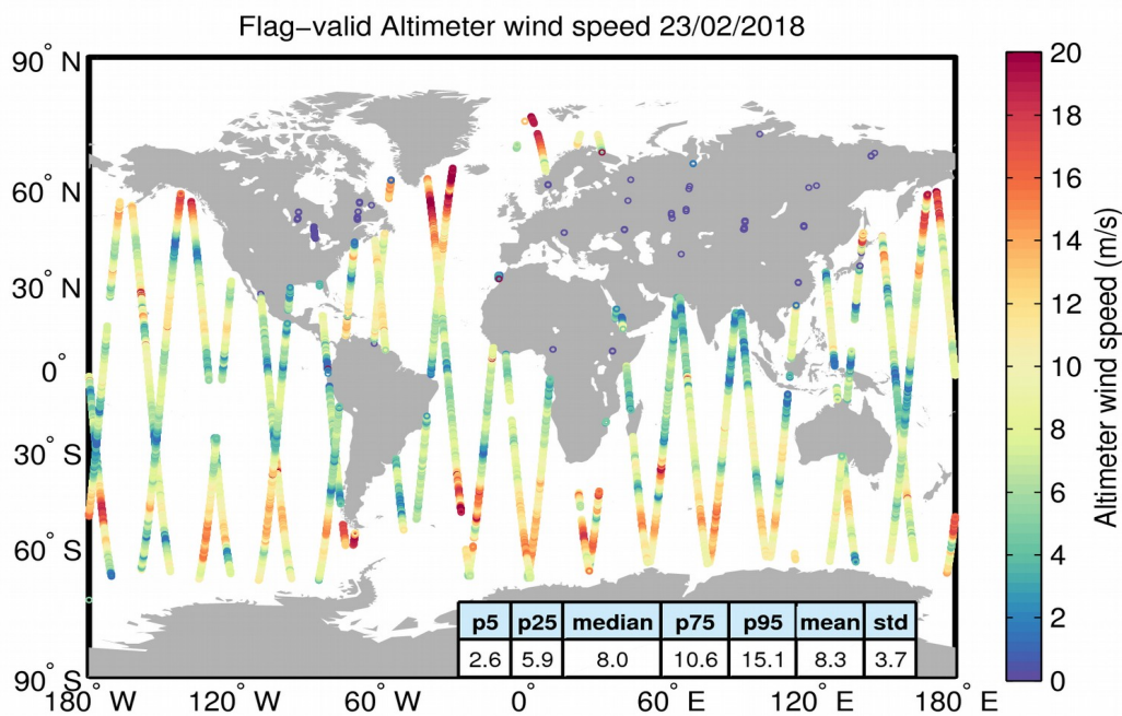
Figure 31. Geographical distribution of flag-valid wind data over oceans and lakes for 23/02/2018. The statistical values shown in the table refer to the wind in m/s and are calculated over all measurements shown in the figure.
