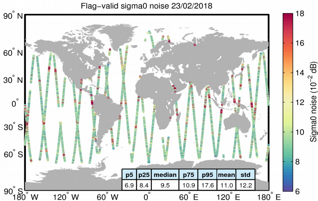
Figure 26. Geographical distribution of flag-valid 20-Hz sigma0 measurement noise over oceans and lakes for 23/02/2018. The statistical values shown in the table refer to the sigma0 noise and are calculated over all measurements shown in the figure.
