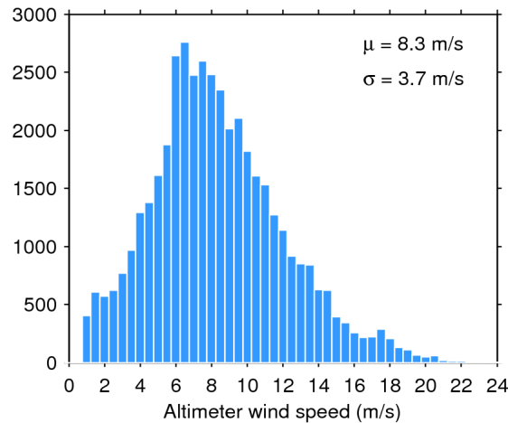
Figure 33. Histogram of flag-valid wind over oceans and lakes for 23/02/2018. The mean ( \mu ) and standard deviation ( \sigma ) are also shown. Note that values larger than 24 m/s are excluded from the histogram for the sake of readability but not from the computation of \mu and \sigma .
