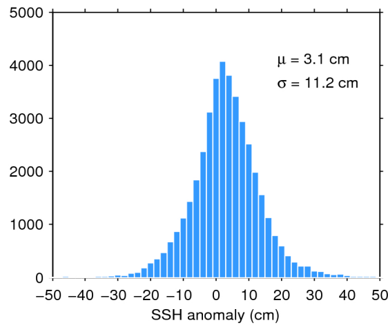
Figure 11. Histogram of science-valid SSH anomaly over oceans and lakes for 23/02/2018. The mean ( \mu ) and standard deviation ( \sigma ) are also shown. Note that values outside [-50 50] cm are excluded from the histogram for the sake of readability but not from the computation of \mu and \sigma .
