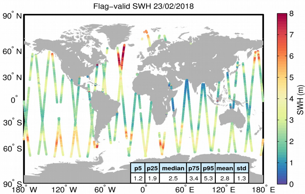
Figure 15. Geographical distribution of flag-valid SWH data over oceans and lakes for 23/02/2018. The statistical values shown in the table refer to the SWH in m and are calculated over all measurements shown in the figure.
