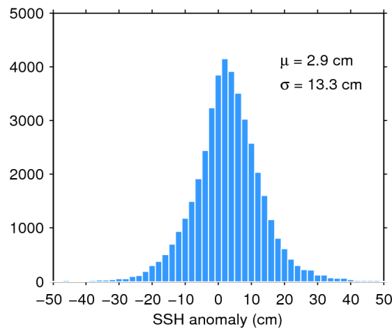
Figure 7. Histogram of flag-valid SSH anomaly over oceans and lakes for 23/02/2018. The mean ( \mu ) and standard deviation ( \sigma ) are also shown. Note that values outside [-50 50] cm are excluded from the histogram for the sake of readability but not from the computation of \mu and \sigma .
