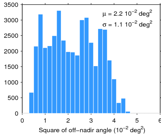
Figure 39. Histogram of flag-valid mispointing over oceans and lakes for 23/02/2018. The mean ( \mu ) and standard deviation ( \sigma ) are also shown. Note that values larger than 6 \cdot 10^{-2} \text{ deg}^2 are excluded from the histogram for the sake of readability but not from the computation of \mu and \sigma .
