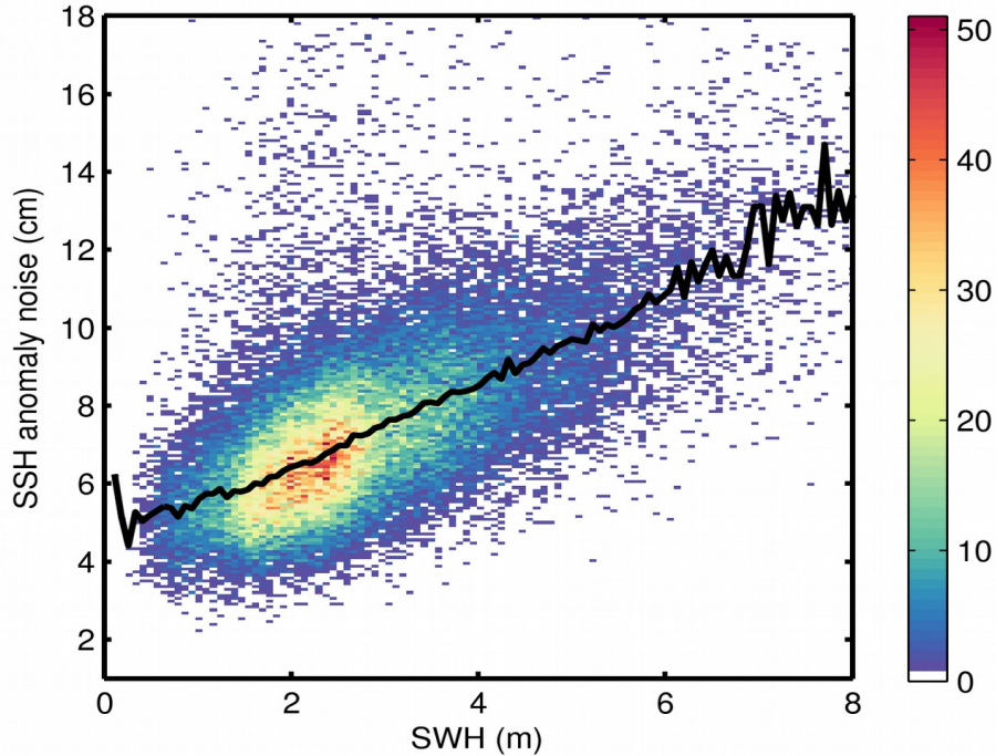
Figure 9. 2D histogram showing flag-valid SSH anomaly noise as a function of SWH for 23/02/2018. The black line denotes the median SSH anomaly noise as a function of SWH.
