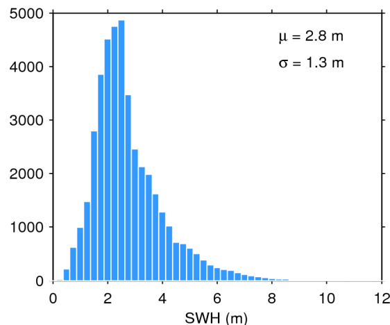
Figure 20. Histogram of science-valid SWH over oceans and lakes for 23/02/2018. The mean ( \mu ) and standard deviation ( \sigma ) are also shown. Note that values larger than 12 m are excluded from the histogram for the sake of readability but not from the computation of \mu and \sigma .
