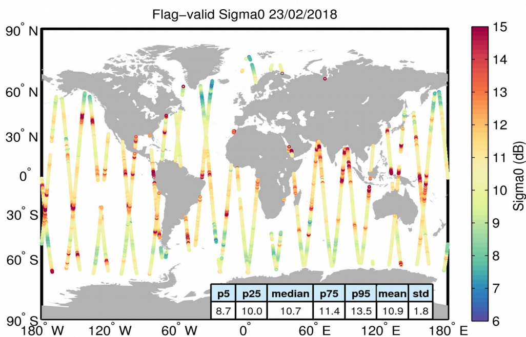
Figure 23. Geographical distribution of flag-valid sigma0 data over oceans and lakes for 23/02/2018. The statistical values shown in the table refer to the sigma0 in dB and are calculated over all measurements shown in the figure.
