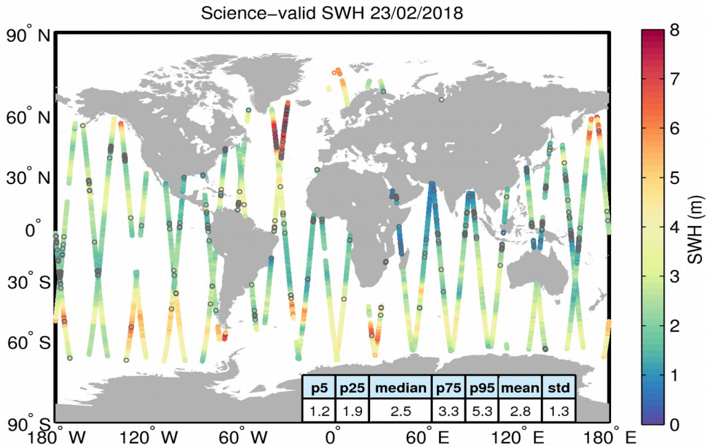
Figure 19. Geographical distribution of science-valid SWH data over oceans and lakes for 23/02/2018. The statistical values shown in the table refer to the SWH in m and are calculated over all measurements shown in the figure. Gray circles denote records that have been rejected based on the editing criteria described in Table 3.
