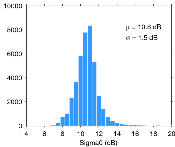
Figure 28. Histogram of science-valid sigma0 over oceans and lakes for 23/02/2018. The mean ( \mu ) and standard deviation ( \sigma ) are also shown. Note that values outside [4 20] dB are excluded from the histogram for the sake of readability but not from the computation of \mu and \sigma .
