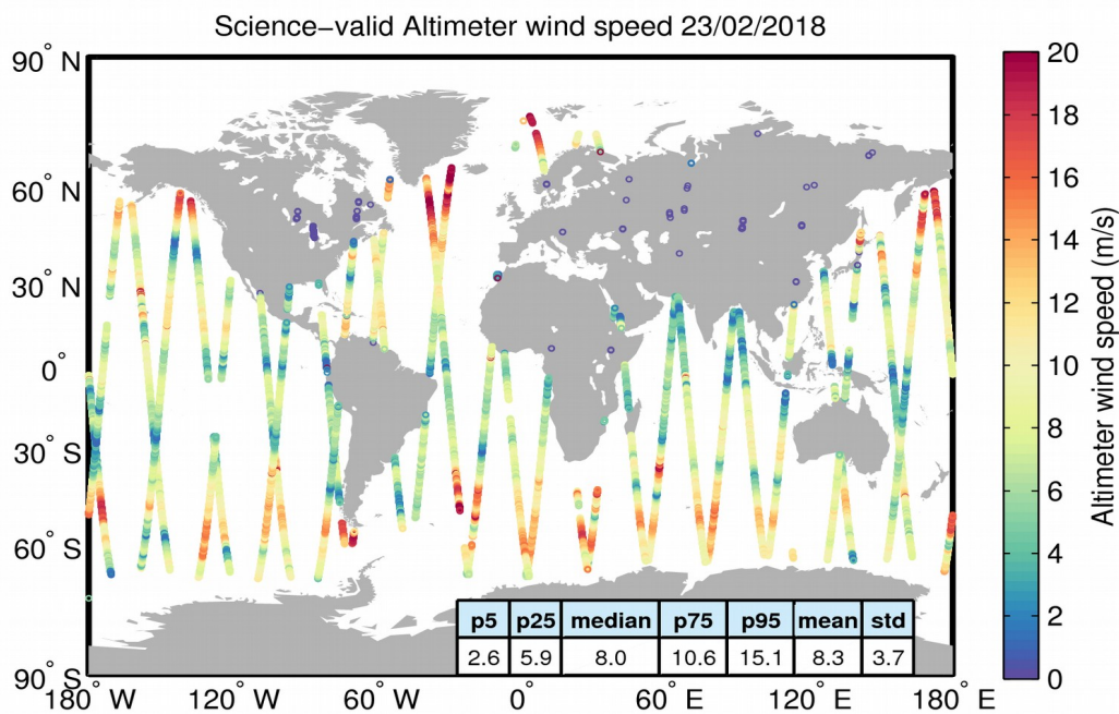
Figure 34. Geographical distribution of science-valid wind data over oceans and lakes for 23/02/2018. The statistical values shown in the table refer to the wind in m/s and are calculated over all measurements shown in the figure. Gray circles denote records that have been rejected based on the editing criteria described in Table 5.
