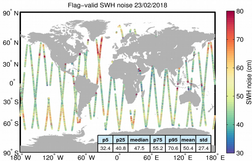
Figure 18. Geographical distribution of flag-valid 20-Hz SWH measurement noise over oceans and lakes for 23/02/2018. The statistical values shown in the figure refer to the SWH noise and are calculated over all measurements shown in the figure.
