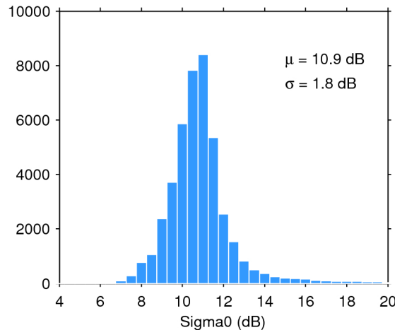
Figure 25. Histogram of flag-valid sigma0 over oceans and lakes for 23/02/2018. The mean ( \mu ) and standard deviation ( \sigma ) are also shown. Note that values outside [4 20] dB are excluded from the histogram for the sake of readability but not from the computation of \mu and \sigma .
