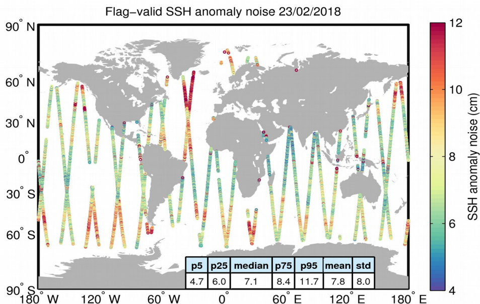
Figure 8. Geographical distribution of flag-valid 20-Hz SSH anomaly measurement noise over oceans and lakes for 23/02/2018. The statistical values shown in the table refer to the SSH anomaly noise and are calculated over all measurements shown in the figure.
