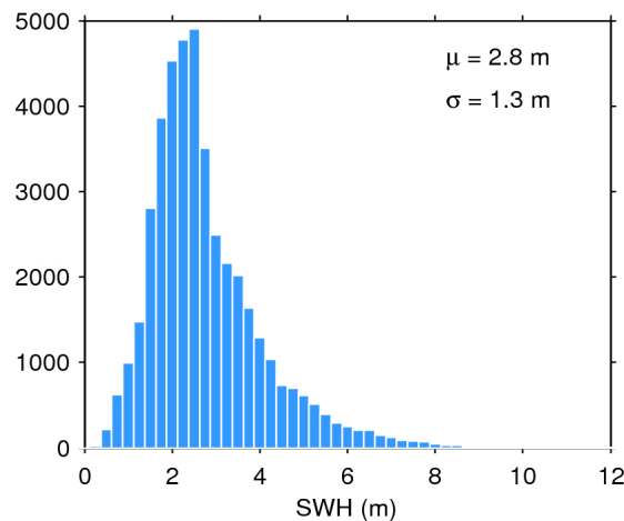
Figure 17. Histogram of flag-valid SWH over oceans and lakes for 23/02/2018. The mean ( \mu ) and standard deviation ( \sigma ) are also shown. Note that values larger than 12 m are excluded from the histogram for the sake of readability but not from the computation of \mu and \sigma .
