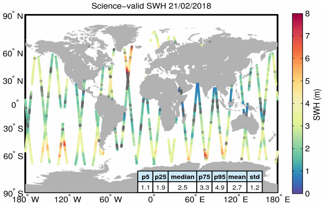
Figure 19. Geographical distribution of science-valid SWH data over oceans and lakes for 21/02/2018. The statistical values shown in the table refer to the SWH in m and are calculated over all measurements shown in the figure. Gray circles denote records that have been rejected based on the editing criteria described in Table 3.
