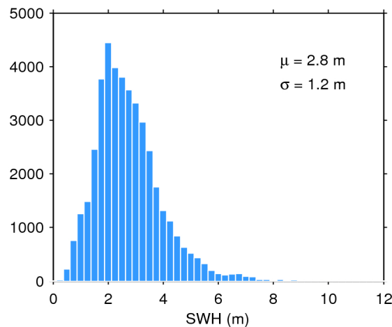
Figure 17. Histogram of flag-valid SWH over oceans and lakes for 21/02/2018. The mean ( \mu ) and standard deviation ( \sigma ) are also shown. Note that values larger than 12 m are excluded from the histogram for the sake of readability but not from the computation of \mu and \sigma .
