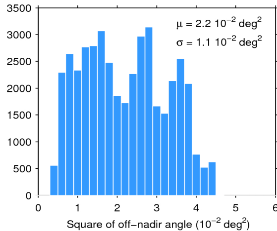
Figure 39. Histogram of flag-valid mispointing over oceans and lakes for 21/02/2018. The mean ( \mu ) and standard deviation ( \sigma ) are also shown. Note that values larger than 6 \cdot 10^{-2} \text{ deg}^2 are excluded from the histogram for the sake of readability but not from the computation of \mu and \sigma .
