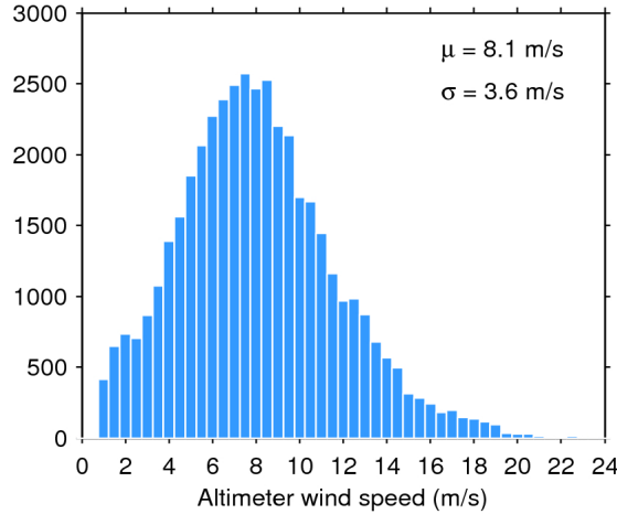
Figure 33. Histogram of flag-valid wind over oceans and lakes for 21/02/2018. The mean ( \mu ) and standard deviation ( \sigma ) are also shown. Note that values larger than 24 m/s are excluded from the histogram for the sake of readability but not from the computation of \mu and \sigma .
