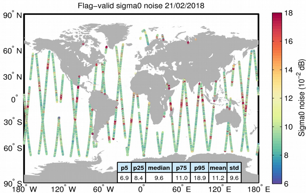
Figure 26. Geographical distribution of flag-valid 20-Hz sigma0 measurement noise over oceans and lakes for 21/02/2018. The statistical values shown in the table refer to the sigma0 noise and are calculated over all measurements shown in the figure.
