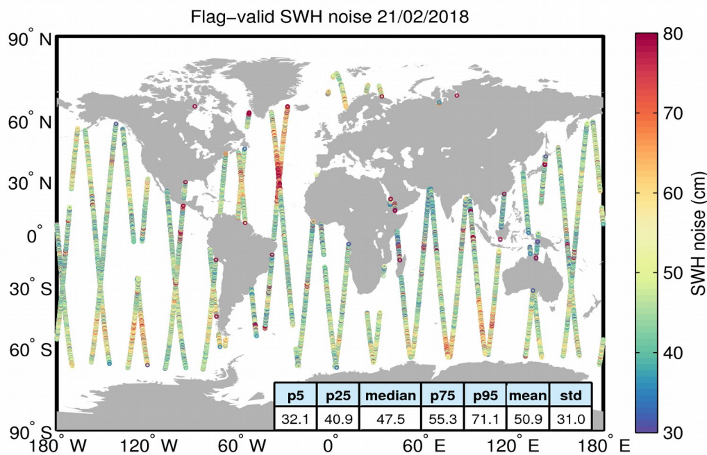
Figure 18. Geographical distribution of flag-valid 20-Hz SWH measurement noise over oceans and lakes for 21/02/2018. The statistical values shown in the table refer to the SWH noise and are calculated over all measurements shown in the figure.
