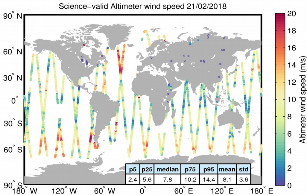
Figure 34. Geographical distribution of science-valid wind data over oceans and lakes for 21/02/2018. The statistical values shown in the table refer to the wind in m/s and are calculated over all measurements shown in the figure. Gray circles denote records that have been rejected based on the editing criteria described in Table 5.
