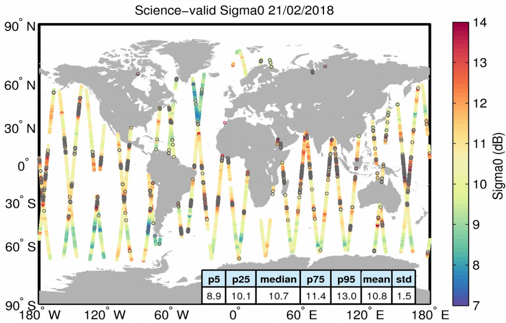
Figure 27. Geographical distribution of science-valid sigma0 data over oceans and lakes for 21/02/2018. The statistical values shown in the table refer to the sigma0 in dB and are calculated over all measurements shown in the figure. Gray circles denote records that have been rejected based on the editing criteria described in Table 4.
