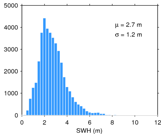
Figure 20. Histogram of science-valid SWH over oceans and lakes for 21/02/2018. The mean ( \mu ) and standard deviation ( \sigma ) are also shown. Note that values larger than 12 m are excluded from the histogram for the sake of readability but not from the computation of \mu and \sigma .
