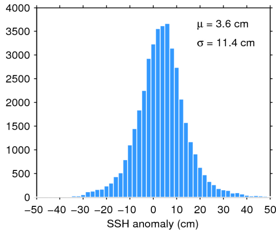
Figure 11. Histogram of science-valid SSH anomaly over oceans and lakes for 21/02/2018. The mean ( \mu ) and standard deviation ( \sigma ) are also shown. Note that values outside [-50 50] cm are excluded from the histogram for the sake of readability but not from the computation of \mu and \sigma .
