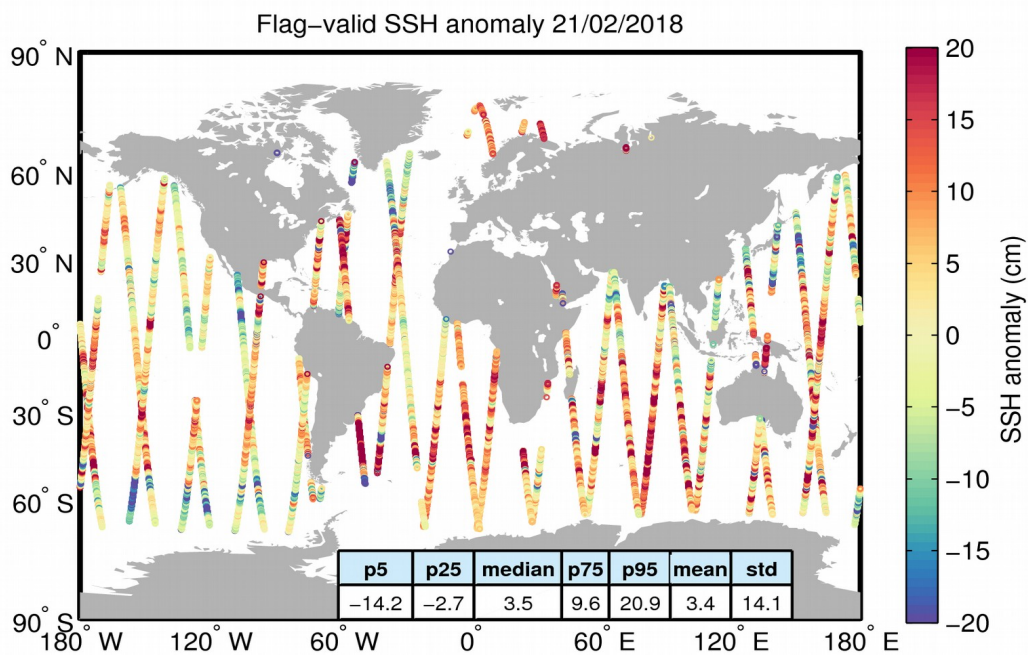
Figure 5. Geographical distribution of flag-valid 1-Hz SSH anomaly data over oceans and lakes for 21/02/2018. The statistical values shown in the table refer to the SSH anomaly in cm and are calculated over all measurements shown in the figure.
