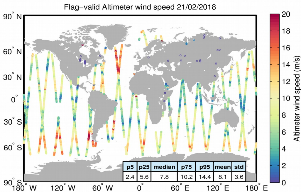
Figure 31. Geographical distribution of flag-valid wind data over oceans and lakes for 21/02/2018. The statistical values shown in the table refer to the wind in m/s and are calculated over all measurements shown in the figure.
