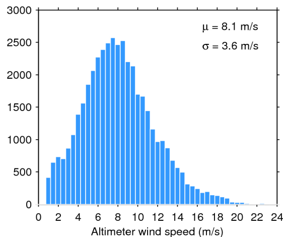
Figure 35. Histogram of science-valid wind over oceans and lakes for 21/02/2018. The mean ( \mu ) and standard deviation ( \sigma ) are also shown. Note that values larger than 24 m/s are excluded from the histogram for the sake of readability but not from the computation of \mu and \sigma .
