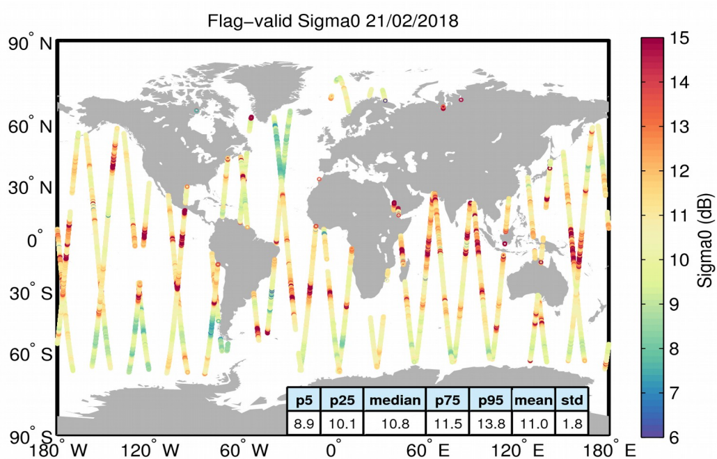
Figure 23. Geographical distribution of flag-valid sigma0 data over oceans and lakes for 21/02/2018. The statistical values shown in the table refer to the sigma0 in dB and are calculated over all measurements shown in the figure.
