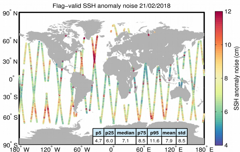
Figure 8. Geographical distribution of flag-valid 20-Hz SSH anomaly measurement noise over oceans and lakes for 21/02/2018. The statistical values shown in the table refer to the SSH anomaly noise and are calculated over all measurements shown in the figure.
