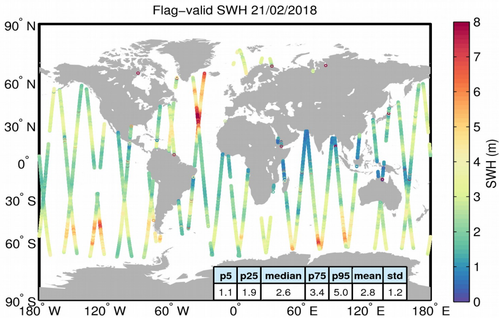
Figure 15. Geographical distribution of flag-valid SWH data over oceans and lakes for 21/02/2018. The statistical values shown in the table refer to the SWH in m and are calculated over all measurements shown in the figure.
