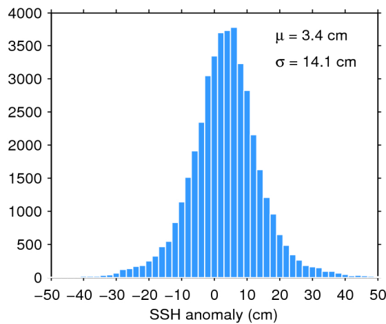
Figure 7. Histogram of flag-valid SSH anomaly over oceans and lakes for 21/02/2018. The mean ( \mu ) and standard deviation ( \sigma ) are also shown. Note that values outside [-50\ 50] cm are excluded from the histogram for the sake of readability but not from the computation of \mu and \sigma .
