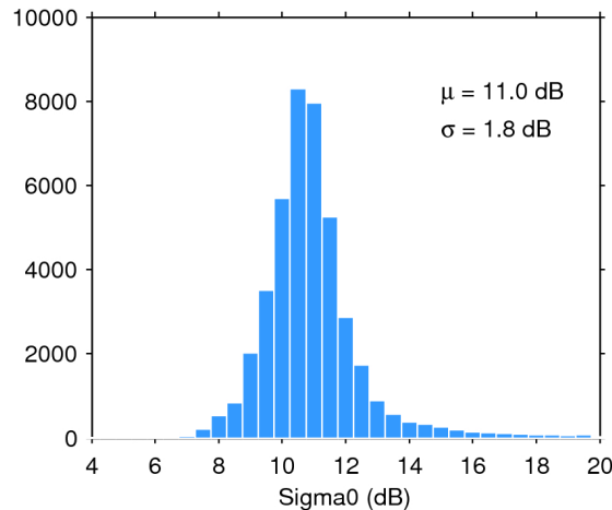
Figure 25. Histogram of flag-valid sigma0 over oceans and lakes for 21/02/2018. The mean ( \mu ) and standard deviation ( \sigma ) are also shown. Note that values outside [4 20] dB are excluded from the histogram for the sake of readability but not from the computation of \mu and \sigma .
