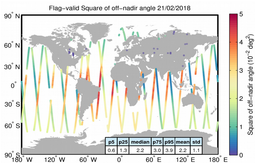
Figure 37. Geographical distribution of flag-valid mispointing data over oceans and lakes for 21/02/2018. The statistical values shown in the table refer to the mispointing in 10^{-2} \text{ deg}^2 and are calculated over all measurements shown in the figure.
