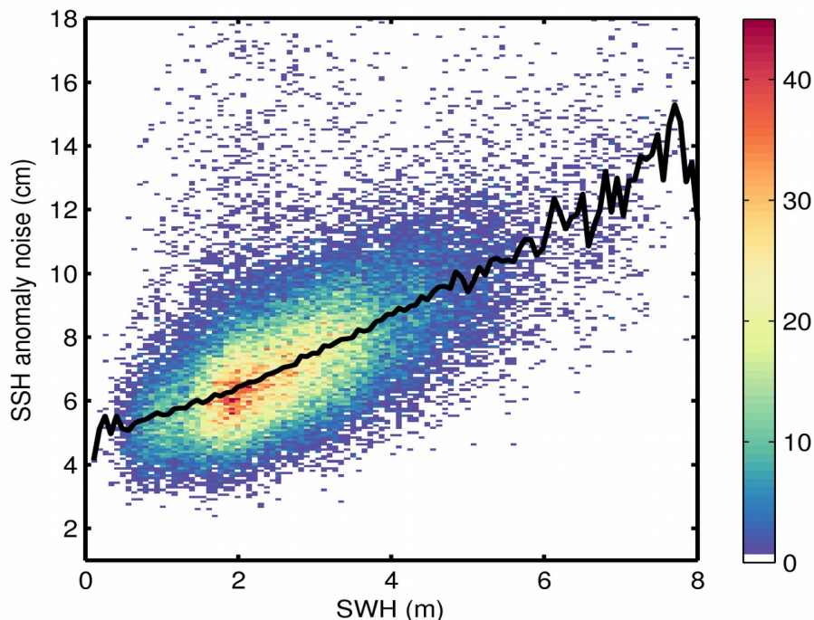
Figure 9. 2D histogram showing flag-valid SSH anomaly noise as a function of SWH for 21/02/2018. The black line denotes the median SSH anomaly noise as a function of SWH.
