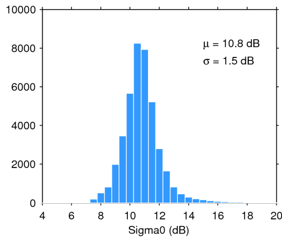
Figure 28. Histogram of science-valid sigma0 over oceans and lakes for 21/02/2018. The mean ( \mu ) and standard deviation ( \sigma ) are also shown. Note that values outside [4 20] dB are excluded from the histogram for the sake of readability but not from the computation of \mu and \sigma .
