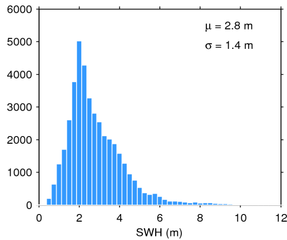
Figure 17. Histogram of flag-valid SWH over oceans and lakes for 20/02/2018. The mean ( \mu ) and standard deviation ( \sigma ) are also shown. Note that values larger than 12 m are excluded from the histogram for the sake of readability but not from the computation of \mu and \sigma .
