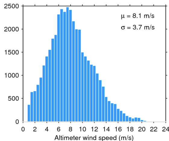
Figure 35. Histogram of science-valid wind over oceans and lakes for 20/02/2018. The mean ( \mu ) and standard deviation ( \sigma ) are also shown. Note that values larger than 24 m/s are excluded from the histogram for the sake of readability but not from the computation of \mu and \sigma .
