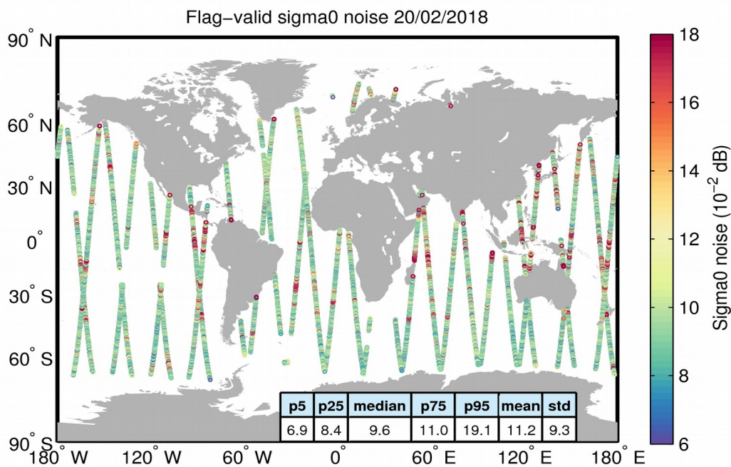
Figure 26. Geographical distribution of flag-valid 20-Hz sigma0 measurement noise over oceans and lakes for 20/02/2018. The statistical values shown in the table refer to the sigma0 noise and are calculated over all measurements shown in the figure.
