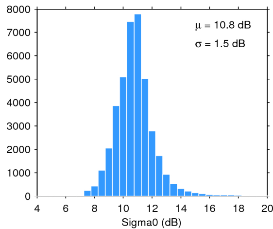
Figure 28. Histogram of science-valid sigma0 over oceans and lakes for 20/02/2018. The mean ( \mu ) and standard deviation ( \sigma ) are also shown. Note that values outside [4 20] dB are excluded from the histogram for the sake of readability but not from the computation of \mu and \sigma .
