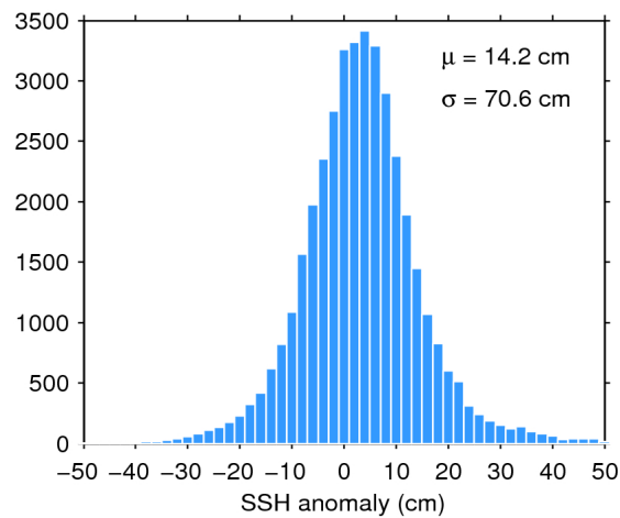
Figure 7. Histogram of flag-valid SSH anomaly over oceans and lakes for 20/02/2018. The mean ( \mu ) and standard deviation ( \sigma ) are also shown. Note that values outside [-50 50] cm are excluded from the histogram for the sake of readability but not from the computation of \mu and \sigma .
