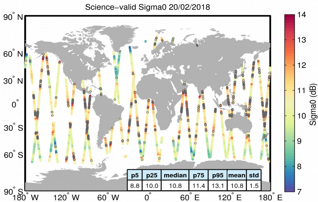
Figure 27. Geographical distribution of science-valid sigma0 data over oceans and lakes for 20/02/2018. The statistical values shown in the table refer to the sigma0 in dB and are calculated over all measurements shown in the figure. Gray circles denote records that have been rejected based on the editing criteria described in Table 4.
