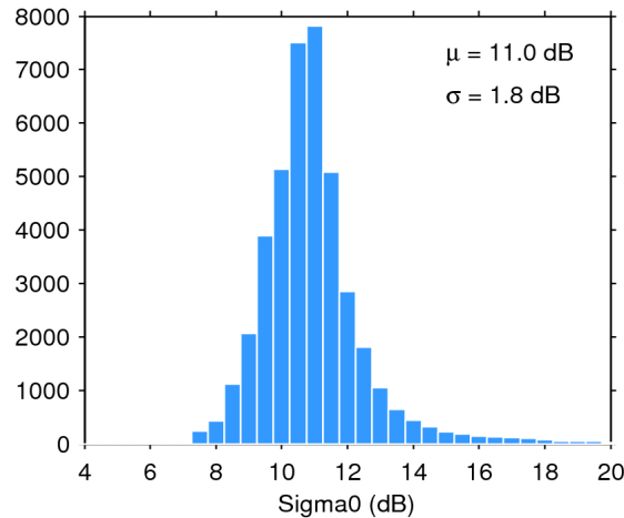
Figure 25. Histogram of flag-valid sigma0 over oceans and lakes for 20/02/2018. The mean ( \mu ) and standard deviation ( \sigma ) are also shown. Note that values outside [4 20] dB are excluded from the histogram for the sake of readability but not from the computation of \mu and \sigma .
