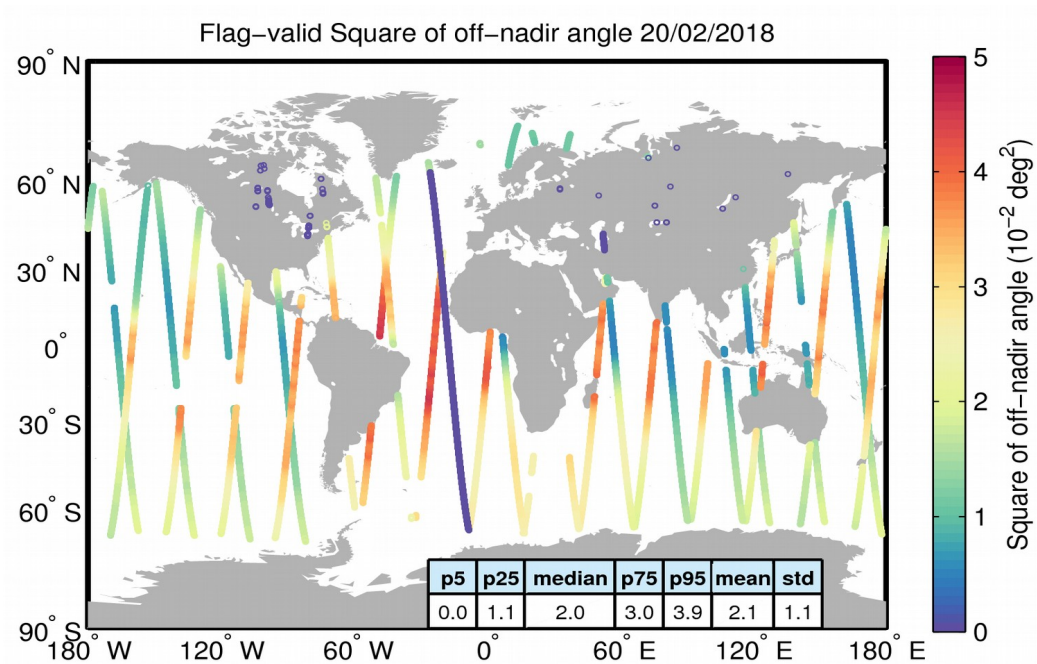
Figure 37. Geographical distribution of flag-valid mispointing data over oceans and lakes for 20/02/2018. The statistical values shown in the table refer to the mispointing in 10^{-2} deg 2 and are calculated over all measurements shown in the figure.
