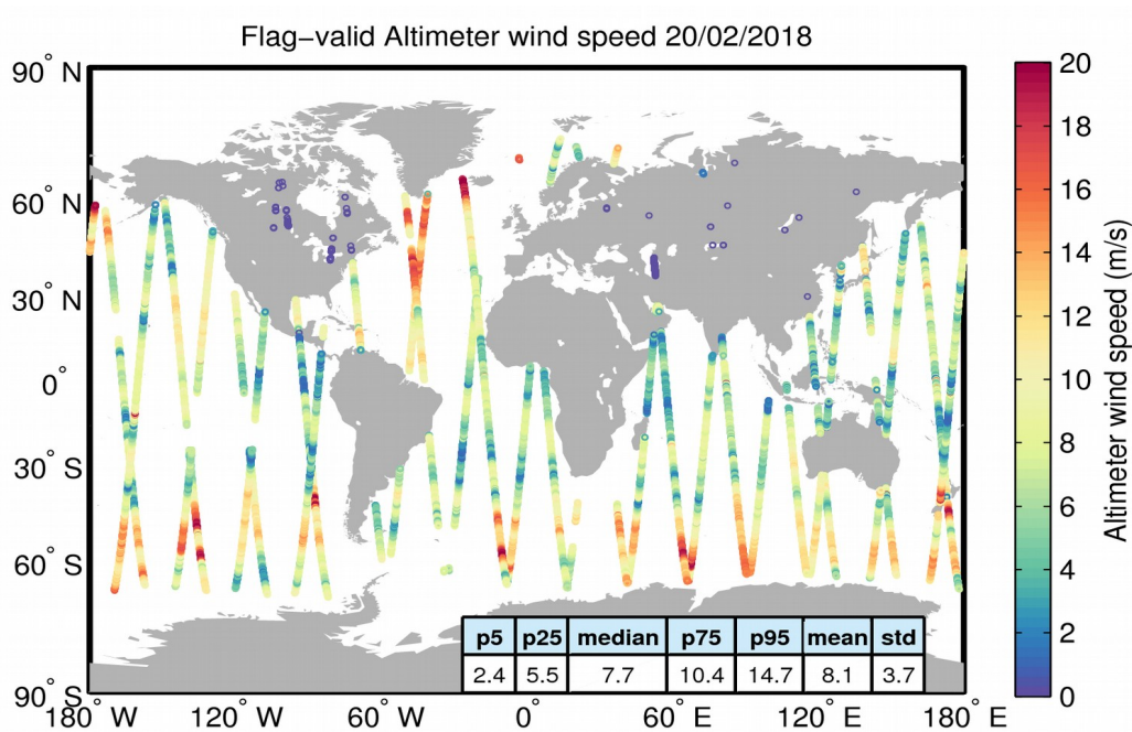
Figure 31. Geographical distribution of flag-valid wind data over oceans and lakes for 20/02/2018. The statistical values shown in the table refer to the wind in m/s and are calculated over all measurements shown in the figure.
