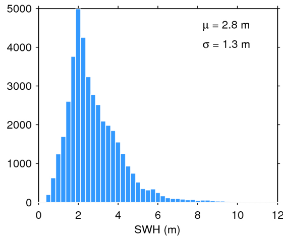
Figure 20. Histogram of science-valid SWH over oceans and lakes for 20/02/2018. The mean ( \mu ) and standard deviation ( \sigma ) are also shown. Note that values larger than 12 m are excluded from the histogram for the sake of readability but not from the computation of \mu and \sigma .
