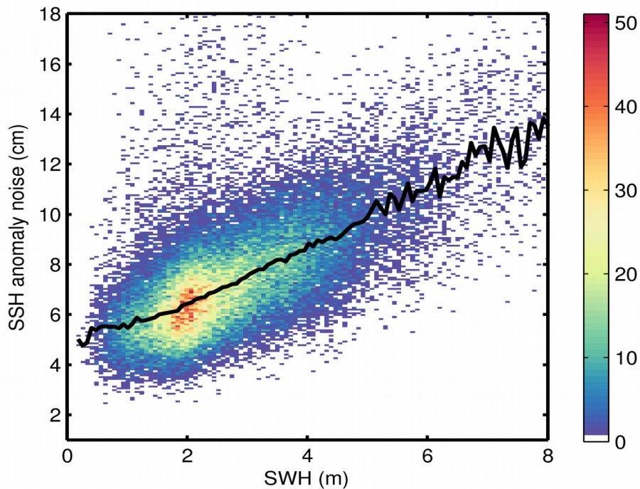
Figure 9. 2D histogram showing flag-valid SSH anomaly noise as a function of SWH for 20/02/2018. The black line denotes the median SSH anomaly noise as a function of SWH.
