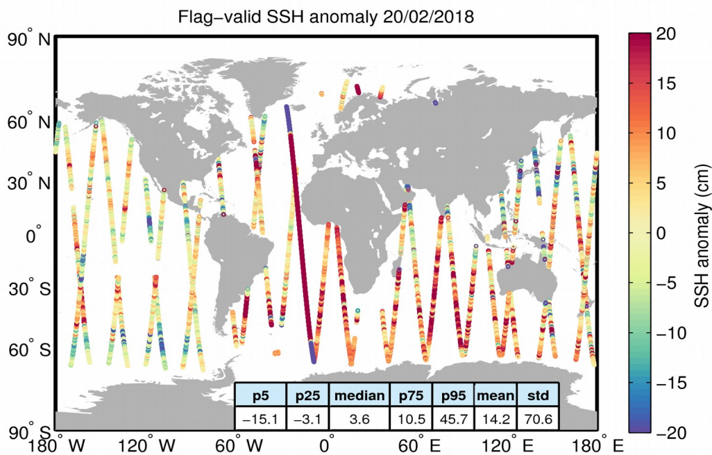
Figure 5. Geographical distribution of flag-valid 1-Hz SSH anomaly data over oceans and lakes for 20/02/2018. The statistical values shown in the table refer to the SSH anomaly in cm and are calculated over all measurements shown in the figure.
