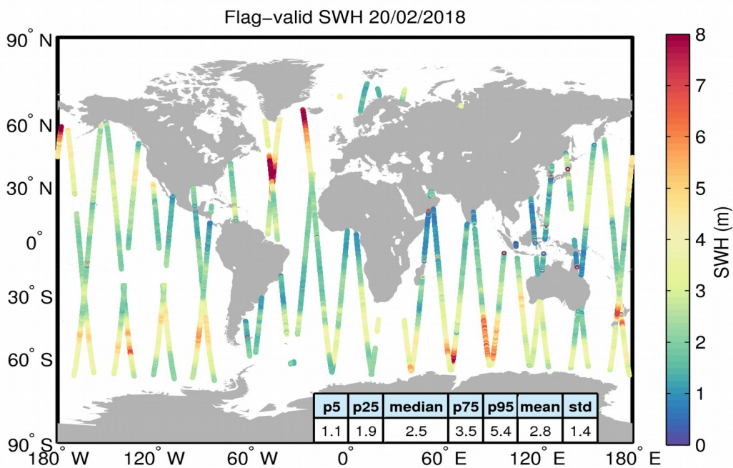
Figure 15. Geographical distribution of flag-valid SWH data over oceans and lakes for 20/02/2018. The statistical values shown in the table refer to the SWH in m and are calculated over all measurements shown in the figure.
