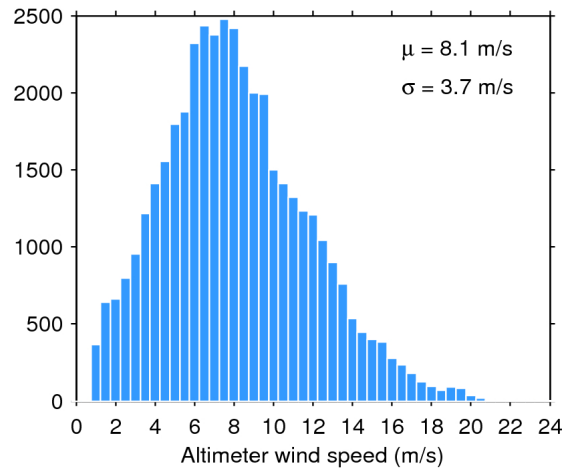
Figure 33. Histogram of flag-valid wind over oceans and lakes for 20/02/2018. The mean ( \mu ) and standard deviation ( \sigma ) are also shown. Note that values larger than 24 m/s are excluded from the histogram for the sake of readability but not from the computation of \mu and \sigma .
