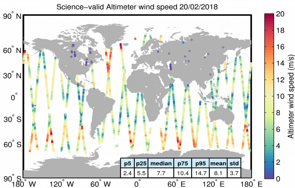
Figure 34. Geographical distribution of science-valid wind data over oceans and lakes for 20/02/2018. The statistical values shown in the table refer to the wind in m/s and are calculated over all measurements shown in the figure. Gray circles denote records that have been rejected based on the editing criteria described in Table 5.
