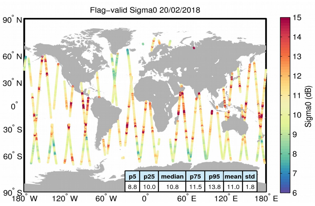
Figure 23. Geographical distribution of flag-valid sigma0 data over oceans and lakes for 20/02/2018. The statistical values shown in the table refer to the sigma0 in dB and are calculated over all measurements shown in the figure.
