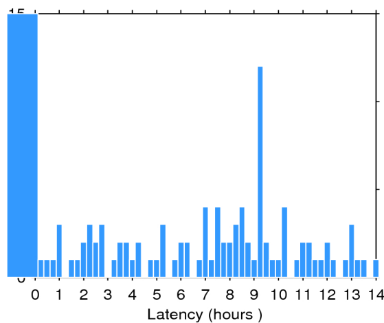
Figure 2. Histogram of the data latency for 20/02/2018. The y-axis denotes the number of files that are made available with a delay of x-hours with respect to the mean time of the records stored in the file.
