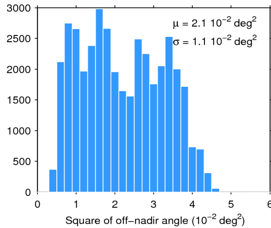
Figure 39. Histogram of flag-valid mispointing over oceans and lakes for 20/02/2018. The mean ( \mu ) and standard deviation ( \sigma ) are also shown. Note that values larger than 6 \cdot 10^{-2} \text{ deg}^2 are excluded from the histogram for the sake of readability but not from the computation of \mu and \sigma .
