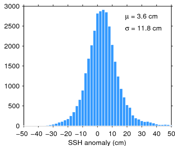
Figure 11. Histogram of science-valid SSH anomaly over oceans and lakes for 20/02/2018. The mean ( \mu ) and standard deviation ( \sigma ) are also shown. Note that values outside [-50 50] cm are excluded from the histogram for the sake of readability but not from the computation of \mu and \sigma .
