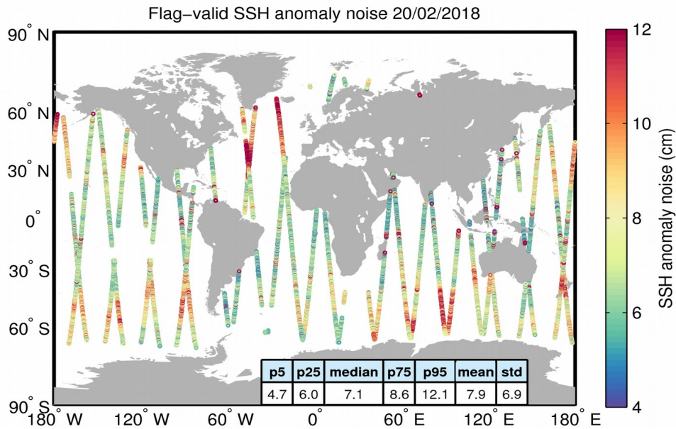
Figure 8. Geographical distribution of flag-valid 20-Hz SSH anomaly measurement noise over oceans and lakes for 20/02/2018. The statistical values shown in the table refer to the SSH anomaly noise and are calculated over all measurements shown in the figure.
