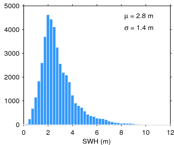
Figure 17. Histogram of flag-valid SWH over oceans and lakes for 19/02/2018. The mean ( \mu ) and standard deviation ( \sigma ) are also shown. Note that values larger than 12 m are excluded from the histogram for the sake of readability but not from the computation of \mu and \sigma .
