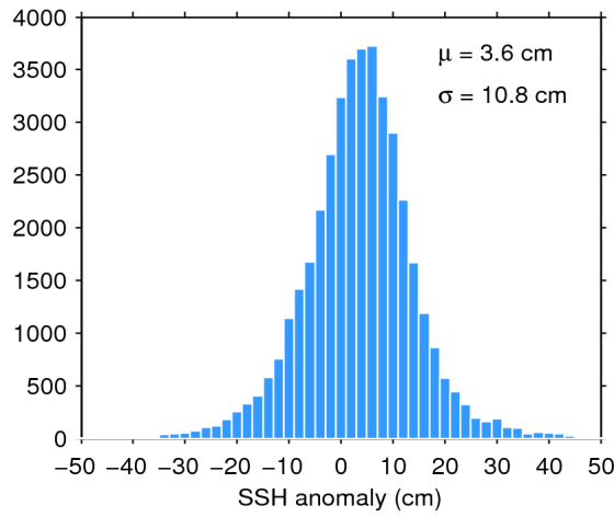
Figure 11. Histogram of science-valid SSH anomaly over oceans and lakes for 19/02/2018. The mean ( \mu ) and standard deviation ( \sigma ) are also shown. Note that values outside [-50 50] cm are excluded from the histogram for the sake of readability but not from the computation of \mu and \sigma .
