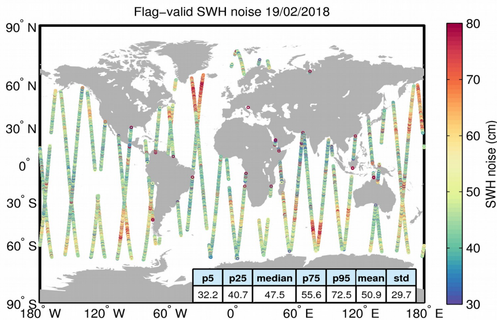
Figure 18. Geographical distribution of flag-valid 20-Hz SWH measurement noise over oceans and lakes for 19/02/2018. The statistical values shown in the table refer to the SWH noise and are calculated over all measurements shown in the figure.
