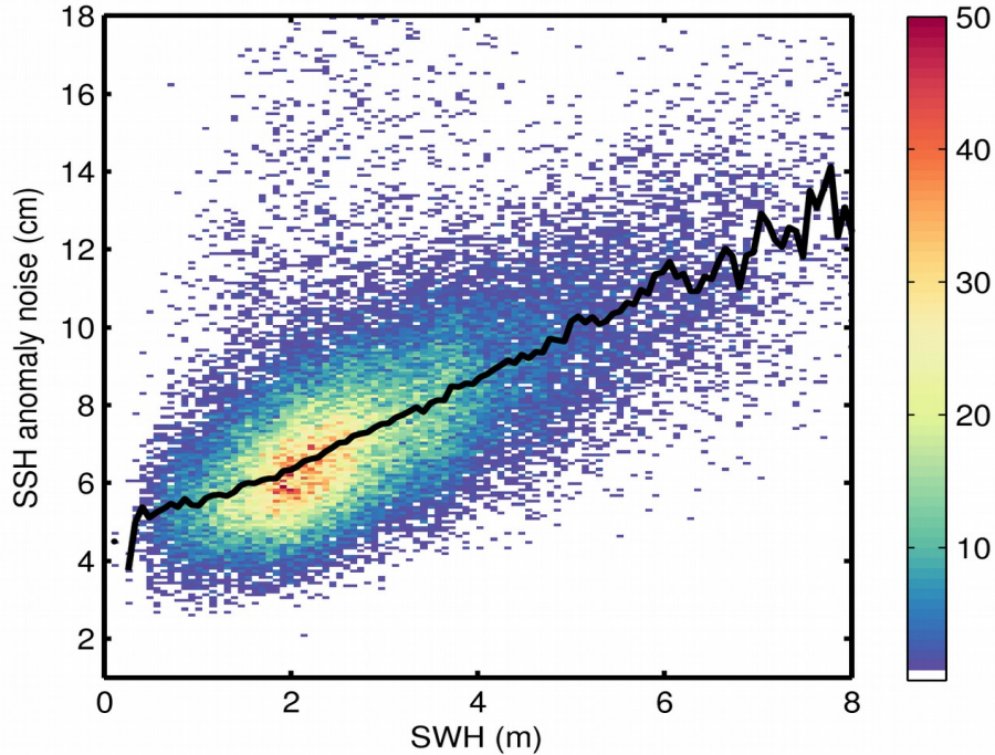
Figure 9. 2D histogram showing flag-valid SSH anomaly noise as a function of SWH for 19/02/2018. The black line denotes the median SSH anomaly noise as a function of SWH.
