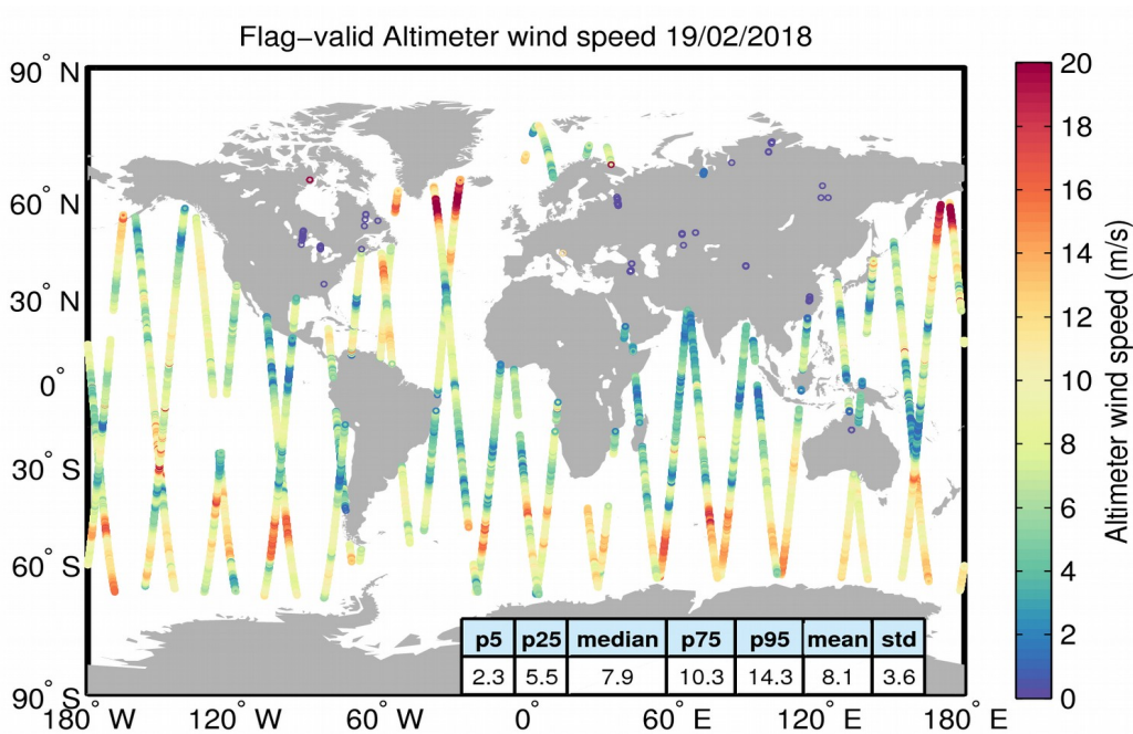
Figure 31. Geographical distribution of flag-valid wind data over oceans and lakes for 19/02/2018. The statistical values shown in the table refer to the wind in m/s and are calculated over all measurements shown in the figure.
