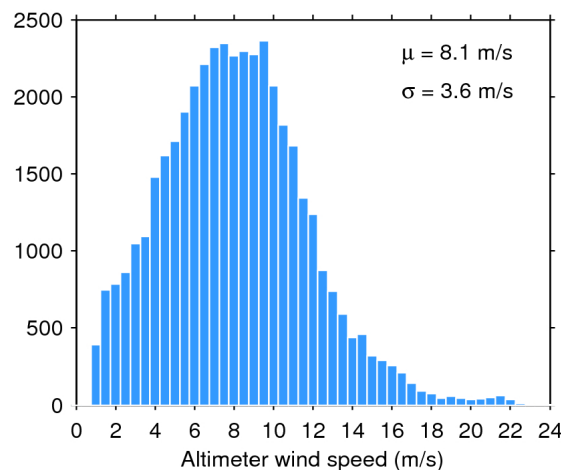
Figure 35. Histogram of science-valid wind over oceans and lakes for 19/02/2018. The mean ( \mu ) and standard deviation ( \sigma ) are also shown. Note that values larger than 24 m/s are excluded from the histogram for the sake of readability but not from the computation of \mu and \sigma .
