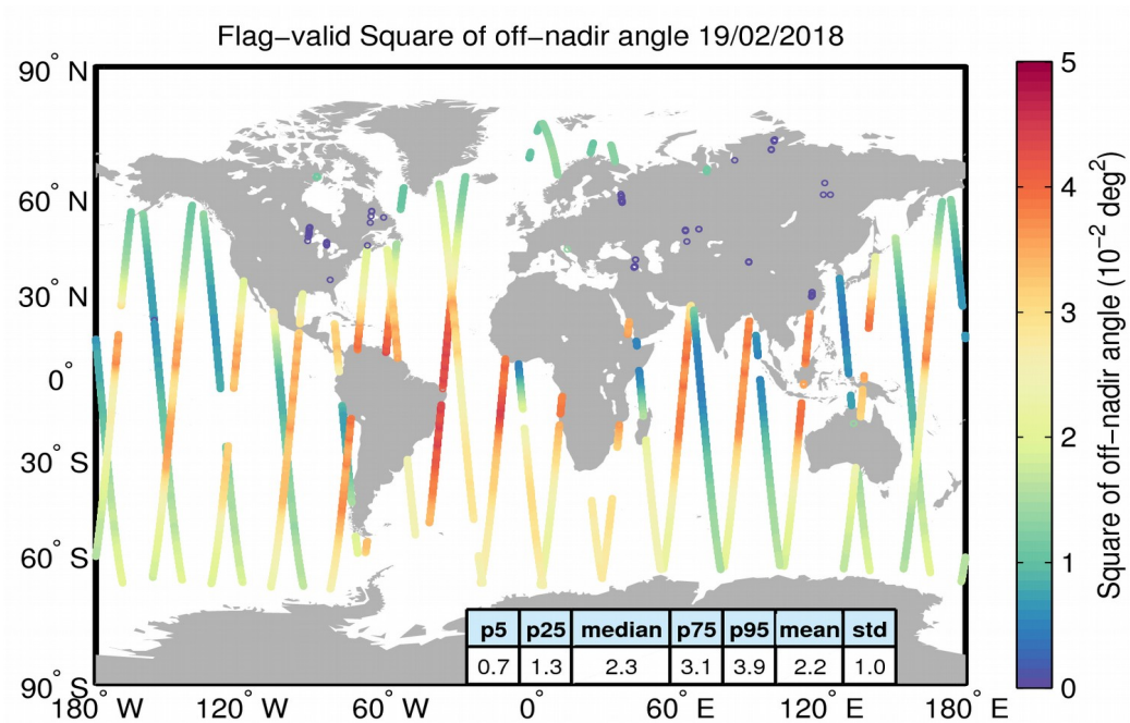
Figure 37. Geographical distribution of flag-valid mispointing data over oceans and lakes for 19/02/2018. The statistical values shown in the table refer to the mispointing in 10^{-2} \text{deg}^2 and are calculated over all measurements shown in the figure.
