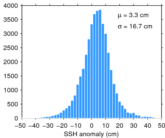
Figure 7. Histogram of flag-valid SSH anomaly over oceans and lakes for 19/02/2018. The mean ( \mu ) and standard deviation ( \sigma ) are also shown. Note that values outside [-50 50] cm are excluded from the histogram for the sake of readability but not from the computation of \mu and \sigma .
