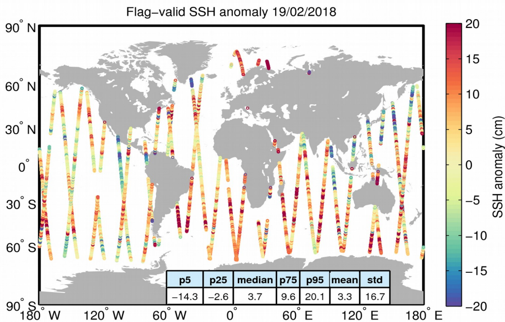
Figure 5. Geographical distribution of flag-valid 1-Hz SSH anomaly data over oceans and lakes for 19/02/2018. The statistical values shown in the table refer to the SSH anomaly in cm and are calculated over all measurements shown in the figure.
