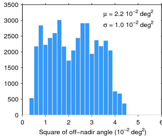
Figure 39. Histogram of flag-valid mispointing over oceans and lakes for 19/02/2018. The mean ( \mu ) and standard deviation ( \sigma ) are also shown. Note that values larger than 6 \cdot 10^{-2} \text{ deg}^2 are excluded from the histogram for the sake of readability but not from the computation of \mu and \sigma .
