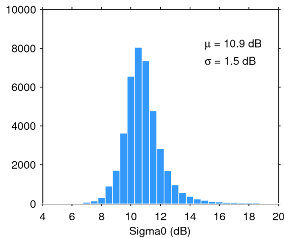
Figure 28. Histogram of science-valid sigma0 over oceans and lakes for 19/02/2018. The mean ( \mu ) and standard deviation ( \sigma ) are also shown. Note that values outside [4 20] dB are excluded from the histogram for the sake of readability but not from the computation of \mu and \sigma .
