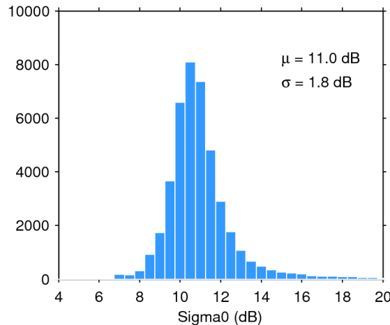
Figure 25. Histogram of flag-valid sigma0 over oceans and lakes for 19/02/2018. The mean ( \mu ) and standard deviation ( \sigma ) are also shown. Note that values outside [4 20] dB are excluded from the histogram for the sake of readability but not from the computation of \mu and \sigma .
