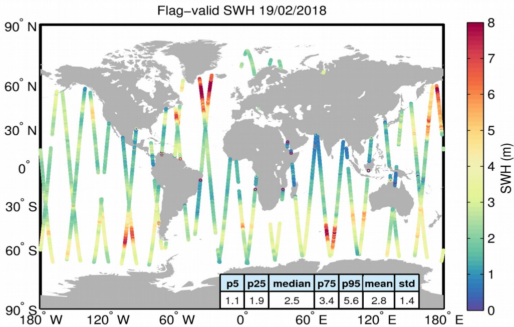
Figure 15. Geographical distribution of flag-valid SWH data over oceans and lakes for 19/02/2018. The statistical values shown in the table refer to the SWH in m and are calculated over all measurements shown in the figure.
