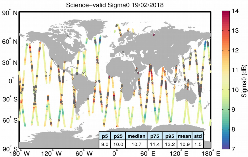
Figure 27. Geographical distribution of science-valid sigma0 data over oceans and lakes for 19/02/2018. The statistical values shown in the table refer to the sigma0 in dB and are calculated over all measurements shown in the figure. Gray circles denote records that have been rejected based on the editing criteria described in Table 4.
