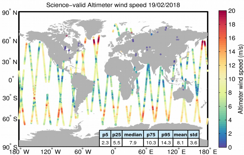
Figure 34. Geographical distribution of science-valid wind data over oceans and lakes for 19/02/2018. The statistical values shown in the table refer to the wind in m/s and are calculated over all measurements shown in the figure. Gray circles denote records that have been rejected based on the editing criteria described in Table 5.
