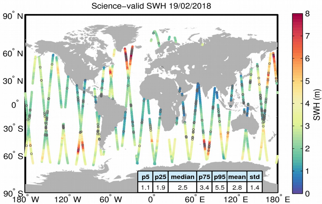
Figure 19. Geographical distribution of science-valid SWH data over oceans and lakes for 19/02/2018. The statistical values shown in the table refer to the SWH in m and are calculated over all measurements shown in the figure. Gray circles denote records that have been rejected based on the editing criteria described in Table 3.
