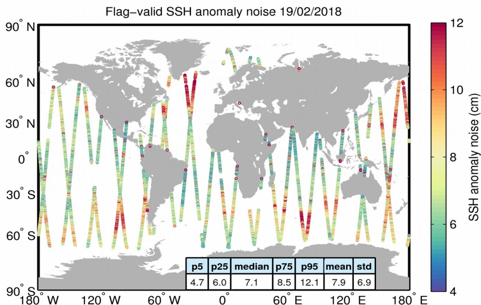
Figure 8. Geographical distribution of flag-valid 20-Hz SSH anomaly measurement noise over oceans and lakes for 19/02/2018. The statistical values shown in the table refer to the SSH anomaly noise and are calculated over all measurements shown in the figure.
