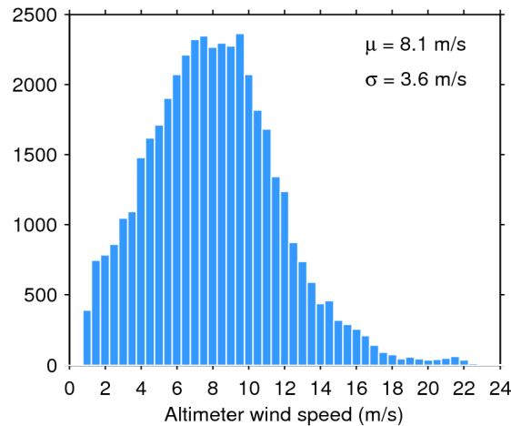
Figure 33. Histogram of flag-valid wind over oceans and lakes for 19/02/2018. The mean ( \mu ) and standard deviation ( \sigma ) are also shown. Note that values larger than 24 m/s are excluded from the histogram for the sake of readability but not from the computation of \mu and \sigma .
