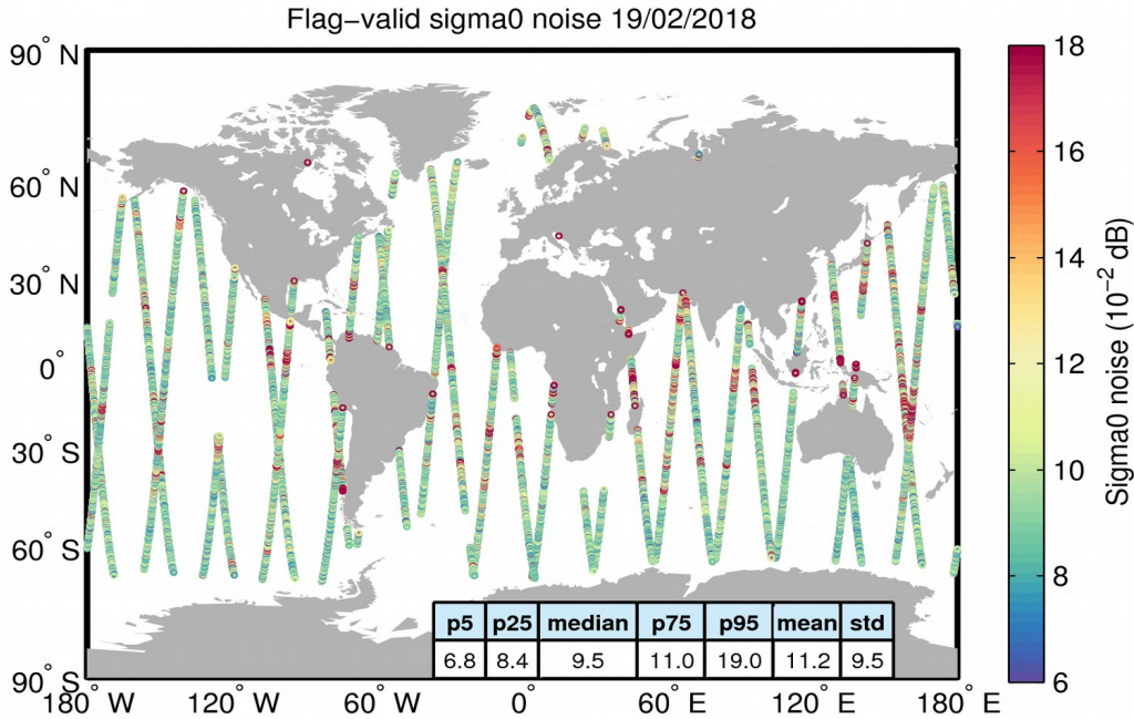
Figure 26. Geographical distribution of flag-valid 20-Hz sigma0 measurement noise over oceans and lakes for 19/02/2018. The statistical values shown in the table refer to the sigma0 noise and are calculated over all measurements shown in the figure.
