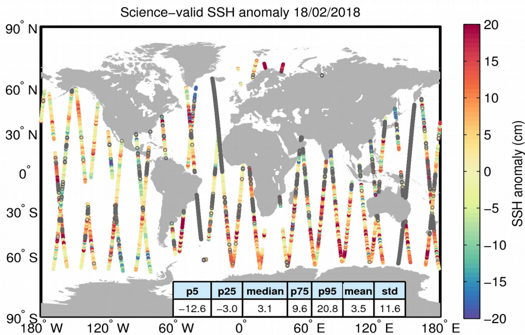
Figure 10. Geographical distribution of science-valid SSH anomaly data over oceans and lakes for 18/02/2018. The statistical values shown in the table refer to the SSH anomaly in cm and are calculated over all measurements shown in the figure. Gray circles denote records that have been rejected based on the editing criteria described in Table 2.
