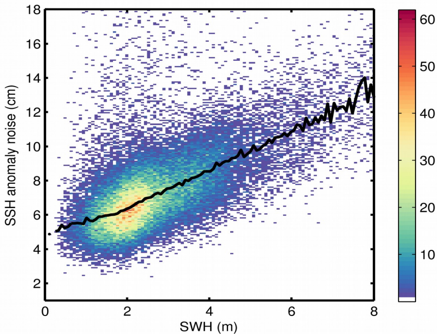
Figure 9. 2D histogram showing flag-valid SSH anomaly noise as a function of SWH for 18/02/2018. The black line denotes the median SSH anomaly noise as a function of SWH.
