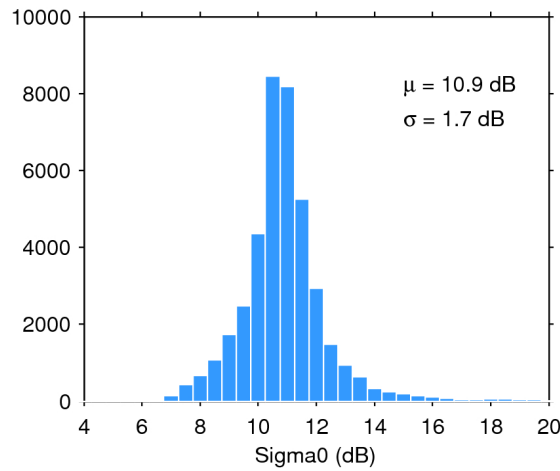
Figure 28. Histogram of science-valid sigma0 over oceans and lakes for 18/02/2018. The mean ( \mu ) and standard deviation ( \sigma ) are also shown. Note that values outside [4 20] dB are excluded from the histogram for the sake of readability but not from the computation of \mu and \sigma .
