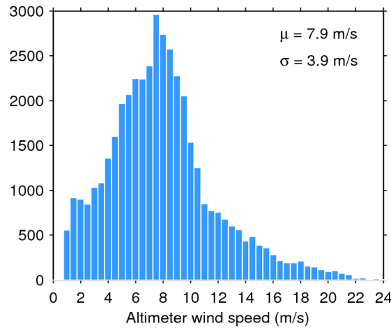
Figure 33. Histogram of flag-valid wind over oceans and lakes for 18/02/2018. The mean ( \mu ) and standard deviation ( \sigma ) are also shown. Note that values larger than 24 m/s are excluded from the histogram for the sake of readability but not from the computation of \mu and \sigma .
