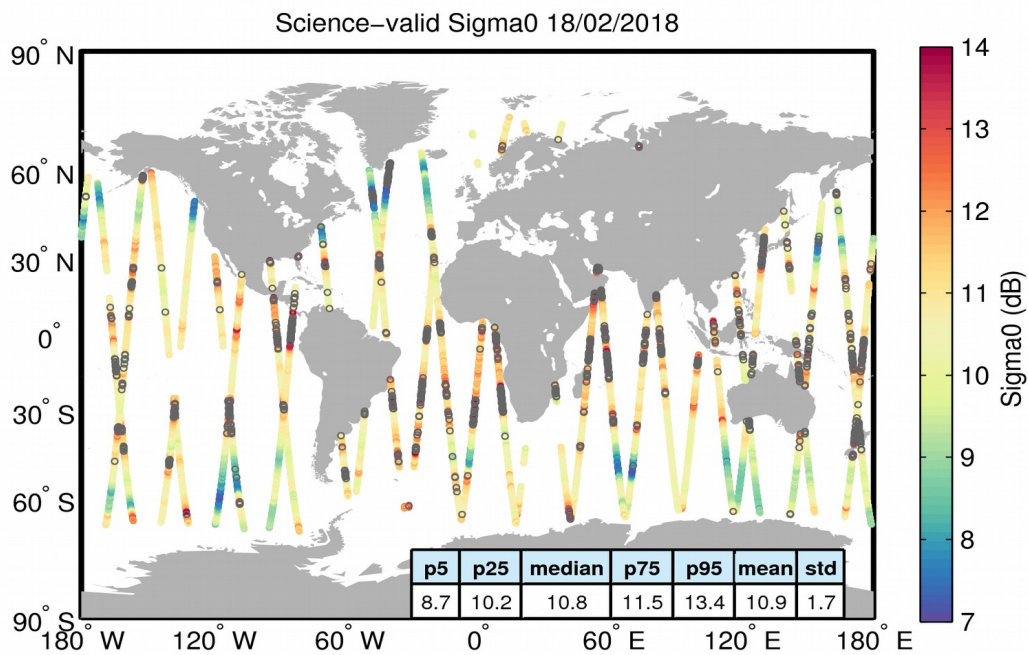
Figure 27. Geographical distribution of science-valid sigma0 data over oceans and lakes for 18/02/2018. The statistical values shown in the table refer to the sigma0 in dB and are calculated over all measurements shown in the figure. Gray circles denote records that have been rejected based on the editing criteria described in Table 4.
