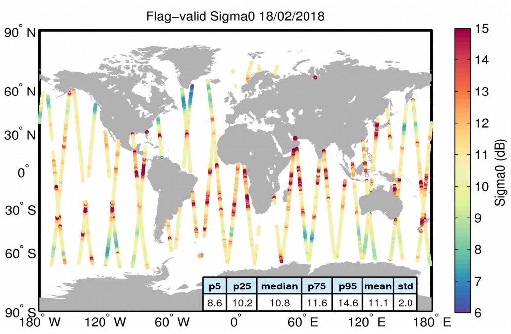
Figure 23. Geographical distribution of flag-valid sigma0 data over oceans and lakes for 18/02/2018. The statistical values shown in the table refer to the sigma0 in dB and are calculated over all measurements shown in the figure.
