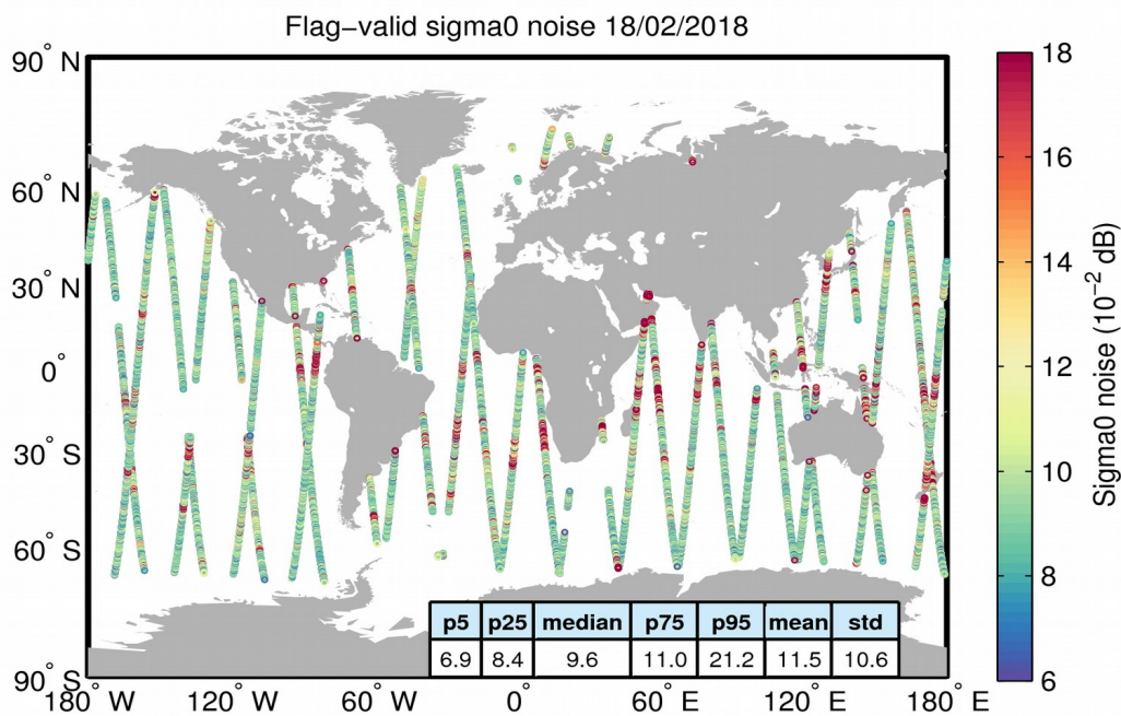
Figure 26. Geographical distribution of flag-valid 20-Hz sigma0 measurement noise over oceans and lakes for 18/02/2018. The statistical values shown in the table refer to the sigma0 noise and are calculated over all measurements shown in the figure.
