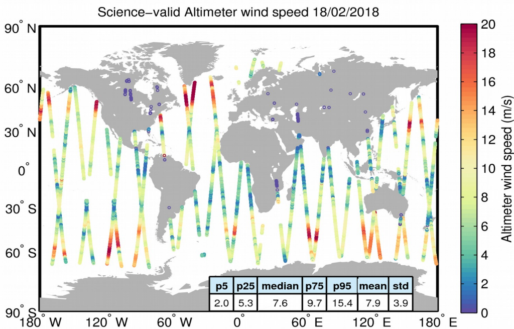
Figure 34. Geographical distribution of science-valid wind data over oceans and lakes for 18/02/2018. The statistical values shown in the table refer to the wind in m/s and are calculated over all measurements shown in the figure. Gray circles denote records that have been rejected based on the editing criteria described in Table 5.
