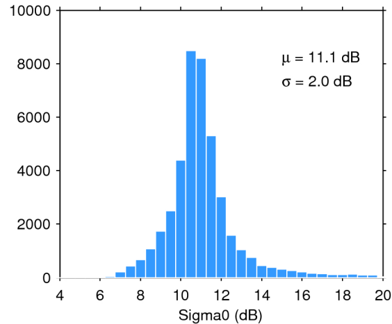
Figure 25. Histogram of flag-valid sigma0 over oceans and lakes for 18/02/2018. The mean ( \mu ) and standard deviation ( \sigma ) are also shown. Note that values outside [4 20] dB are excluded from the histogram for the sake of readability but not from the computation of \mu and \sigma .
