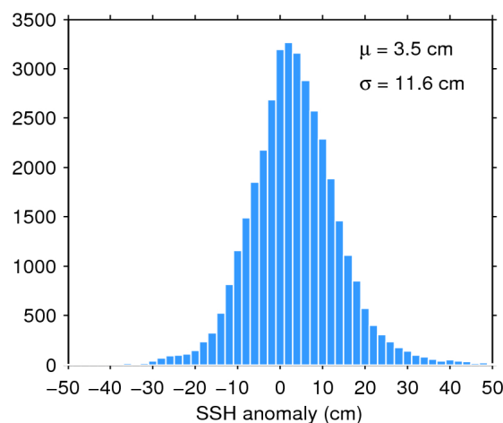
Figure 11. Histogram of science-valid SSH anomaly over oceans and lakes for 18/02/2018. The mean ( \mu ) and standard deviation ( \sigma ) are also shown. Note that values outside [-50 50] cm are excluded from the histogram for the sake of readability but not from the computation of \mu and \sigma .
