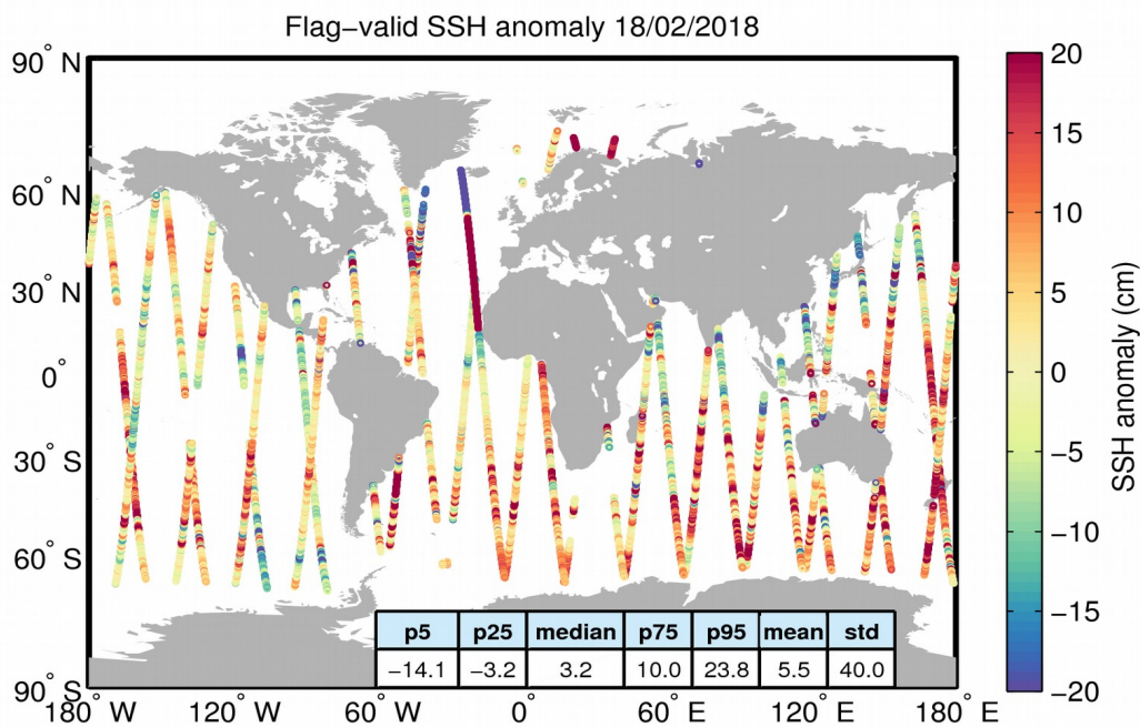
Figure 5. Geographical distribution of flag-valid 1-Hz SSH anomaly data over oceans and lakes for 18/02/2018. The statistical values shown in the table refer to the SSH anomaly in cm and are calculated over all measurements shown in the figure.
