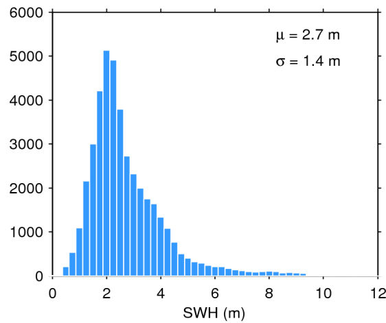
Figure 17. Histogram of flag-valid SWH over oceans and lakes for 18/02/2018. The mean ( \mu ) and standard deviation ( \sigma ) are also shown. Note that values larger than 12 m are excluded from the histogram for the sake of readability but not from the computation of \mu and \sigma .
