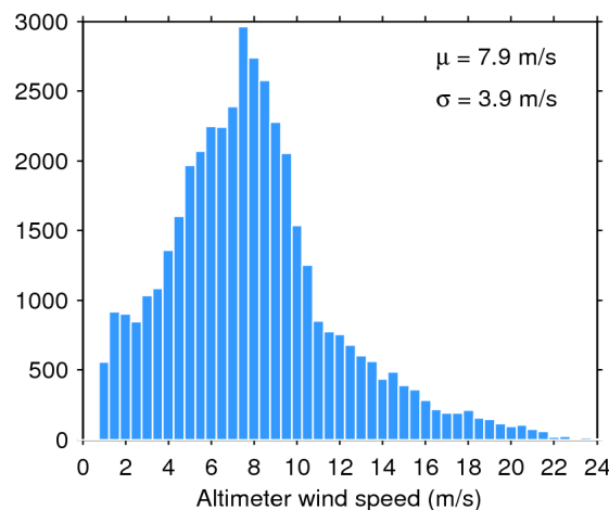
Figure 35. Histogram of science-valid wind over oceans and lakes for 18/02/2018. The mean ( \mu ) and standard deviation ( \sigma ) are also shown. Note that values larger than 24 m/s are excluded from the histogram for the sake of readability but not from the computation of \mu and \sigma .
