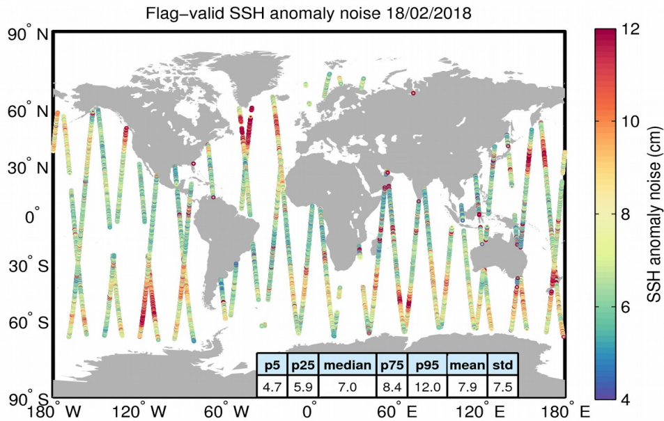
Figure 8. Geographical distribution of flag-valid 20-Hz SSH anomaly measurement noise over oceans and lakes for 18/02/2018. The statistical values shown in the table refer to the SSH anomaly noise and are calculated over all measurements shown in the figure.
