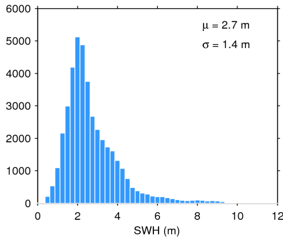
Figure 20. Histogram of science-valid SWH over oceans and lakes for 18/02/2018. The mean ( \mu ) and standard deviation ( \sigma ) are also shown. Note that values larger than 12 m are excluded from the histogram for the sake of readability but not from the computation of \mu and \sigma .
