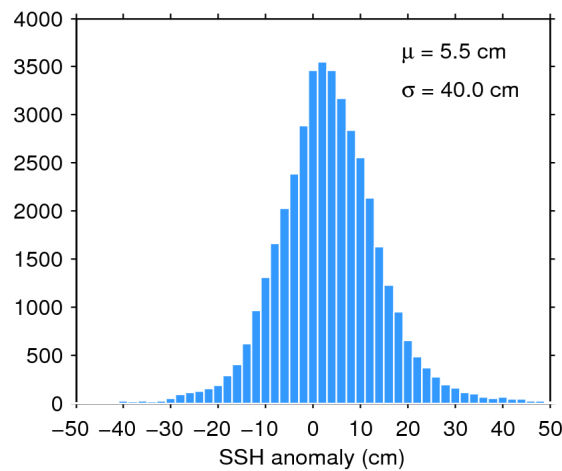
Figure 7. Histogram of flag-valid SSH anomaly over oceans and lakes for 18/02/2018. The mean ( \mu ) and standard deviation ( \sigma ) are also shown. Note that values outside [-50 50] cm are excluded from the histogram for the sake of readability but not from the computation of \mu and \sigma .
