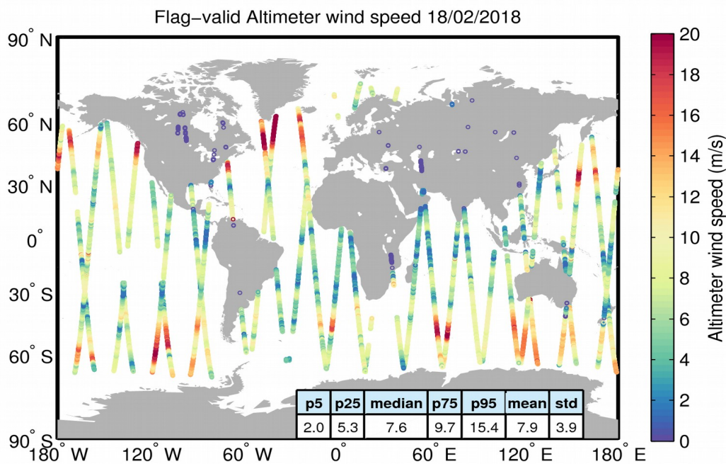
Figure 31. Geographical distribution of flag-valid wind data over oceans and lakes for 18/02/2018. The statistical values shown in the table refer to the wind in m/s and are calculated over all measurements shown in the figure.
