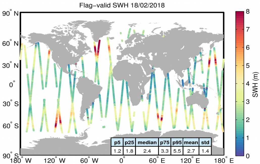
Figure 15. Geographical distribution of flag-valid SWH data over oceans and lakes for 18/02/2018. The statistical values shown in the table refer to the SWH in m and are calculated over all measurements shown in the figure.
