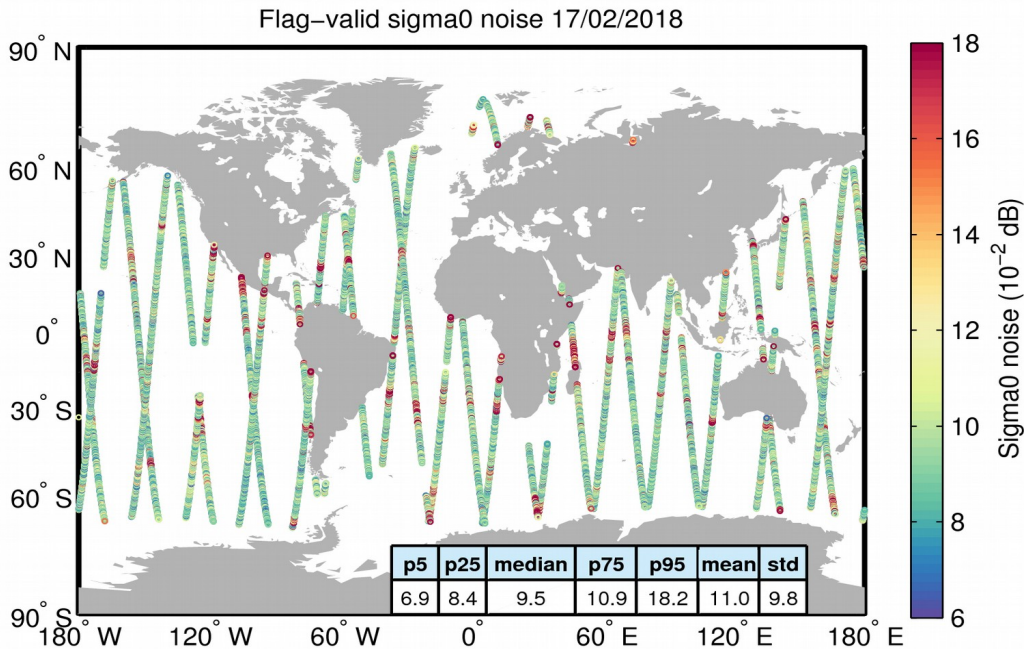
Figure 26. Geographical distribution of flag-valid 20-Hz sigma0 measurement noise over oceans and lakes for 17/02/2018. The statistical values shown in the table refer to the sigma0 noise and are calculated over all measurements shown in the figure.
