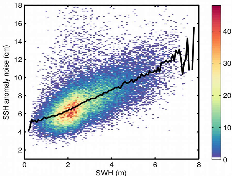
Figure 9. 2D histogram showing flag-valid SSH anomaly noise as a function of SWH for 17/02/2018. The black line denotes the median SSH anomaly noise as a function of SWH.
