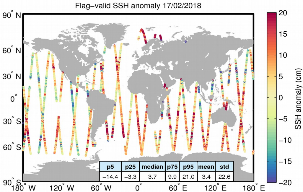
Figure 5. Geographical distribution of flag-valid 1-Hz SSH anomaly data over oceans and lakes for 17/02/2018. The statistical values shown in the table refer to the SSH anomaly in cm and are calculated over all measurements shown in the figure.
