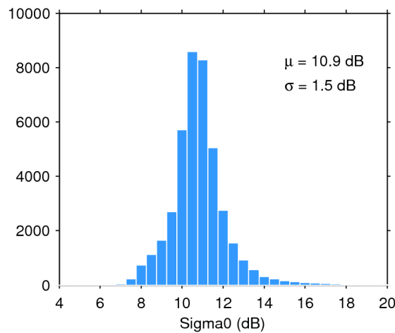
Figure 28. Histogram of science-valid sigma0 over oceans and lakes for 17/02/2018. The mean ( \mu ) and standard deviation ( \sigma ) are also shown. Note that values outside [4 20] dB are excluded from the histogram for the sake of readability but not from the computation of \mu and \sigma .
