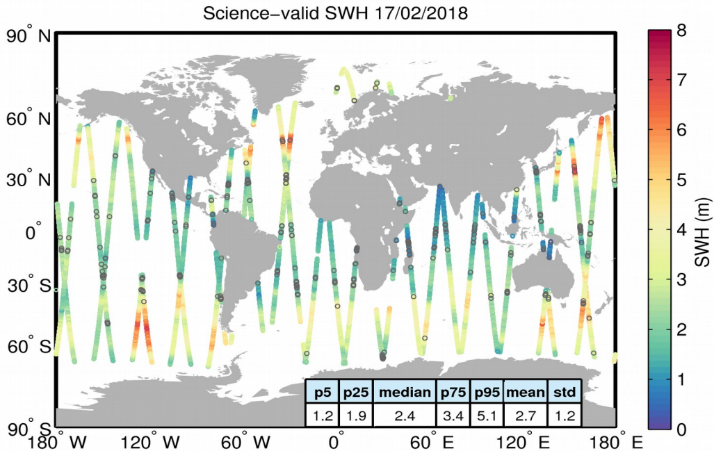
Figure 19. Geographical distribution of science-valid SWH data over oceans and lakes for 17/02/2018. The statistical values shown in the table refer to the SWH in m and are calculated over all measurements shown in the figure. Gray circles denote records that have been rejected based on the editing criteria described in Table 3.
