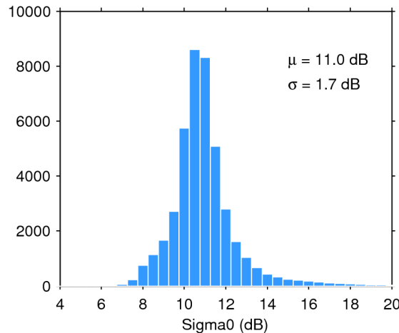
Figure 25. Histogram of flag-valid sigma0 over oceans and lakes for 17/02/2018. The mean ( \mu ) and standard deviation ( \sigma ) are also shown. Note that values outside [4 20] dB are excluded from the histogram for the sake of readability but not from the computation of \mu and \sigma .
