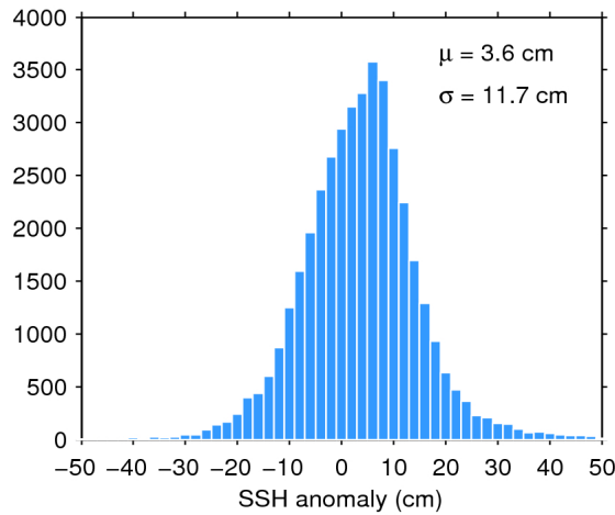
Figure 11. Histogram of science-valid SSH anomaly over oceans and lakes for 17/02/2018. The mean ( \mu ) and standard deviation ( \sigma ) are also shown. Note that values outside [-50 50] cm are excluded from the histogram for the sake of readability but not from the computation of \mu and \sigma .
