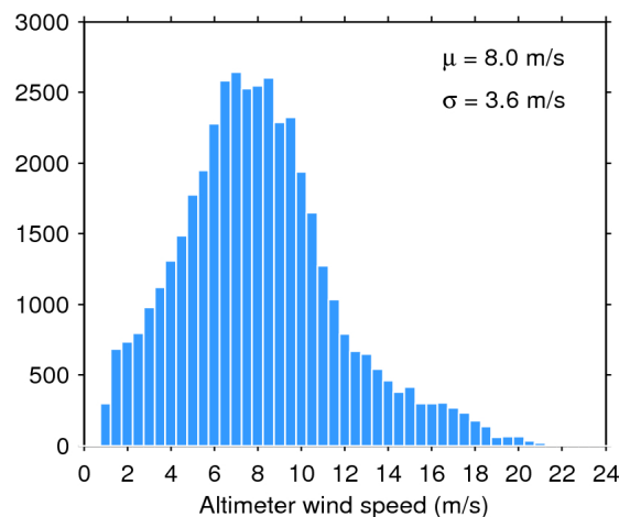
Figure 35. Histogram of science-valid wind over oceans and lakes for 17/02/2018. The mean ( \mu ) and standard deviation ( \sigma ) are also shown. Note that values larger than 24 m/s are excluded from the histogram for the sake of readability but not from the computation of \mu and \sigma .
