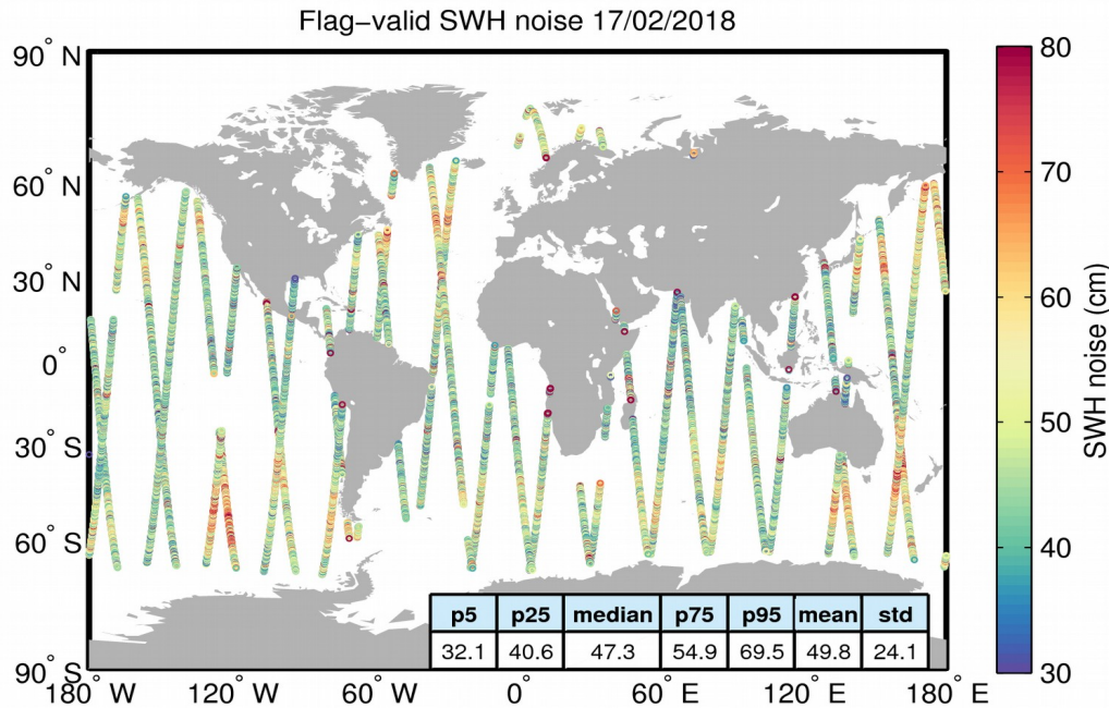
Figure 18. Geographical distribution of flag-valid 20-Hz SWH measurement noise over oceans and lakes for 17/02/2018. The statistical values shown in the figure refer to the SWH noise and are calculated over all measurements shown in the figure.
