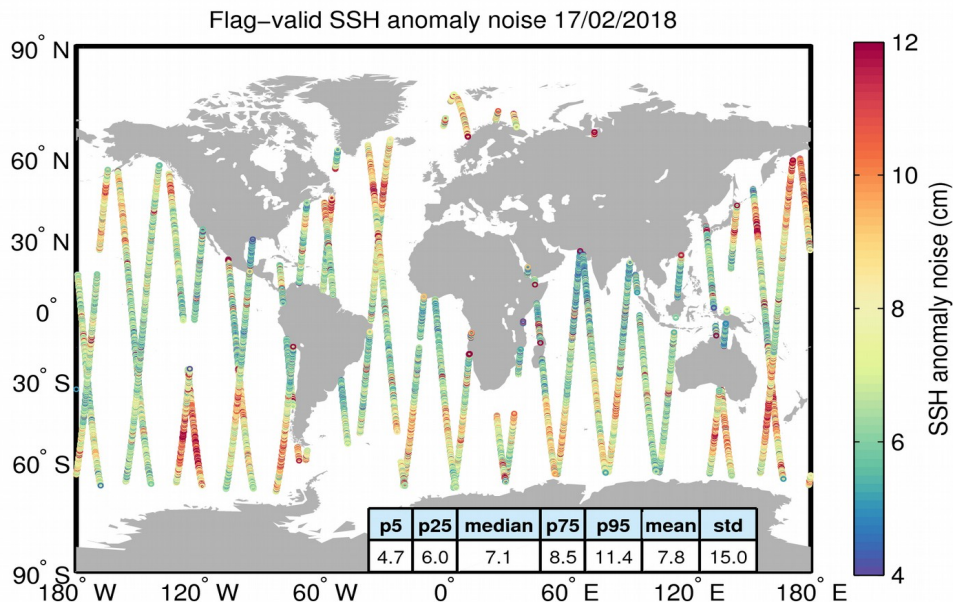
Figure 8. Geographical distribution of flag-valid 20-Hz SSH anomaly measurement noise over oceans and lakes for 17/02/2018. The statistical values shown in the table refer to the SSH anomaly noise and are calculated over all measurements shown in the figure.
