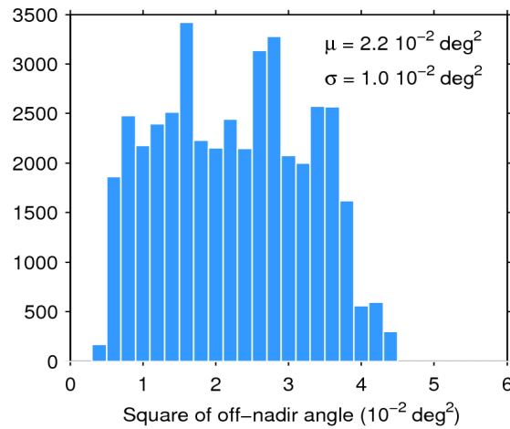
Figure 39. Histogram of flag-valid mispointing over oceans and lakes for 17/02/2018. The mean ( \mu ) and standard deviation ( \sigma ) are also shown. Note that values larger than 6 \cdot 10^{-2} \text{ deg}^2 are excluded from the histogram for the sake of readability but not from the computation of \mu and \sigma .
