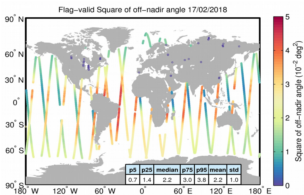
Figure 37. Geographical distribution of flag-valid mispointing data over oceans and lakes for 17/02/2018. The statistical values shown in the table refer to the mispointing in 10^{-2} \text{ deg}^2 and are calculated over all measurements shown in the figure.
