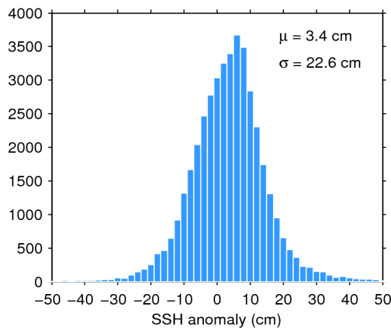
Figure 7. Histogram of flag-valid SSH anomaly over oceans and lakes for 17/02/2018. The mean ( \mu ) and standard deviation ( \sigma ) are also shown. Note that values outside [-50 50] cm are excluded from the histogram for the sake of readability but not from the computation of \mu and \sigma .
