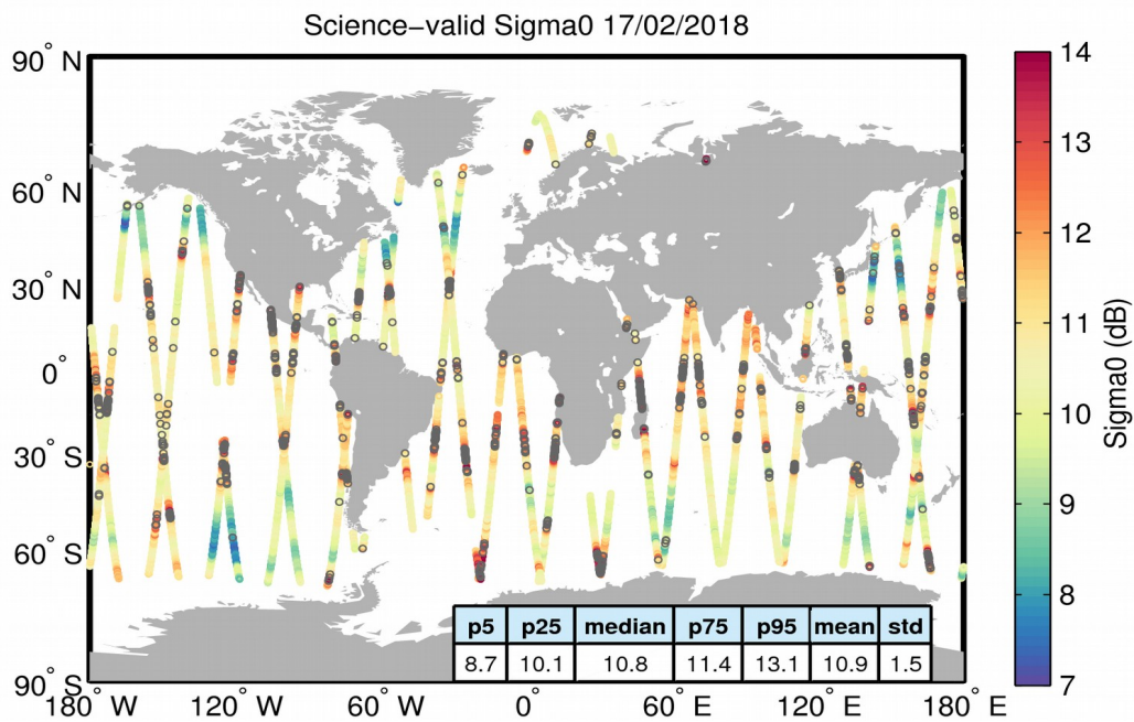
Figure 27. Geographical distribution of science-valid sigma0 data over oceans and lakes for 17/02/2018. The statistical values shown in the table refer to the sigma0 in dB and are calculated over all measurements shown in the figure. Gray circles denote records that have been rejected based on the editing criteria described in Table 4.
