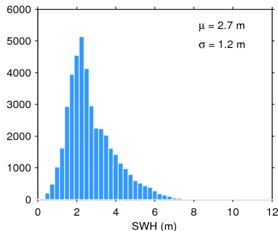
Figure 20. Histogram of science-valid SWH over oceans and lakes for 17/02/2018. The mean ( \mu ) and standard deviation ( \sigma ) are also shown. Note that values larger than 12 m are excluded from the histogram for the sake of readability but not from the computation of \mu and \sigma .
