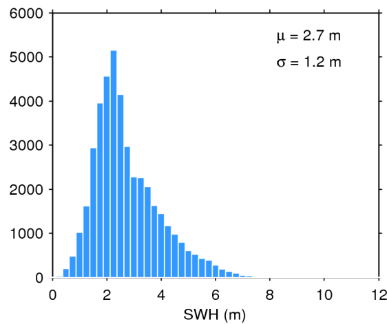
Figure 17. Histogram of flag-valid SWH over oceans and lakes for 17/02/2018. The mean ( \mu ) and standard deviation ( \sigma ) are also shown. Note that values larger than 12 m are excluded from the histogram for the sake of readability but not from the computation of \mu and \sigma .
