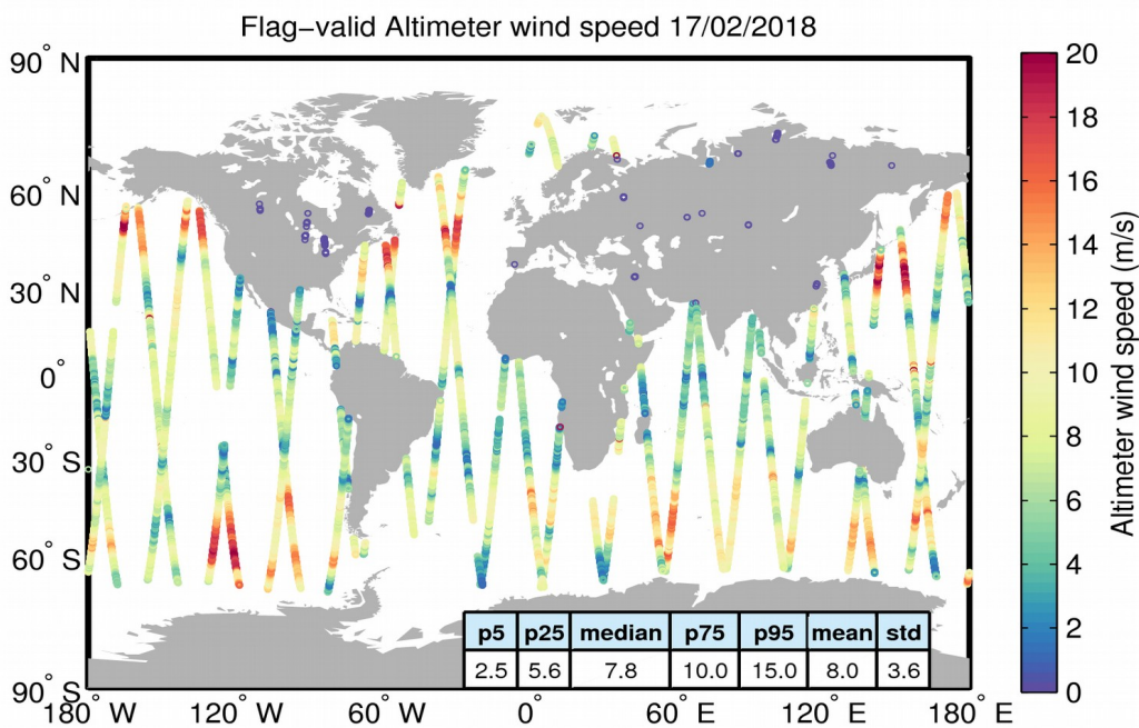
Figure 31. Geographical distribution of flag-valid wind data over oceans and lakes for 17/02/2018. The statistical values shown in the table refer to the wind in m/s and are calculated over all measurements shown in the figure.
