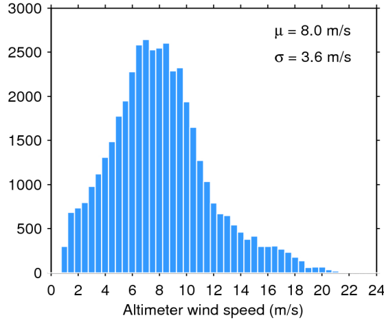
Figure 33. Histogram of flag-valid wind over oceans and lakes for 17/02/2018. The mean ( \mu ) and standard deviation ( \sigma ) are also shown. Note that values larger than 24 m/s are excluded from the histogram for the sake of readability but not from the computation of \mu and \sigma .
