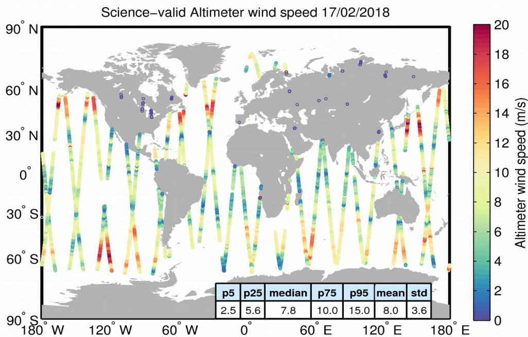
Figure 34. Geographical distribution of science-valid wind data over oceans and lakes for 17/02/2018. The statistical values shown in the table refer to the wind in m/s and are calculated over all measurements shown in the figure. Gray circles denote records that have been rejected based on the editing criteria described in Table 5.
