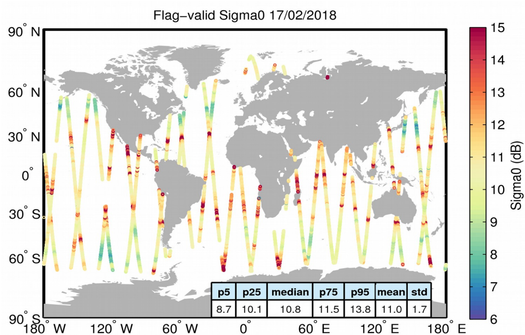
Figure 23. Geographical distribution of flag-valid sigma0 data over oceans and lakes for 17/02/2018. The statistical values shown in the table refer to the sigma0 in dB and are calculated over all measurements shown in the figure.
