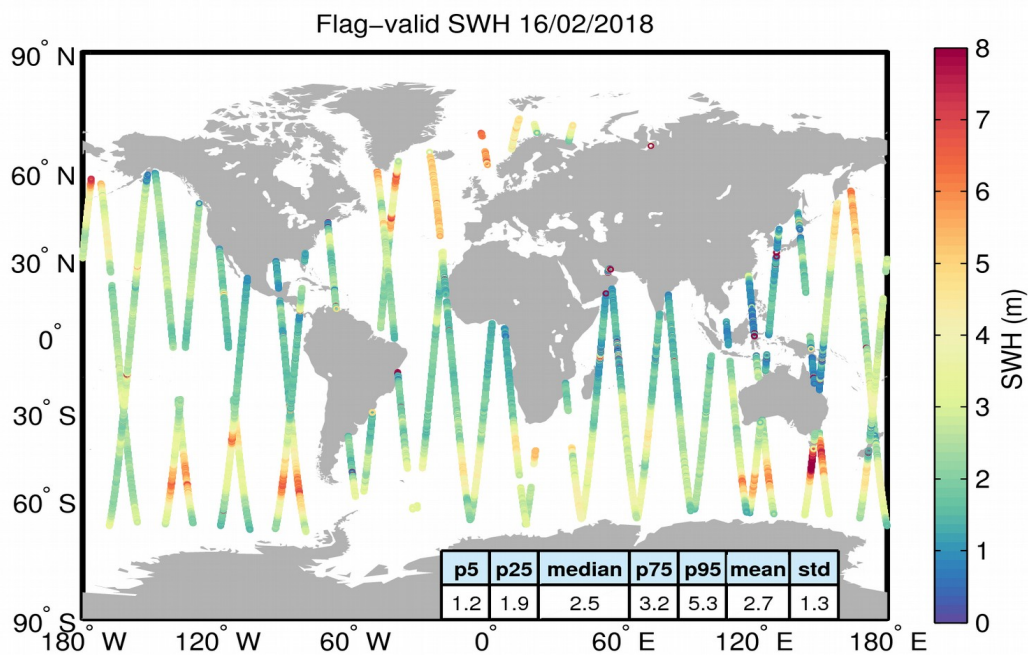
Figure 15. Geographical distribution of flag-valid SWH data over oceans and lakes for 16/02/2018. The statistical values shown in the table refer to the SWH in m and are calculated over all measurements shown in the figure.
