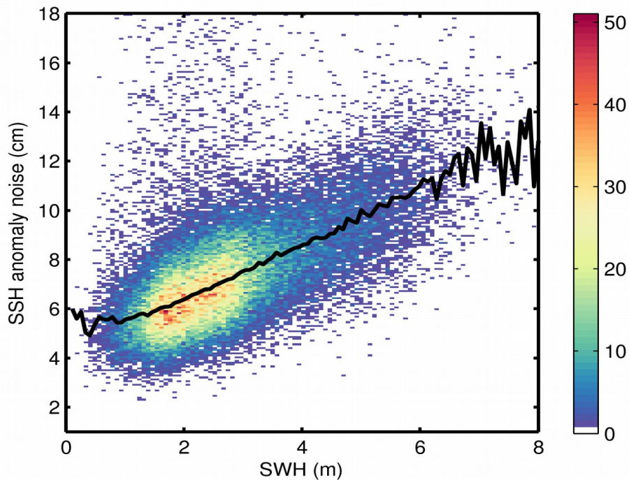
Figure 9. 2D histogram showing flag-valid SSH anomaly noise as a function of SWH for 16/02/2018. The black line denotes the median SSH anomaly noise as a function of SWH.
