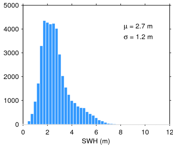
Figure 20. Histogram of science-valid SWH over oceans and lakes for 16/02/2018. The mean ( \mu ) and standard deviation ( \sigma ) are also shown. Note that values larger than 12 m are excluded from the histogram for the sake of readability but not from the computation of \mu and \sigma .
