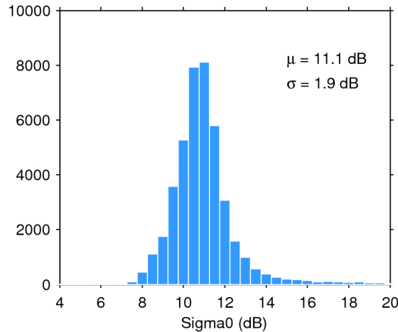
Figure 25. Histogram of flag-valid sigma0 over oceans and lakes for 16/02/2018. The mean ( \mu ) and standard deviation ( \sigma ) are also shown. Note that values outside [4 20] dB are excluded from the histogram for the sake of readability but not from the computation of \mu and \sigma .
