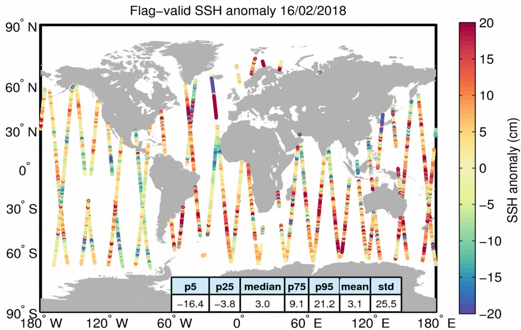
Figure 5. Geographical distribution of flag-valid 1-Hz SSH anomaly data over oceans and lakes for 16/02/2018. The statistical values shown in the table refer to the SSH anomaly in cm and are calculated over all measurements shown in the figure.
