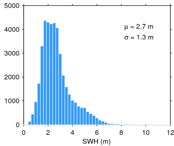
Figure 17. Histogram of flag-valid SWH over oceans and lakes for 16/02/2018. The mean ( \mu ) and standard deviation ( \sigma ) are also shown. Note that values larger than 12 m are excluded from the histogram for the sake of readability but not from the computation of \mu and \sigma .
