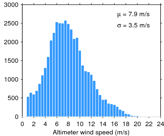
Figure 33. Histogram of flag-valid wind over oceans and lakes for 16/02/2018. The mean ( \mu ) and standard deviation ( \sigma ) are also shown. Note that values larger than 24 m/s are excluded from the histogram for the sake of readability but not from the computation of \mu and \sigma .
