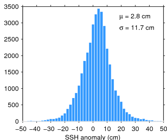
Figure 11. Histogram of science-valid SSH anomaly over oceans and lakes for 16/02/2018. The mean ( \mu ) and standard deviation ( \sigma ) are also shown. Note that values outside [-50 50] cm are excluded from the histogram for the sake of readability but not from the computation of \mu and \sigma .
