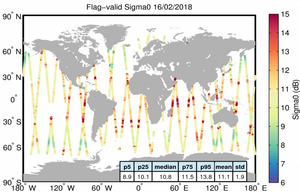
Figure 23. Geographical distribution of flag-valid sigma0 data over oceans and lakes for 16/02/2018. The statistical values shown in the table refer to the sigma0 in dB and are calculated over all measurements shown in the figure.
