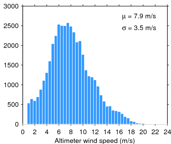
Figure 35. Histogram of science-valid wind over oceans and lakes for 16/02/2018. The mean ( \mu ) and standard deviation ( \sigma ) are also shown. Note that values larger than 24 m/s are excluded from the histogram for the sake of readability but not from the computation of \mu and \sigma .
