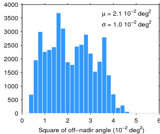
Figure 39. Histogram of flag-valid mispointing over oceans and lakes for 16/02/2018. The mean ( \mu ) and standard deviation ( \sigma ) are also shown. Note that values larger than 6 \cdot 10^{-2} \text{ deg}^2 are excluded from the histogram for the sake of readability but not from the computation of \mu and \sigma .
