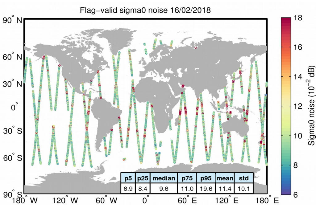
Figure 26. Geographical distribution of flag-valid 20-Hz sigma0 measurement noise over oceans and lakes for 16/02/2018. The statistical values shown in the table refer to the sigma0 noise and are calculated over all measurements shown in the figure.
