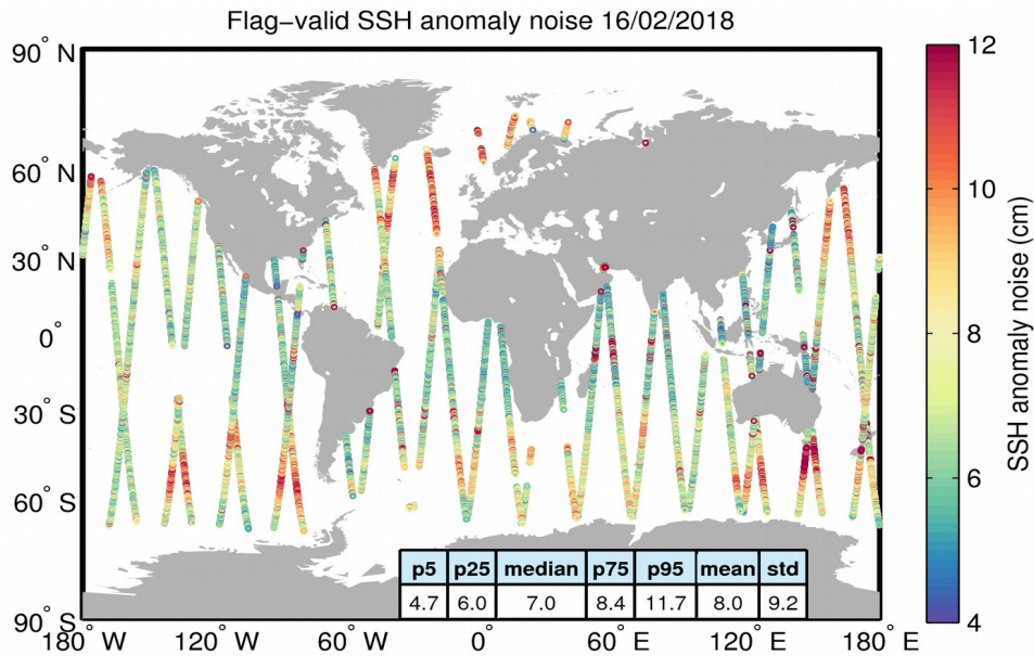
Figure 8. Geographical distribution of flag-valid 20-Hz SSH anomaly measurement noise over oceans and lakes for 16/02/2018. The statistical values shown in the table refer to the SSH anomaly noise and are calculated over all measurements shown in the figure.
