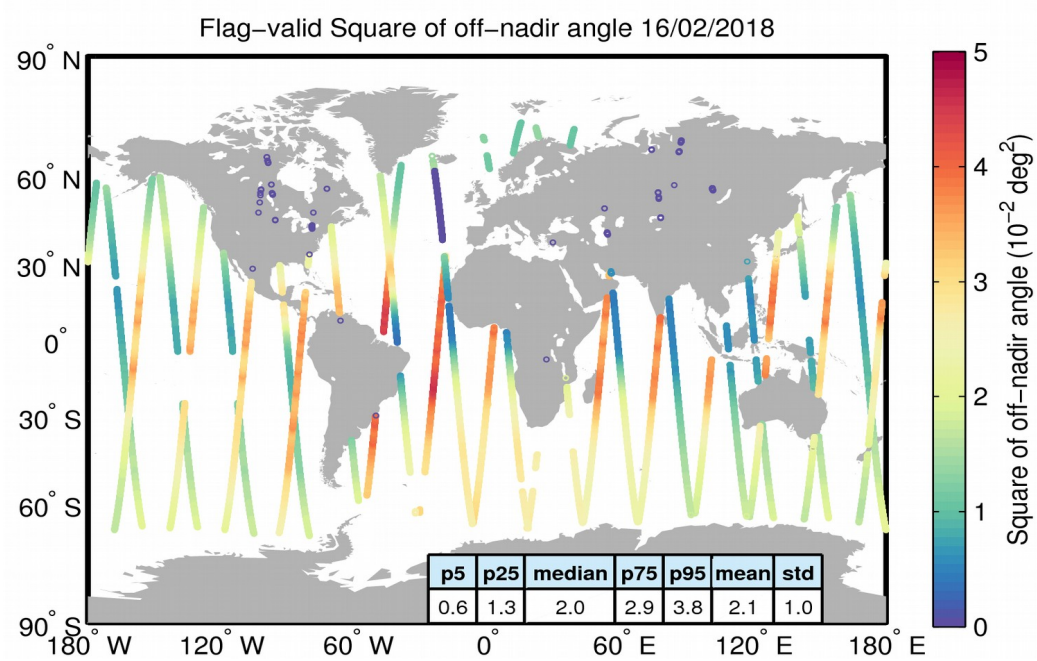
Figure 37. Geographical distribution of flag-valid mispointing data over oceans and lakes for 16/02/2018. The statistical values shown in the table refer to the mispointing in 10^{-2} deg 2 and are calculated over all measurements shown in the figure.
