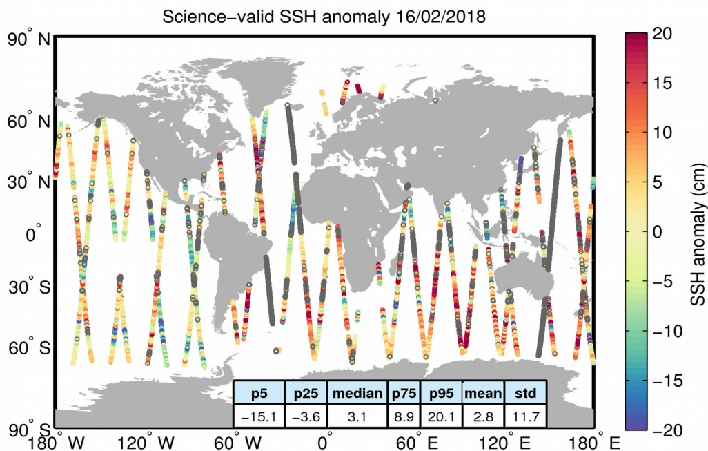
Figure 10. Geographical distribution of science-valid SSH anomaly data over oceans and lakes for 16/02/2018. The statistical values shown in the table refer to the SSH anomaly in cm and are calculated over all measurements shown in the figure. Gray circles denote records that have been rejected based on the editing criteria described in Table 2.
