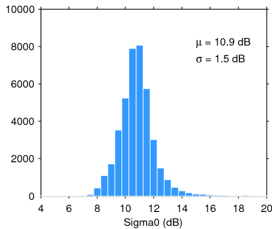
Figure 28. Histogram of science-valid sigma0 over oceans and lakes for 16/02/2018. The mean ( \mu ) and standard deviation ( \sigma ) are also shown. Note that values outside [4 20] dB are excluded from the histogram for the sake of readability but not from the computation of \mu and \sigma .
