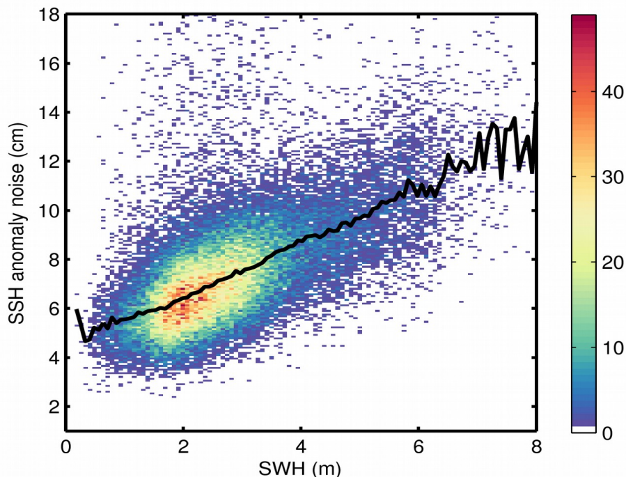
Figure 9. 2D histogram showing flag-valid SSH anomaly noise as a function of SWH for 15/02/2018. The black line denotes the median SSH anomaly noise as a function of SWH.
