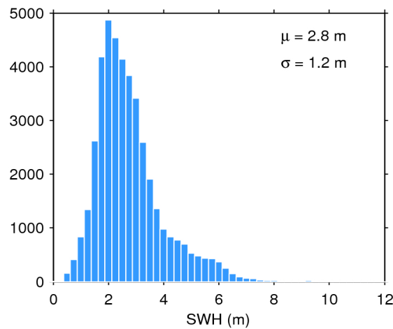
Figure 17. Histogram of flag-valid SWH over oceans and lakes for 15/02/2018. The mean ( \mu ) and standard deviation ( \sigma ) are also shown. Note that values larger than 12 m are excluded from the histogram for the sake of readability but not from the computation of \mu and \sigma .
