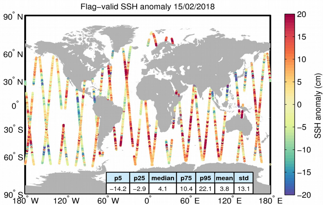
Figure 5. Geographical distribution of flag-valid 1-Hz SSH anomaly data over oceans and lakes for 15/02/2018. The statistical values shown in the table refer to the SSH anomaly in cm and are calculated over all measurements shown in the figure.
