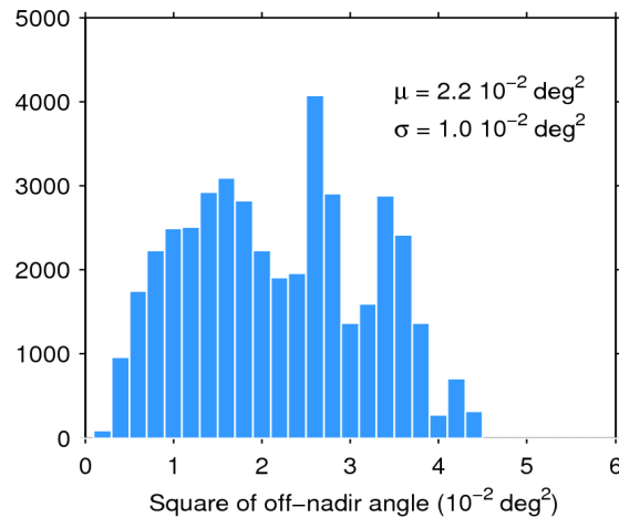
Figure 39. Histogram of flag-valid mispointing over oceans and lakes for 15/02/2018. The mean ( \mu ) and standard deviation ( \sigma ) are also shown. Note that values larger than 6 \cdot 10^{-2} \text{ deg}^2 are excluded from the histogram for the sake of readability but not from the computation of \mu and \sigma .
