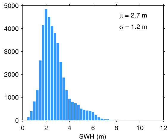
Figure 20. Histogram of science-valid SWH over oceans and lakes for 15/02/2018. The mean ( \mu ) and standard deviation ( \sigma ) are also shown. Note that values larger than 12 m are excluded from the histogram for the sake of readability but not from the computation of \mu and \sigma .
