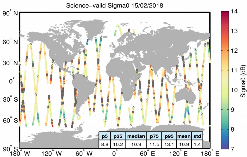
Figure 27. Geographical distribution of science-valid sigma0 data over oceans and lakes for 15/02/2018. The statistical values shown in the table refer to the sigma0 in dB and are calculated over all measurements shown in the figure. Gray circles denote records that have been rejected based on the editing criteria described in Table 4.
