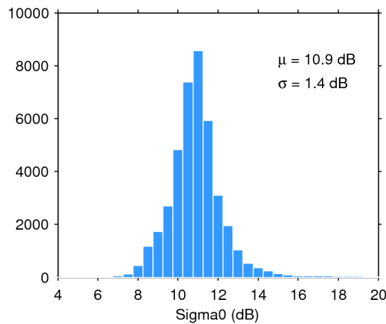
Figure 28. Histogram of science-valid sigma0 over oceans and lakes for 15/02/2018. The mean ( \mu ) and standard deviation ( \sigma ) are also shown. Note that values outside [4 20] dB are excluded from the histogram for the sake of readability but not from the computation of \mu and \sigma .
