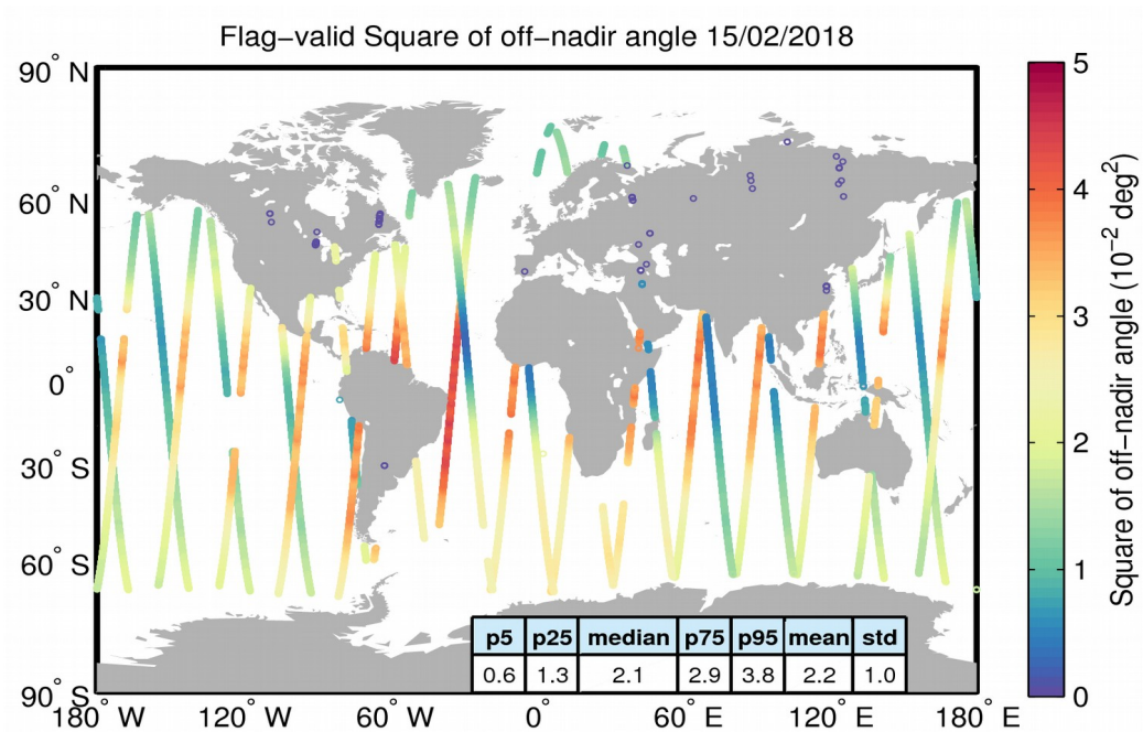
Figure 37. Geographical distribution of flag-valid mispointing data over oceans and lakes for 15/02/2018. The statistical values shown in the table refer to the mispointing in 10^{-2} \text{ deg}^2 and are calculated over all measurements shown in the figure.
