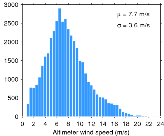
Figure 33. Histogram of flag-valid wind over oceans and lakes for 15/02/2018. The mean ( \mu ) and standard deviation ( \sigma ) are also shown. Note that values larger than 24 m/s are excluded from the histogram for the sake of readability but not from the computation of \mu and \sigma .
