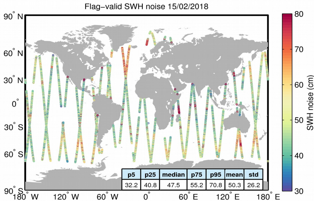
Figure 18. Geographical distribution of flag-valid 20-Hz SWH measurement noise over oceans and lakes for 15/02/2018. The statistical values shown in the figure refer to the SWH noise and are calculated over all measurements shown in the figure.
