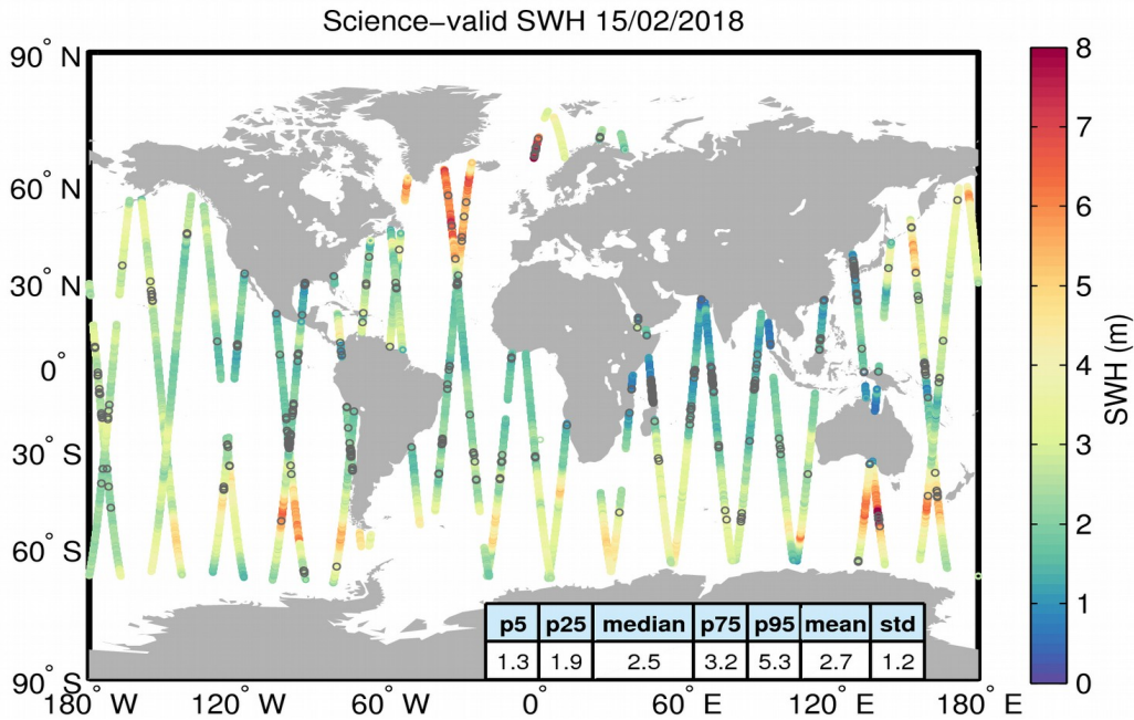
Figure 19. Geographical distribution of science-valid SWH data over oceans and lakes for 15/02/2018. The statistical values shown in the table refer to the SWH in m and are calculated over all measurements shown in the figure. Gray circles denote records that have been rejected based on the editing criteria described in Table 3.
