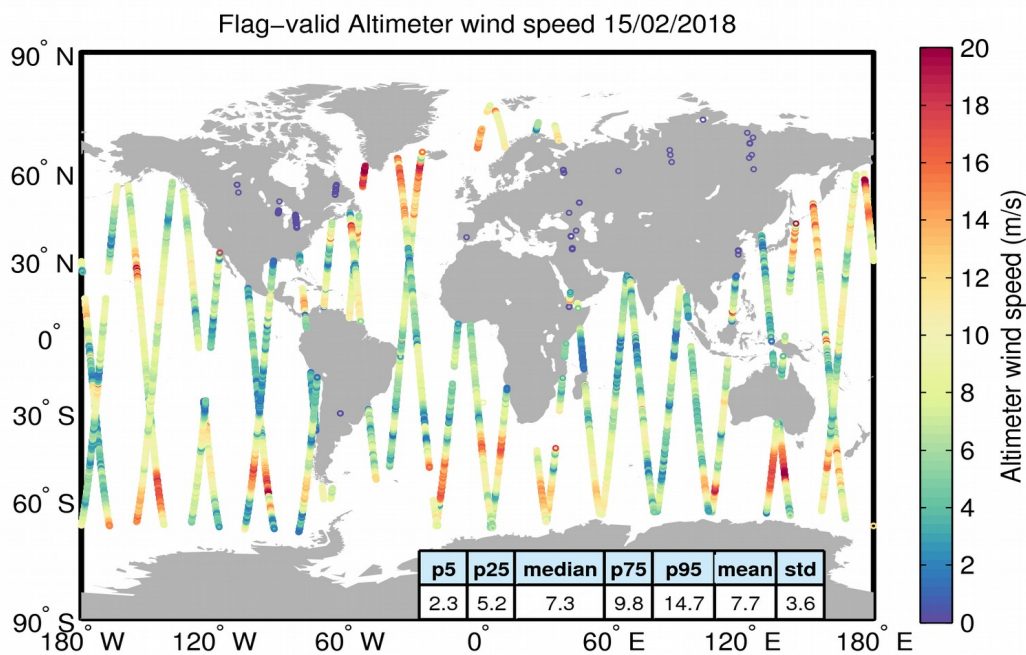
Figure 31. Geographical distribution of flag-valid wind data over oceans and lakes for 15/02/2018. The statistical values shown in the table refer to the wind in m/s and are calculated over all measurements shown in the figure.
