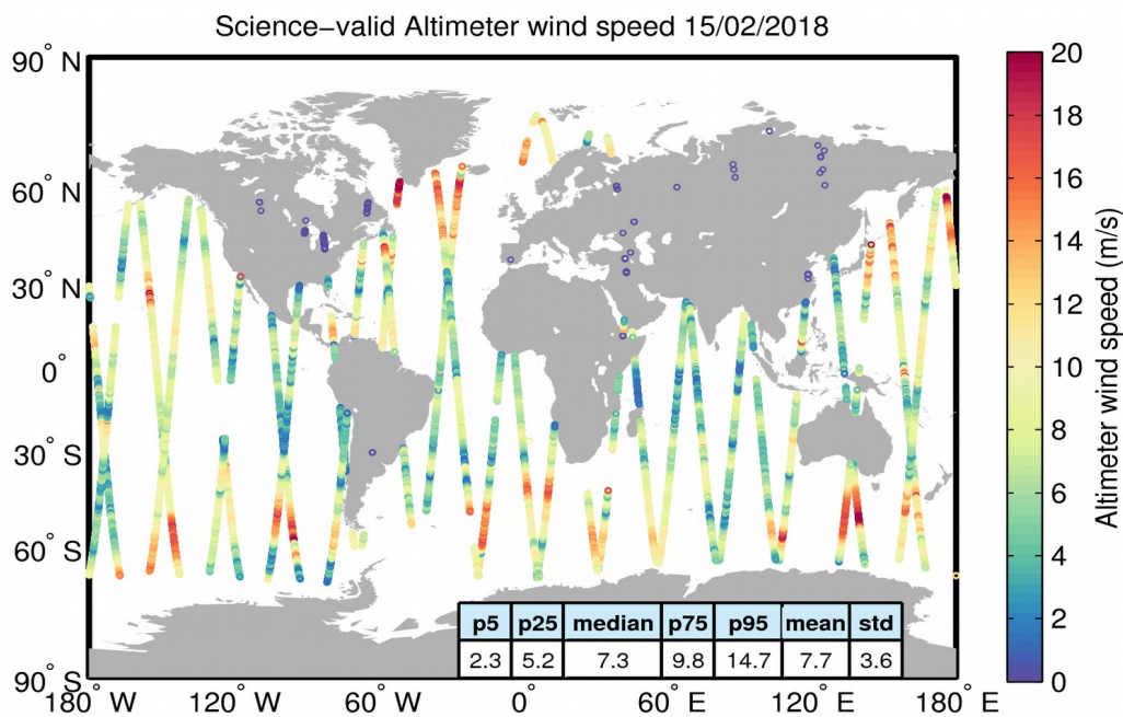
Figure 34. Geographical distribution of science-valid wind data over oceans and lakes for 15/02/2018. The statistical values shown in the table refer to the wind in m/s and are calculated over all measurements shown in the figure. Gray circles denote records that have been rejected based on the editing criteria described in Table 5.
