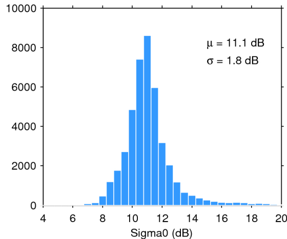
Figure 25. Histogram of flag-valid sigma0 over oceans and lakes for 15/02/2018. The mean ( \mu ) and standard deviation ( \sigma ) are also shown. Note that values outside [4 20] dB are excluded from the histogram for the sake of readability but not from the computation of \mu and \sigma .
