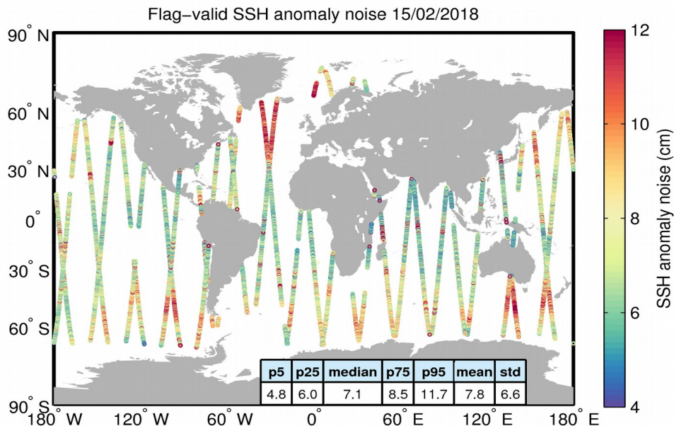
Figure 8. Geographical distribution of flag-valid 20-Hz SSH anomaly measurement noise over oceans and lakes for 15/02/2018. The statistical values shown in the table refer to the SSH anomaly noise and are calculated over all measurements shown in the figure.
