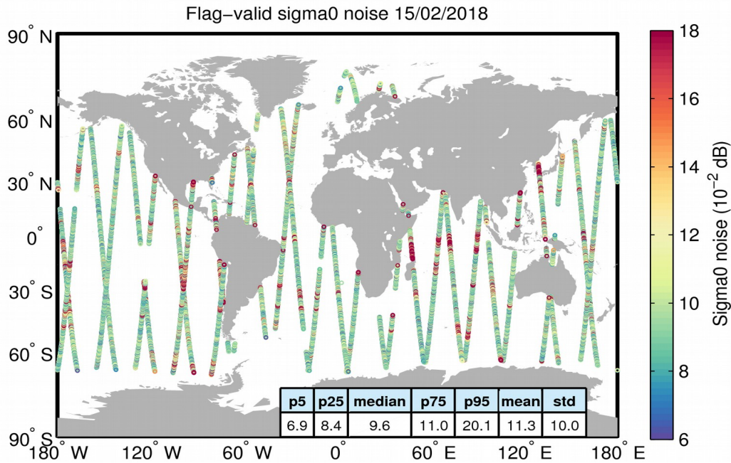
Figure 26. Geographical distribution of flag-valid 20-Hz sigma0 measurement noise over oceans and lakes for 15/02/2018. The statistical values shown in the table refer to the sigma0 noise and are calculated over all measurements shown in the figure.
