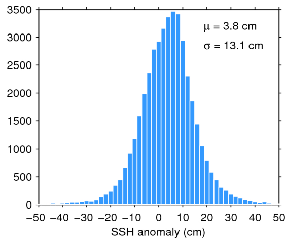
Figure 7. Histogram of flag-valid SSH anomaly over oceans and lakes for 15/02/2018. The mean ( \mu ) and standard deviation ( \sigma ) are also shown. Note that values outside [-50 50] cm are excluded from the histogram for the sake of readability but not from the computation of \mu and \sigma .
