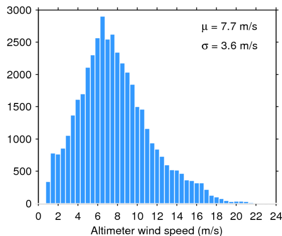
Figure 35. Histogram of science-valid wind over oceans and lakes for 15/02/2018. The mean ( \mu ) and standard deviation ( \sigma ) are also shown. Note that values larger than 24 m/s are excluded from the histogram for the sake of readability but not from the computation of \mu and \sigma .
