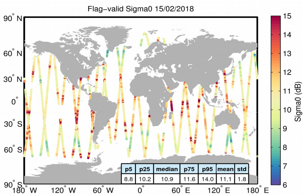
Figure 23. Geographical distribution of flag-valid sigma0 data over oceans and lakes for 15/02/2018. The statistical values shown in the table refer to the sigma0 in dB and are calculated over all measurements shown in the figure.
