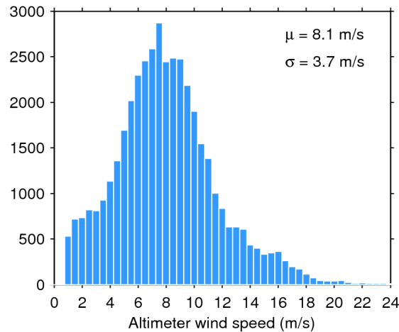
Figure 33. Histogram of flag-valid wind over oceans and lakes for 14/02/2018. The mean ( \mu ) and standard deviation ( \sigma ) are also shown. Note that values larger than 24 m/s are excluded from the histogram for the sake of readability but not from the computation of \mu and \sigma .
