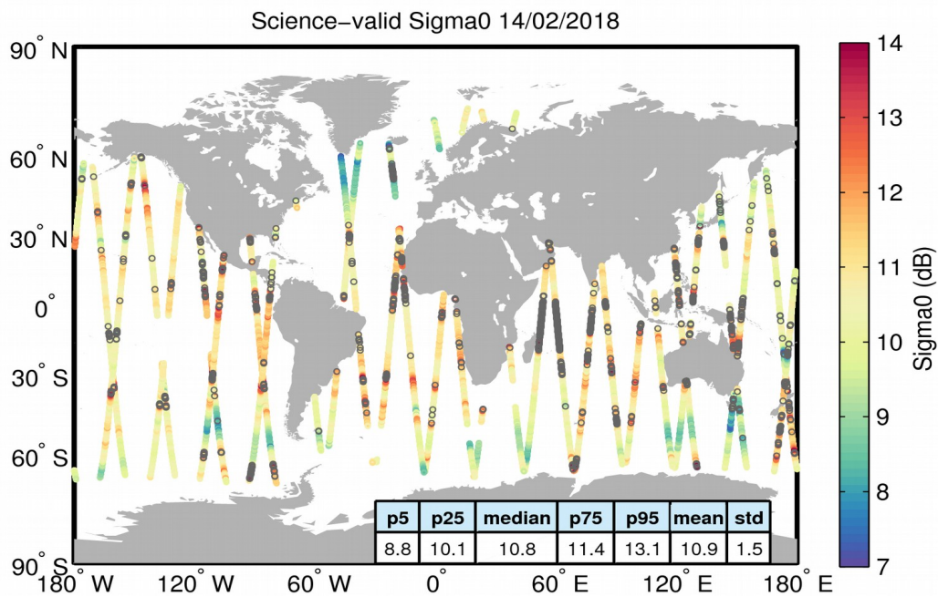
Figure 27. Geographical distribution of science-valid sigma0 data over oceans and lakes for 14/02/2018. The statistical values shown in the table refer to the sigma0 in dB and are calculated over all measurements shown in the figure. Gray circles denote records that have been rejected based on the editing criteria described in Table 4.
