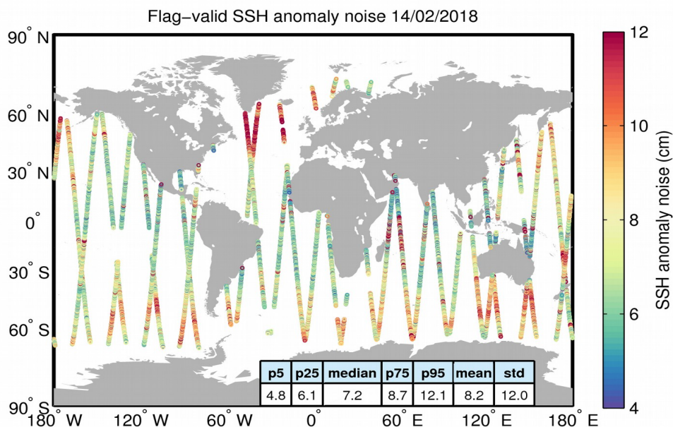
Figure 8. Geographical distribution of flag-valid 20-Hz SSH anomaly measurement noise over oceans and lakes for 14/02/2018. The statistical values shown in the table refer to the SSH anomaly noise and are calculated over all measurements shown in the figure.
