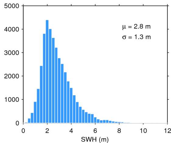
Figure 20. Histogram of science-valid SWH over oceans and lakes for 14/02/2018. The mean ( \mu ) and standard deviation ( \sigma ) are also shown. Note that values larger than 12 m are excluded from the histogram for the sake of readability but not from the computation of \mu and \sigma .
