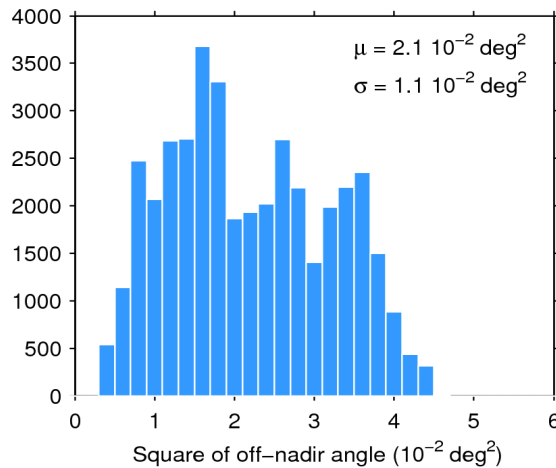
Figure 39. Histogram of flag-valid mispointing over oceans and lakes for 14/02/2018. The mean ( \mu ) and standard deviation ( \sigma ) are also shown. Note that values larger than 6 \cdot 10^{-2} \text{ deg}^2 are excluded from the histogram for the sake of readability but not from the computation of \mu and \sigma .
