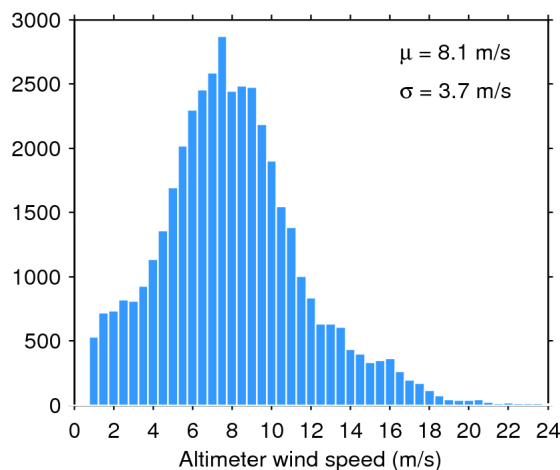
Figure 35. Histogram of science-valid wind over oceans and lakes for 14/02/2018. The mean ( \mu ) and standard deviation ( \sigma ) are also shown. Note that values larger than 24 m/s are excluded from the histogram for the sake of readability but not from the computation of \mu and \sigma .
