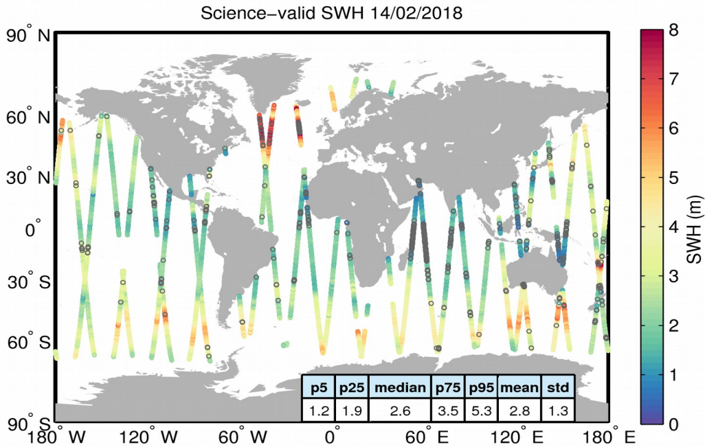
Figure 19. Geographical distribution of science-valid SWH data over oceans and lakes for 14/02/2018. The statistical values shown in the table refer to the SWH in m and are calculated over all measurements shown in the figure. Gray circles denote records that have been rejected based on the editing criteria described in Table 3.
