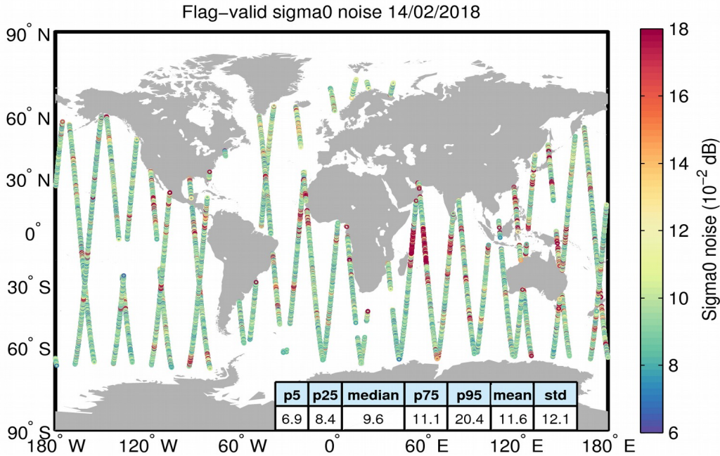
Figure 26. Geographical distribution of flag-valid 20-Hz sigma0 measurement noise over oceans and lakes for 14/02/2018. The statistical values shown in the table refer to the sigma0 noise and are calculated over all measurements shown in the figure.
