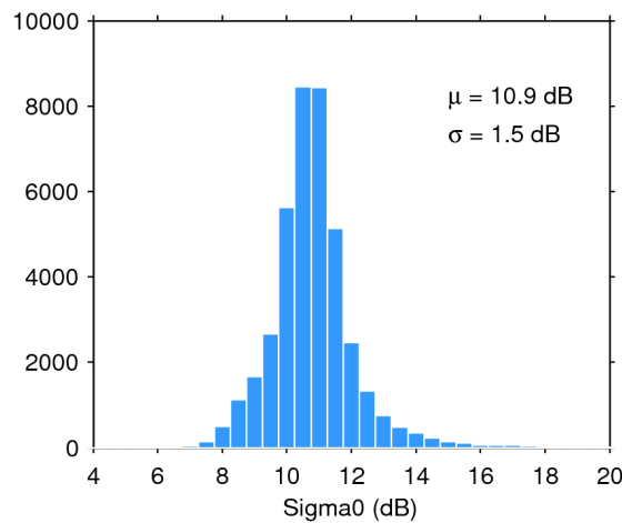
Figure 28. Histogram of science-valid sigma0 over oceans and lakes for 14/02/2018. The mean ( \mu ) and standard deviation ( \sigma ) are also shown. Note that values outside [4 20] dB are excluded from the histogram for the sake of readability but not from the computation of \mu and \sigma .
