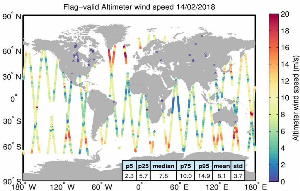
Figure 31. Geographical distribution of flag-valid wind data over oceans and lakes for 14/02/2018. The statistical values shown in the table refer to the wind in m/s and are calculated over all measurements shown in the figure.
