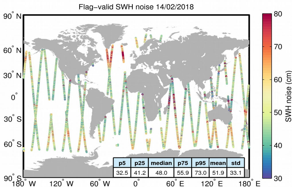
Figure 18. Geographical distribution of flag-valid 20-Hz SWH measurement noise over oceans and lakes for 14/02/2018. The statistical values shown in the figure refer to the SWH noise and are calculated over all measurements shown in the figure.
