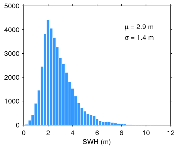
Figure 17. Histogram of flag-valid SWH over oceans and lakes for 14/02/2018. The mean ( \mu ) and standard deviation ( \sigma ) are also shown. Note that values larger than 12 m are excluded from the histogram for the sake of readability but not from the computation of \mu and \sigma .
