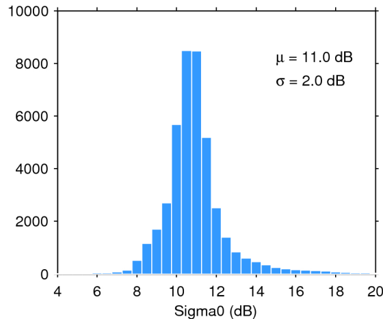
Figure 25. Histogram of flag-valid sigma0 over oceans and lakes for 14/02/2018. The mean ( \mu ) and standard deviation ( \sigma ) are also shown. Note that values outside [4 20] dB are excluded from the histogram for the sake of readability but not from the computation of \mu and \sigma .
