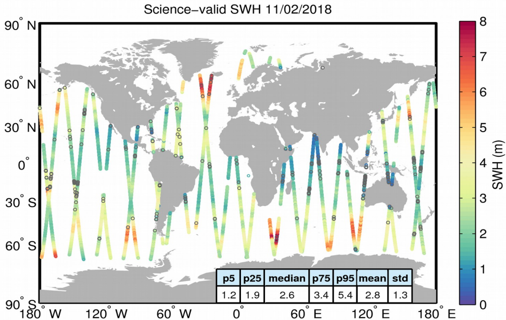
Figure 19. Geographical distribution of science-valid SWH data over oceans and lakes for 11/02/2018. The statistical values shown in the table refer to the SWH in m and are calculated over all measurements shown in the figure. Gray circles denote records that have been rejected based on the editing criteria described in Table 3.
