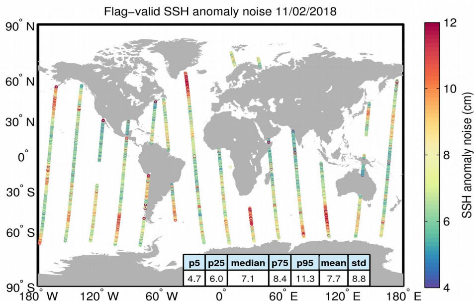
Figure 8. Geographical distribution of flag-valid 20-Hz SSH anomaly measurement noise over oceans and lakes for 11/02/2018. The statistical values shown in the table refer to the SSH anomaly noise and are calculated over all measurements shown in the figure.
