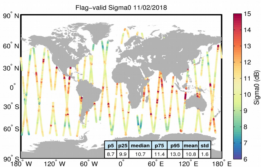
Figure 23. Geographical distribution of flag-valid sigma0 data over oceans and lakes for 11/02/2018. The statistical values shown in the table refer to the sigma0 in dB and are calculated over all measurements shown in the figure.
