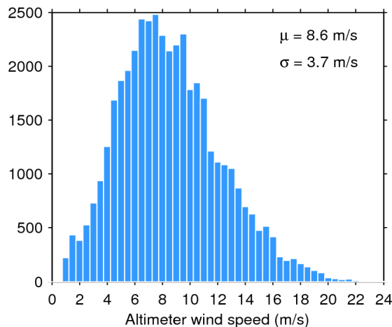
Figure 33. Histogram of flag-valid wind over oceans and lakes for 11/02/2018. The mean ( \mu ) and standard deviation ( \sigma ) are also shown. Note that values larger than 24 m/s are excluded from the histogram for the sake of readability but not from the computation of \mu and \sigma .
