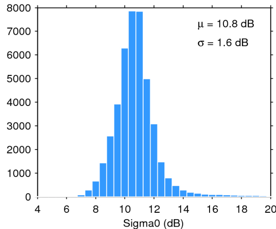
Figure 25. Histogram of flag-valid sigma0 over oceans and lakes for 11/02/2018. The mean ( \mu ) and standard deviation ( \sigma ) are also shown. Note that values outside [4 20] dB are excluded from the histogram for the sake of readability but not from the computation of \mu and \sigma .
