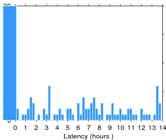
Figure 2. Histogram of the data latency for 11/02/2018. The y-axis denotes the number of files that are made available with a delay of x-hours with respect to the mean time of the records stored in the file.
