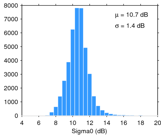
Figure 28. Histogram of science-valid sigma0 over oceans and lakes for 11/02/2018. The mean ( \mu ) and standard deviation ( \sigma ) are also shown. Note that values outside [4 20] dB are excluded from the histogram for the sake of readability but not from the computation of \mu and \sigma .
