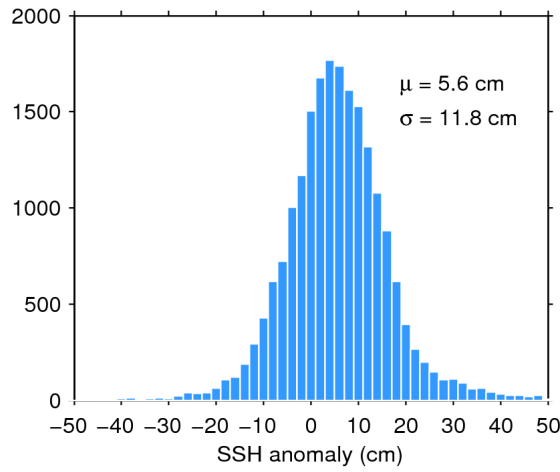
Figure 11. Histogram of science-valid SSH anomaly over oceans and lakes for 11/02/2018. The mean ( \mu ) and standard deviation ( \sigma ) are also shown. Note that values outside [-50 50] cm are excluded from the histogram for the sake of readability but not from the computation of \mu and \sigma .
