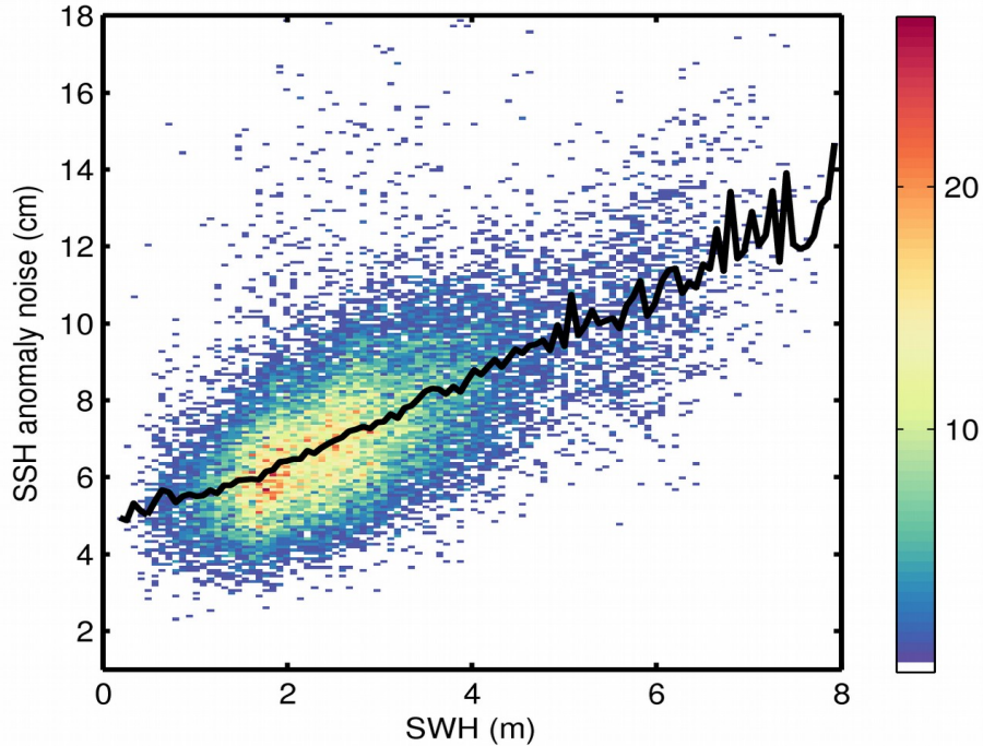
Figure 9. 2D histogram showing flag-valid SSH anomaly noise as a function of SWH for 11/02/2018. The black line denotes the median SSH anomaly noise as a function of SWH.
