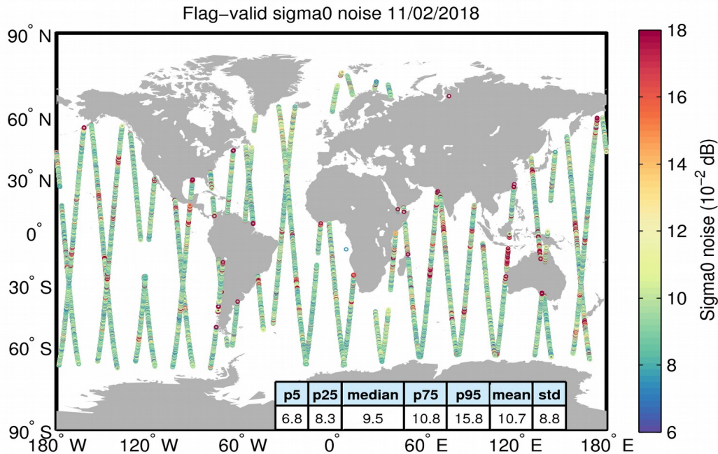
Figure 26. Geographical distribution of flag-valid 20-Hz sigma0 measurement noise over oceans and lakes for 11/02/2018. The statistical values shown in the table refer to the sigma0 noise and are calculated over all measurements shown in the figure.
