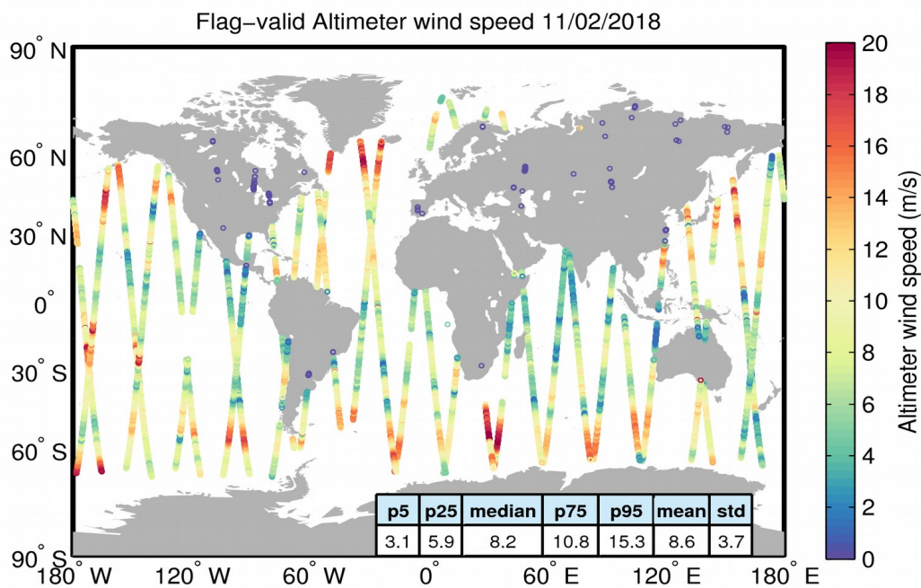
Figure 31. Geographical distribution of flag-valid wind data over oceans and lakes for 11/02/2018. The statistical values shown in the table refer to the wind in m/s and are calculated over all measurements shown in the figure.
