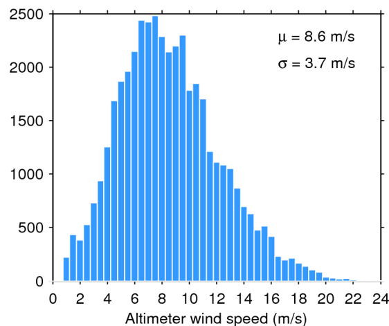
Figure 35. Histogram of science-valid wind over oceans and lakes for 11/02/2018. The mean ( \mu ) and standard deviation ( \sigma ) are also shown. Note that values larger than 24 m/s are excluded from the histogram for the sake of readability but not from the computation of \mu and \sigma .
