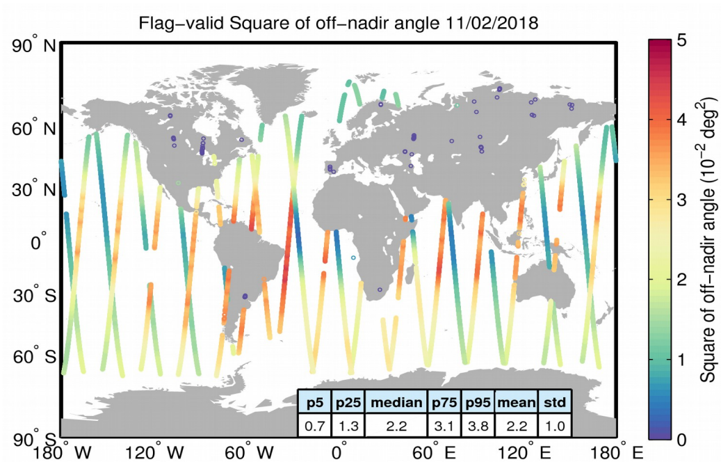
Figure 37. Geographical distribution of flag-valid mispointing data over oceans and lakes for 11/02/2018. The statistical values shown in the table refer to the mispointing in 10^{-2} \text{ deg}^2 and are calculated over all measurements shown in the figure.
