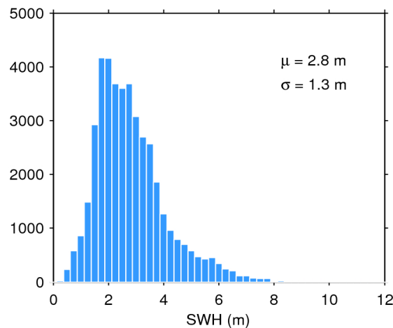
Figure 20. Histogram of science-valid SWH over oceans and lakes for 11/02/2018. The mean ( \mu ) and standard deviation ( \sigma ) are also shown. Note that values larger than 12 m are excluded from the histogram for the sake of readability but not from the computation of \mu and \sigma .
