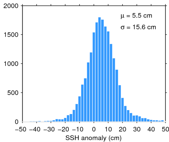
Figure 7. Histogram of flag-valid SSH anomaly over oceans and lakes for 11/02/2018. The mean ( \mu ) and standard deviation ( \sigma ) are also shown. Note that values outside [-50\ 50] cm are excluded from the histogram for the sake of readability but not from the computation of \mu and \sigma .
