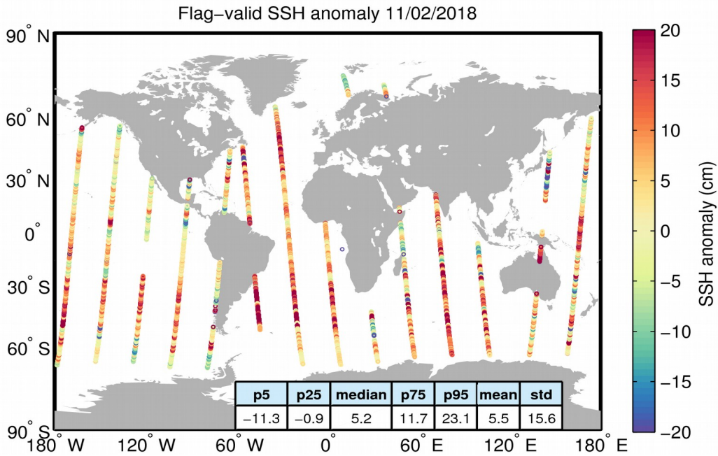
Figure 5. Geographical distribution of flag-valid 1-Hz SSH anomaly data over oceans and lakes for 11/02/2018. The statistical values shown in the table refer to the SSH anomaly in cm and are calculated over all measurements shown in the figure.
