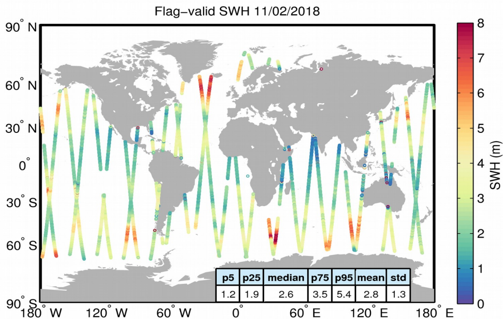
Figure 15. Geographical distribution of flag-valid SWH data over oceans and lakes for 11/02/2018. The statistical values shown in the table refer to the SWH in m and are calculated over all measurements shown in the figure.
