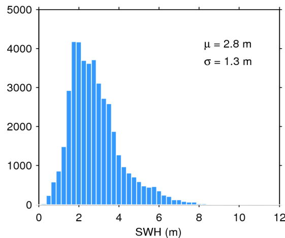
Figure 17. Histogram of flag-valid SWH over oceans and lakes for 11/02/2018. The mean ( \mu ) and standard deviation ( \sigma ) are also shown. Note that values larger than 12 m are excluded from the histogram for the sake of readability but not from the computation of \mu and \sigma .
