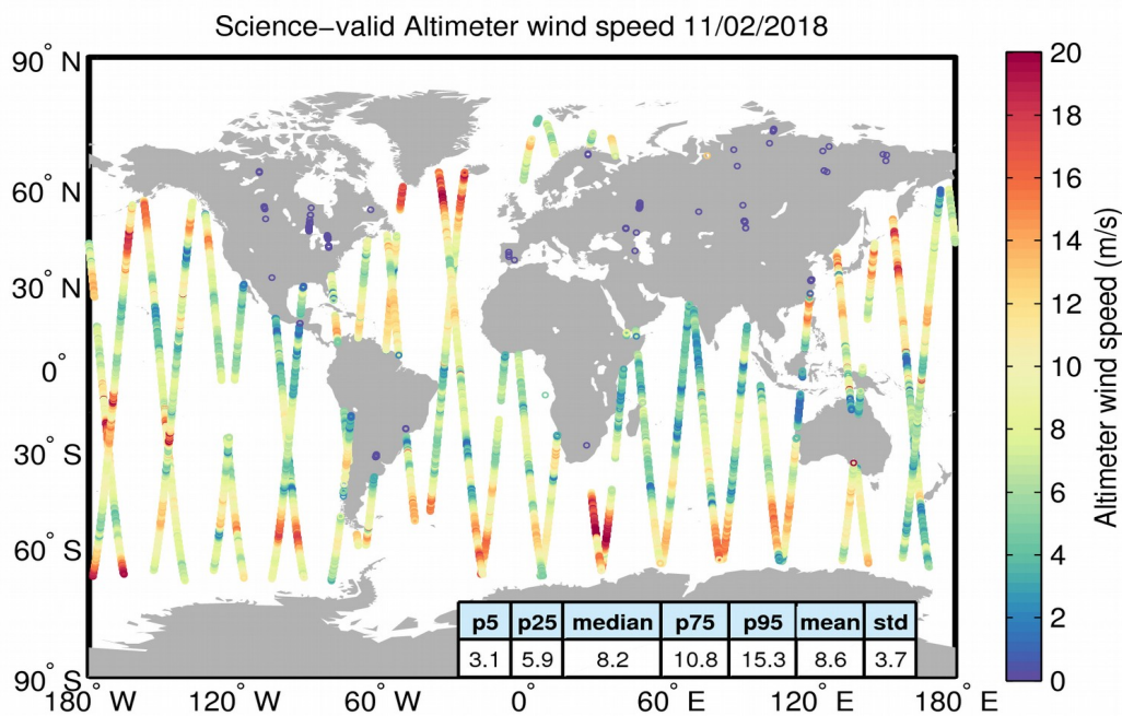
Figure 34. Geographical distribution of science-valid wind data over oceans and lakes for 11/02/2018. The statistical values shown in the table refer to the wind in m/s and are calculated over all measurements shown in the figure. Gray circles denote records that have been rejected based on the editing criteria described in Table 5.
