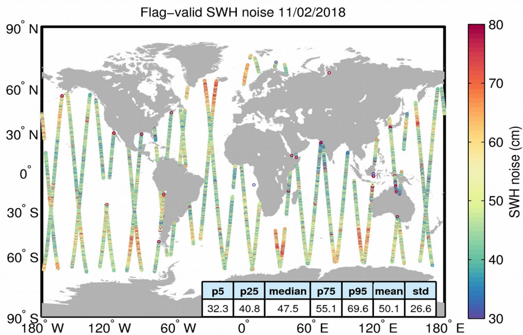
Figure 18. Geographical distribution of flag-valid 20-Hz SWH measurement noise over oceans and lakes for 11/02/2018. The statistical values shown in the figure refer to the SWH noise and are calculated over all measurements shown in the figure.
