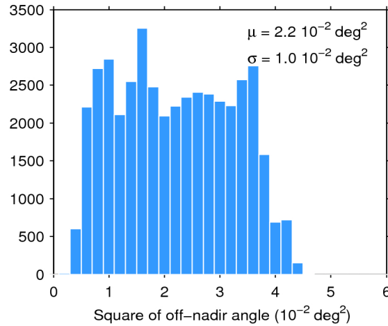
Figure 39. Histogram of flag-valid mispointing over oceans and lakes for 11/02/2018. The mean ( \mu ) and standard deviation ( \sigma ) are also shown. Note that values larger than 6 \cdot 10^{-2} \text{ deg}^2 are excluded from the histogram for the sake of readability but not from the computation of \mu and \sigma .
