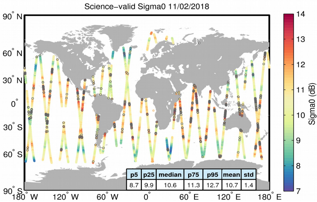
Figure 27. Geographical distribution of science-valid sigma0 data over oceans and lakes for 11/02/2018. The statistical values shown in the table refer to the sigma0 in dB and are calculated over all measurements shown in the figure. Gray circles denote records that have been rejected based on the editing criteria described in Table 4.
